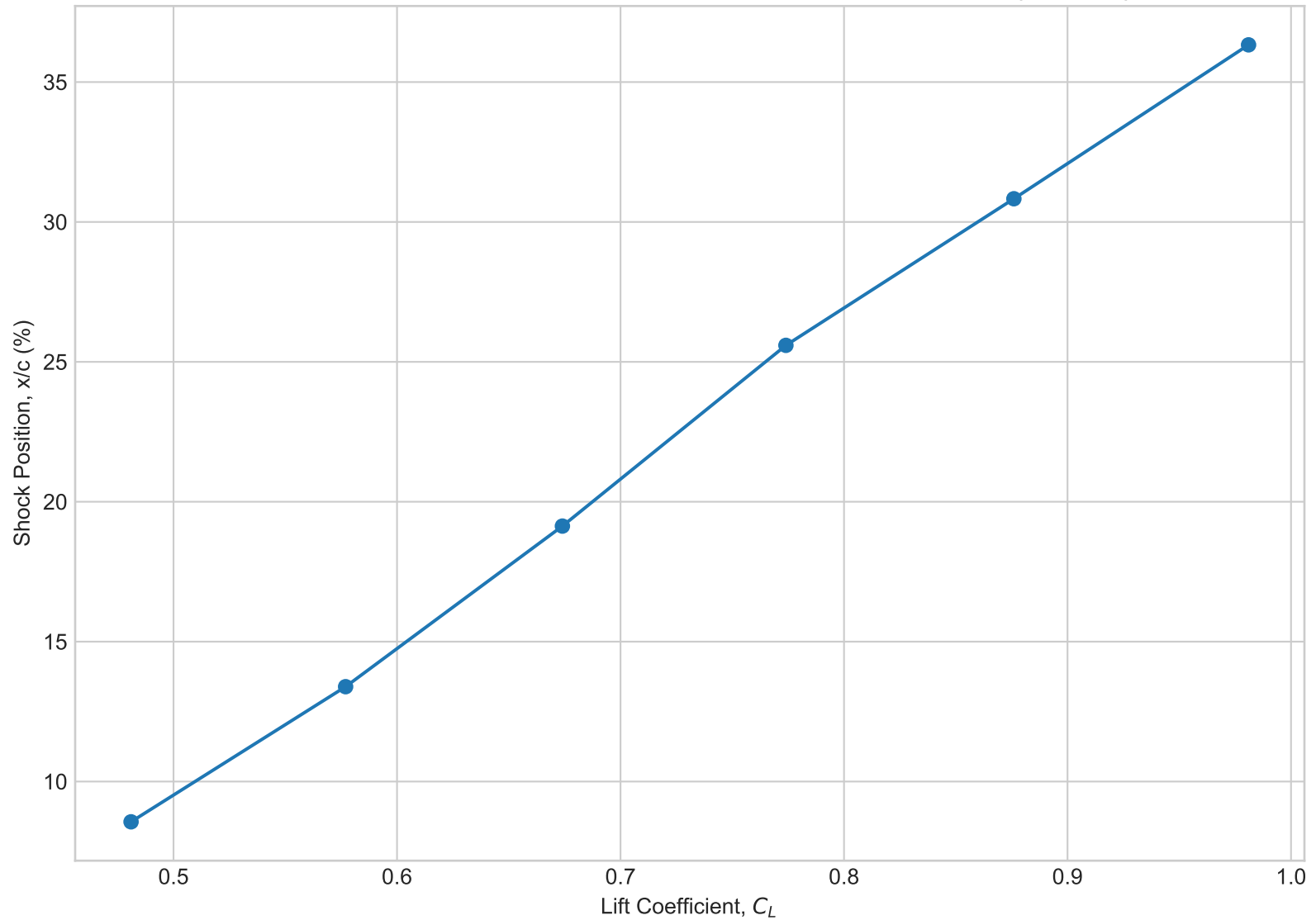
Upper Surface Shock Position vs. Lift Coefficient (M=0.7)
