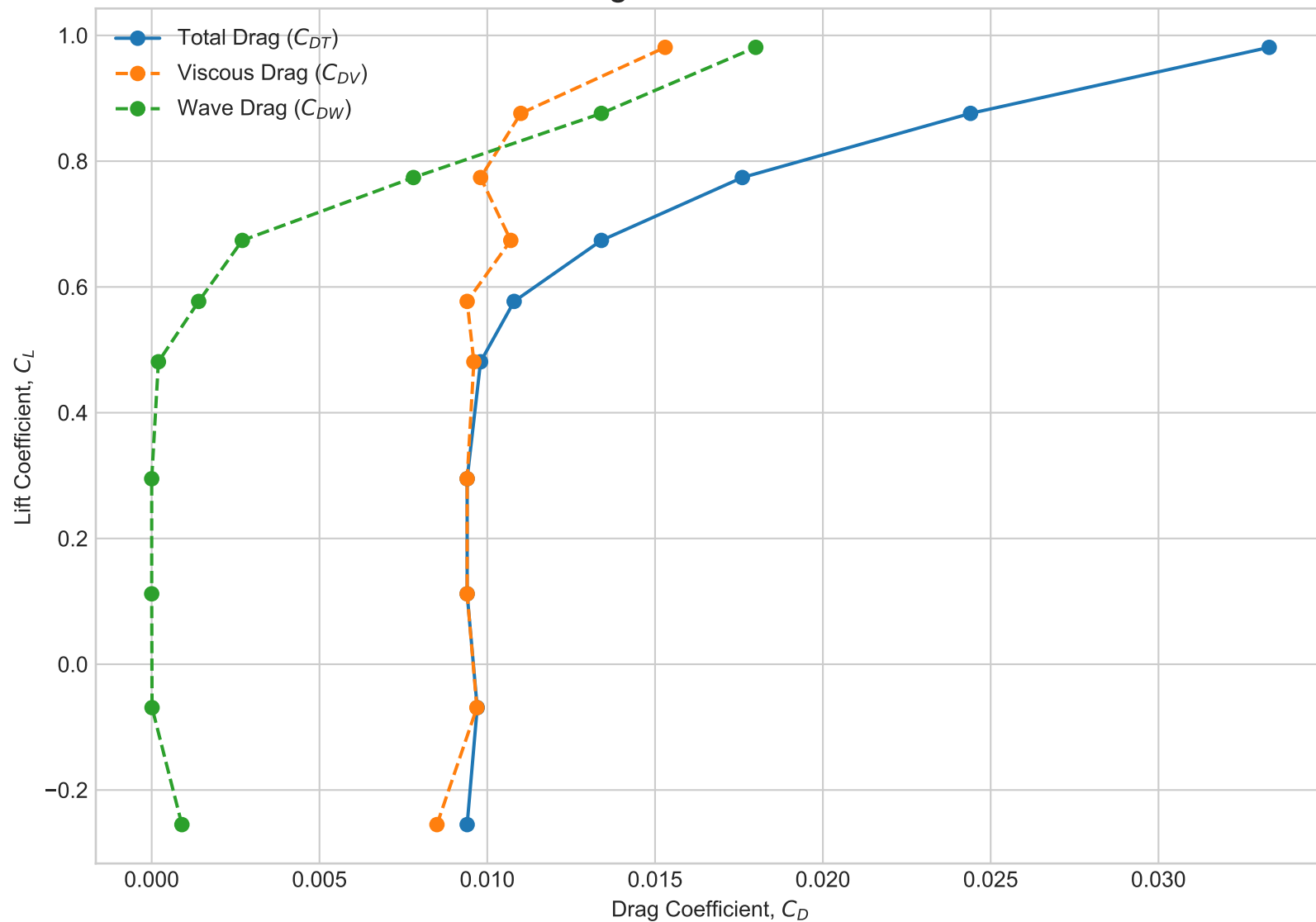
Drag Polar at M=0.7
