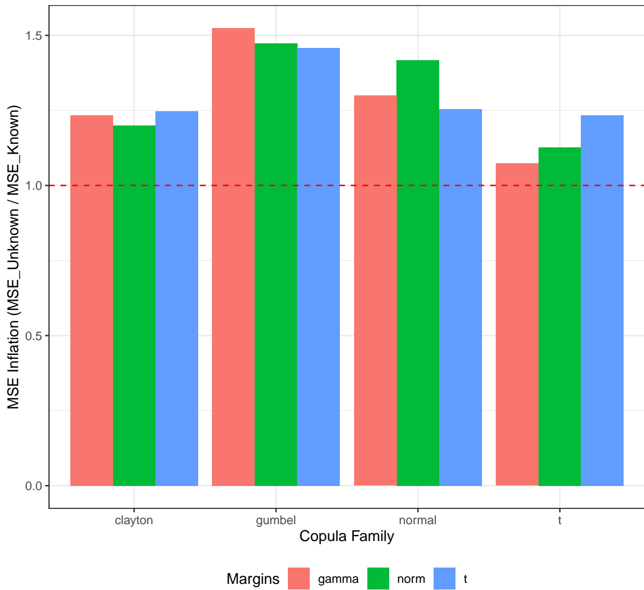
Effect of Copula Family on 'Cost of Ignorance' Grouped by Marginal Distribution (n=200, N_sim=500)
