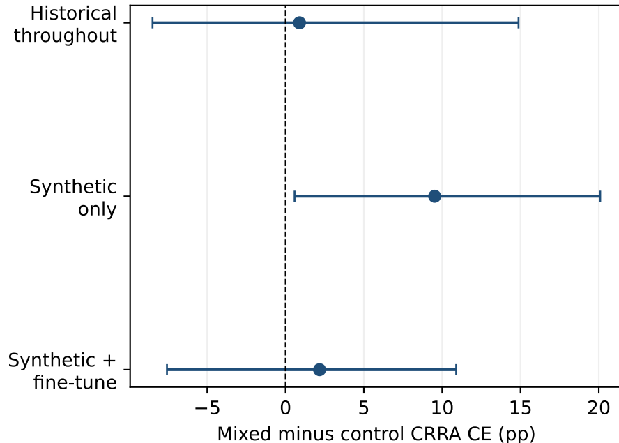
Paired circular-block intervals
