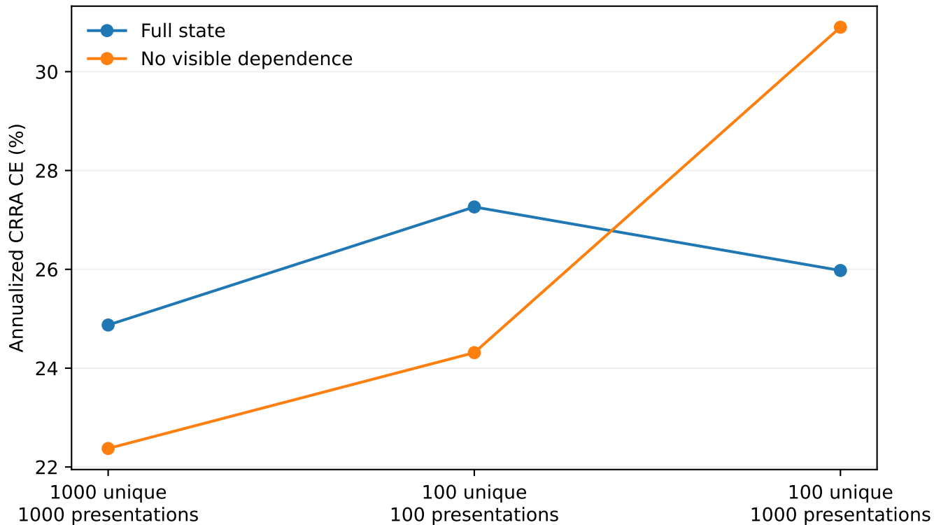
Identification of diversity and presentation mechanisms
