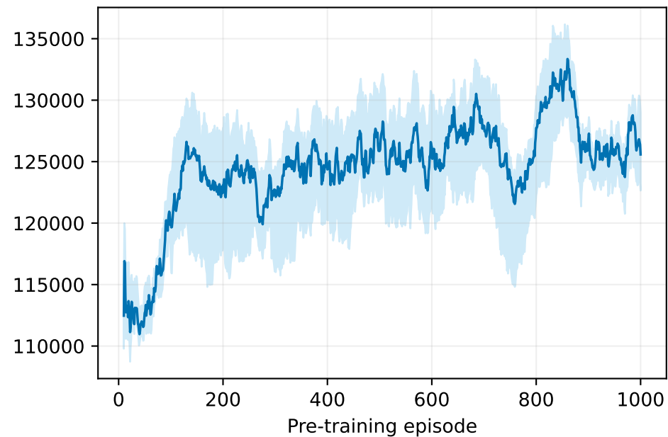
mean gross exposure
