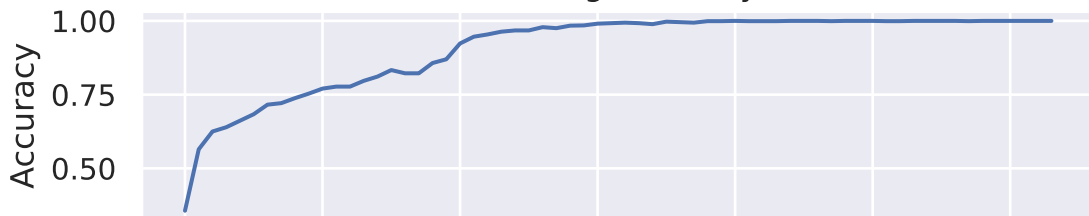
Test accuracy
