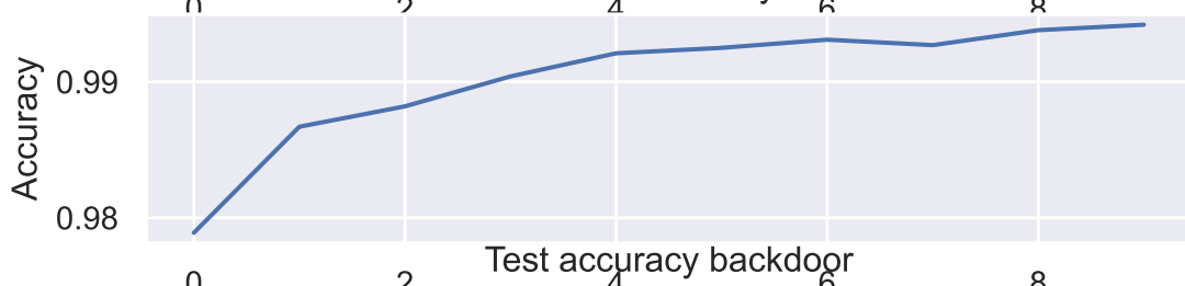
Test accuracy
