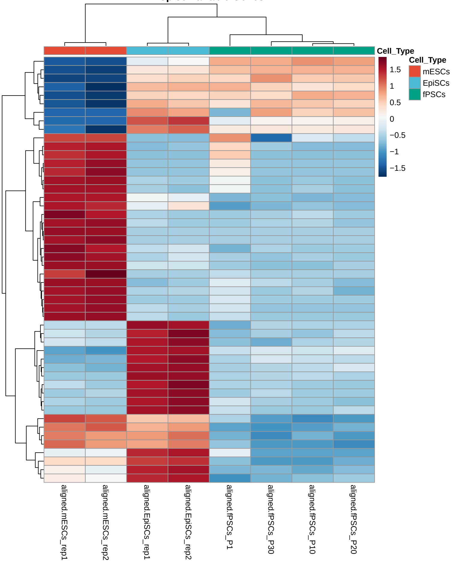
Top 50 Variable Genes
