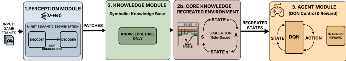
Figure 4.1: The figure illustrates the overall architecture of the system, which consists of three main modules. The Perception Module uses a U-Net for semantic segmentation of raw game frames, extracting structured patches via an encoder-decoder architecture with skip connections. These patches are passed to the Knowledge Module, which builds a symbolic knowledge base and recreates the game environment through a rule-based simulation, producing symbolic states. Finally, the Agent Module will receive these reconstructed states and uses a DQN to select actions, guided by an intrinsic reward signal.
