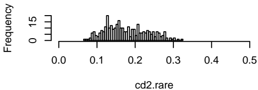
SD distribution E(rho) rare
