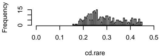
SD distribution rho rare
