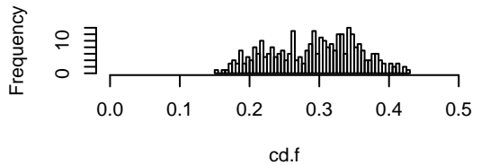
SD distribution Spearman all
