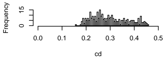
SD distribution rho all
