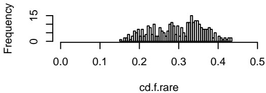
SD distribution Spearman rare
