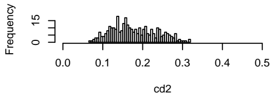
SD distribution E(rho) all
