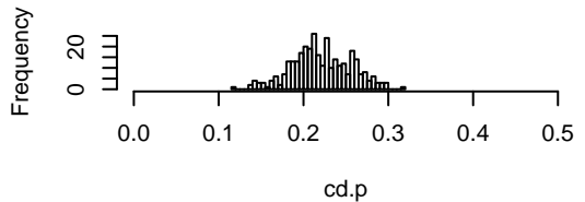
SD distribution Pearson all
