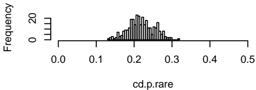
SD distribution Pearson rare
