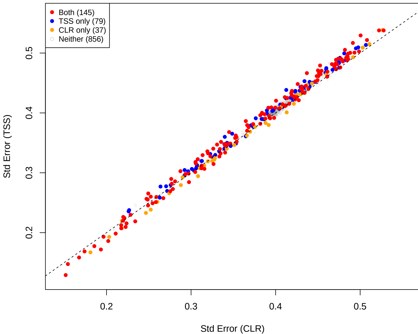
mid vs pup [gamma = 0.1]
