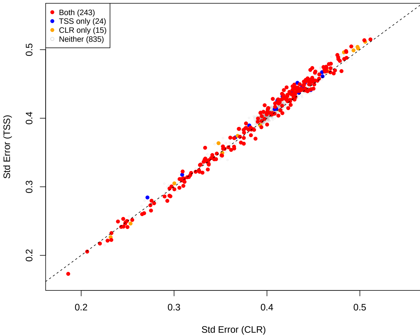
cent vs kin [gamma = 0.1]
