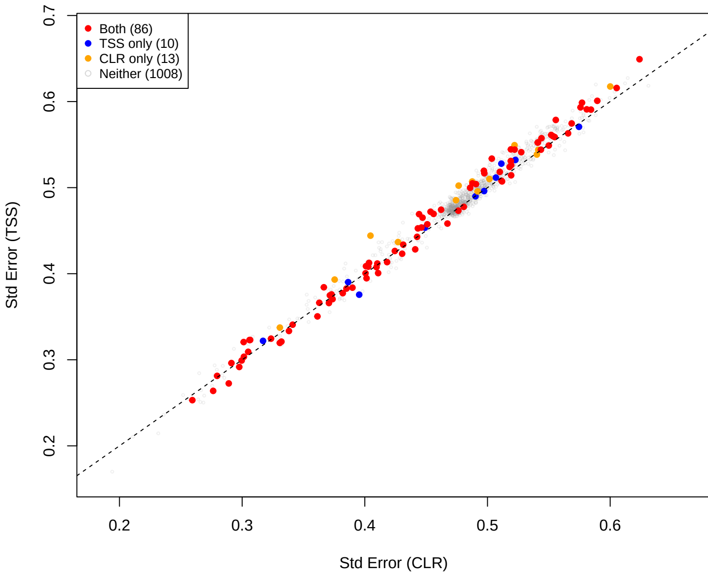
kin vs mage [gamma = 0.1]
