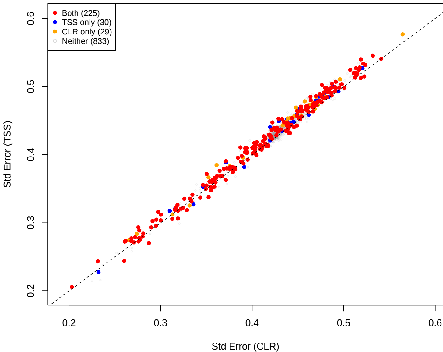
kin vs you [gamma = 0.1]
