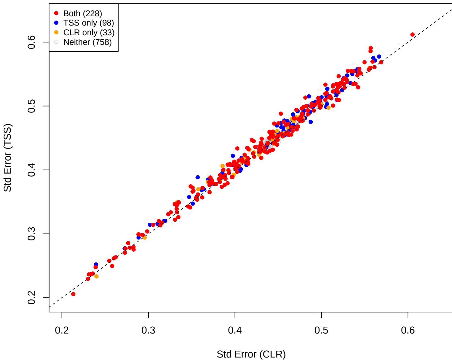
eld vs pup [gamma = 0.1]
