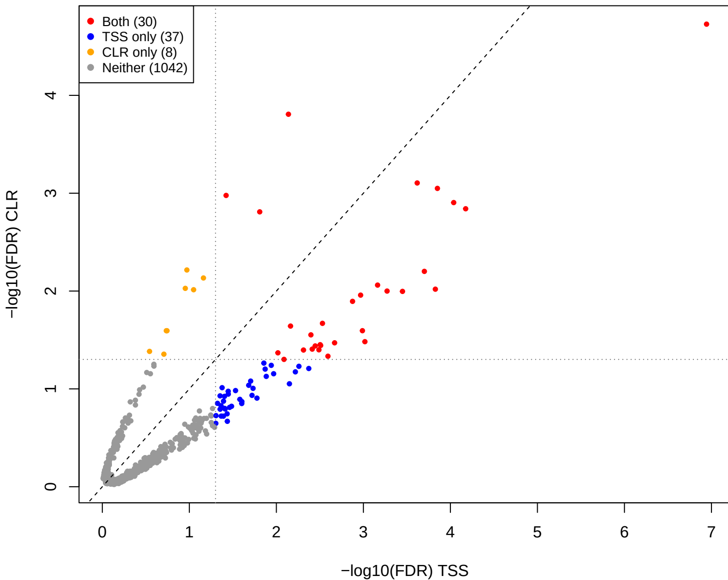
eld vs you – CLR vs TSS (gamma = 0.3)
