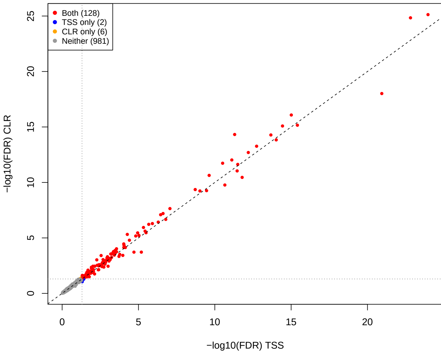
eld vs mid – CLR vs TSS (gamma = 0.3)
