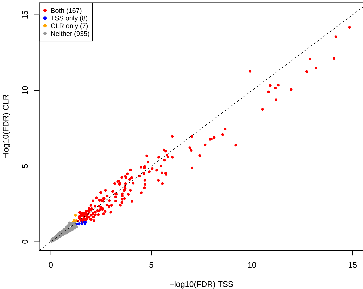
mage vs you - CLR vs TSS (gamma = 0.3)
