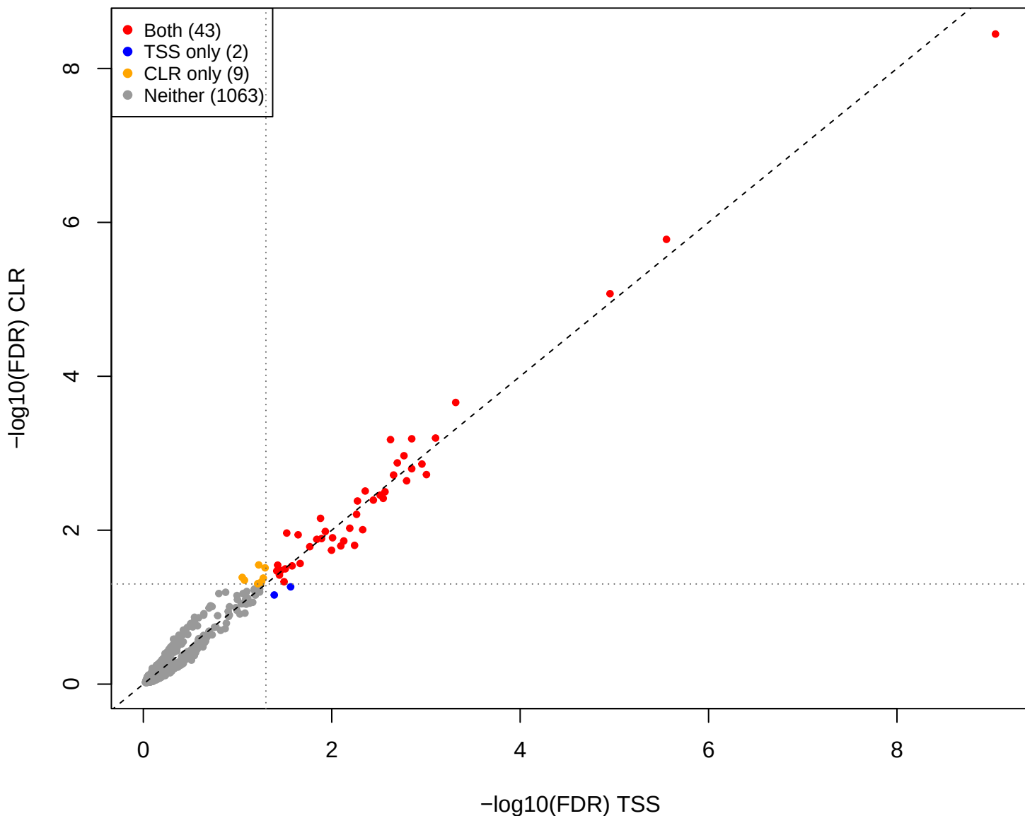
mage vs mid – CLR vs TSS (gamma = 0.3)
