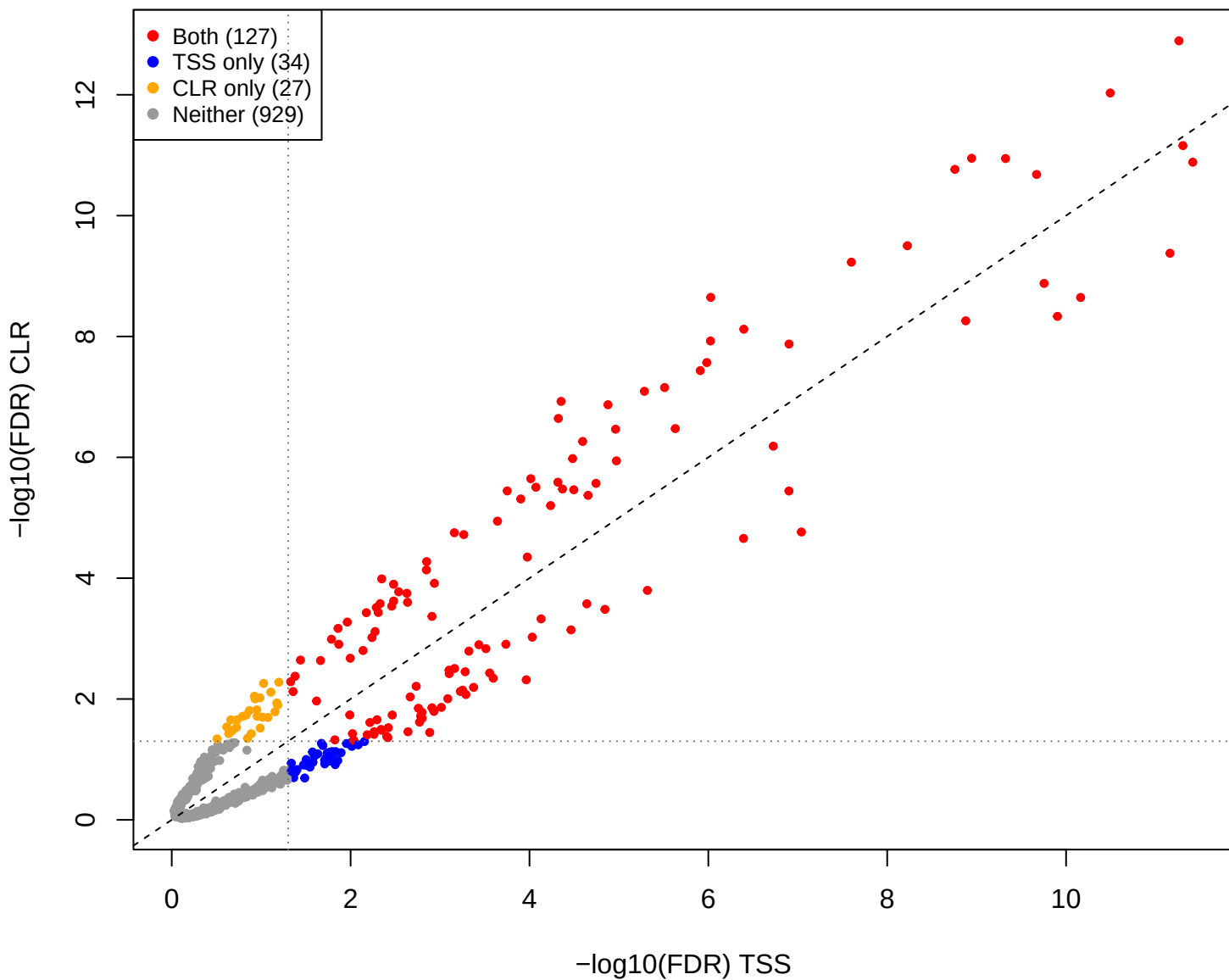
cent vs mage – CLR vs TSS (gamma = 0.3)
