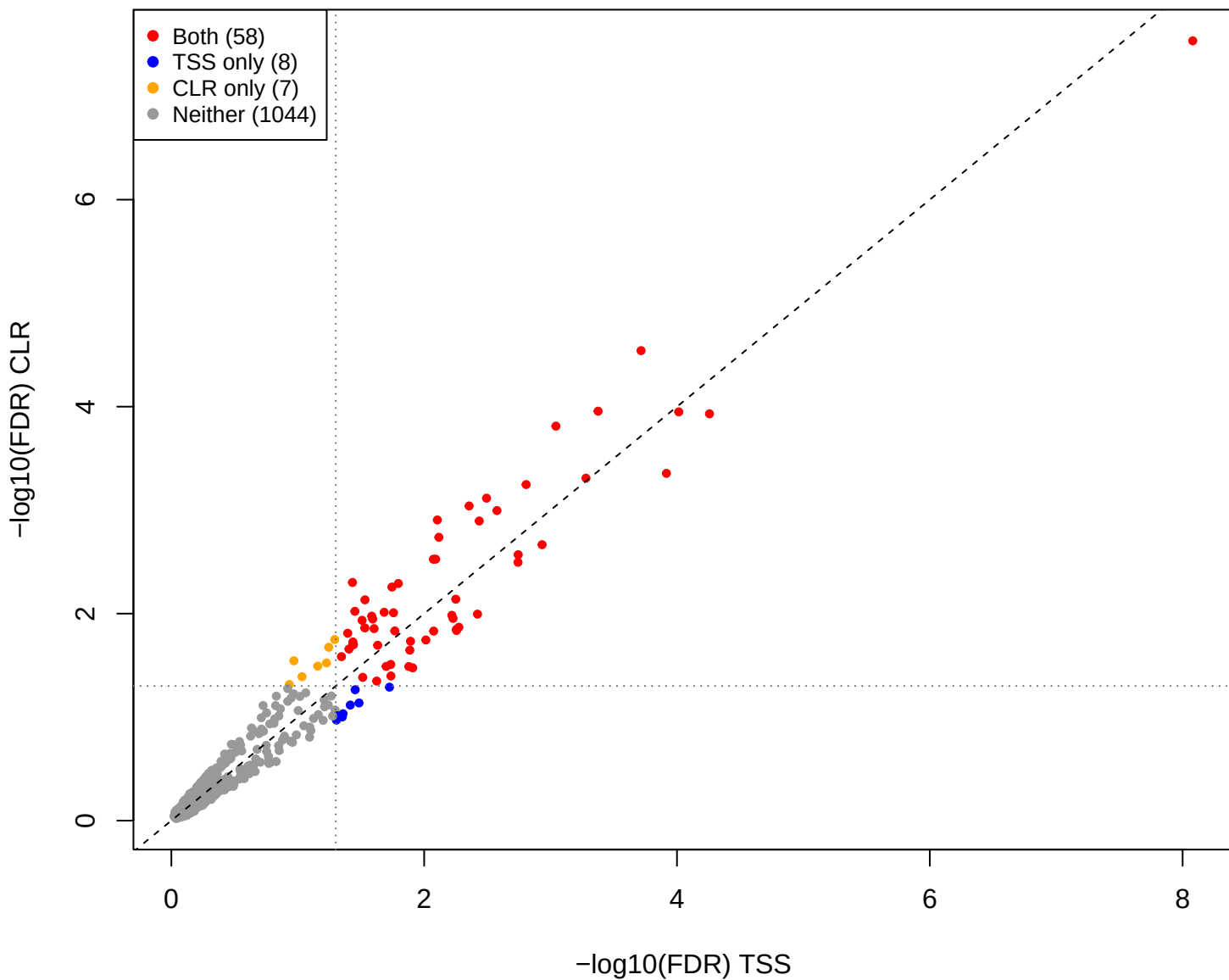
kin vs mage – CLR vs TSS (gamma = 0.3)
