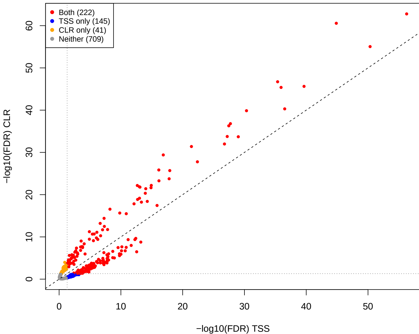
cent vs pup – CLR vs TSS (gamma = 0.3)
