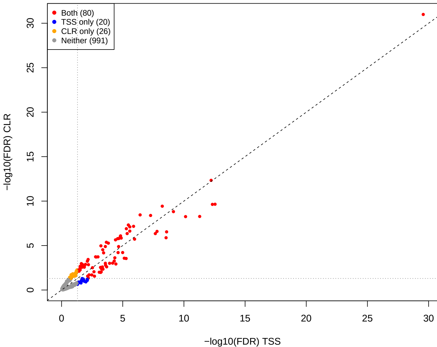
mage vs pup – CLR vs TSS (gamma = 0.3)
