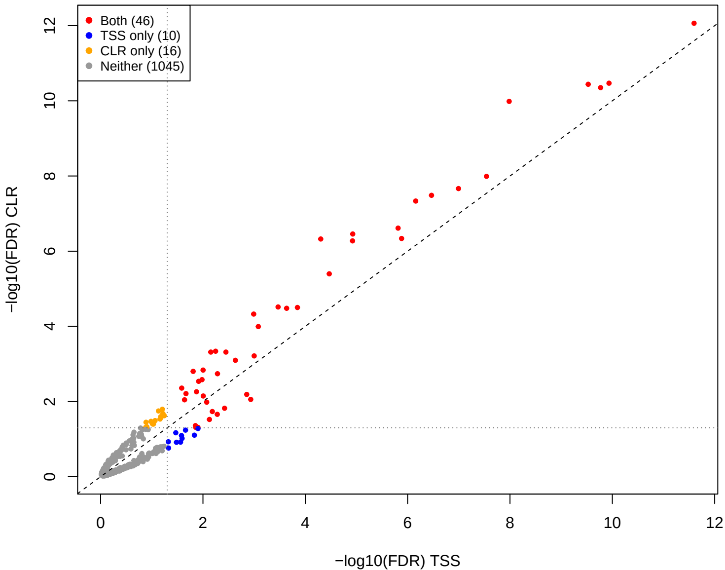
eld vs mage – CLR vs TSS (gamma = 0.3)
