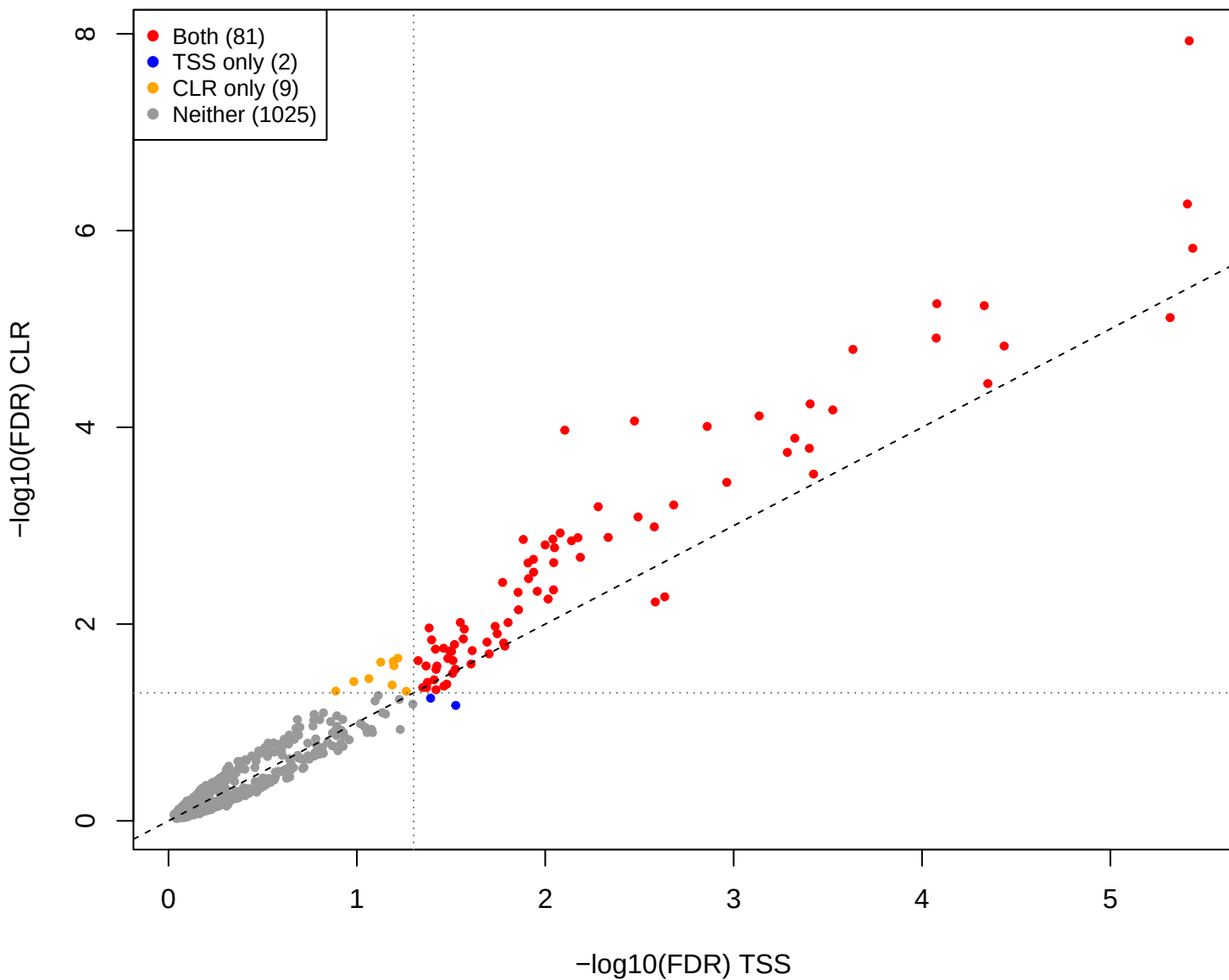
cent vs eld – CLR vs TSS (gamma = 0.3)
