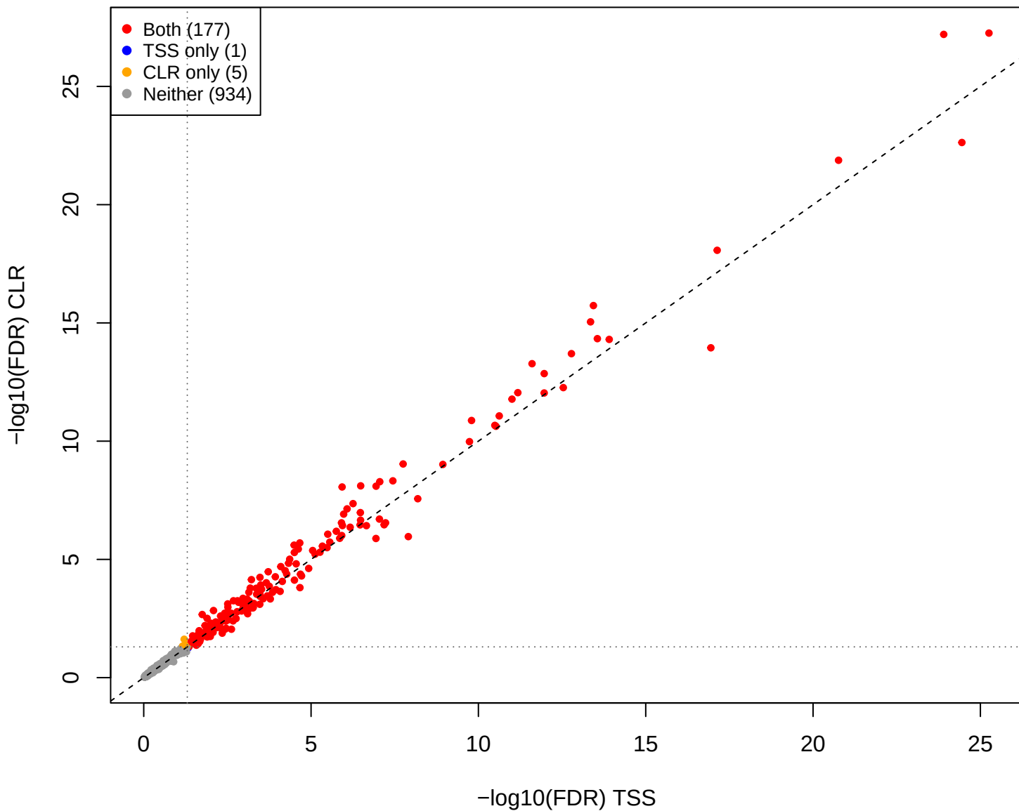
eld vs kin – CLR vs TSS (gamma = 0.3)
