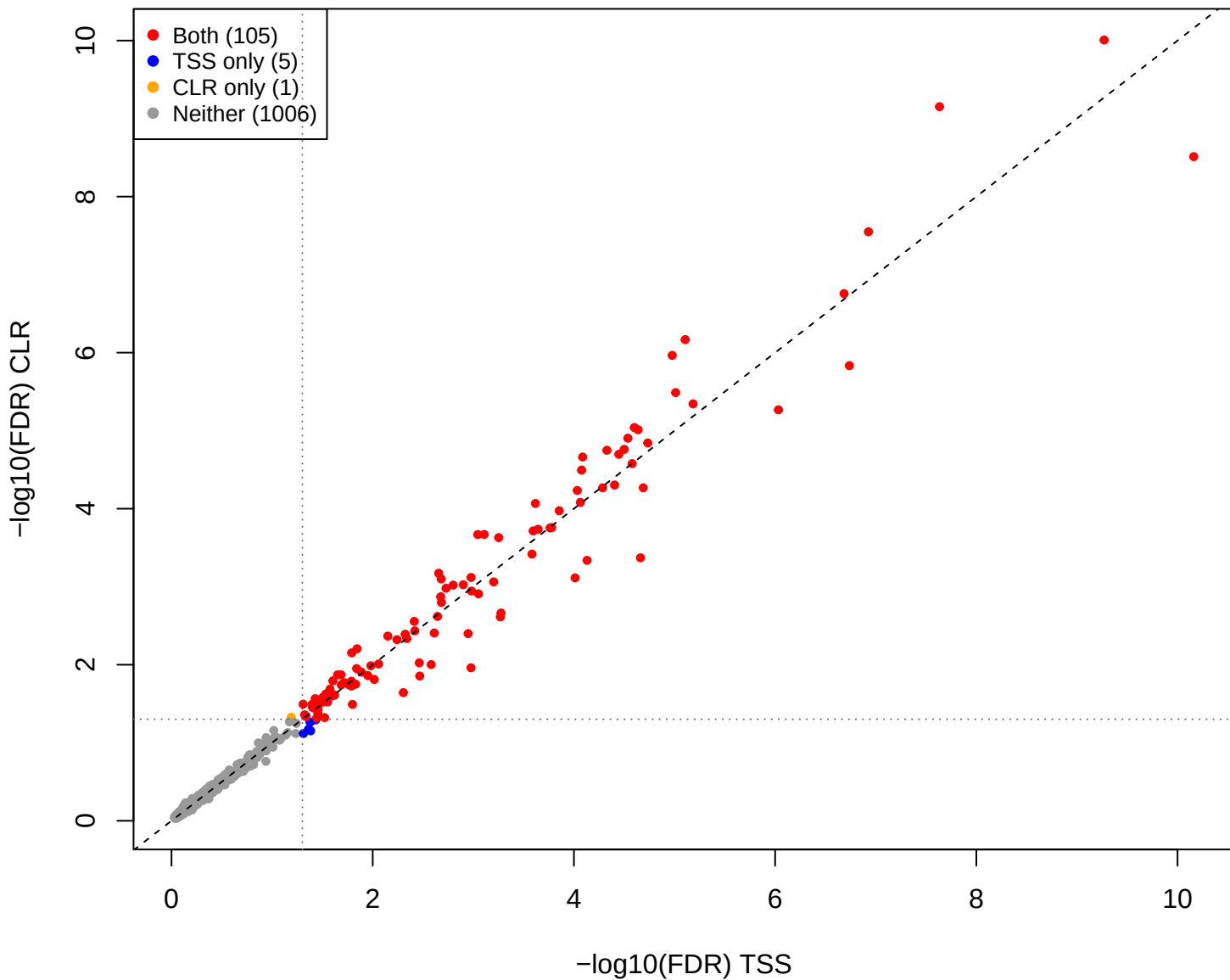
kin vs mid – CLR vs TSS (gamma = 0.3)
