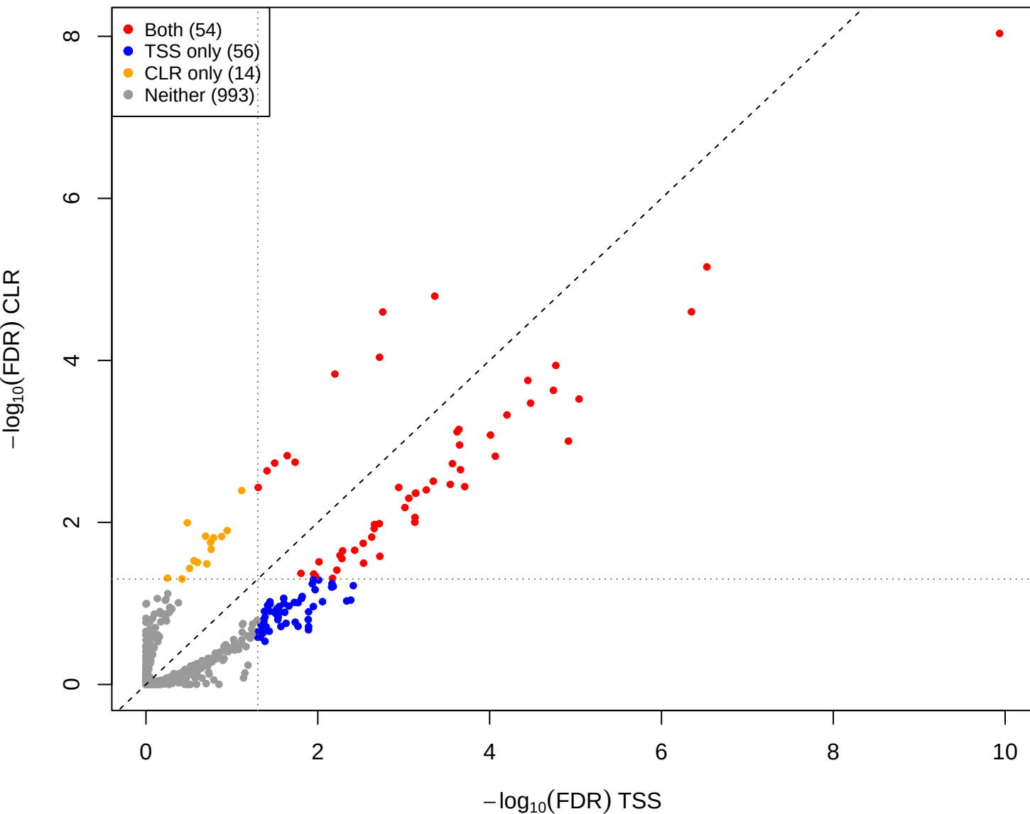
eld vs you – CLR vs TSS (gamma = 1e-05, const = 0)
