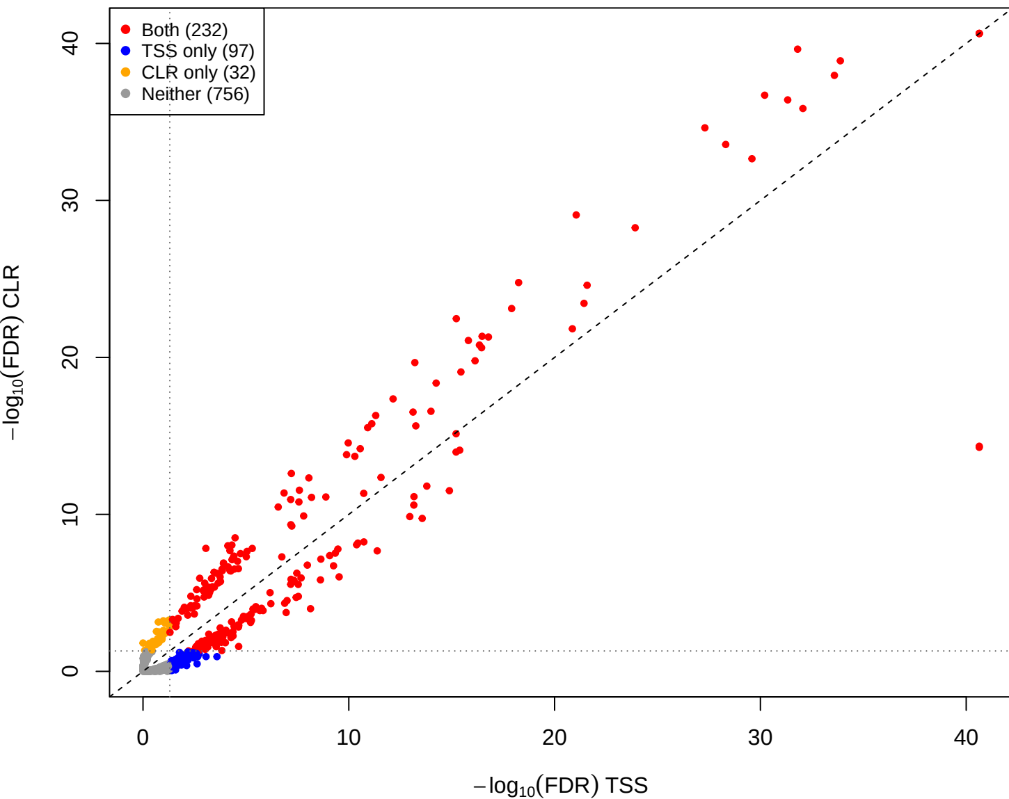
eld vs pup – CLR vs TSS (gamma = 1e-05, const = 0)
