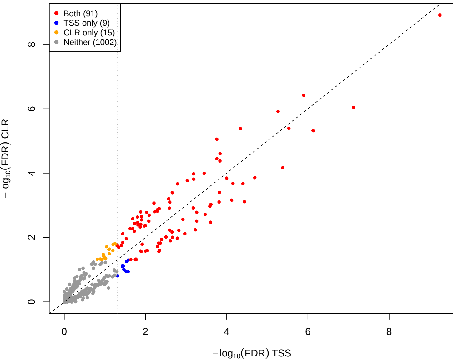
kin vs mage – CLR vs TSS (gamma = 1e-05, const = 0)
