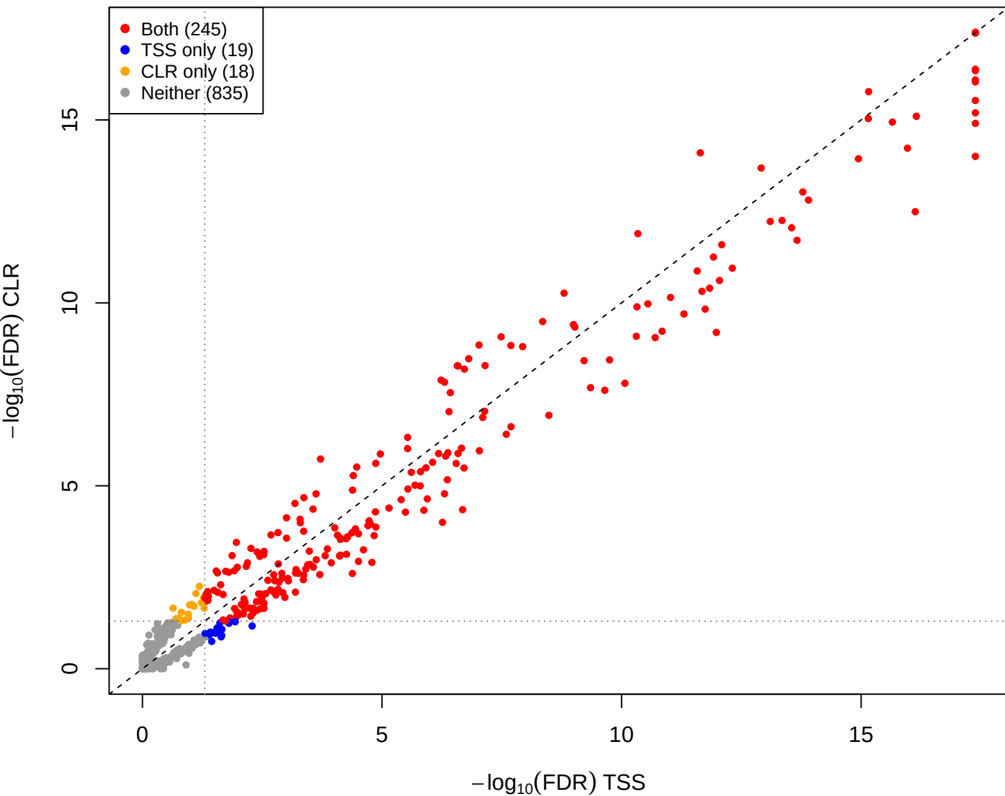
mid vs you – CLR vs TSS (gamma = 1e-05, const = 0)
