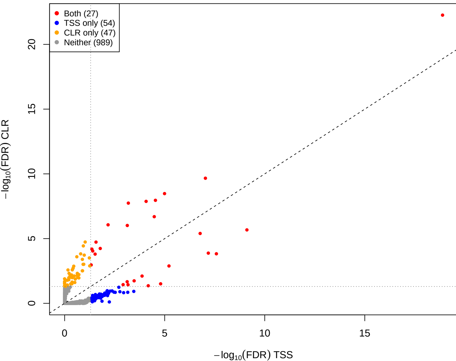
kin vs pup – CLR vs TSS (gamma = 1e-05, const = 0)
