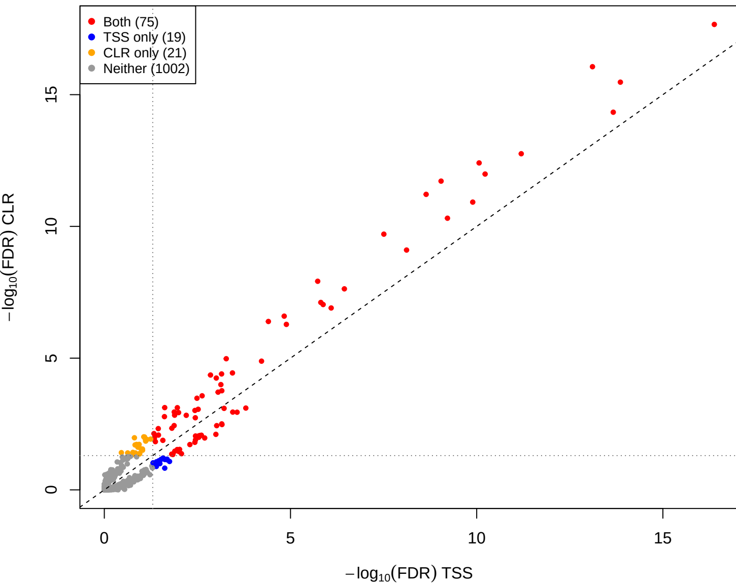
eld vs mage – CLR vs TSS (gamma = 1e-05, const = 0)
