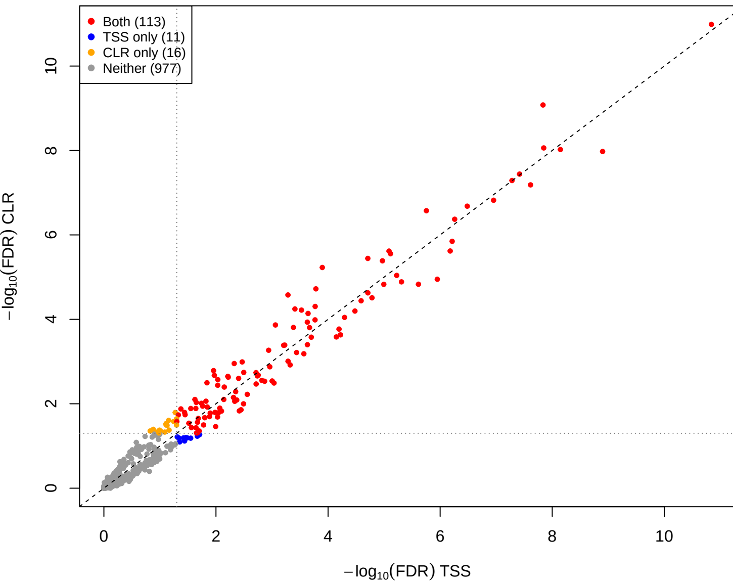
cent vs eld – CLR vs TSS (gamma = 1e-05, const = 0)
