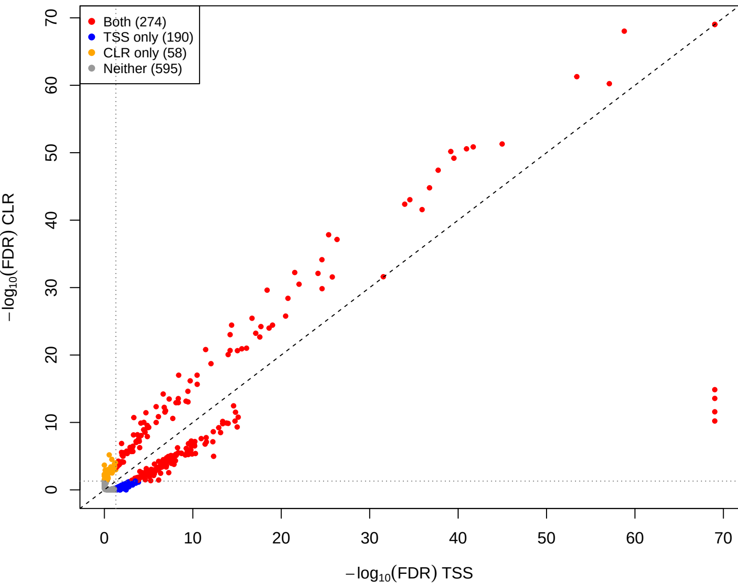
cent vs pup – CLR vs TSS (gamma = 1e-05, const = 0)
