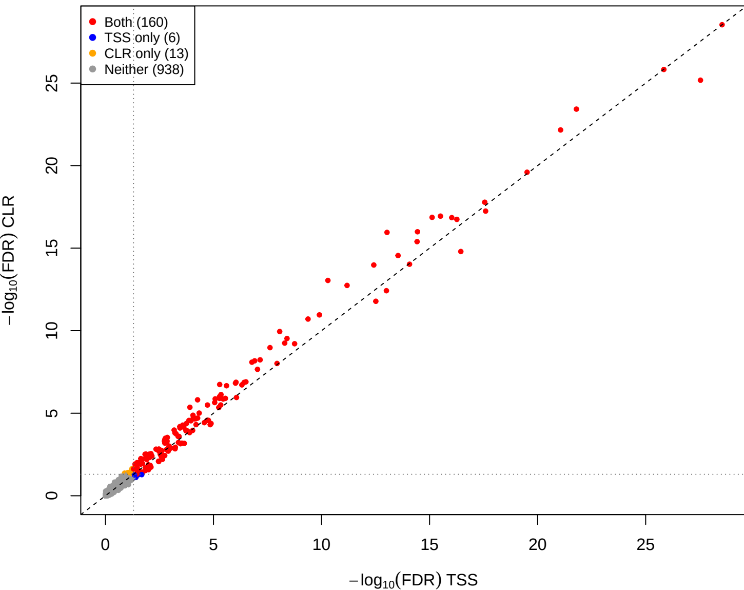
eld vs mid – CLR vs TSS (gamma = 1e-05, const = 0)
