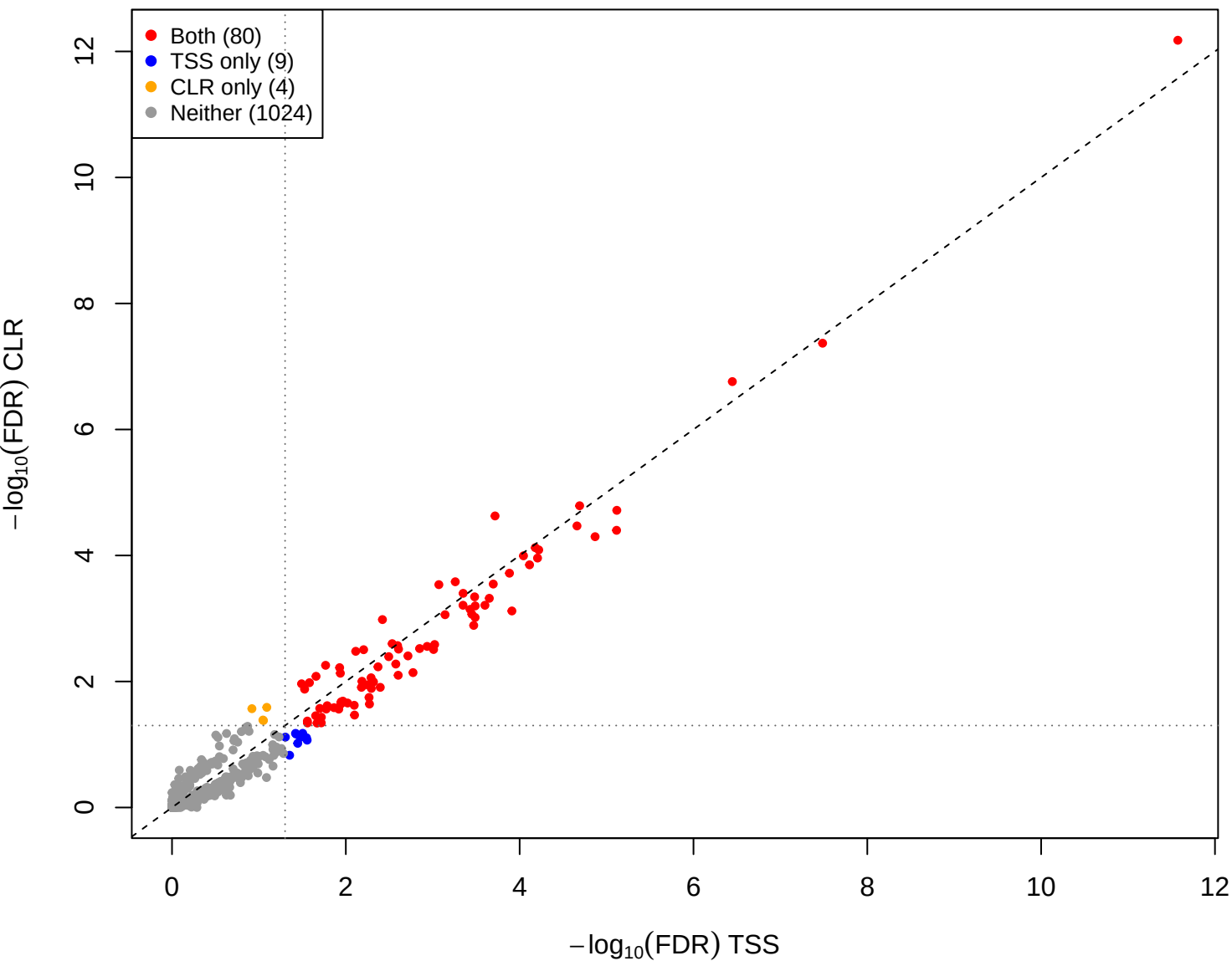
mage vs mid – CLR vs TSS (gamma = 1e-05, const = 0)
