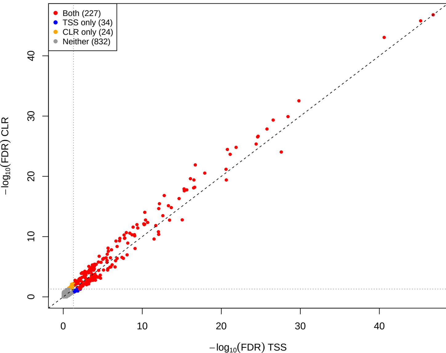
cent vs mid – CLR vs TSS (gamma = 1e-05, const = 0)
