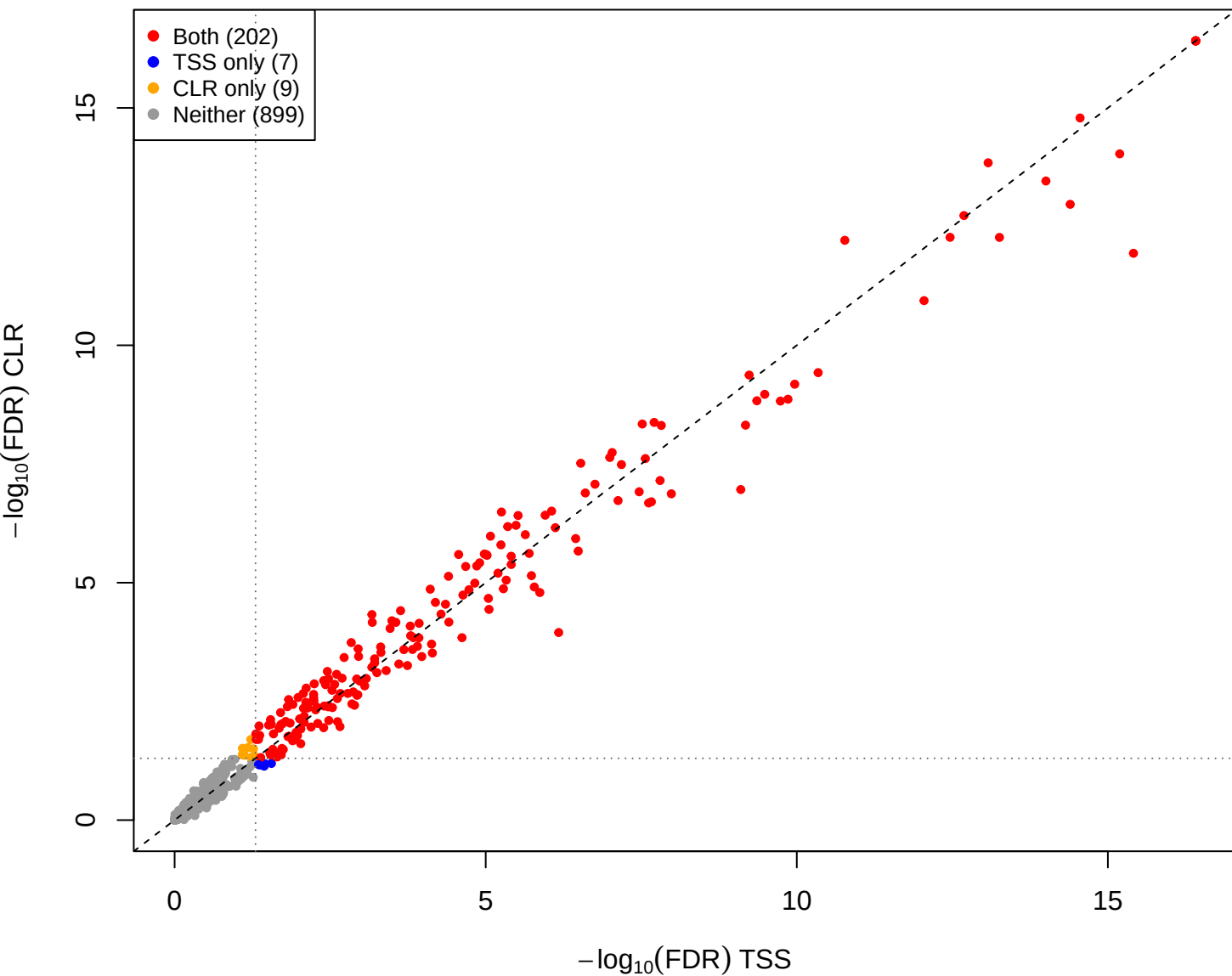
mage vs you – CLR vs TSS (gamma = 1e-05, const = 0)
