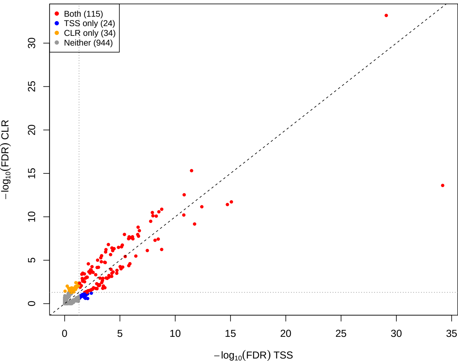
mage vs pup – CLR vs TSS (gamma = 1e-05, const = 0)
