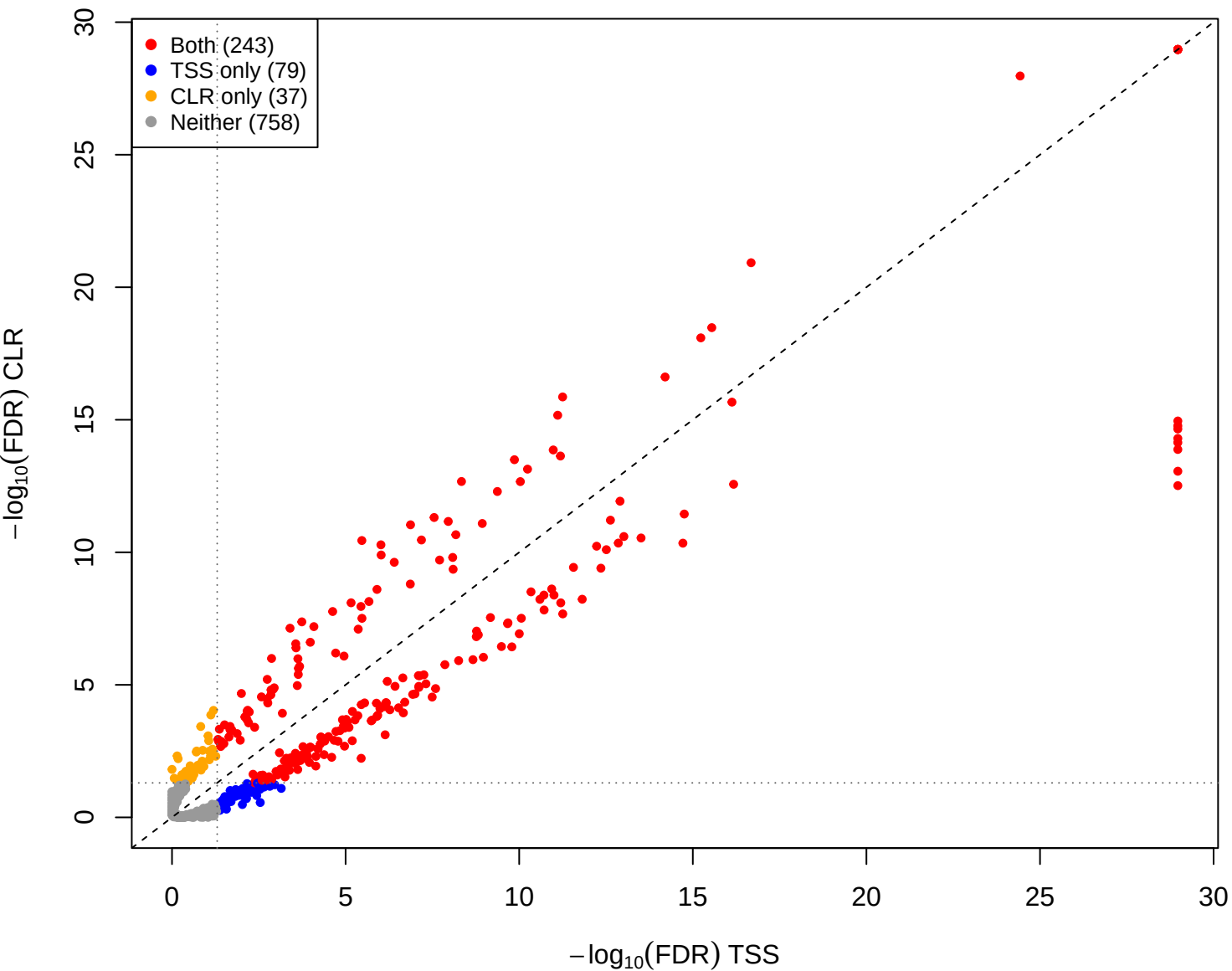
cent vs you - CLR vs TSS (gamma = 1e-05, const = 0)
