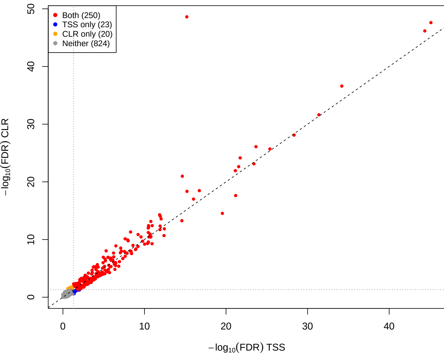
cent vs kin – CLR vs TSS (gamma = 1e-05, const = 0)
