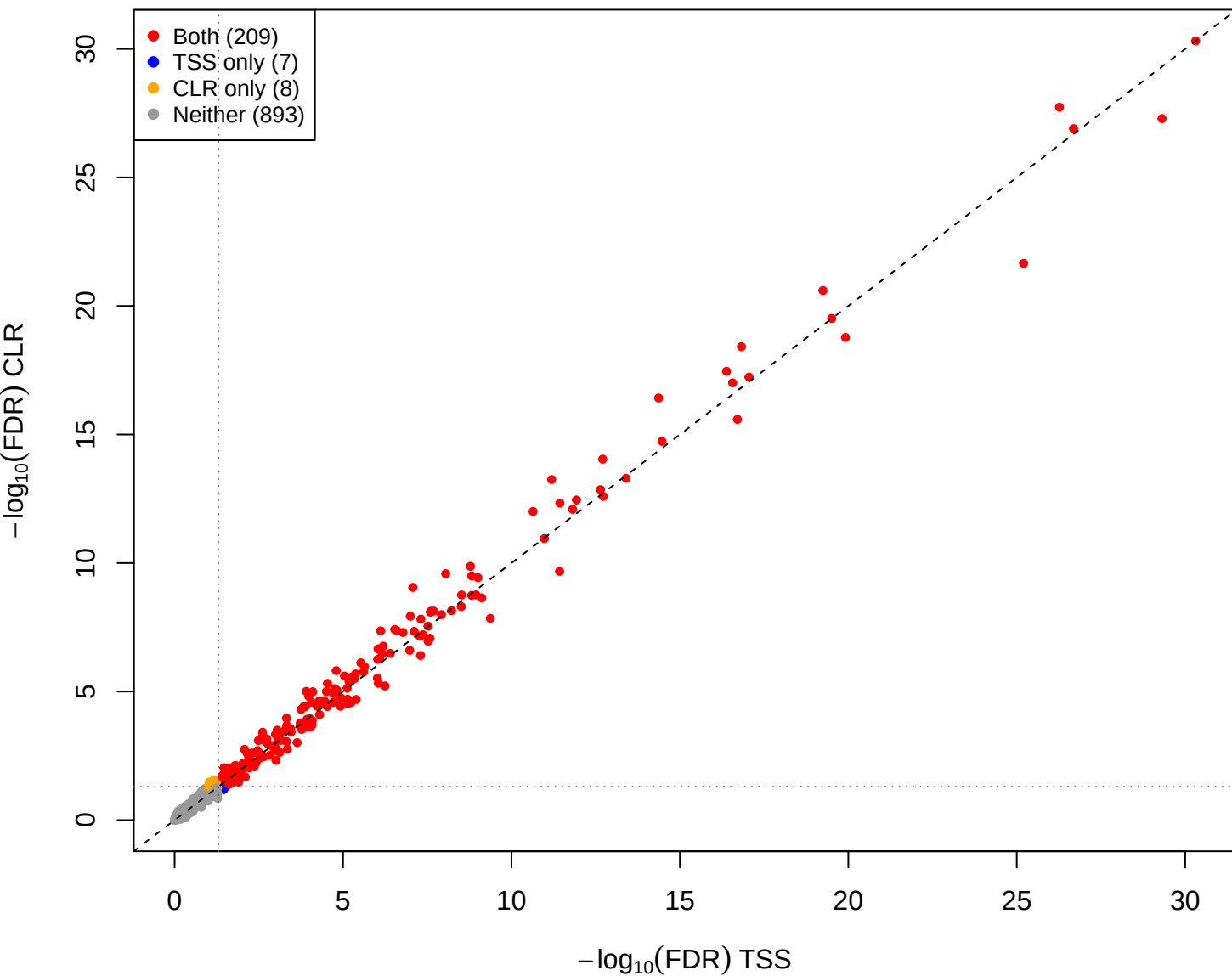
eld vs kin - CLR vs TSS (gamma = 1e-05, const = 0)
