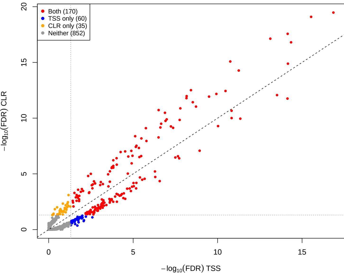
cent vs mage – CLR vs TSS (gamma = 1e-05, const = 0)
