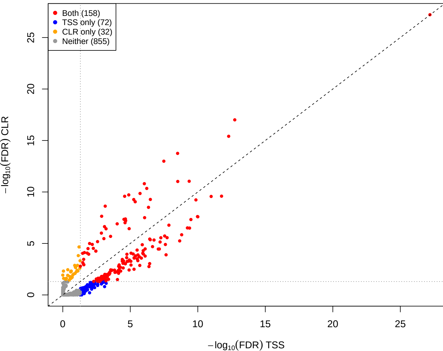
mid vs pup – CLR vs TSS (gamma = 1e-05, const = 0)
