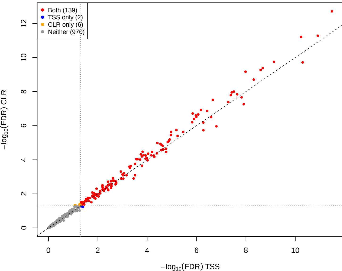
kin vs mid – CLR vs TSS (gamma = 1e-05, const = 0)
