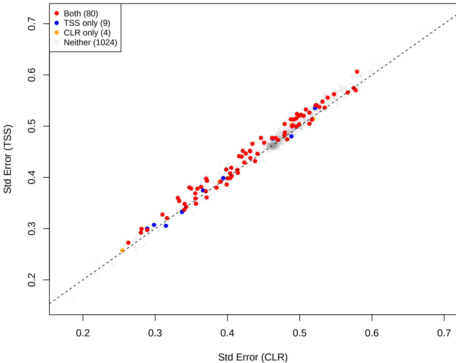
mage vs mid [gamma = 0.05]
