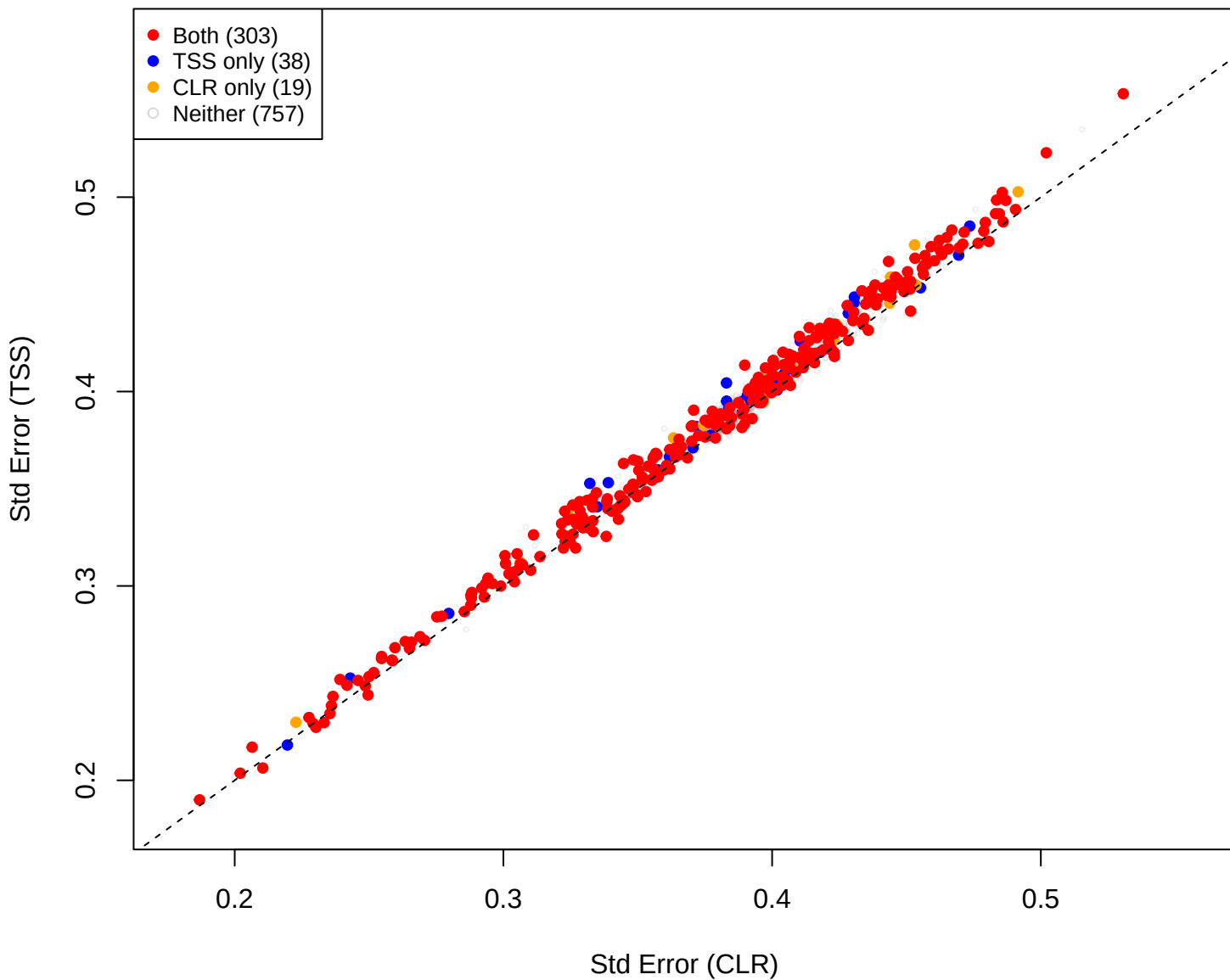
pup vs you [gamma = 0.05]
