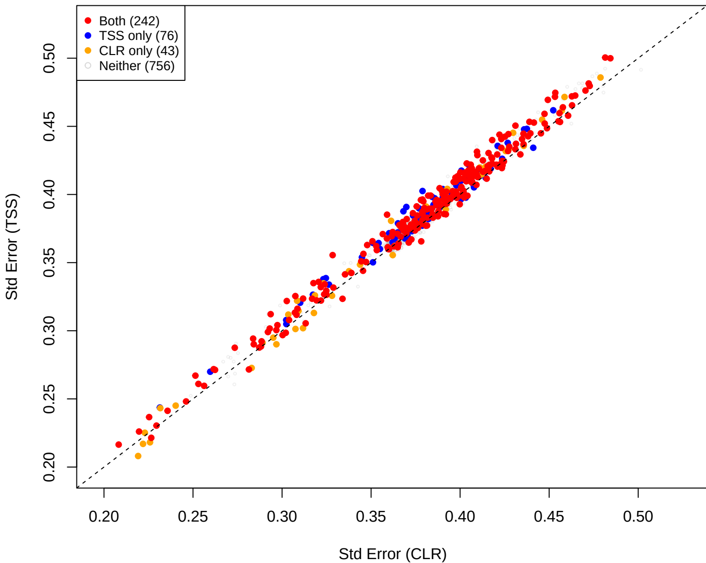
cent vs you [gamma = 0.05]
