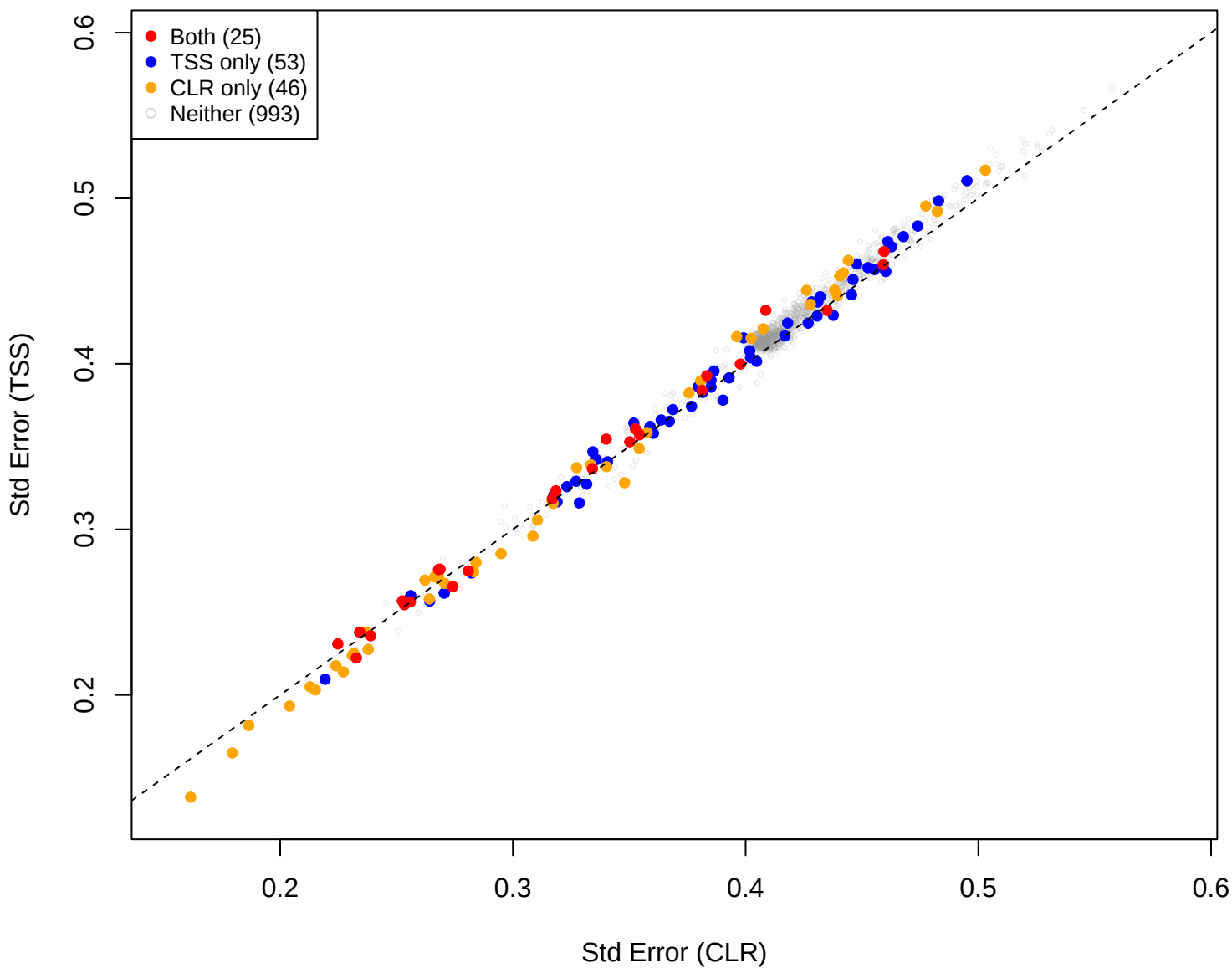
kin vs pup [gamma = 0.05]
