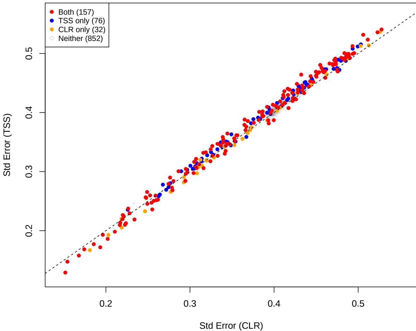
mid vs pup [gamma = 0.05]
