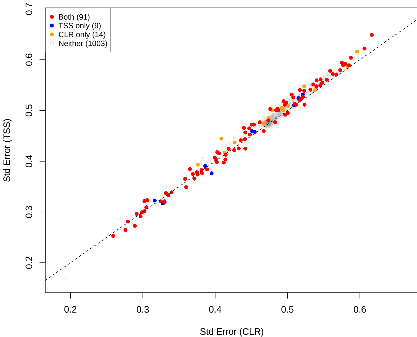
kin vs mage [gamma = 0.05]
