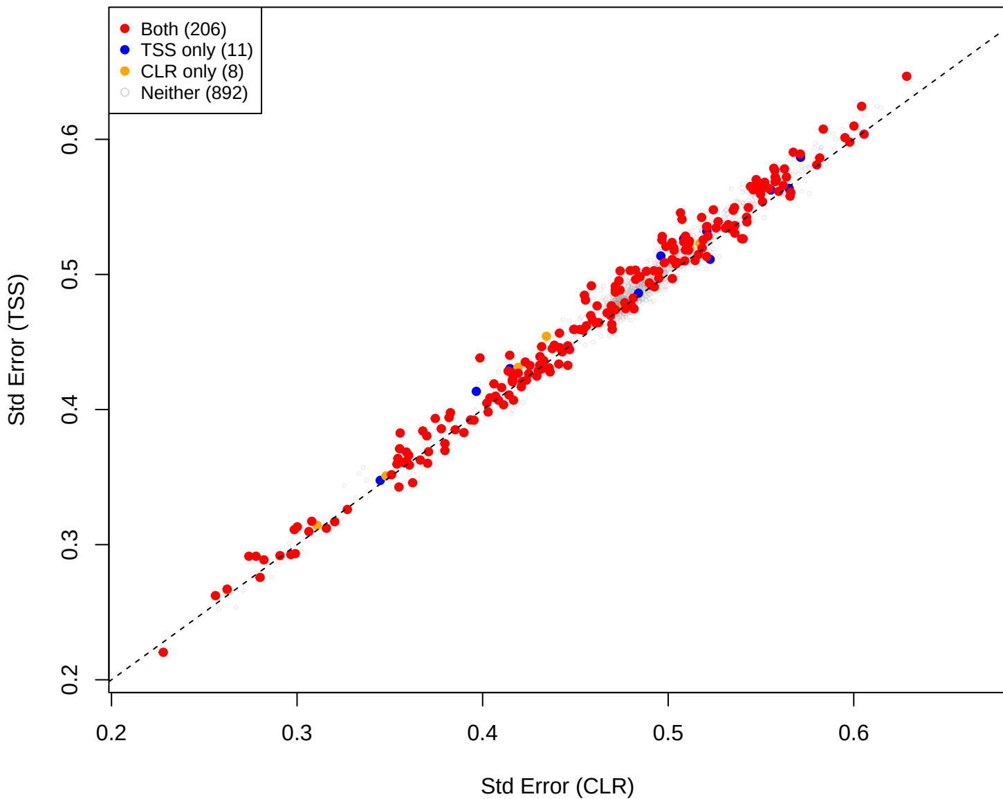
eld vs kin [gamma = 0.05]
