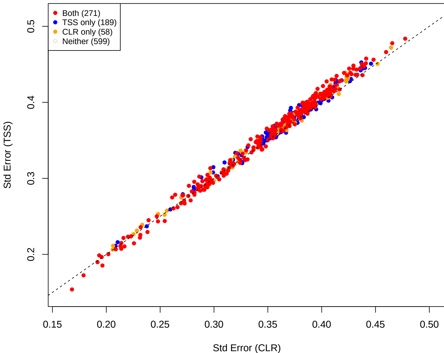
cent vs pup [gamma = 0.05]
