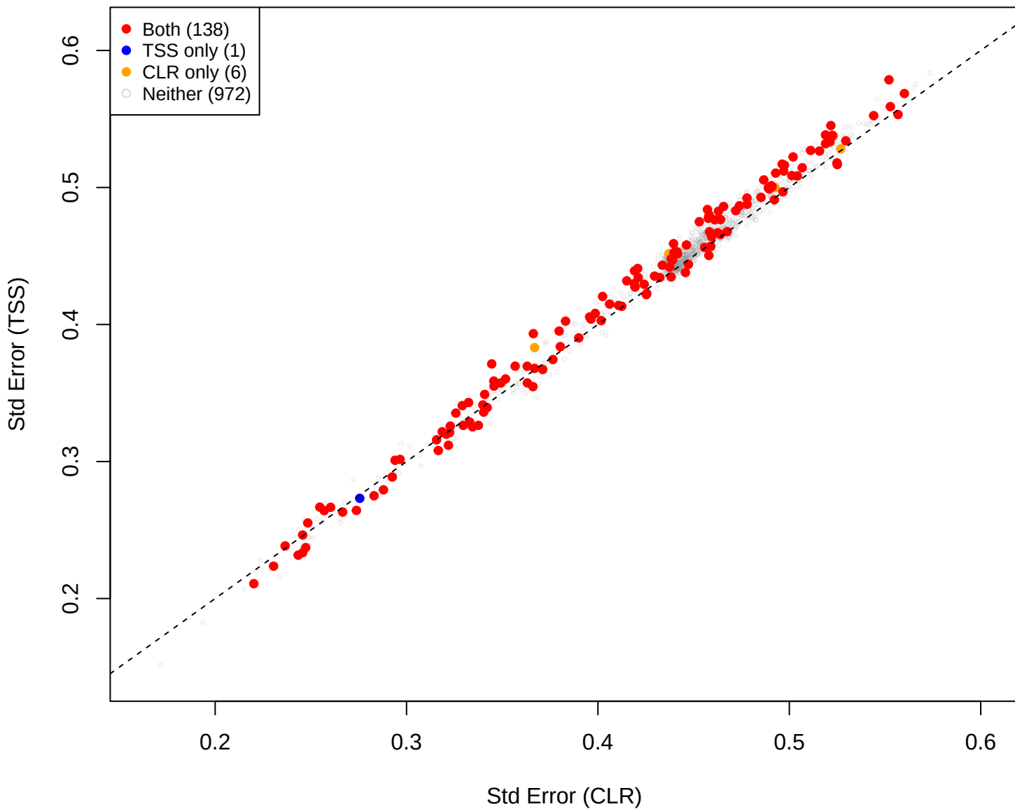
kin vs mid [gamma = 0.05]
