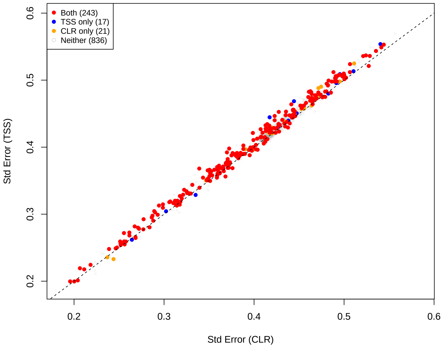
mid vs you [gamma = 0.05]
