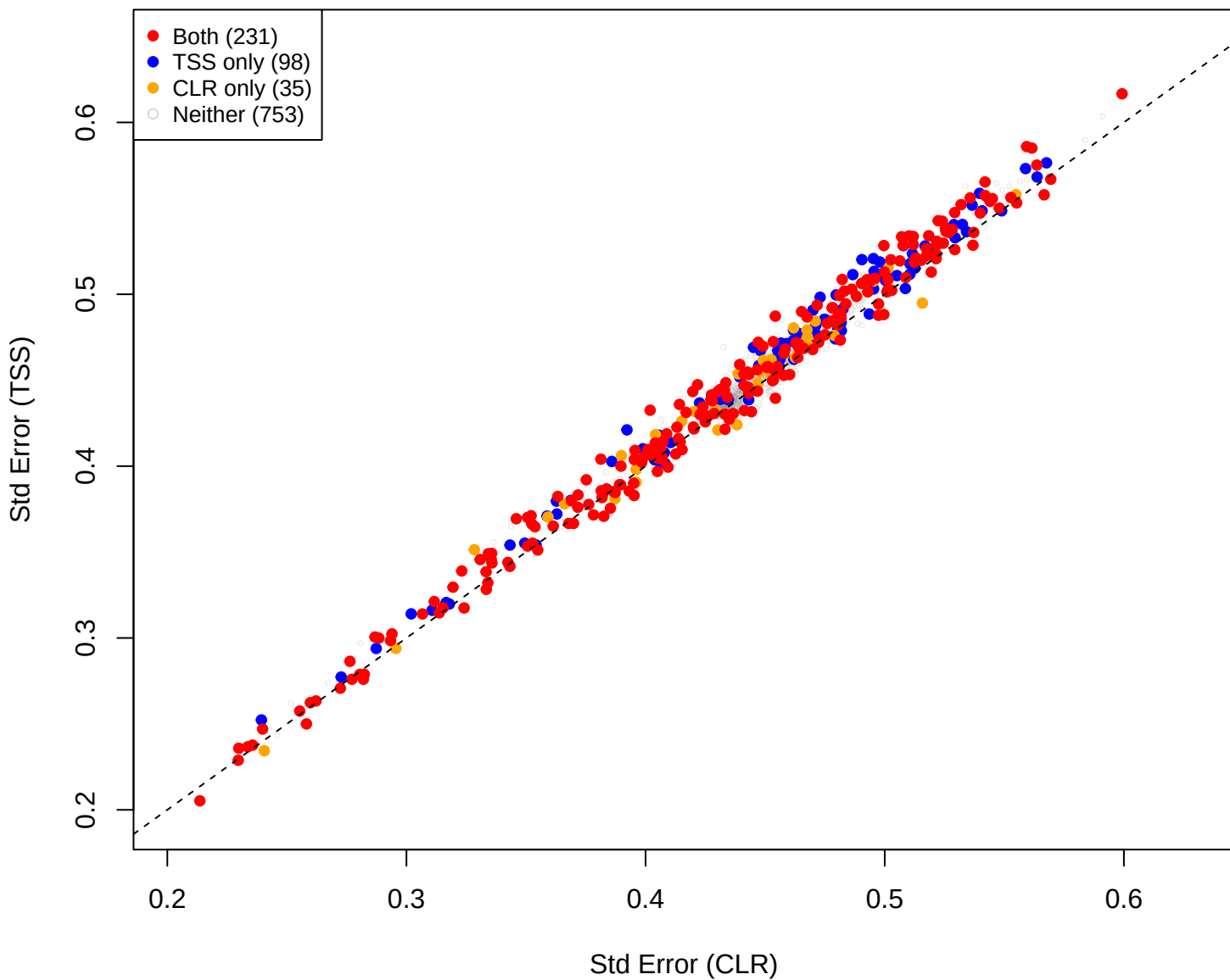
eld vs pup [gamma = 0.05]
