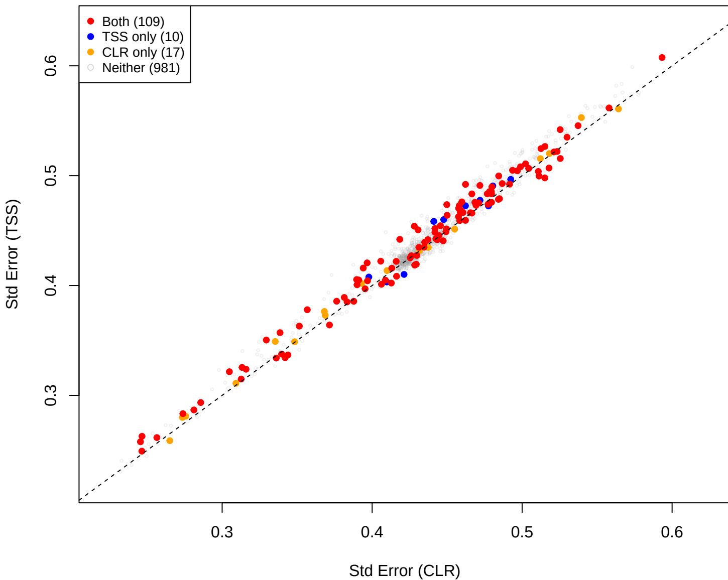
cent vs eld [gamma = 0.05]
