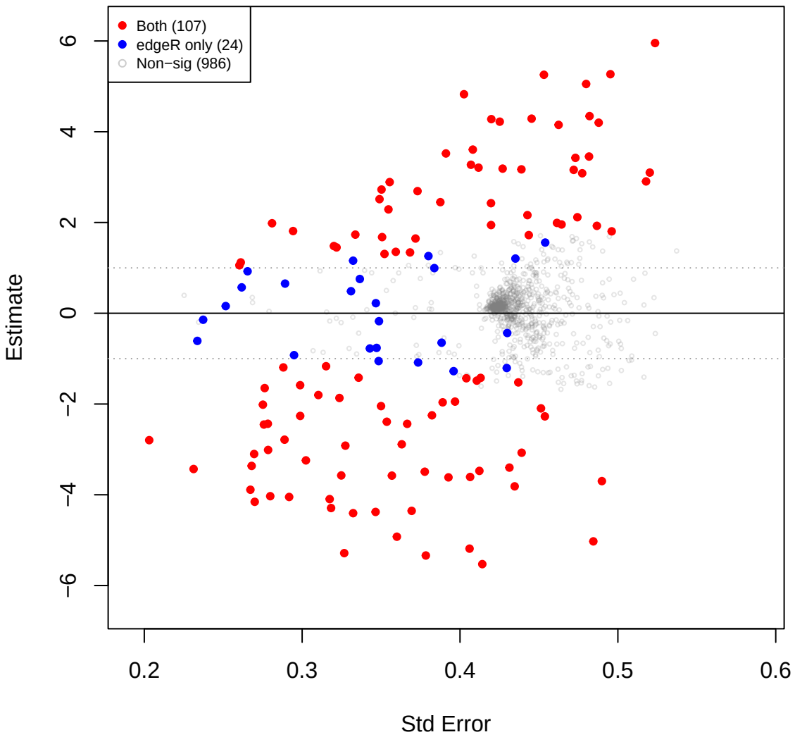
kin vs you – CLR (edgeR RLE sig overlay)
