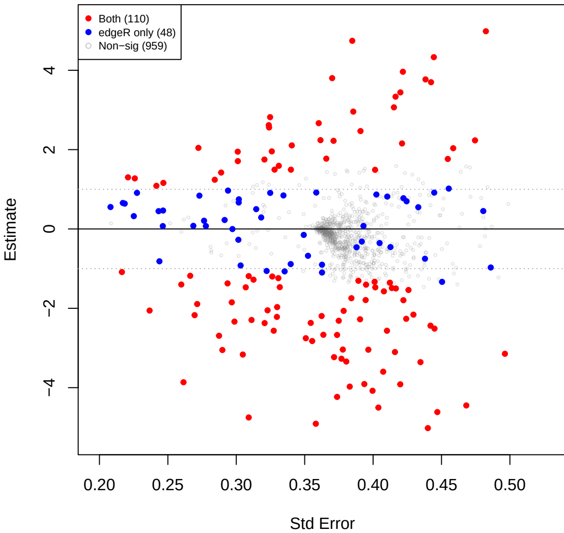
you vs cent – TSS (edgeR TMM sig overlay)
