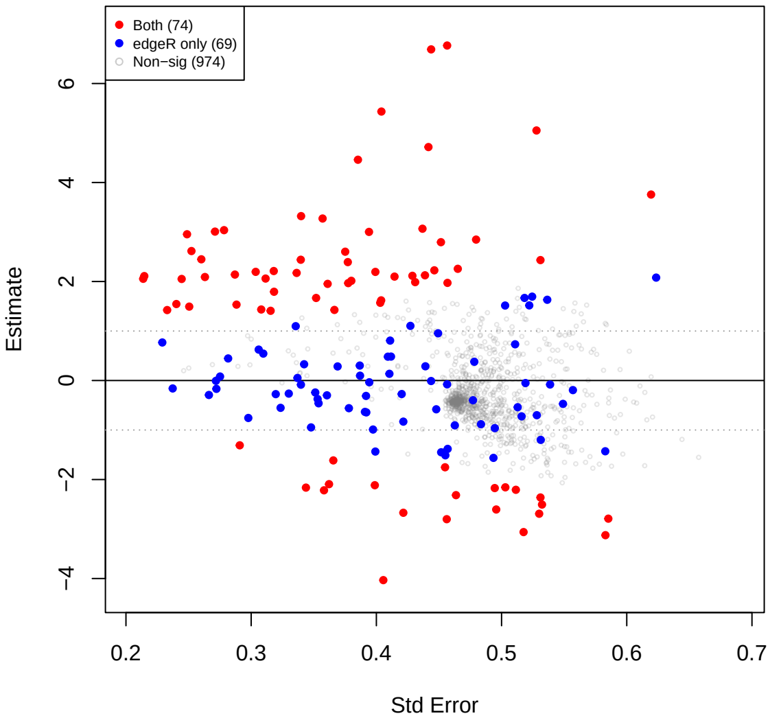
mid vs eld – TSS (edgeR TMM sig overlay)
