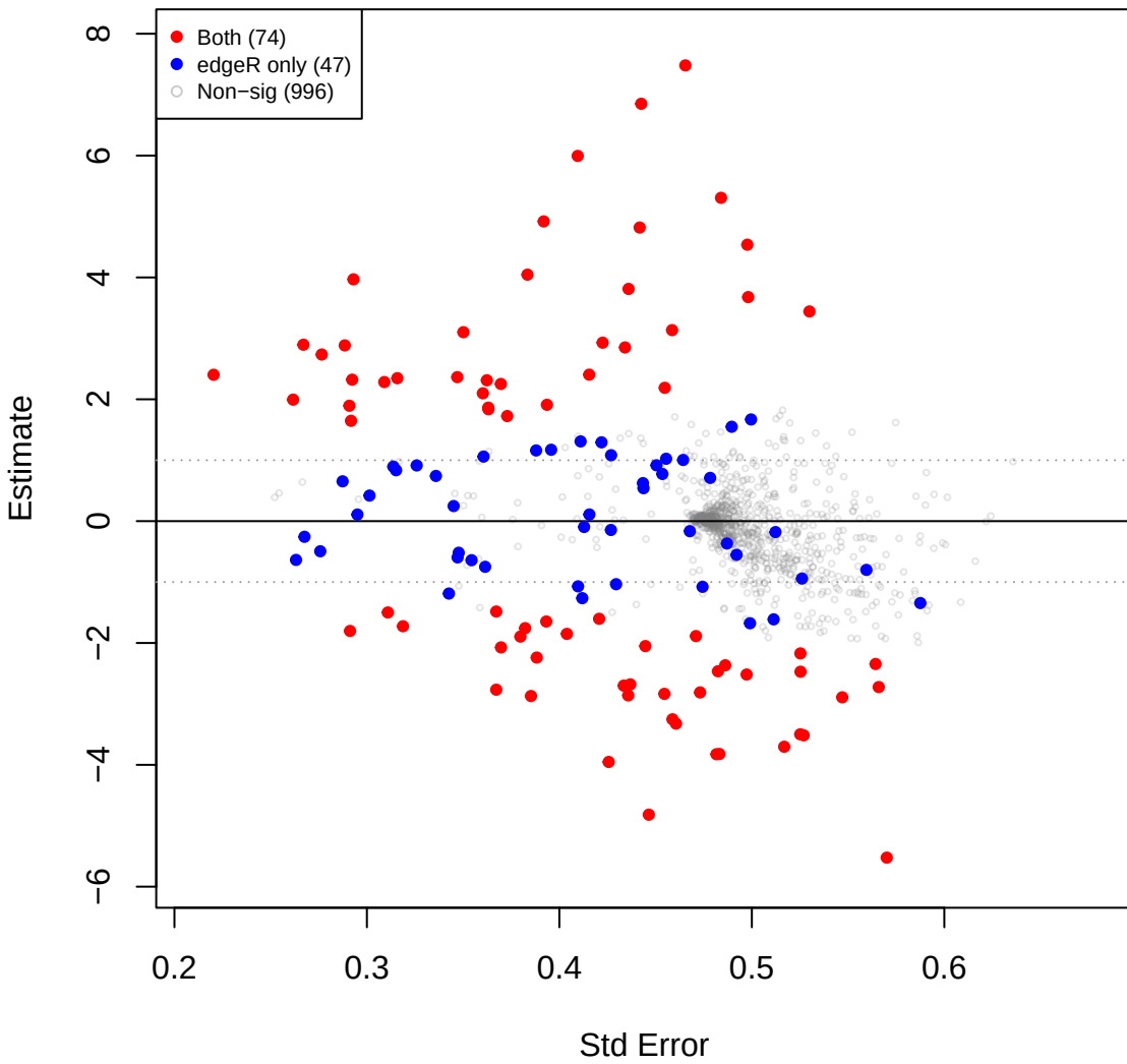
kin vs eld – TSS (edgeR TMM sig overlay)
