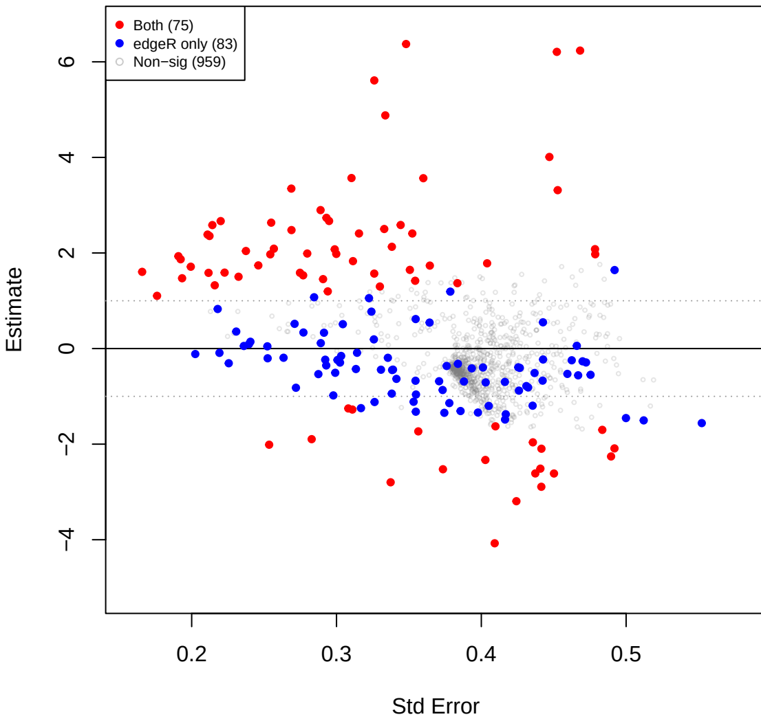
mid vs cent – TSS (edgeR TMM sig overlay)
