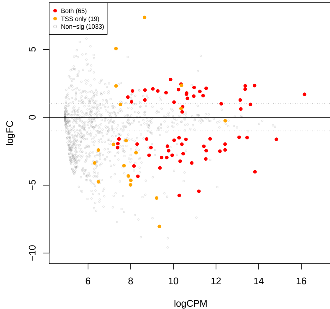
eld vs cent – edgeR TMM (TSS sig overlay)
