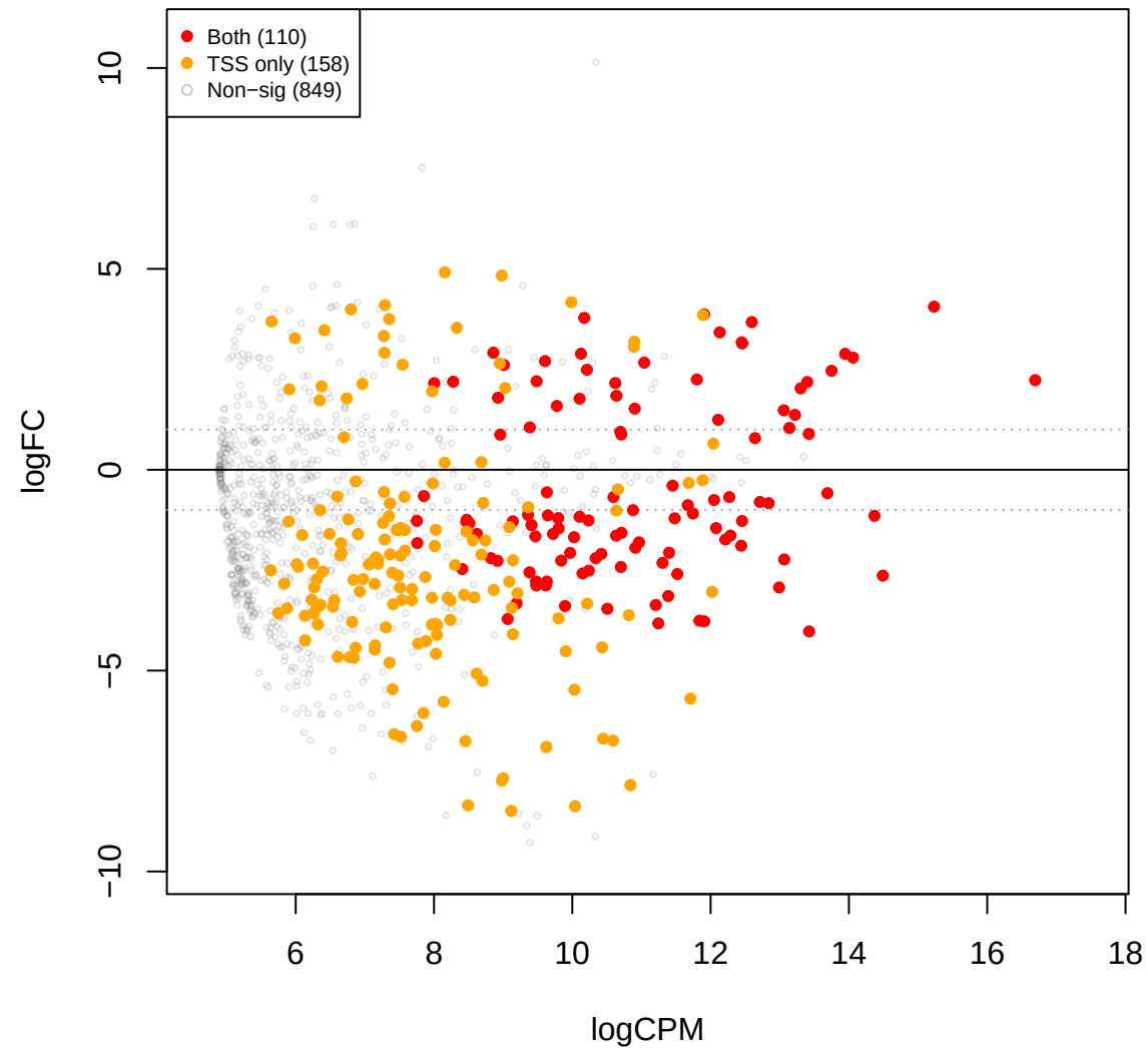
you vs cent – edgeR TMM (TSS sig overlay)
