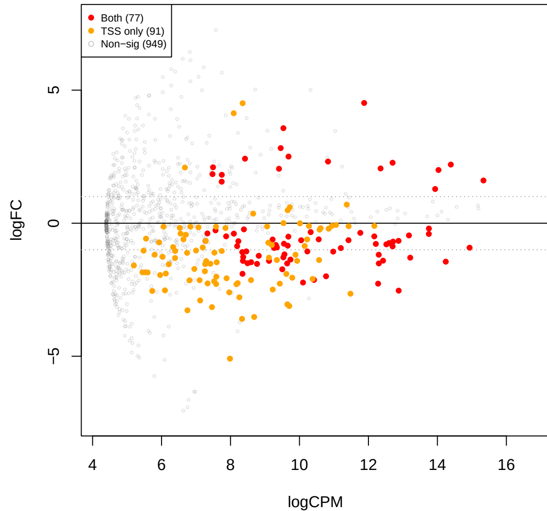
pup vs mid – edgeR TMM (TSS sig overlay)
