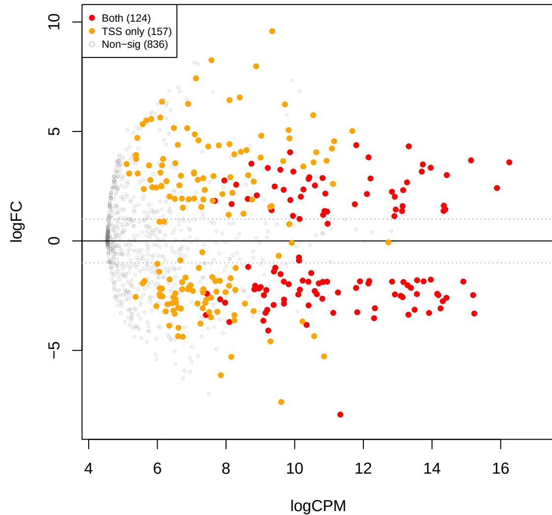
pup vs you – edgeR TMM (TSS sig overlay)
