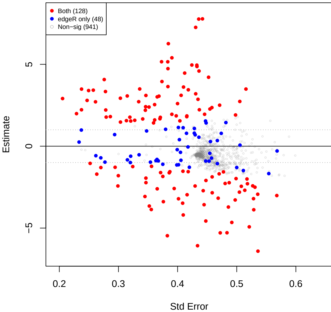
pup vs eld – TSS (edgeR TMM sig overlay)
