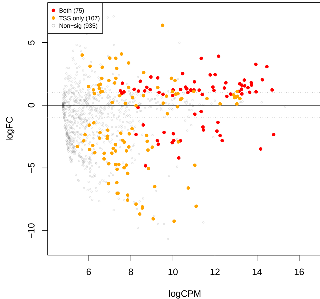
mid vs cent – edgeR TMM (TSS sig overlay)
