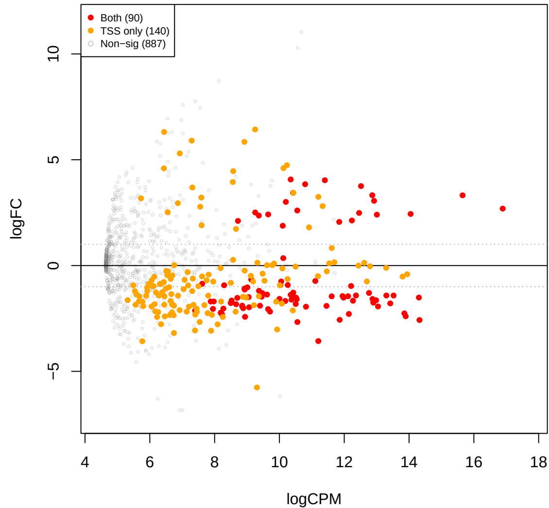
mid vs you – edgeR TMM (TSS sig overlay)
