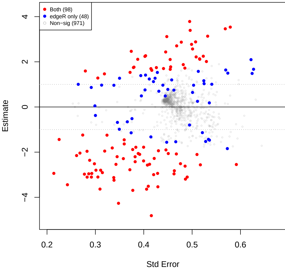
you vs mage – TSS (edgeR TMM sig overlay)
