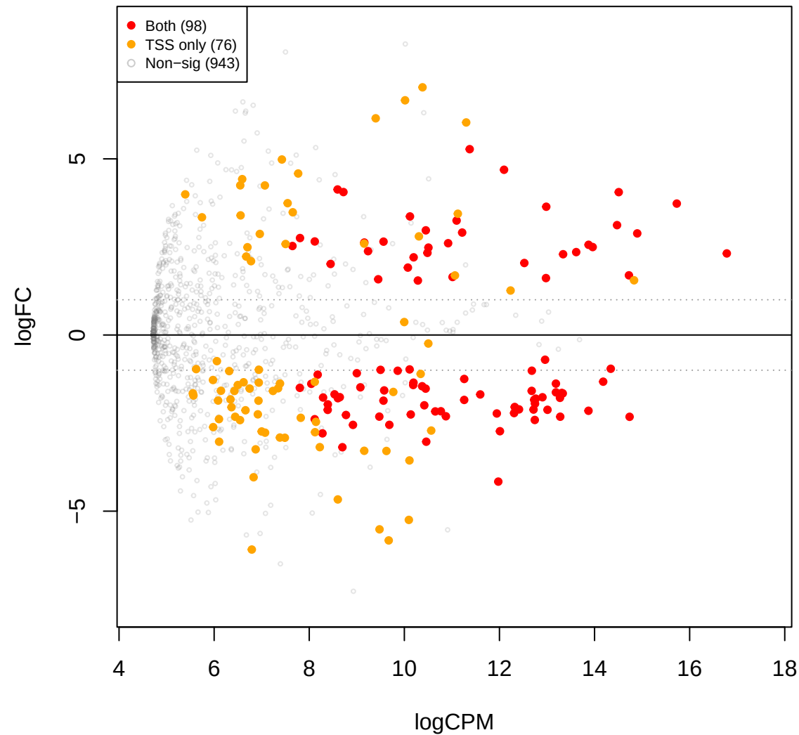
you vs mage – edgeR TMM (TSS sig overlay)
