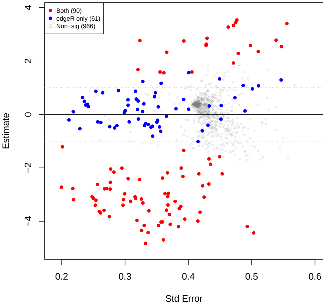
mid vs you – TSS (edgeR TMM sig overlay)
