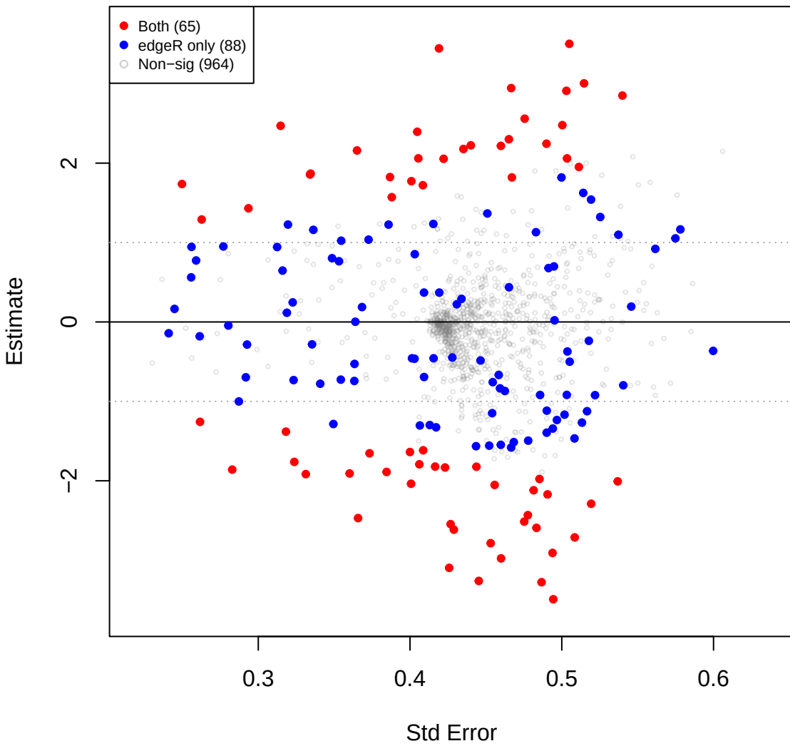
eld vs cent – TSS (edgeR TMM sig overlay)
