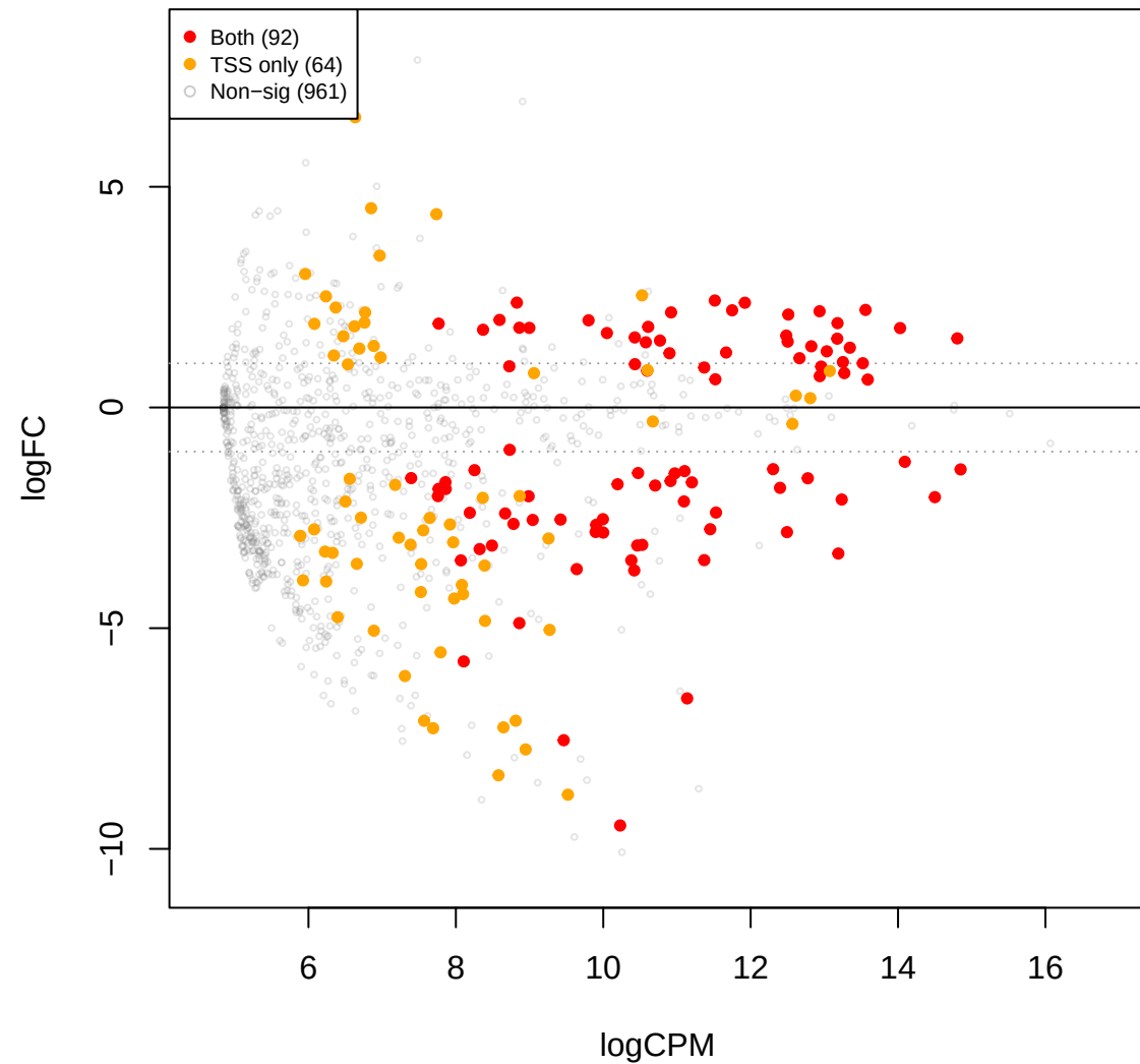
mage vs cent – edgeR TMM (TSS sig overlay)
