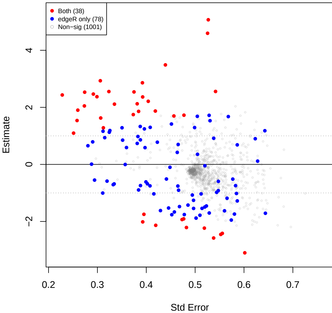
mage vs eld – TSS (edgeR TMM sig overlay)
