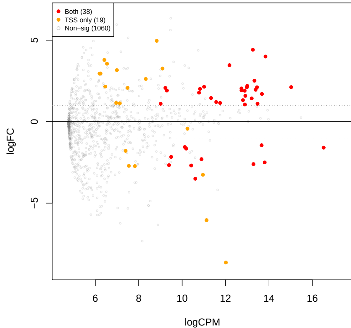
mage vs eld – edgeR TMM (TSS sig overlay)
