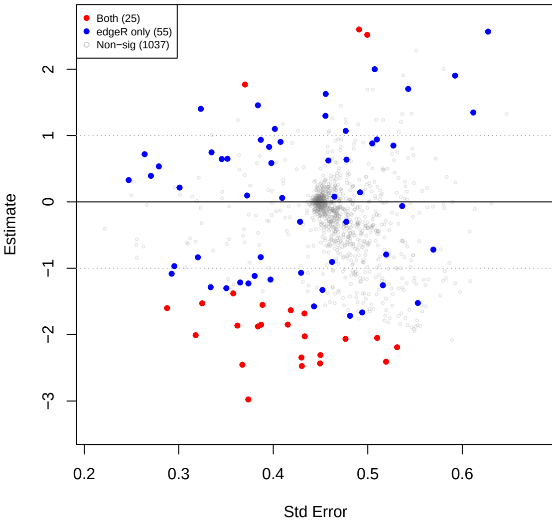
you vs eld – TSS (edgeR TMM sig overlay)
