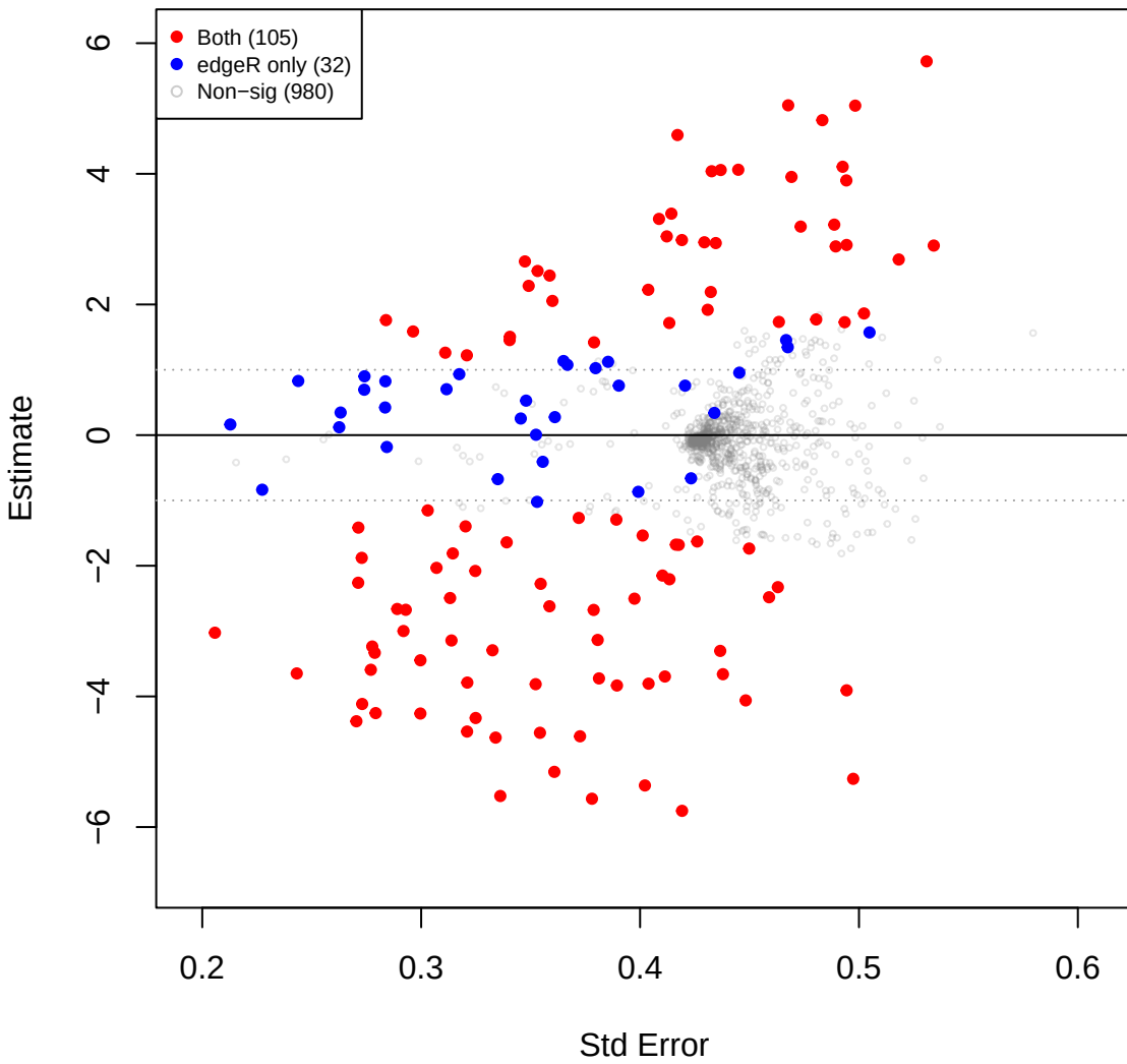
kin vs you – TSS (edgeR TMM sig overlay)
