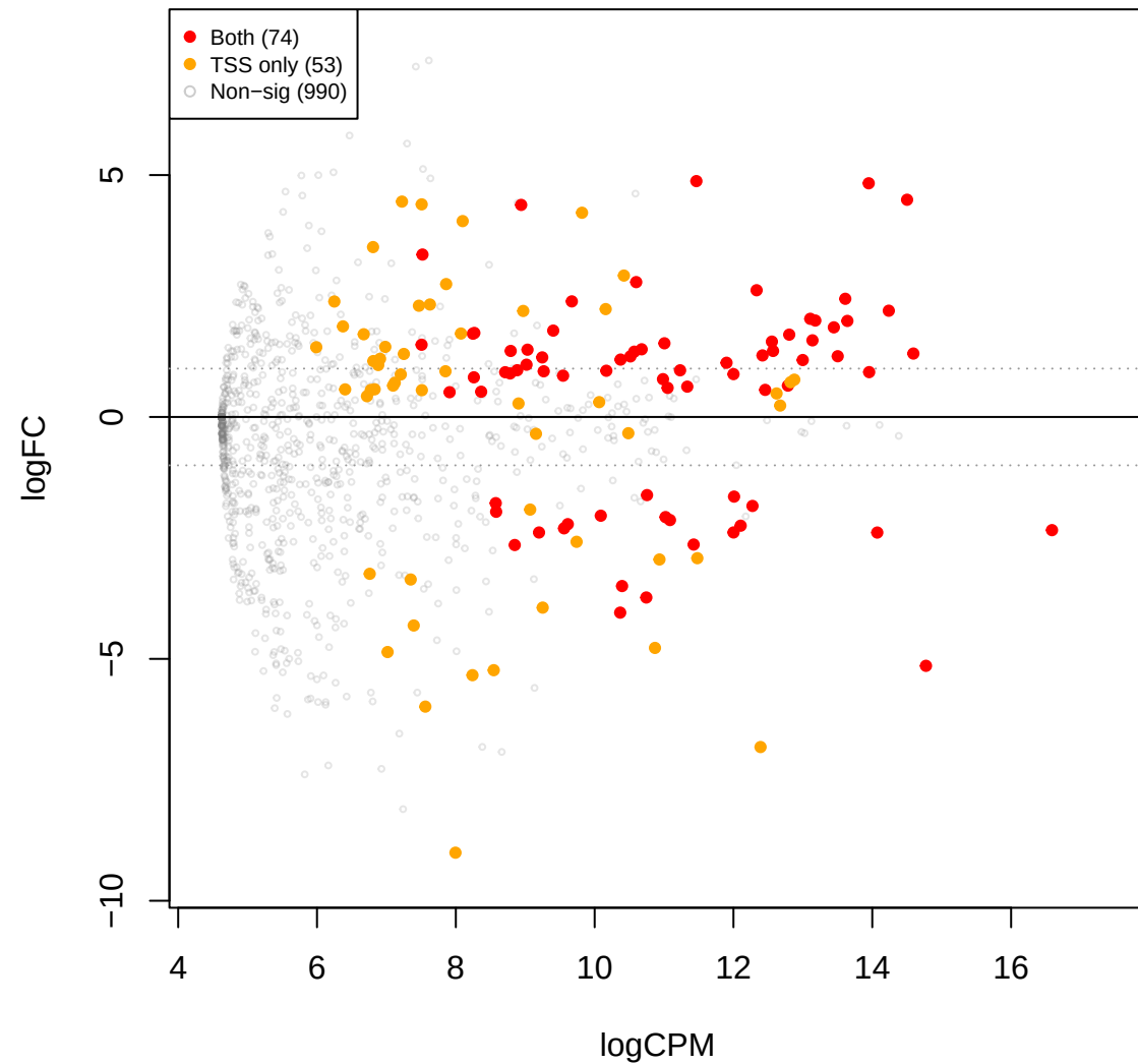
mid vs eld – edgeR TMM (TSS sig overlay)
