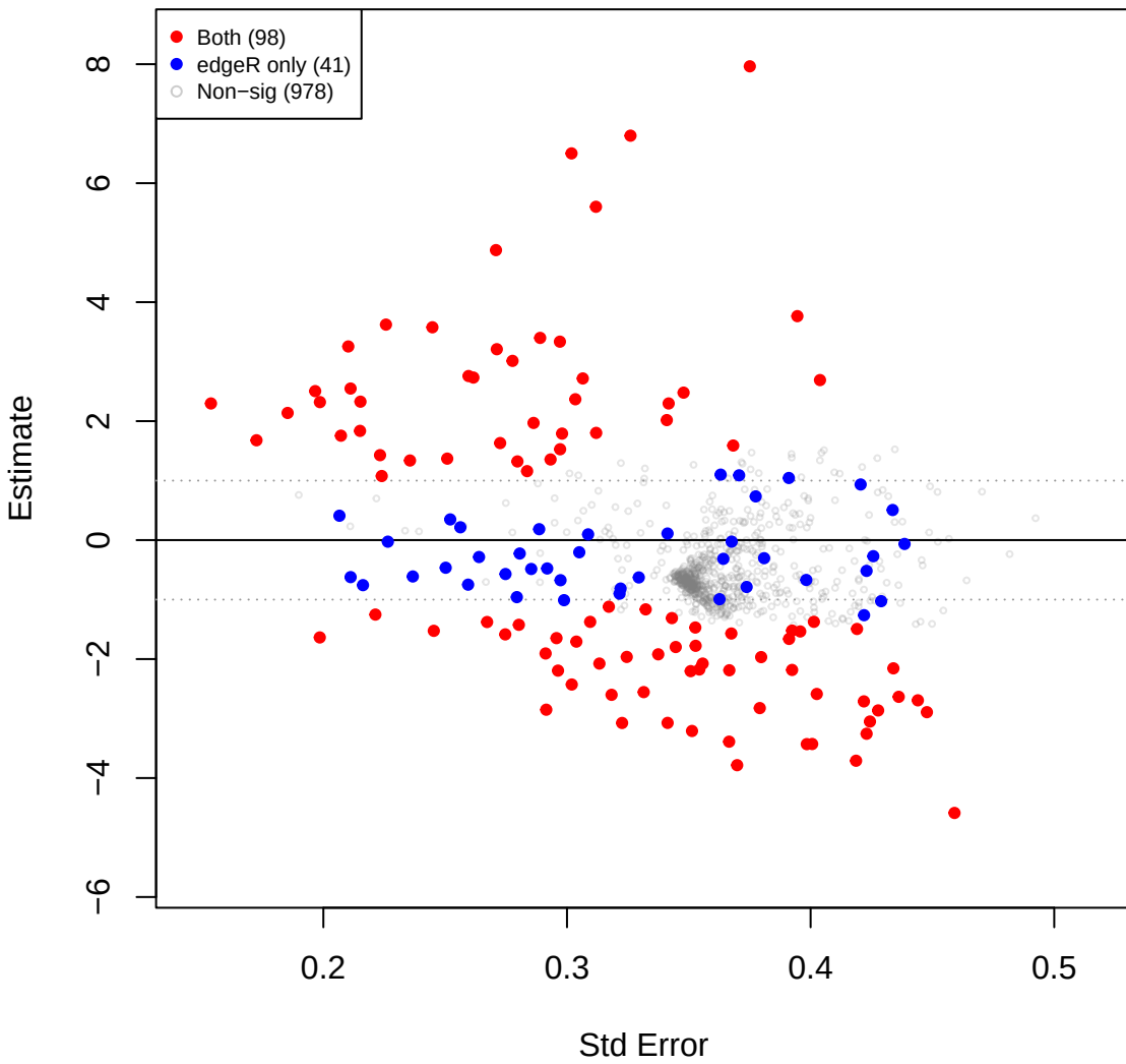
pup vs cent – TSS (edgeR TMM sig overlay)
