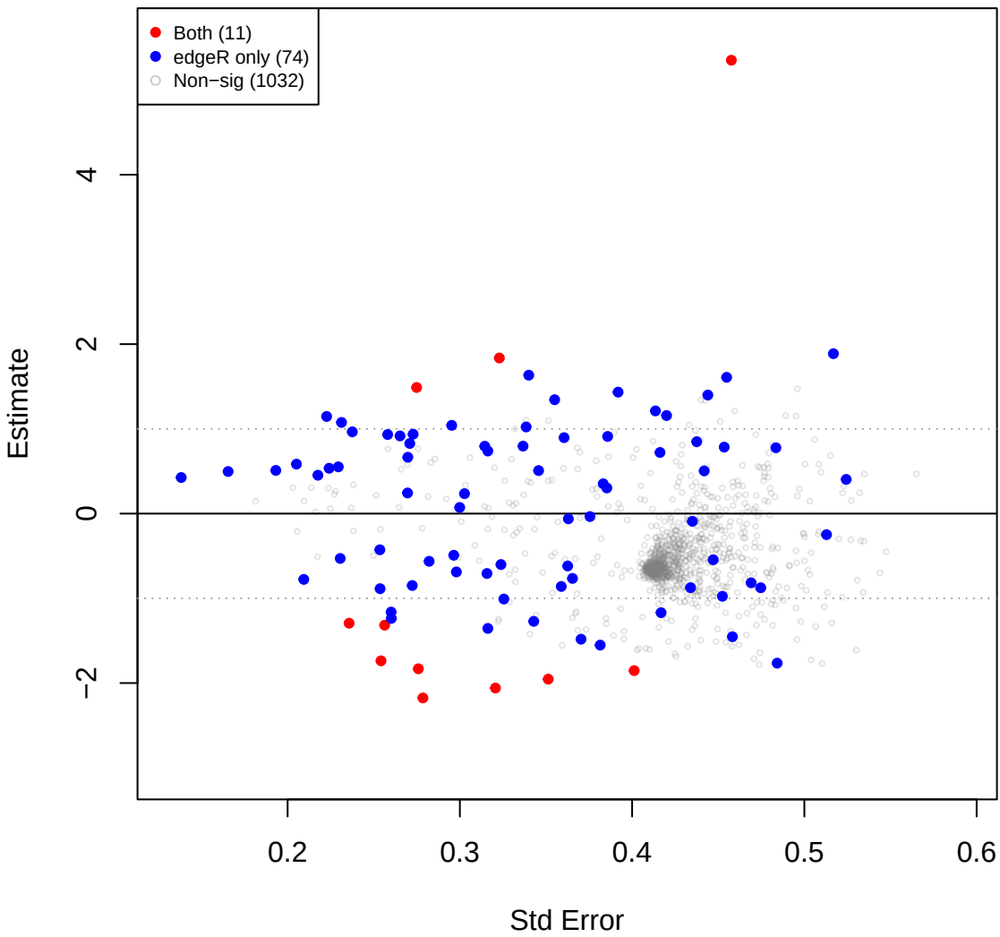
kin vs pup – TSS (edgeR TMM sig overlay)
