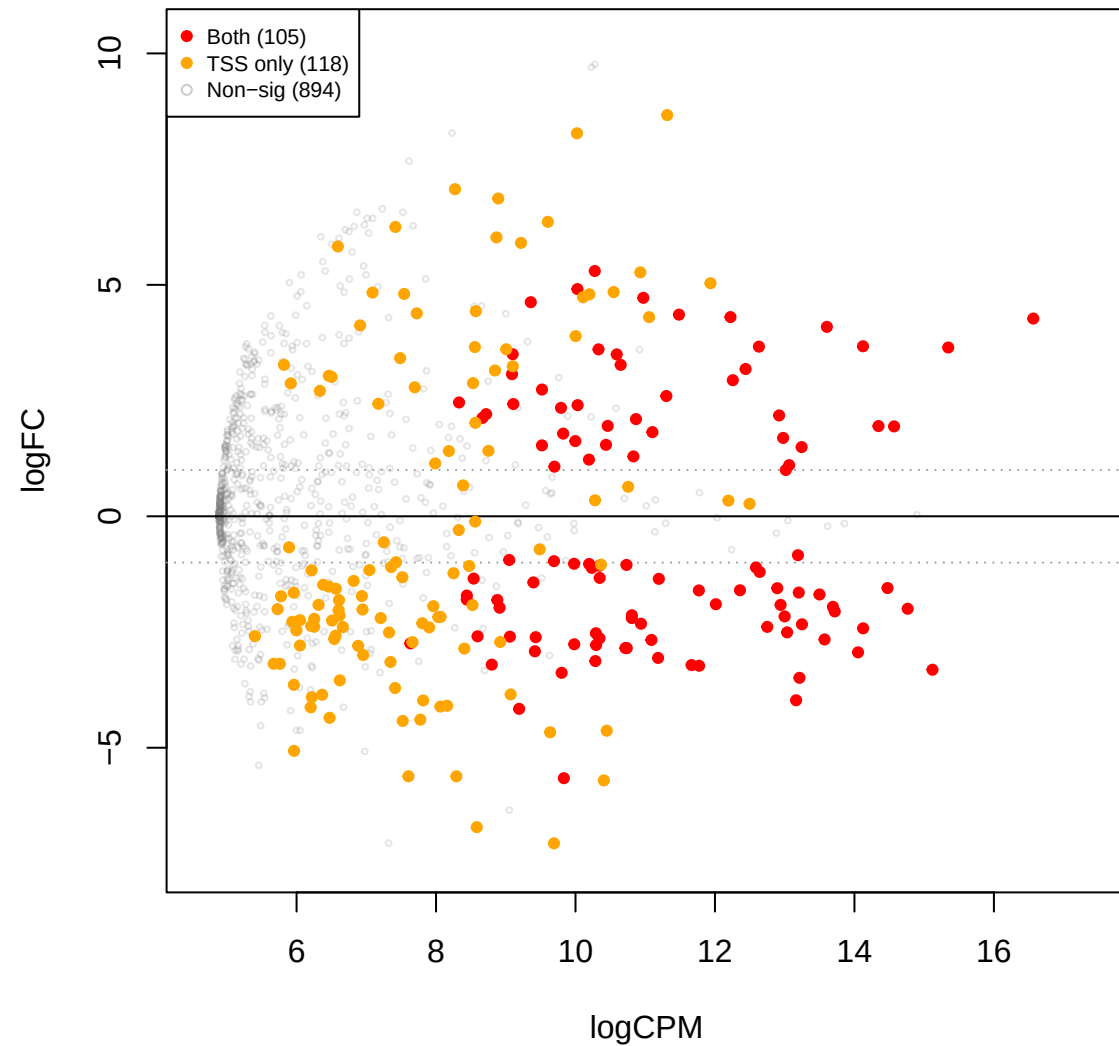
kin vs you – edgeR TMM (TSS sig overlay)
