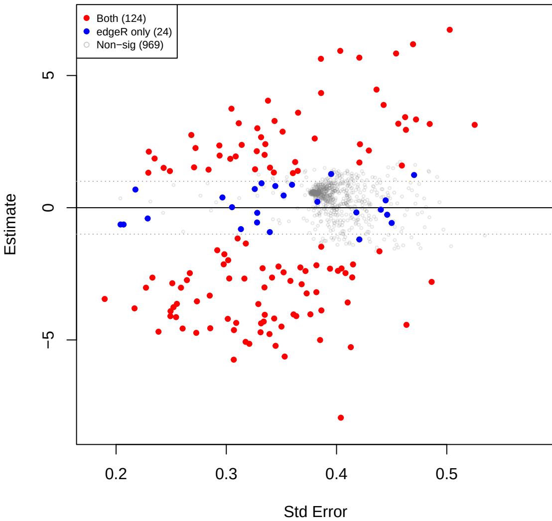
pup vs you – TSS (edgeR TMM sig overlay)
