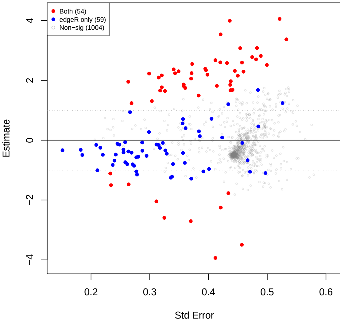
kin vs mid – TSS (edgeR TMM sig overlay)
