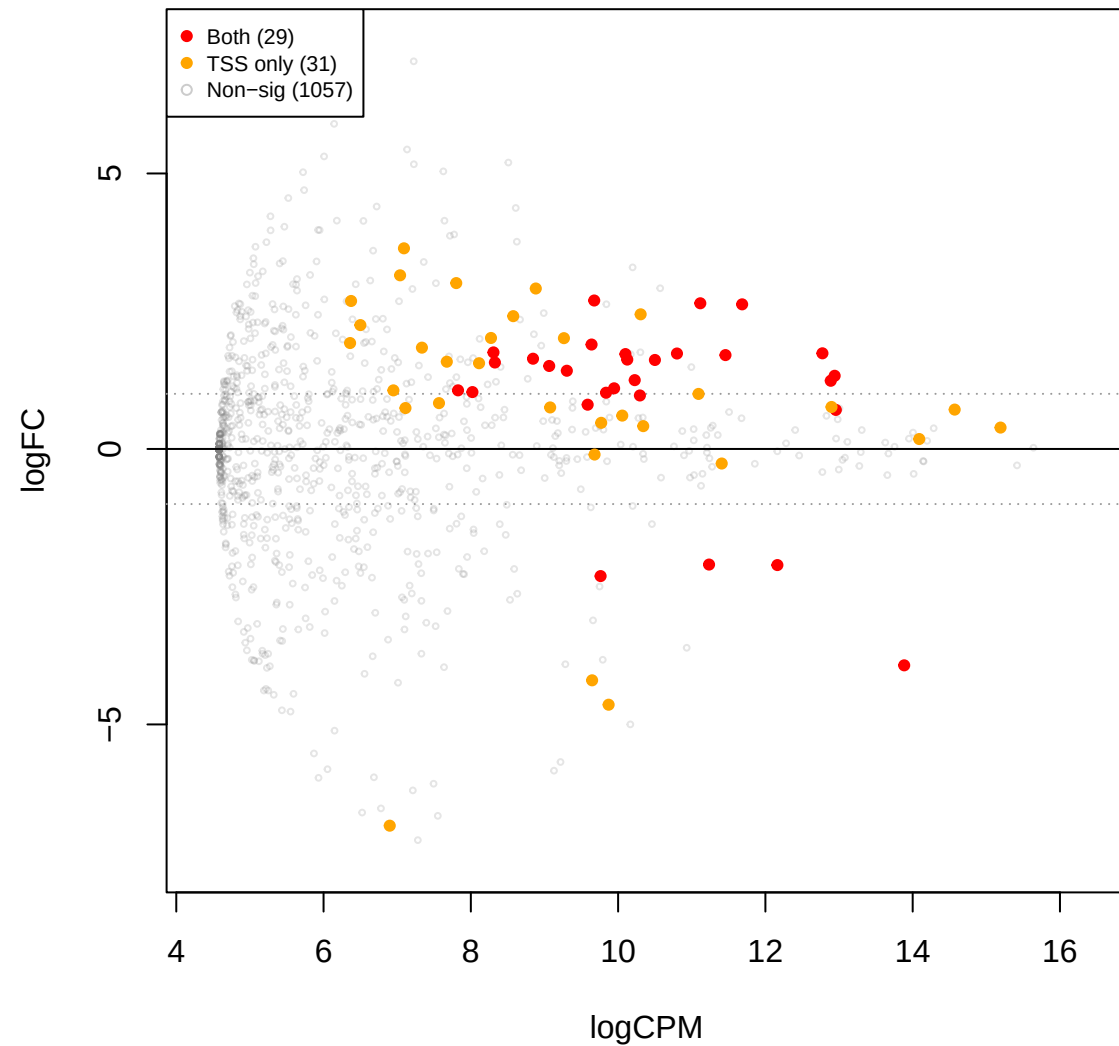
mid vs mage – edgeR TMM (TSS sig overlay)
