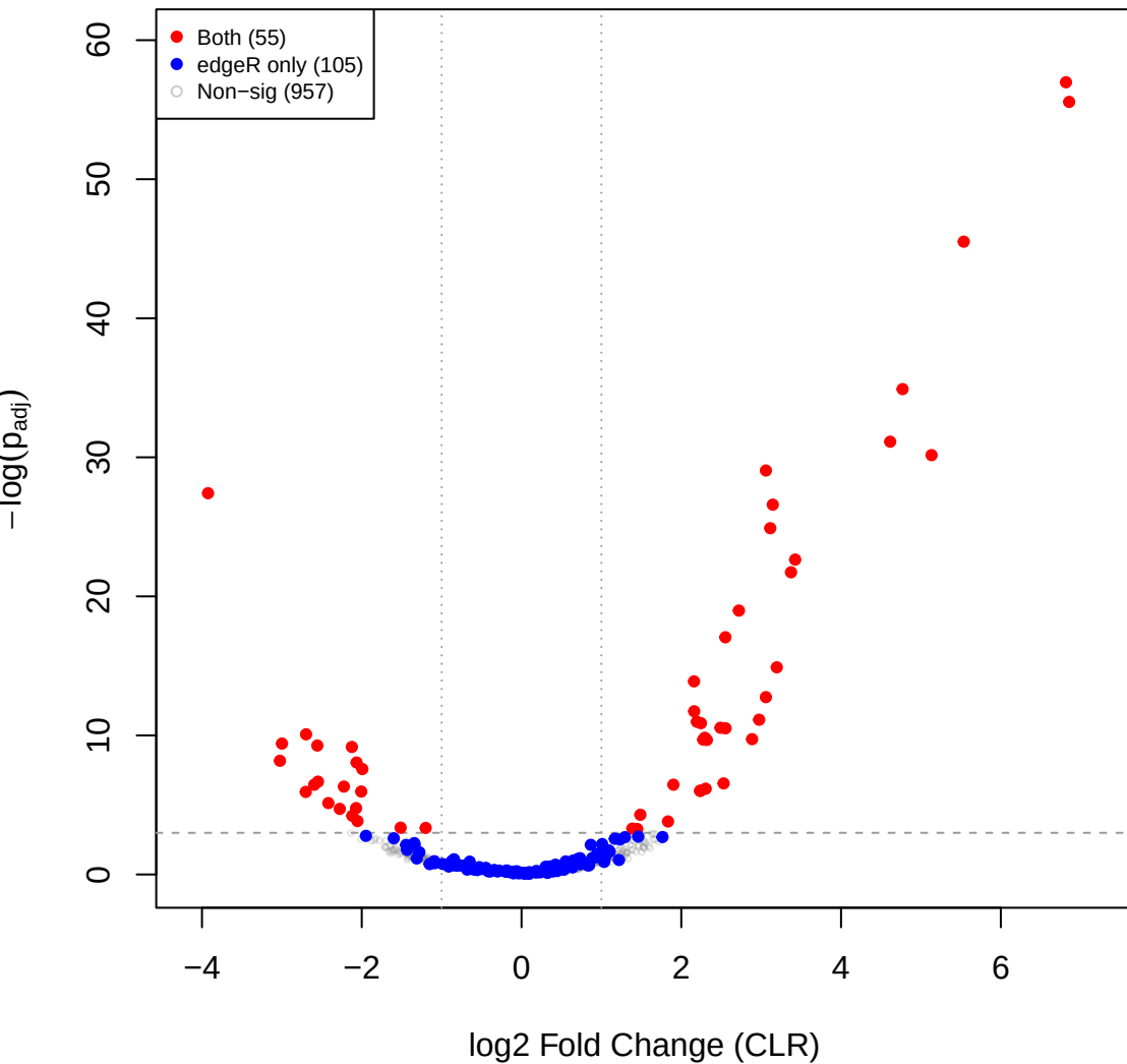
mid vs eld – CLR volcano (edgeR RLE sig overlay)
