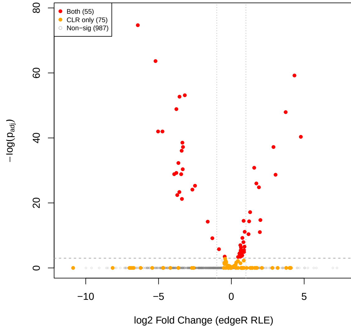
mid vs eld – edgeR RLE volcano (CLR sig overlay)
