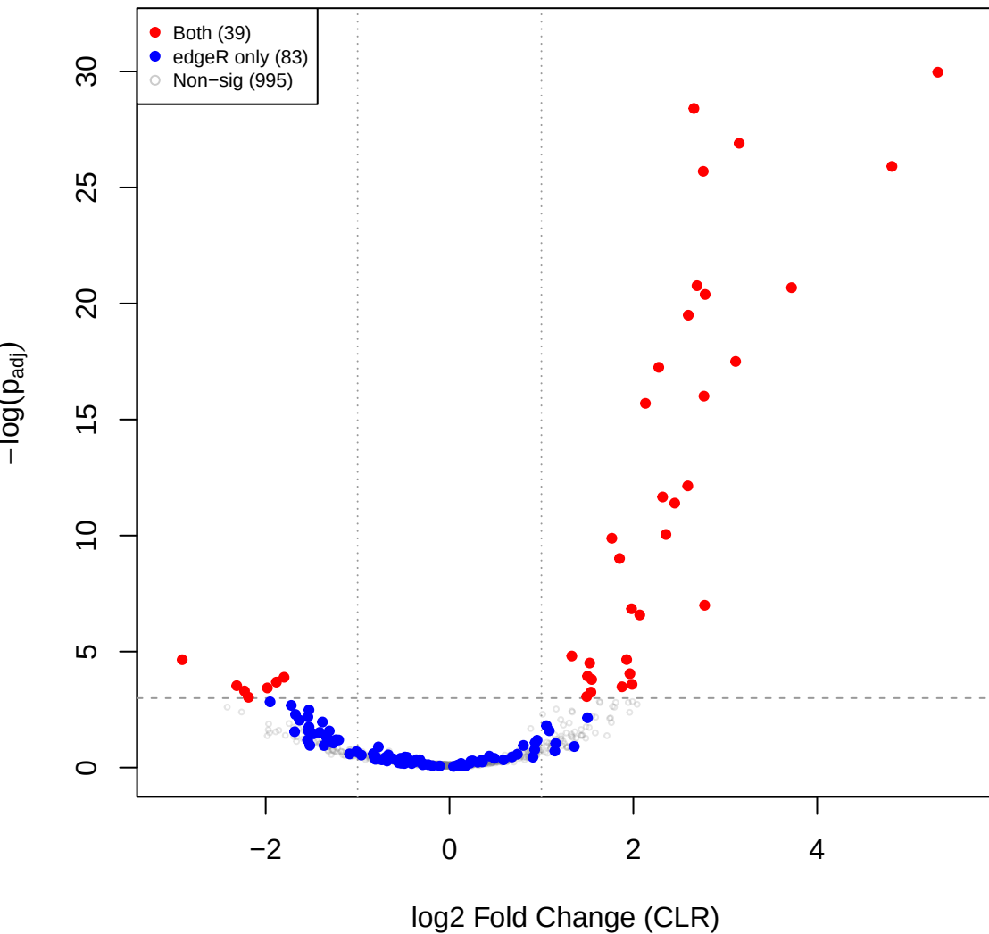
mage vs eld – CLR volcano (edgeR RLE sig overlay)
