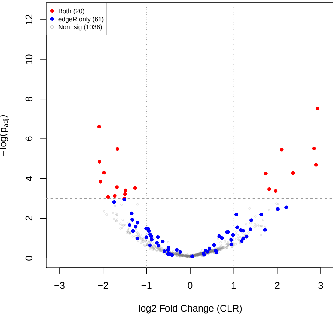
you vs eld – CLR volcano (edgeR RLE sig overlay)
