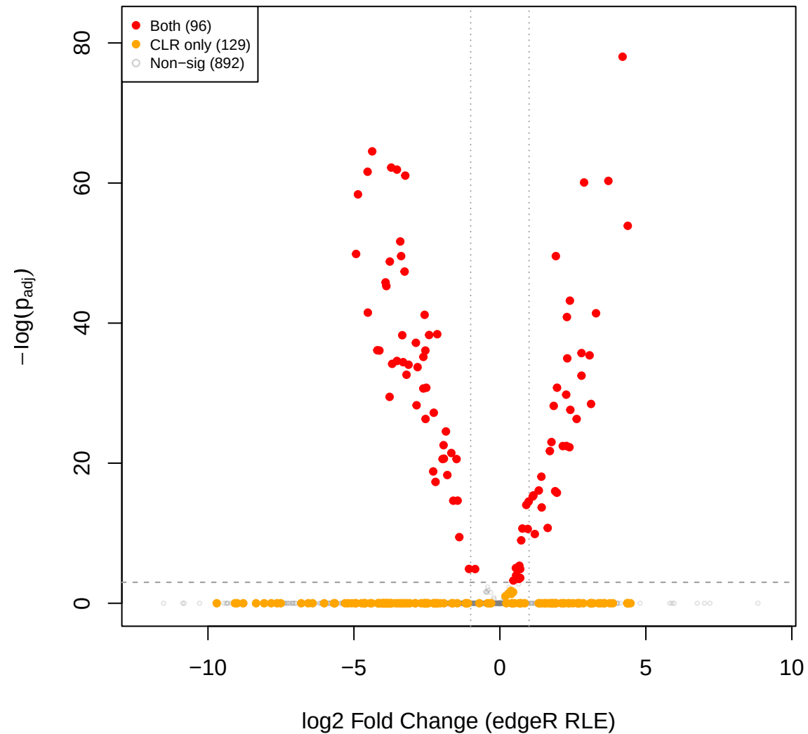
you vs cent – edgeR RLE volcano (CLR sig overlay)
