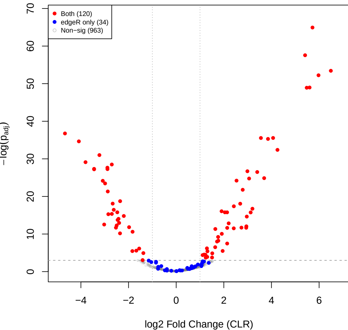
pup vs you – CLR volcano (edgeR RLE sig overlay)
