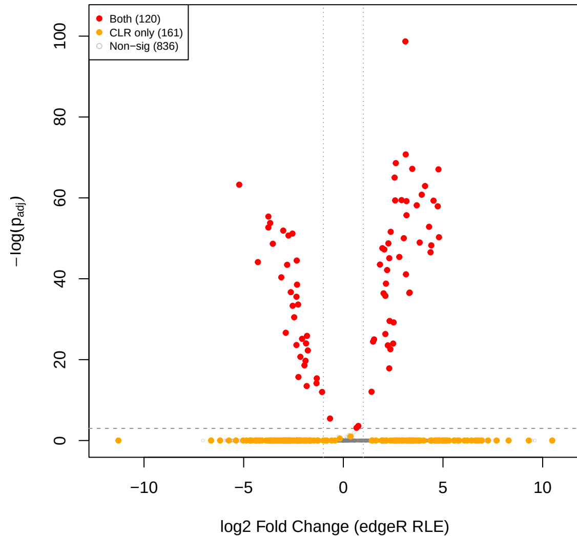
pup vs you – edgeR RLE volcano (CLR sig overlay)
