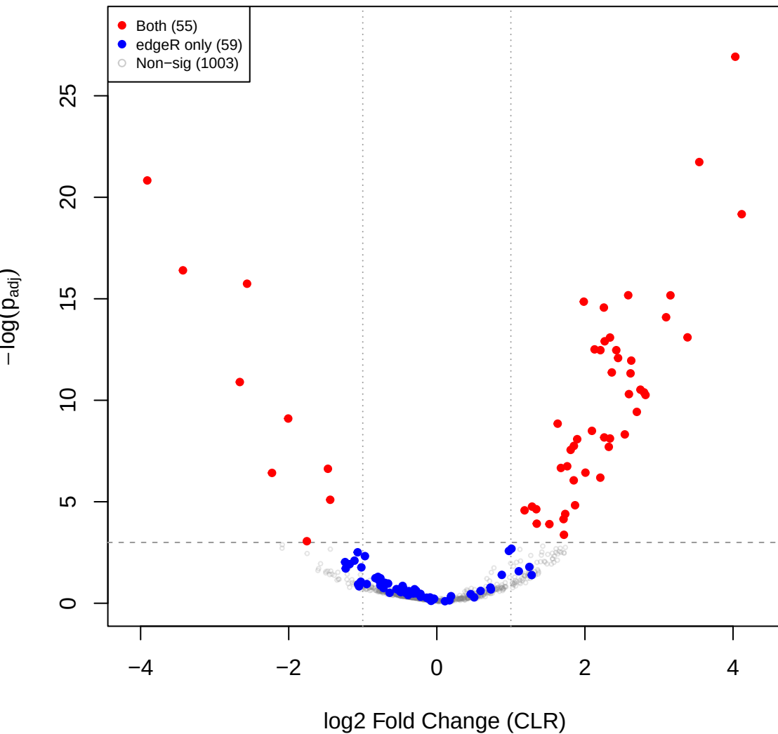
kin vs mid – CLR volcano (edgeR RLE sig overlay)
