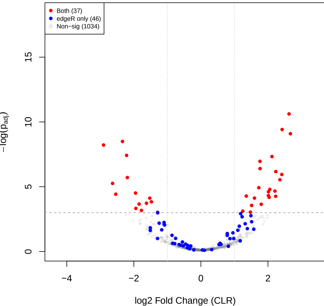
kin vs mage – CLR volcano (edgeR RLE sig overlay)
