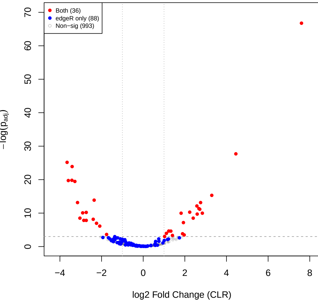
pup vs mage – CLR volcano (edgeR RLE sig overlay)
