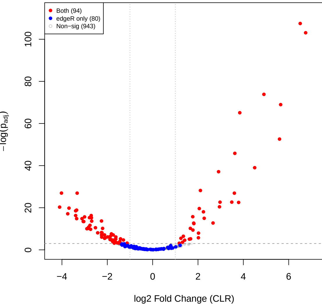
kin vs cent – CLR volcano (edgeR RLE sig overlay)
