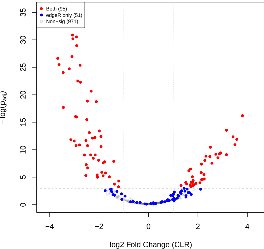
you vs mage – CLR volcano (edgeR RLE sig overlay)
