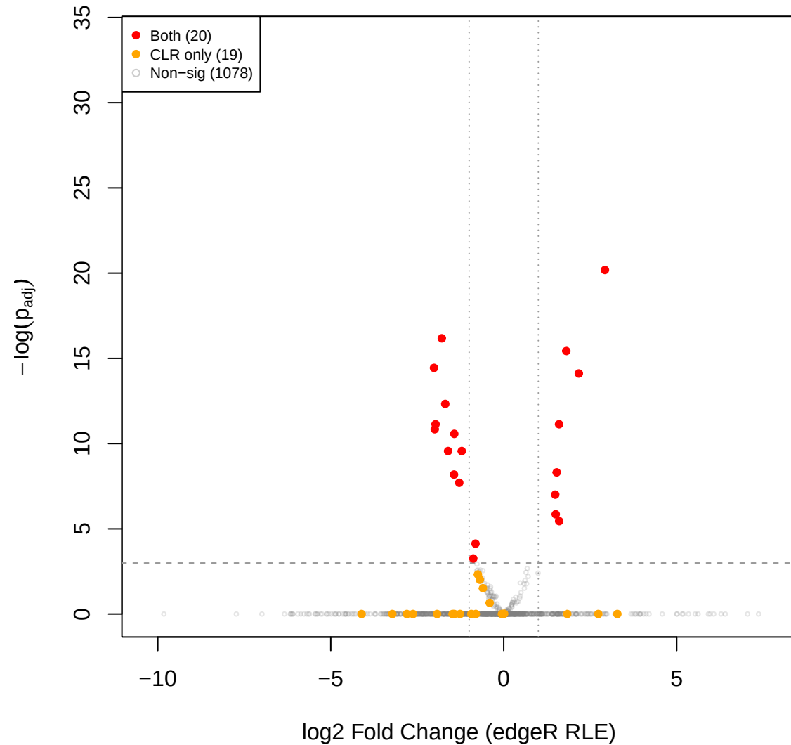
you vs eld – edgeR RLE volcano (CLR sig overlay)
