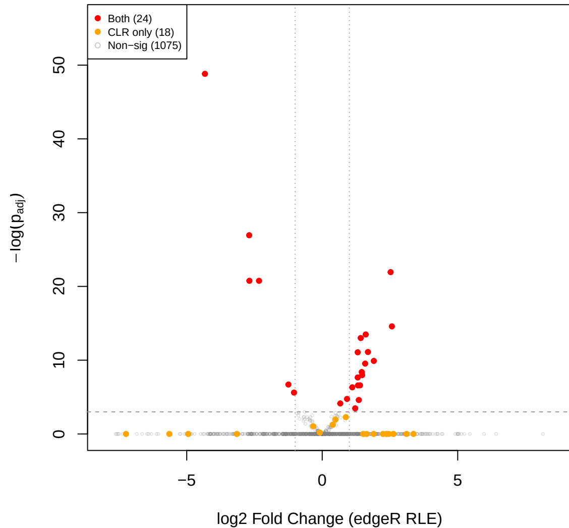
mid vs mage – edgeR RLE volcano (CLR sig overlay)
