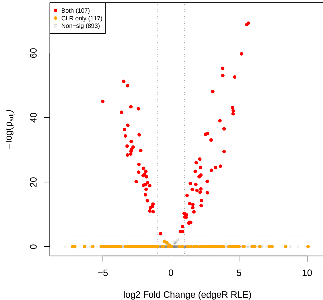
kin vs you – edgeR RLE volcano (CLR sig overlay)
