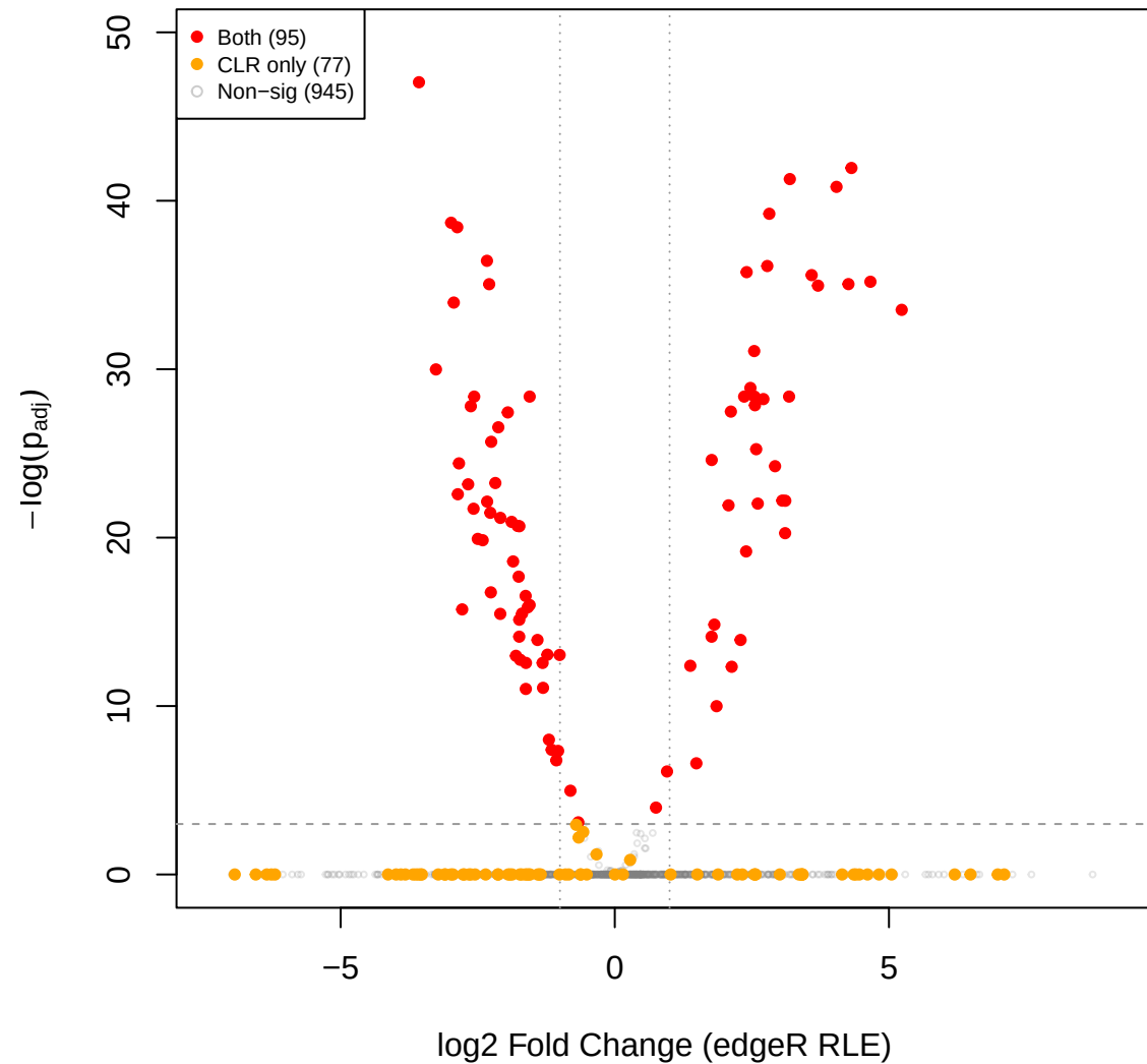
you vs mage – edgeR RLE volcano (CLR sig overlay)
