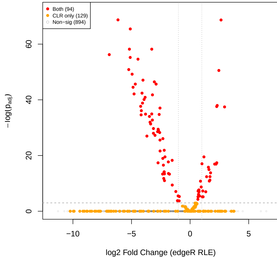
kin vs cent – edgeR RLE volcano (CLR sig overlay)
