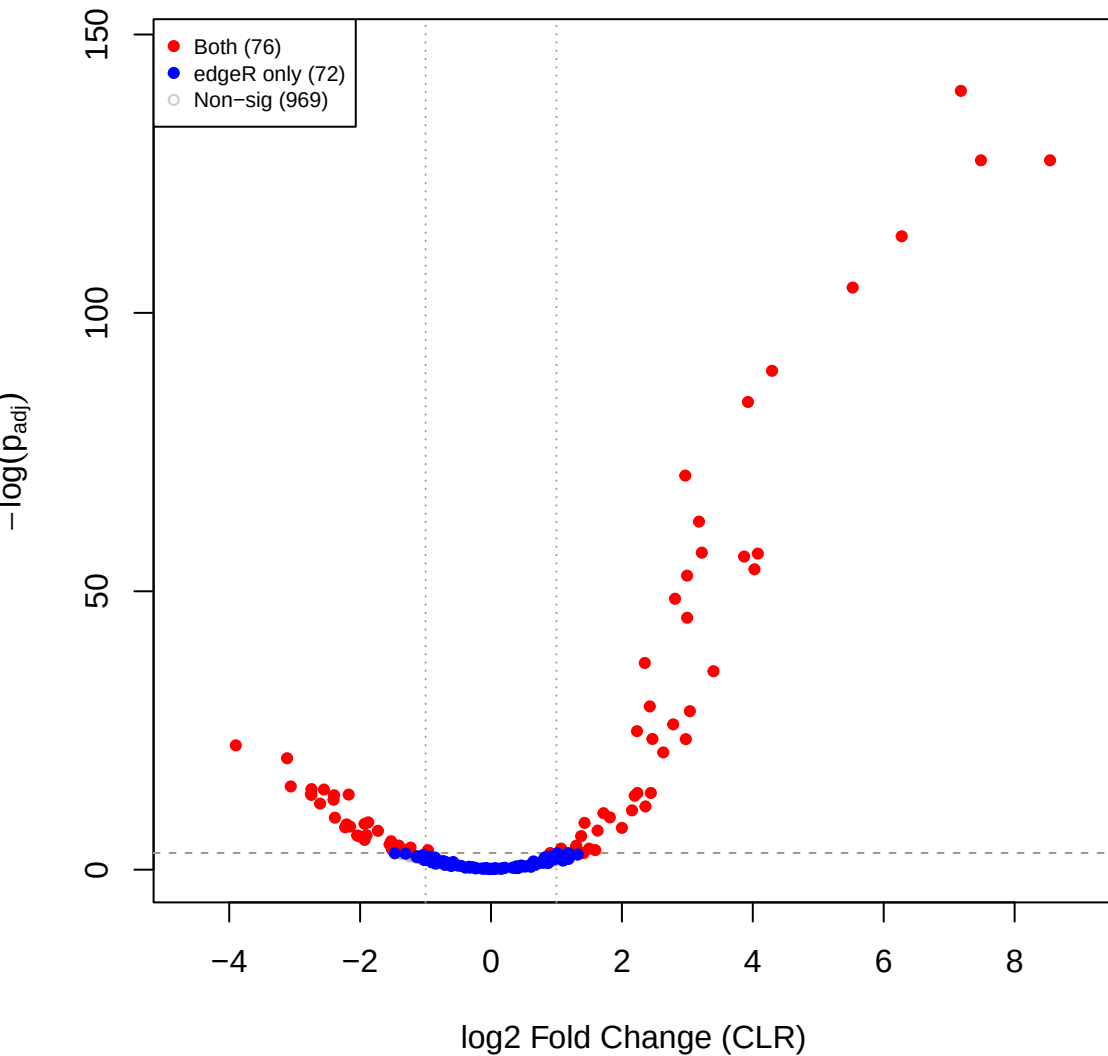
pup vs cent – CLR volcano (edgeR RLE sig overlay)
