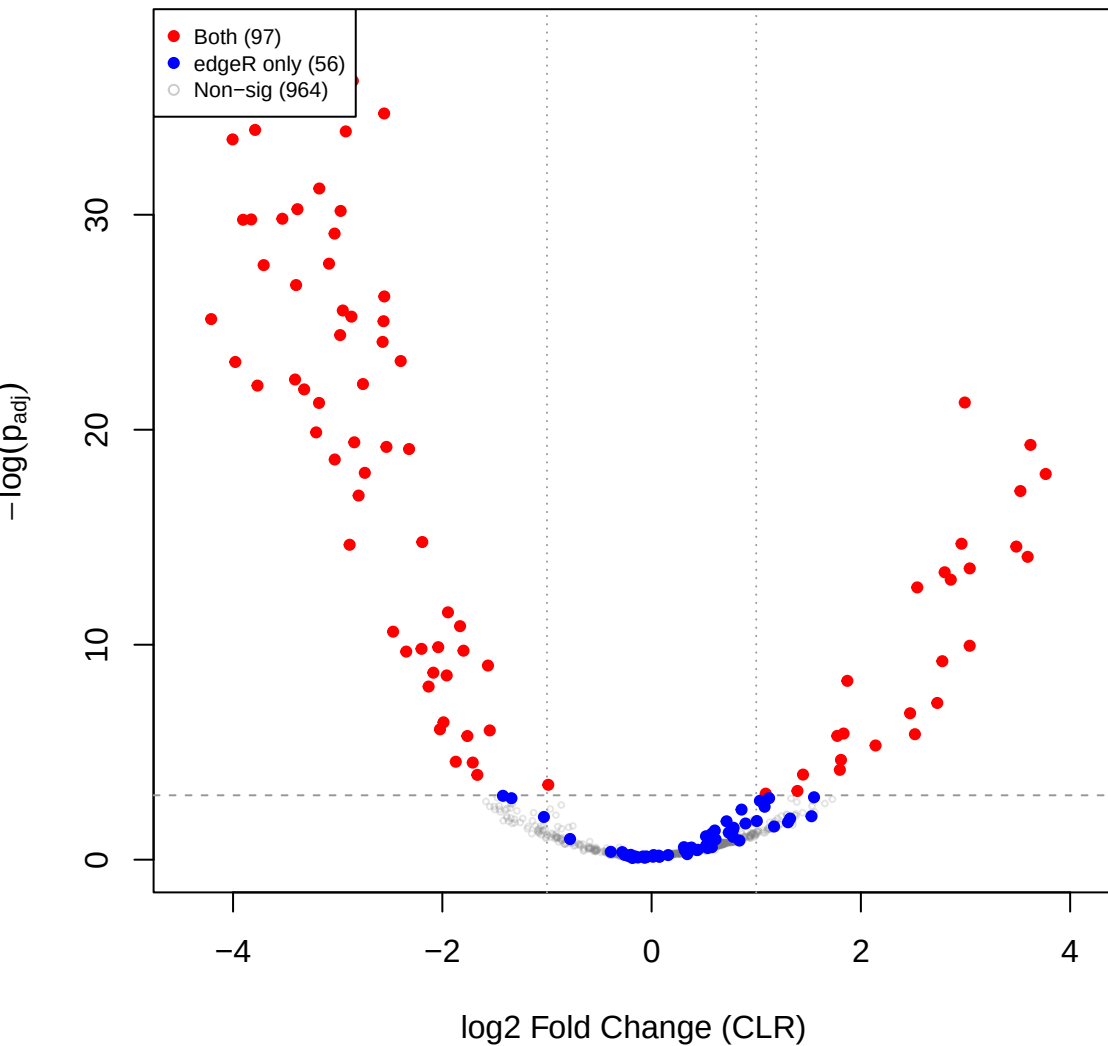
mid vs you – CLR volcano (edgeR RLE sig overlay)
