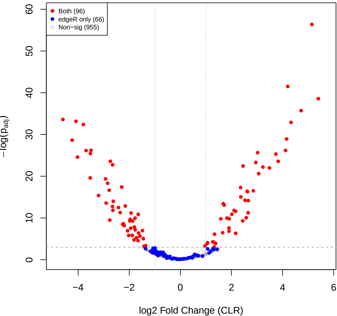
you vs cent – CLR volcano (edgeR RLE sig overlay)
