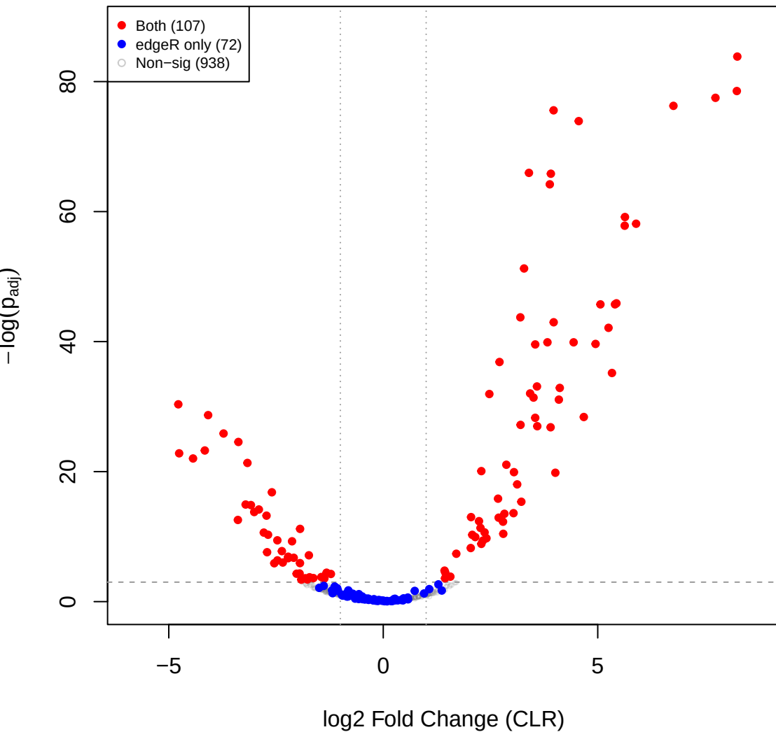
pup vs eld – CLR volcano (edgeR RLE sig overlay)
