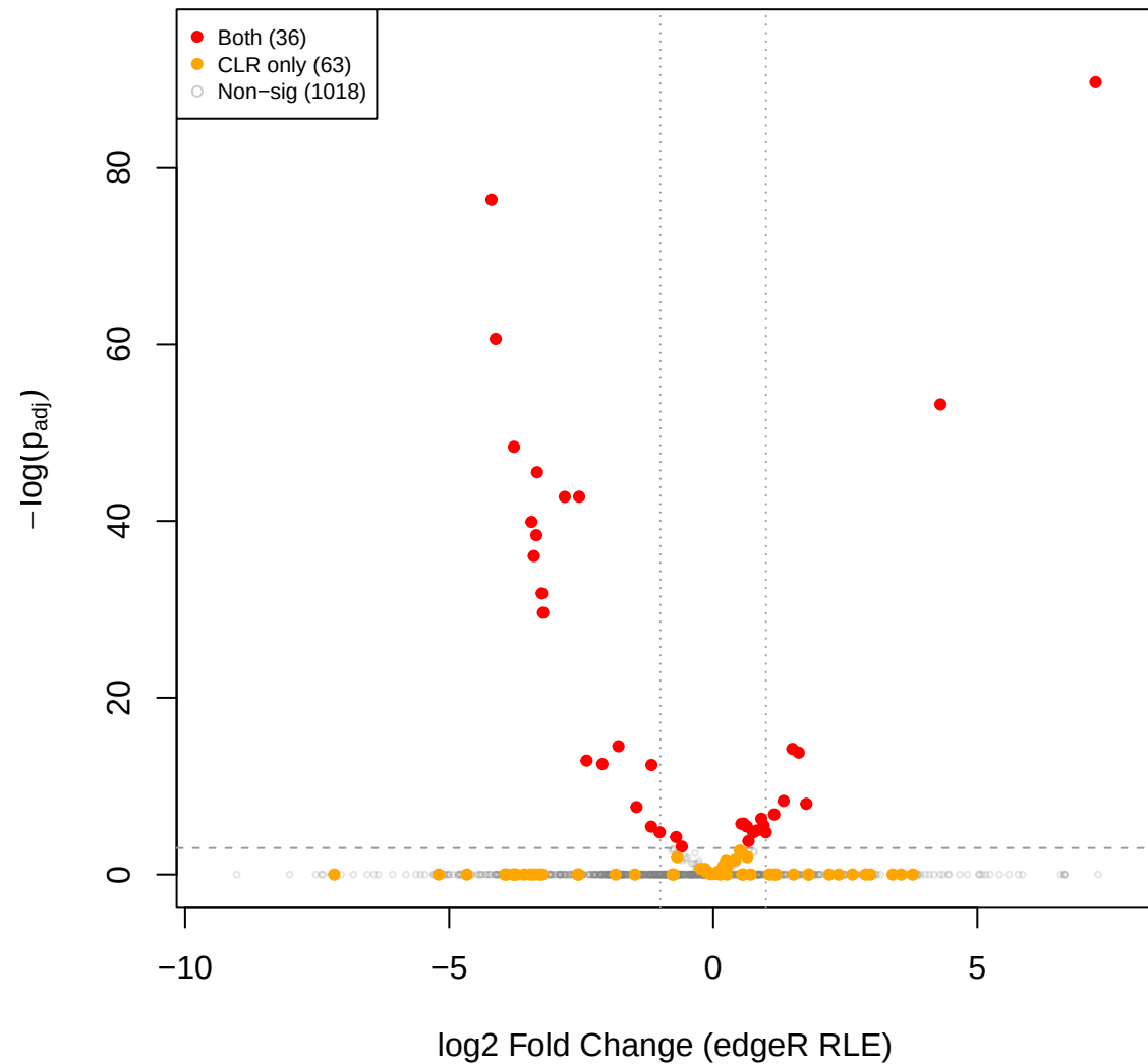
pup vs mage – edgeR RLE volcano (CLR sig overlay)
