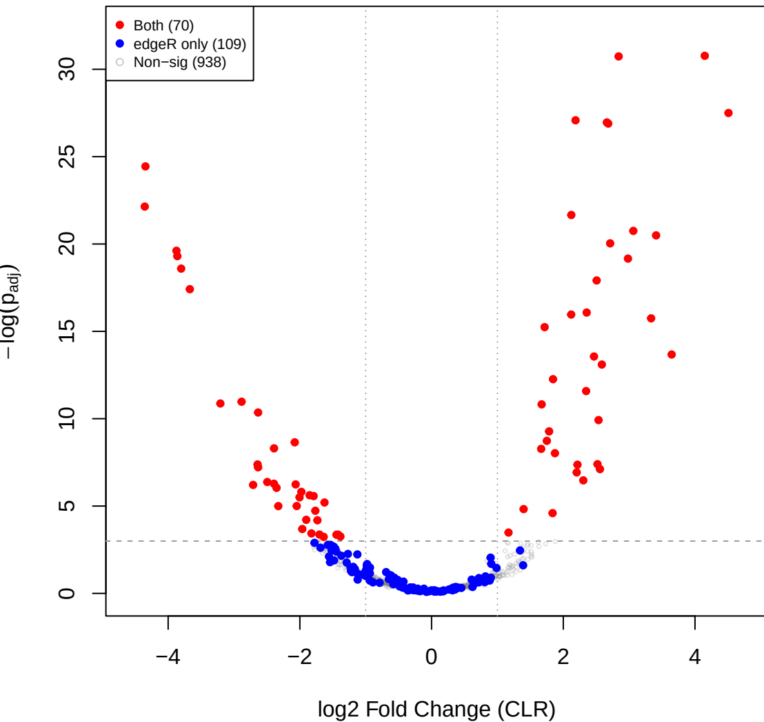
mage vs cent – CLR volcano (edgeR RLE sig overlay)
