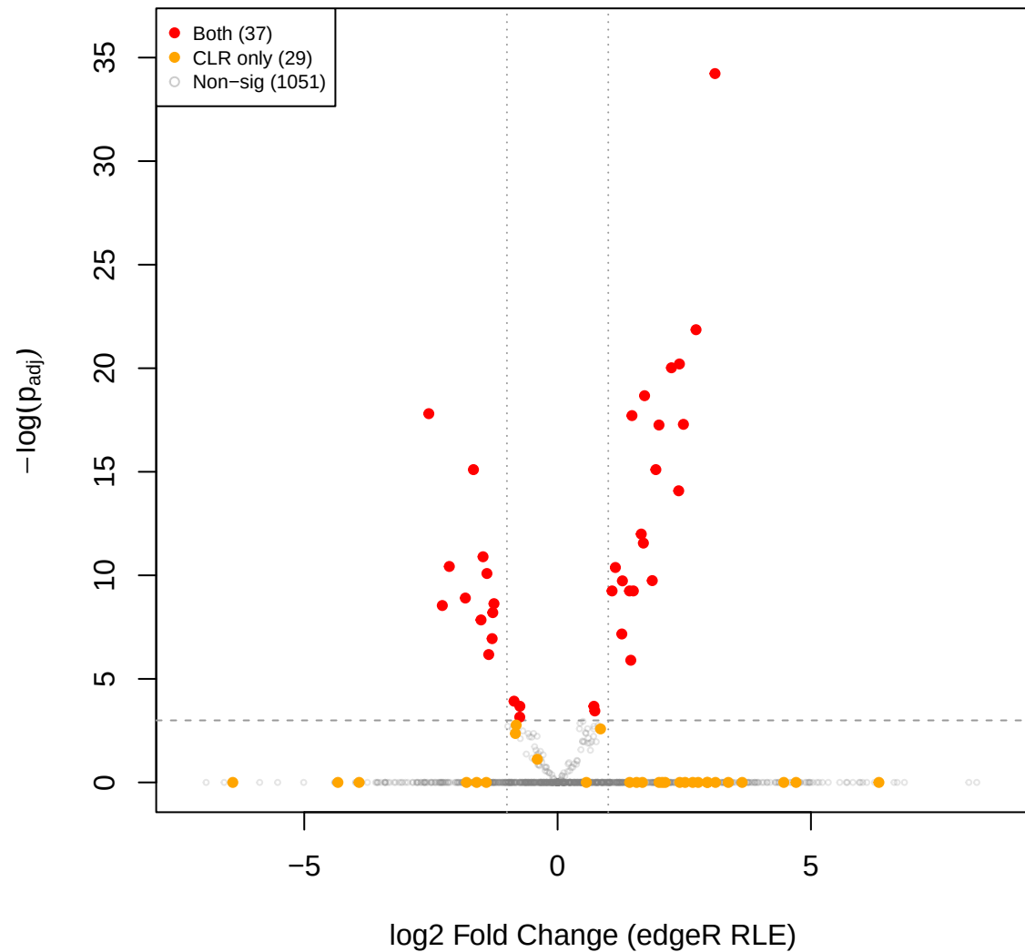
kin vs mage – edgeR RLE volcano (CLR sig overlay)
