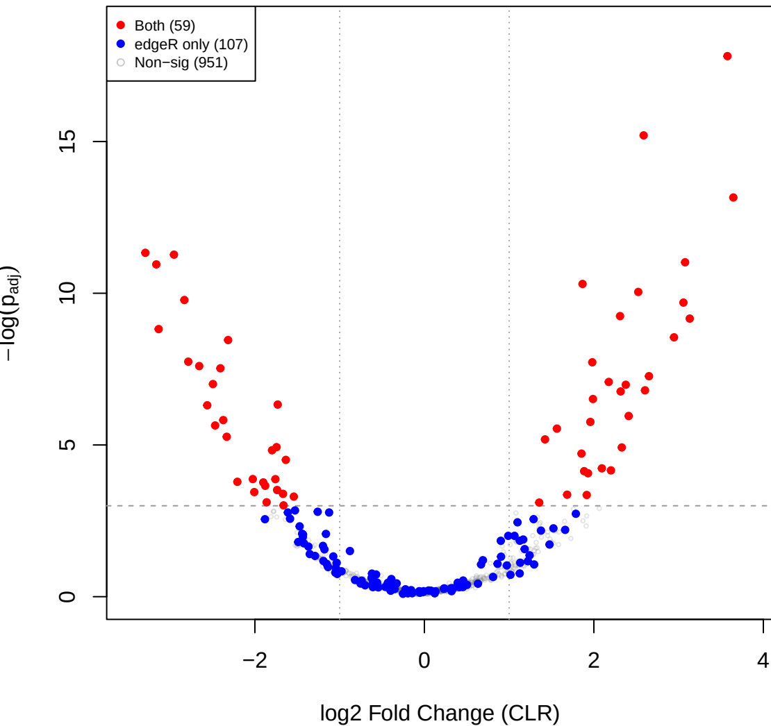
eld vs cent – CLR volcano (edgeR RLE sig overlay)
