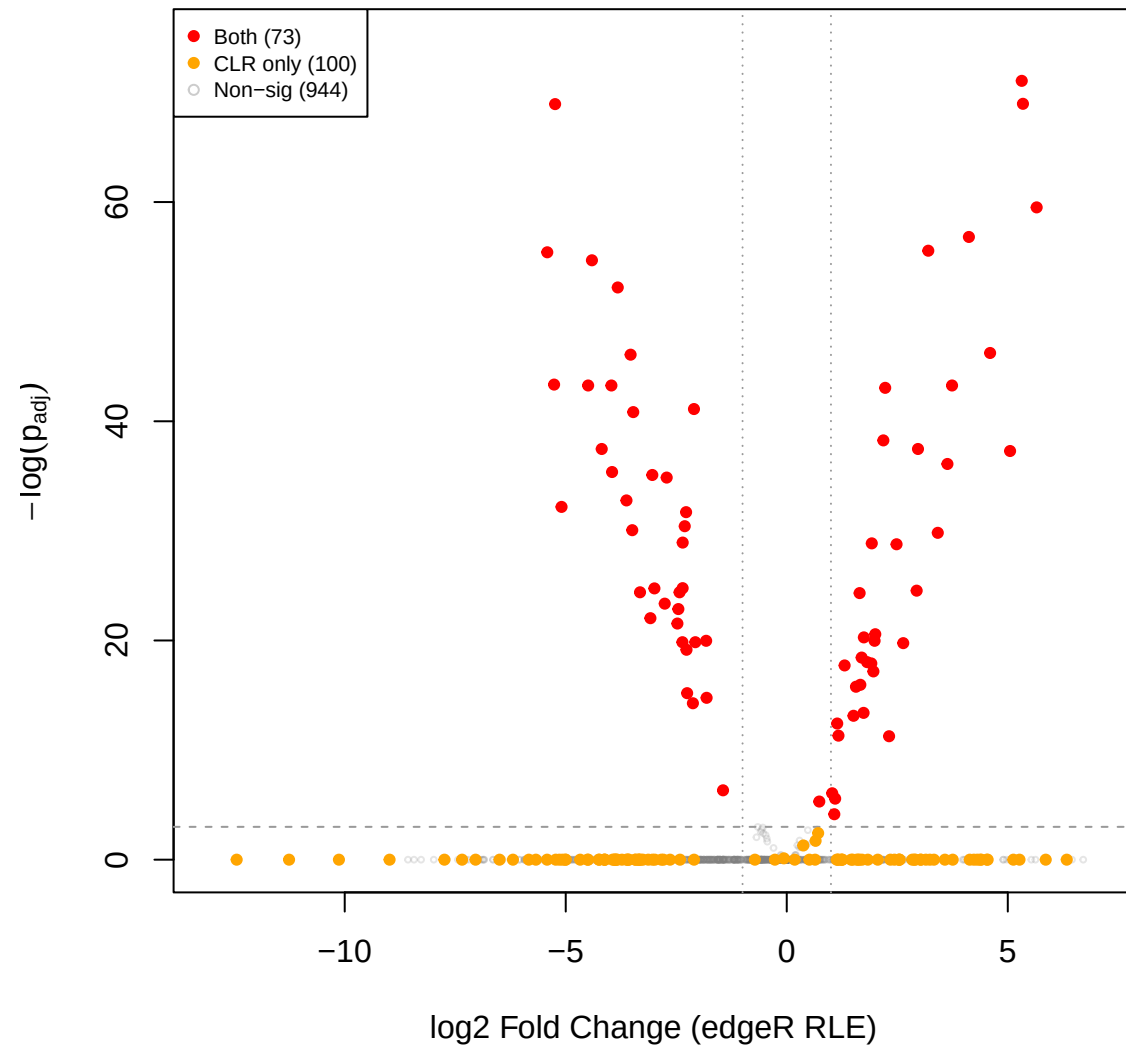
kin vs eld – edgeR RLE volcano (CLR sig overlay)
