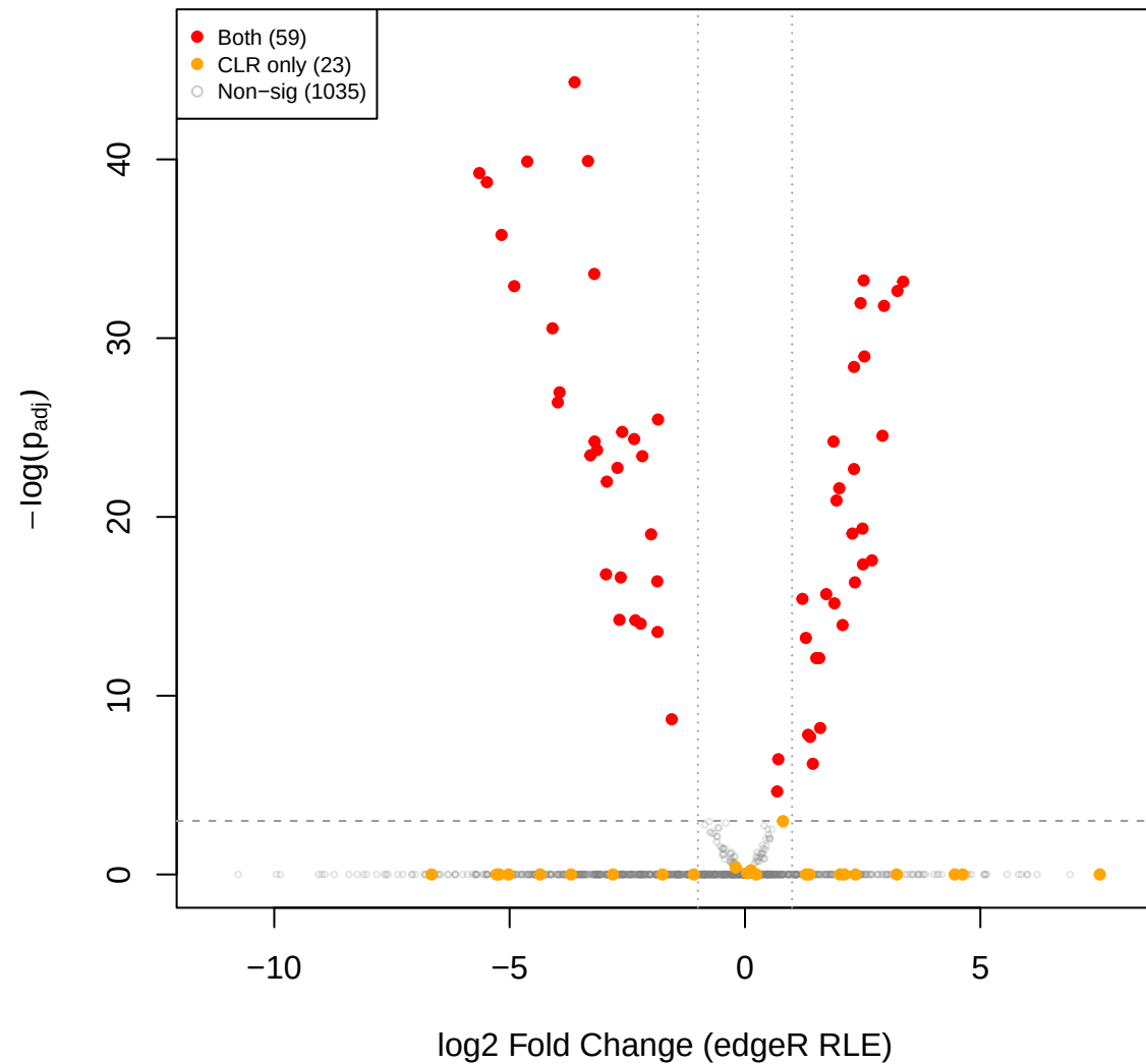
eld vs cent – edgeR RLE volcano (CLR sig overlay)
