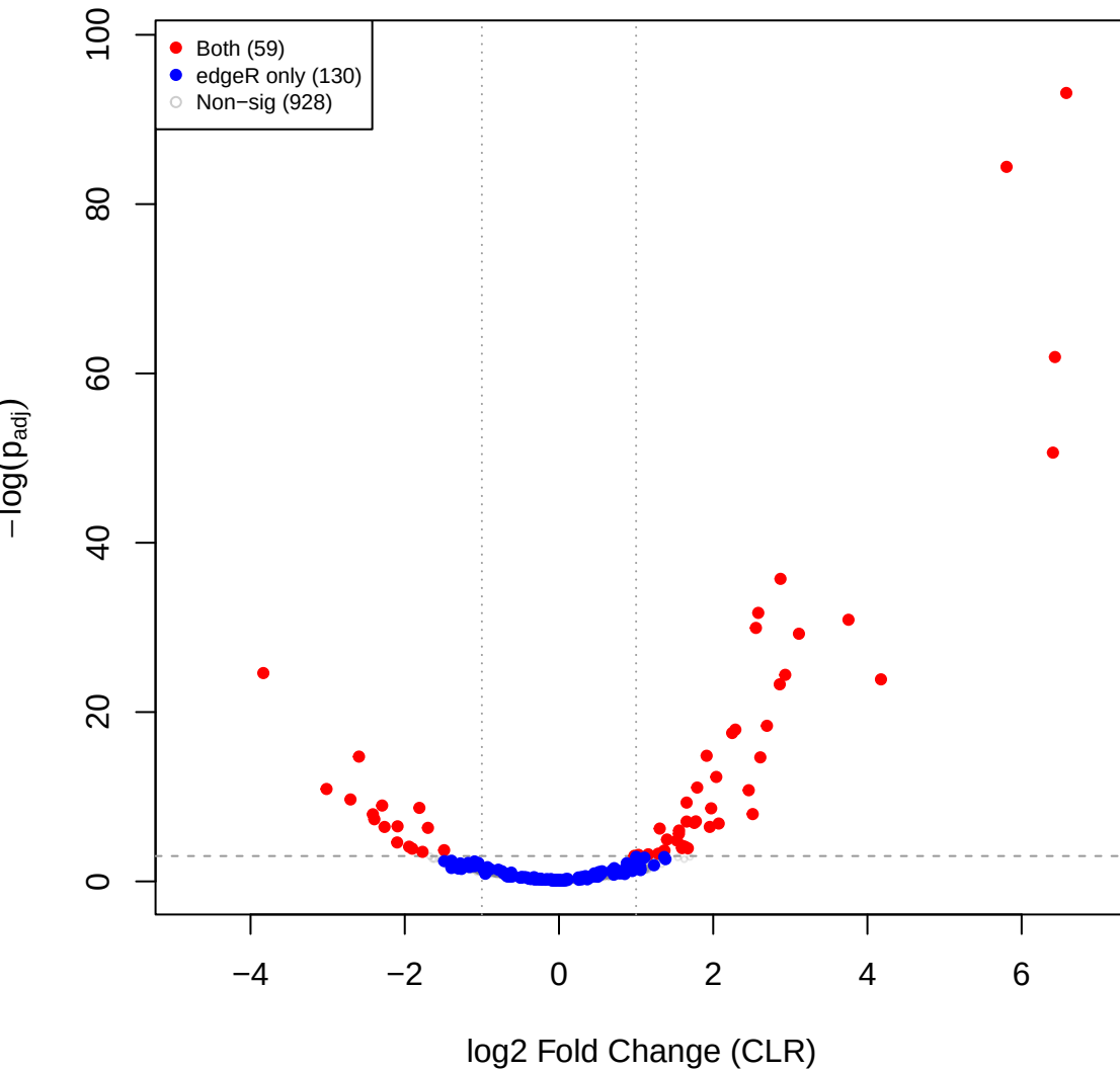
mid vs cent – CLR volcano (edgeR RLE sig overlay)
