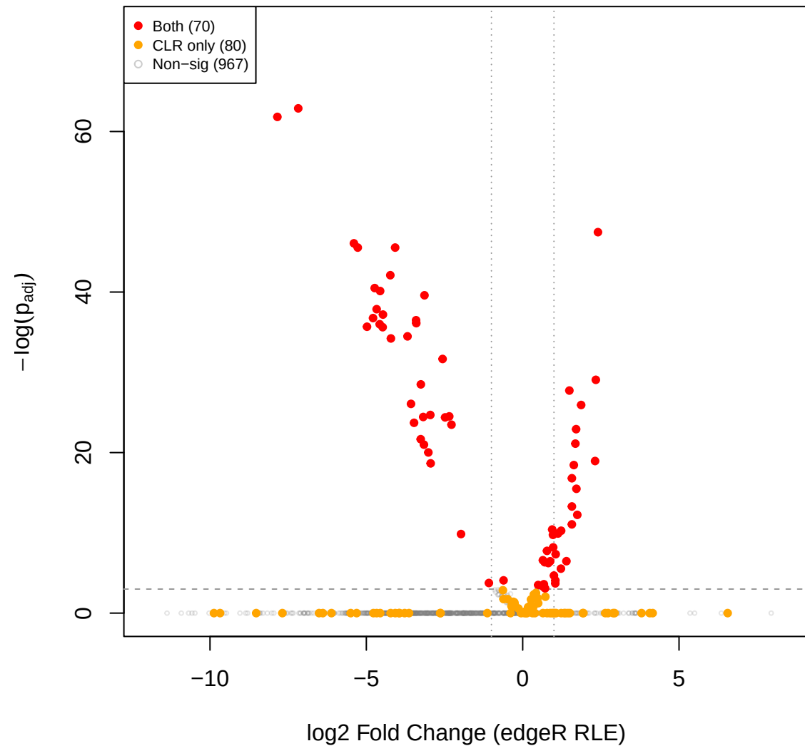
mage vs cent – edgeR RLE volcano (CLR sig overlay)
