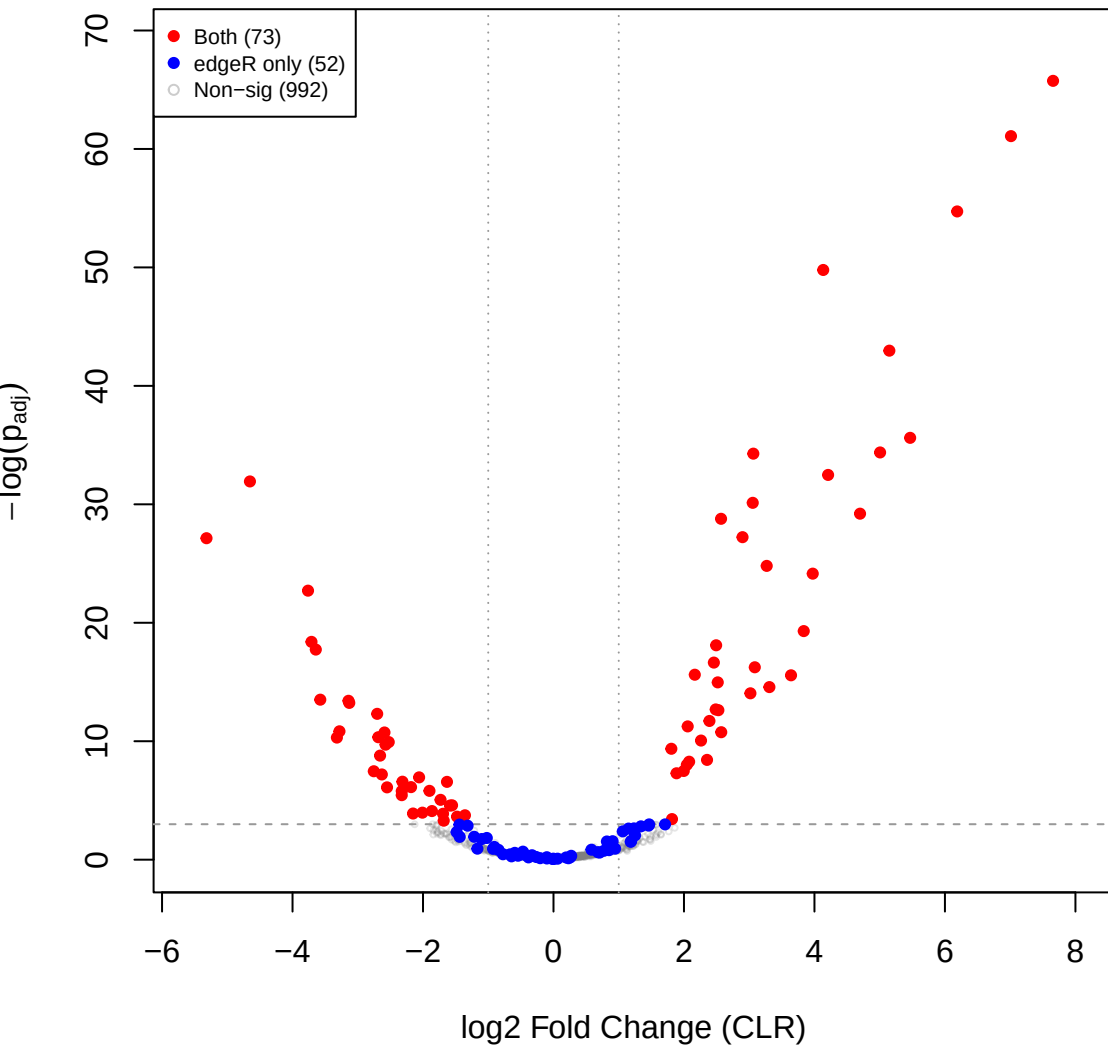
kin vs eld – CLR volcano (edgeR RLE sig overlay)
