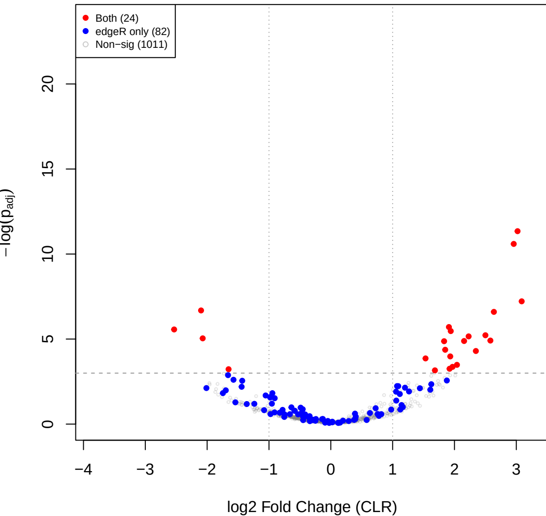
mid vs mage – CLR volcano (edgeR RLE sig overlay)
