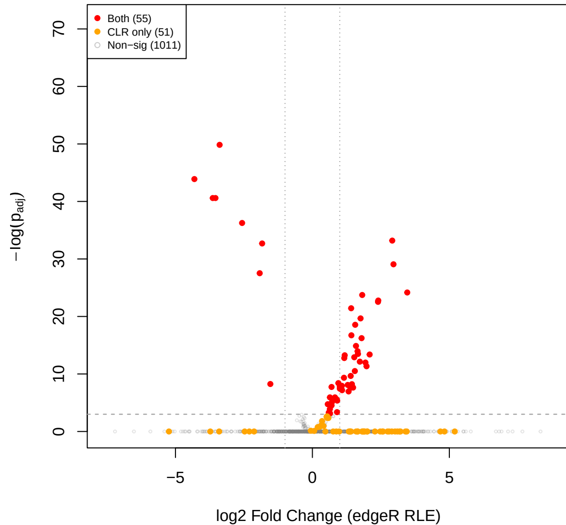
kin vs mid – edgeR RLE volcano (CLR sig overlay)
