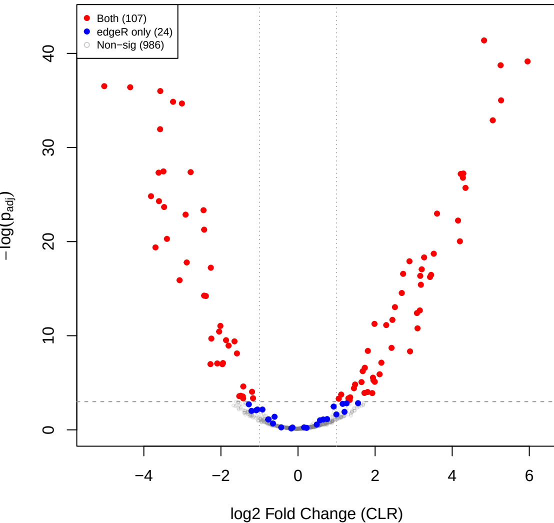
kin vs you – CLR volcano (edgeR RLE sig overlay)
