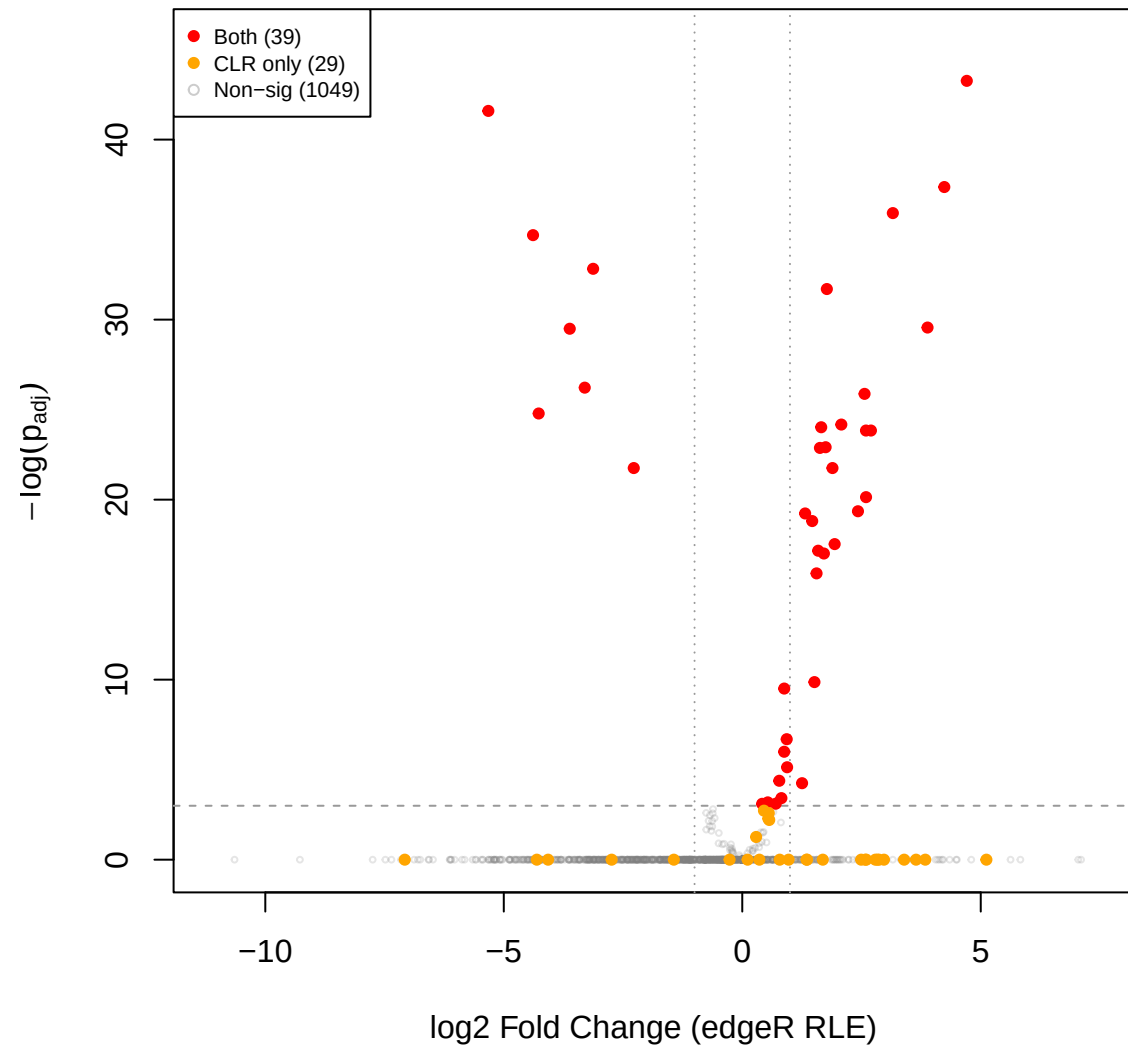
mage vs eld – edgeR RLE volcano (CLR sig overlay)
