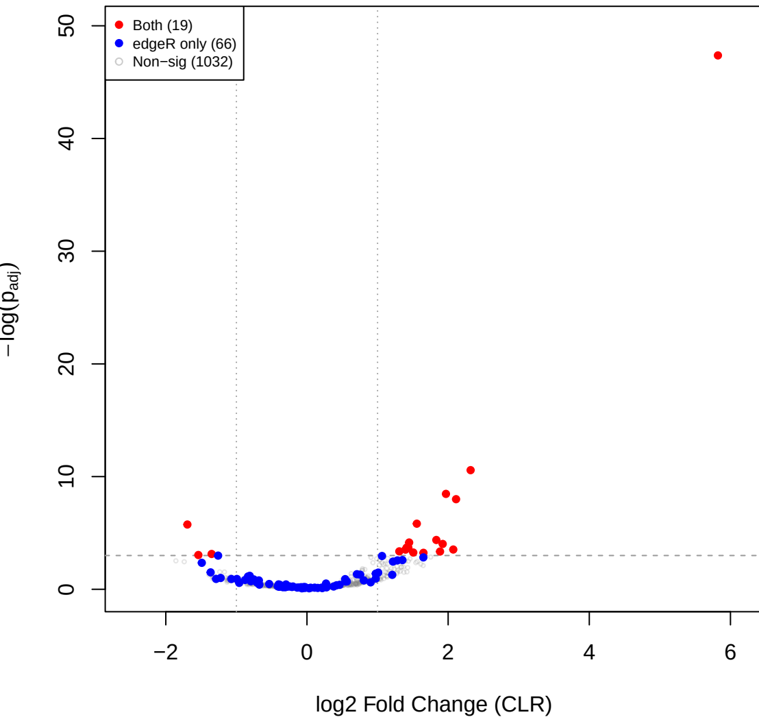
kin vs pup – CLR volcano (edgeR RLE sig overlay)
