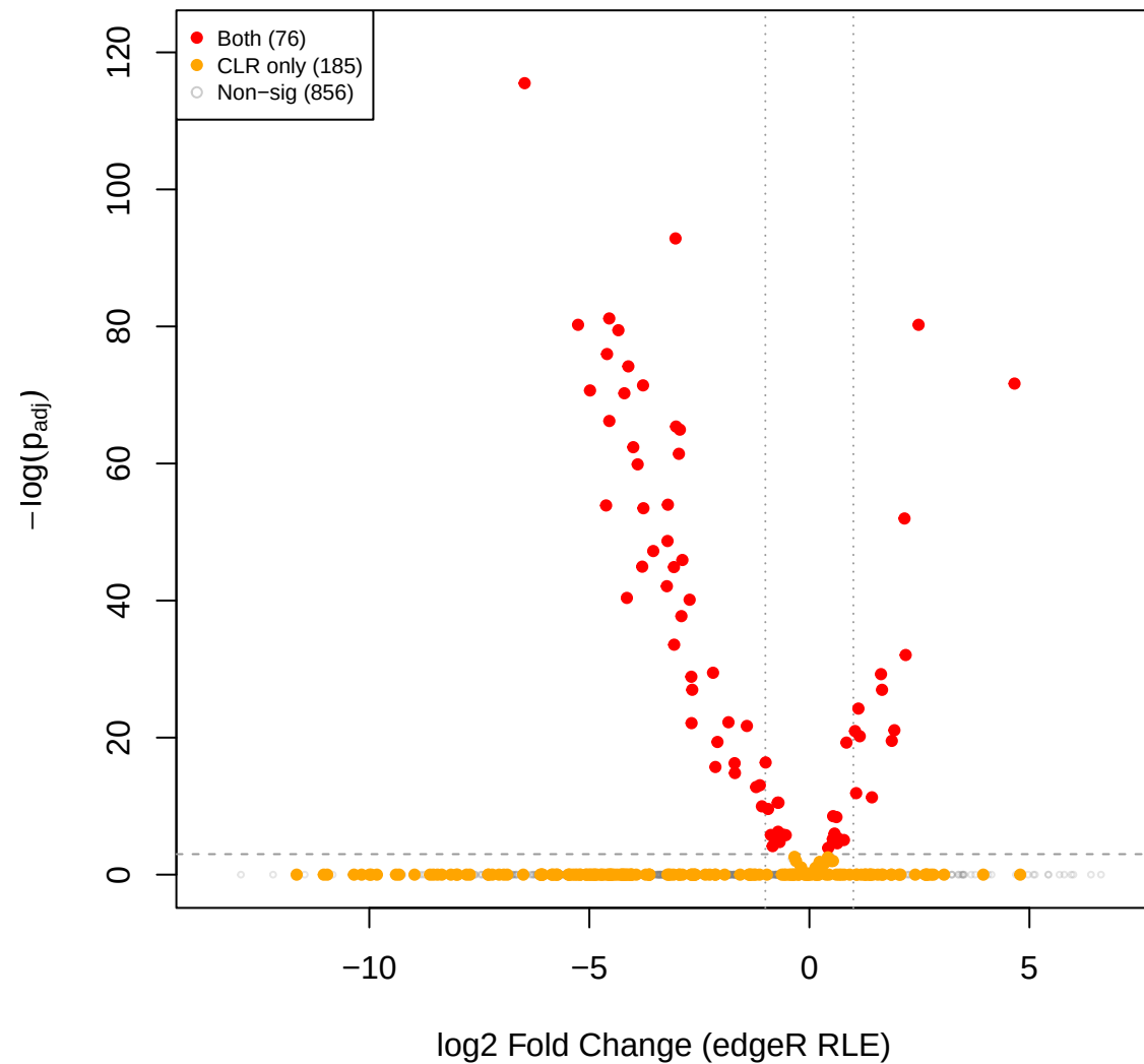
pup vs cent – edgeR RLE volcano (CLR sig overlay)
