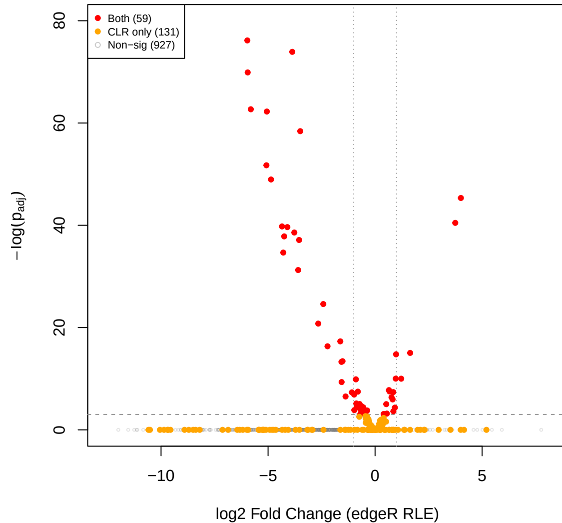
mid vs cent – edgeR RLE volcano (CLR sig overlay)
