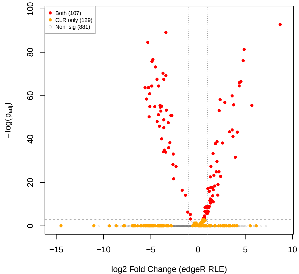
pup vs eld – edgeR RLE volcano (CLR sig overlay)
