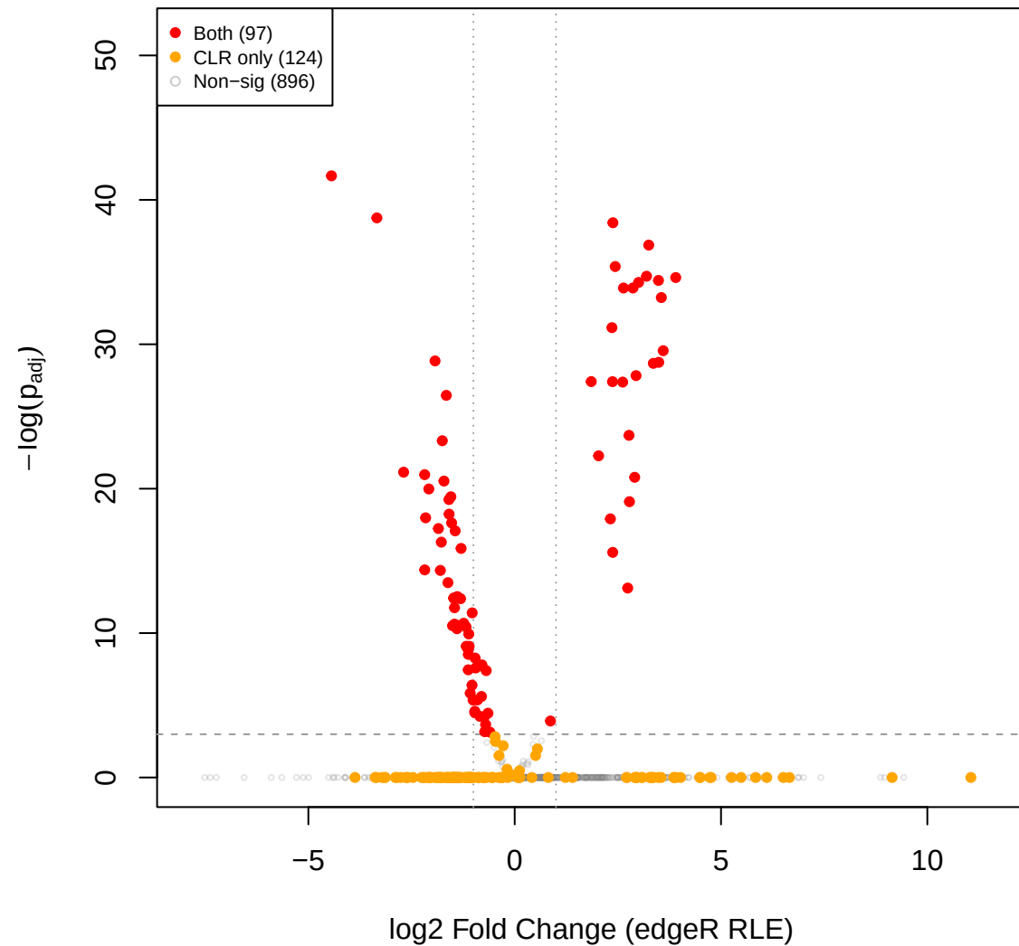
mid vs you – edgeR RLE volcano (CLR sig overlay)
