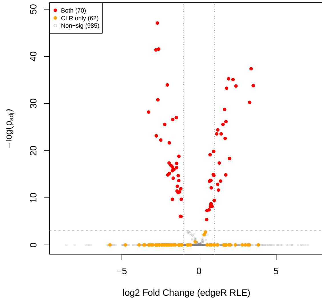
pup vs mid – edgeR RLE volcano (CLR sig overlay)
