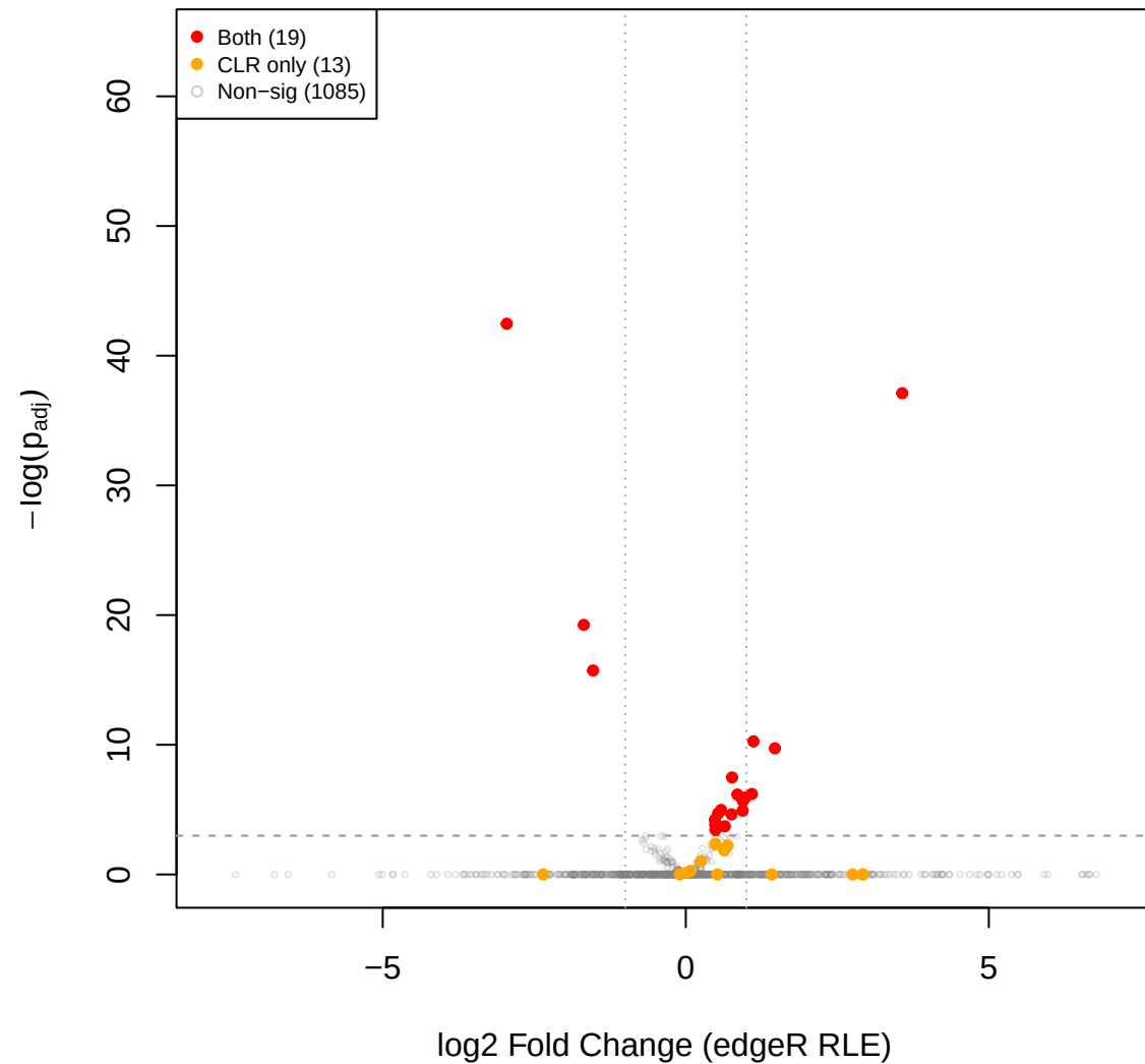
kin vs pup – edgeR RLE volcano (CLR sig overlay)
