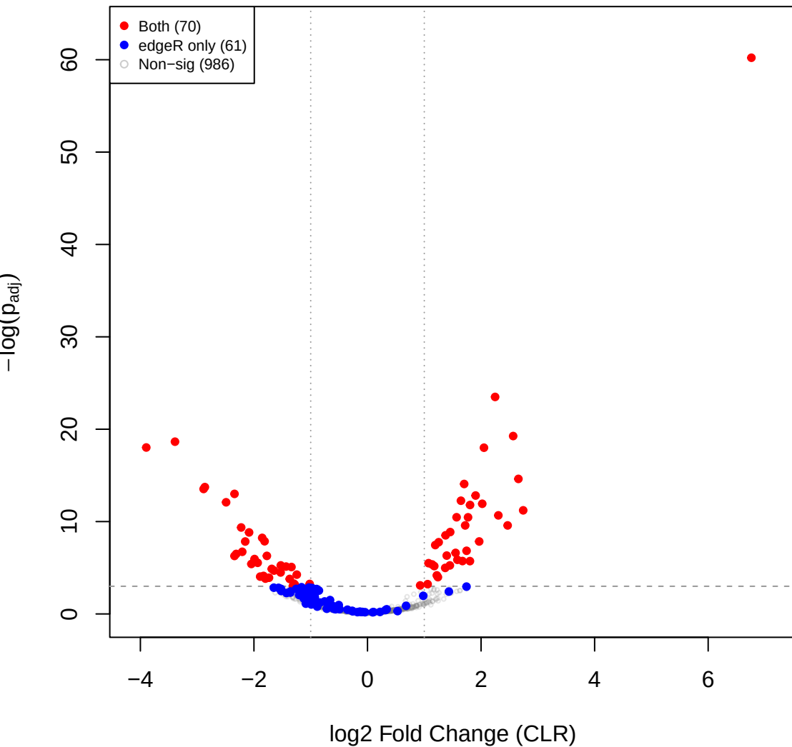
pup vs mid – CLR volcano (edgeR RLE sig overlay)
