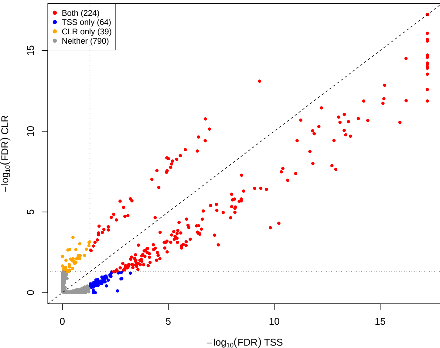
mid vs you – CLR vs TSS(const=-0.3) (gamma = 0.001)
