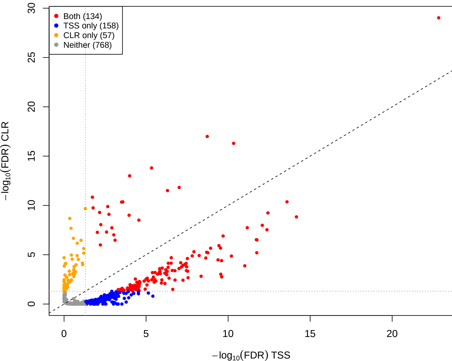
mid vs pup – CLR vs TSS(const=-0.3) (gamma = 0.001)
