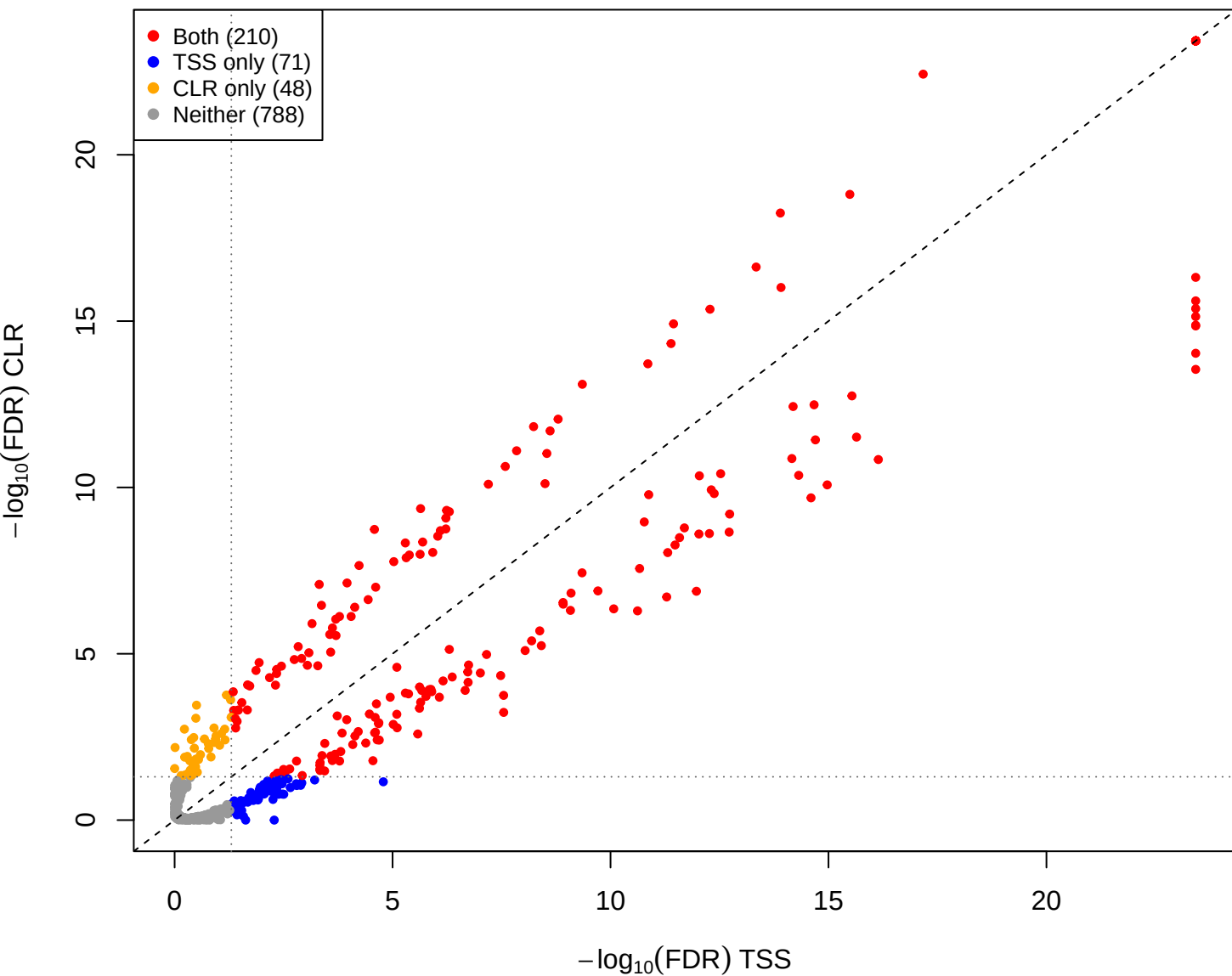
kin vs you – CLR vs TSS(const=-0.3) (gamma = 0.001)
