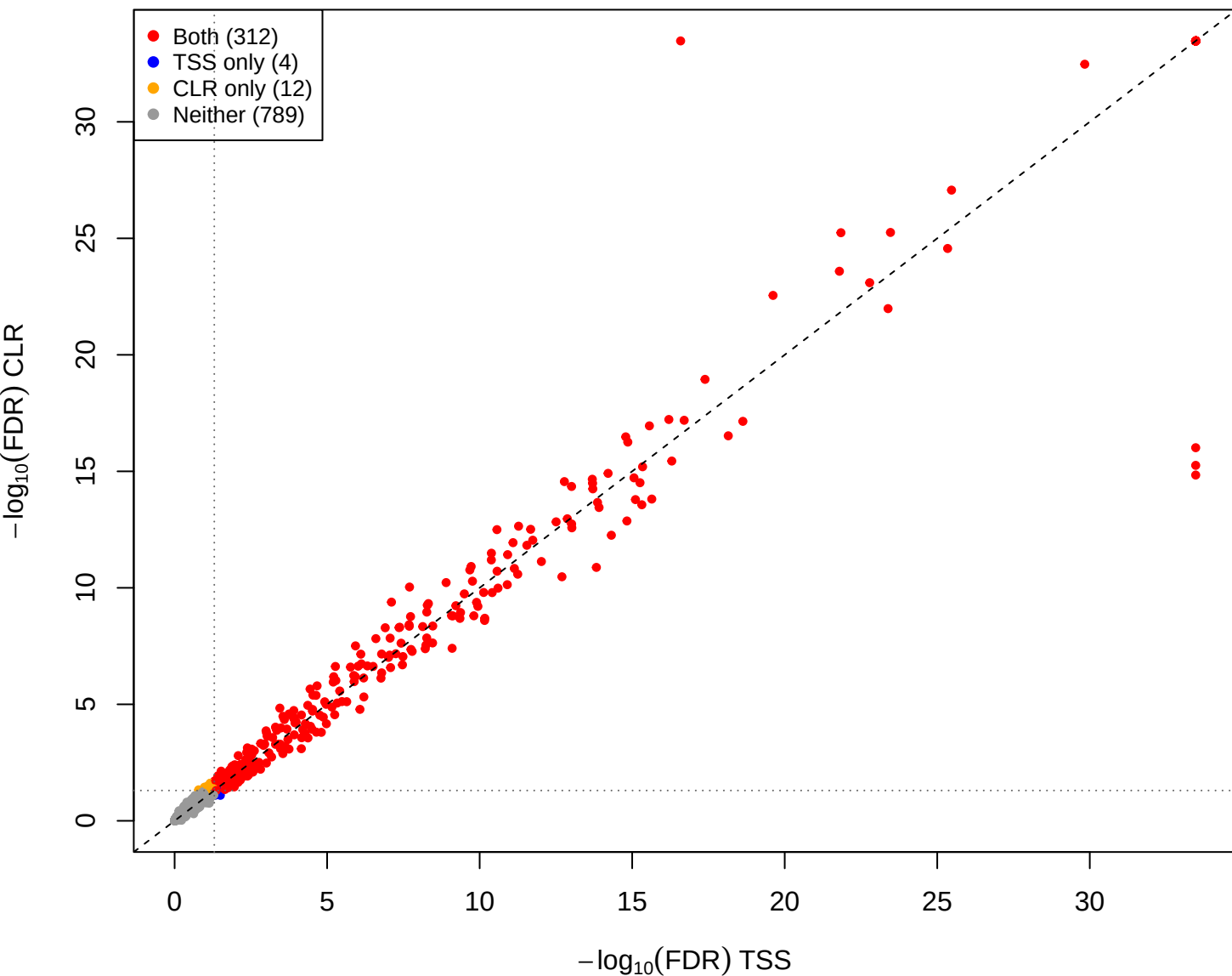
pup vs you - CLR vs TSS(const=-0.3) (gamma = 0.001)
