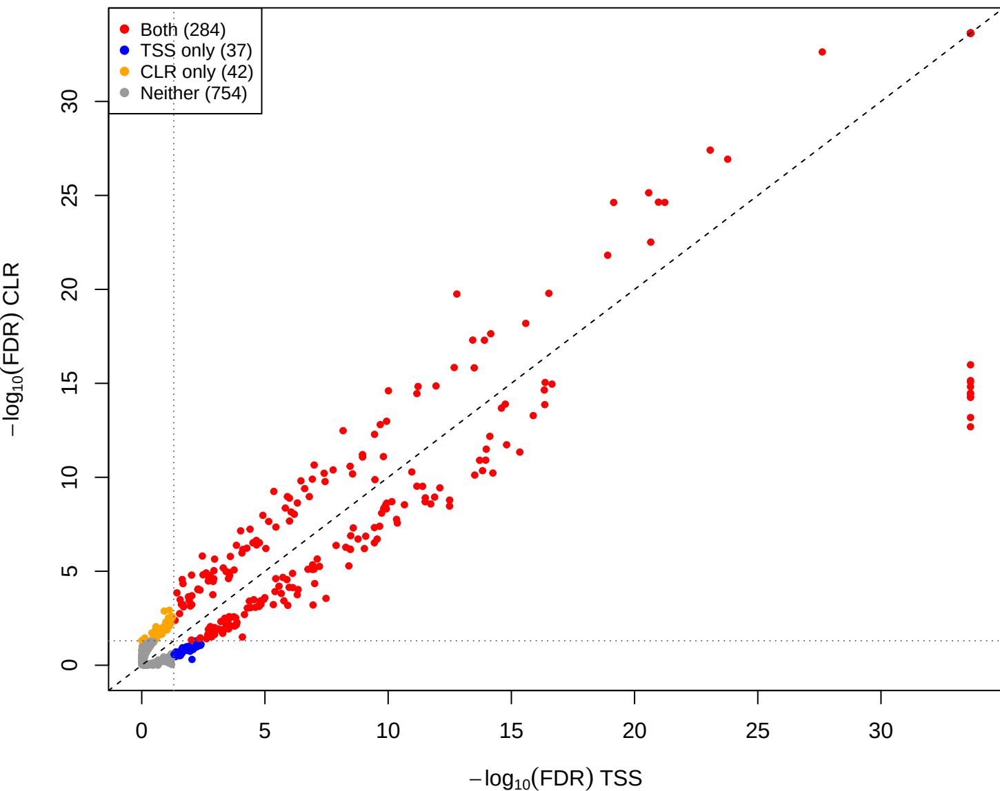
pup vs you - CLR vs TSS(const=-0.6) (gamma = 0.001)
