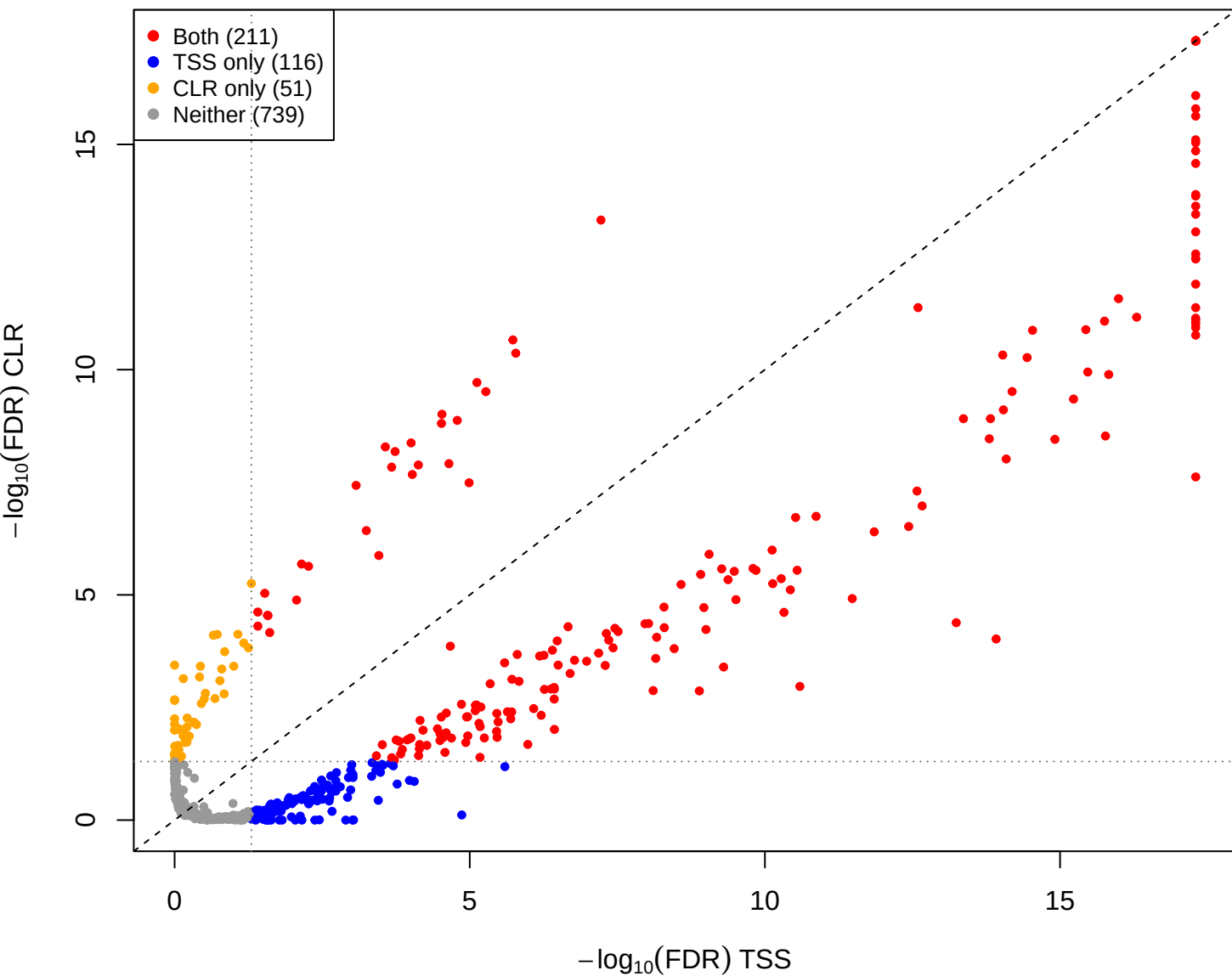
mid vs you – CLR vs TSS(const=-0.6) (gamma = 0.001)
