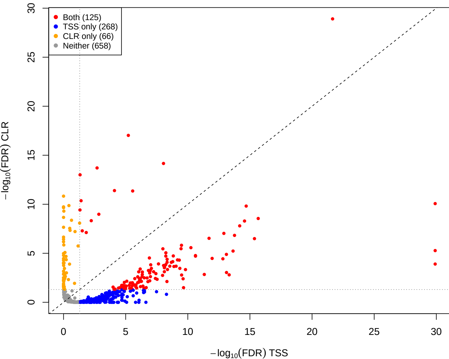
mid vs pup – CLR vs TSS(const=-0.6) (gamma = 0.001)
