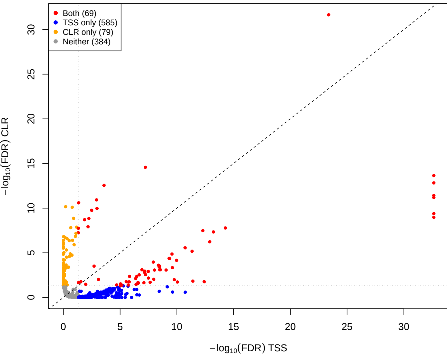
mage vs pup – CLR vs TSS(const=-1) (gamma = 0.001)
