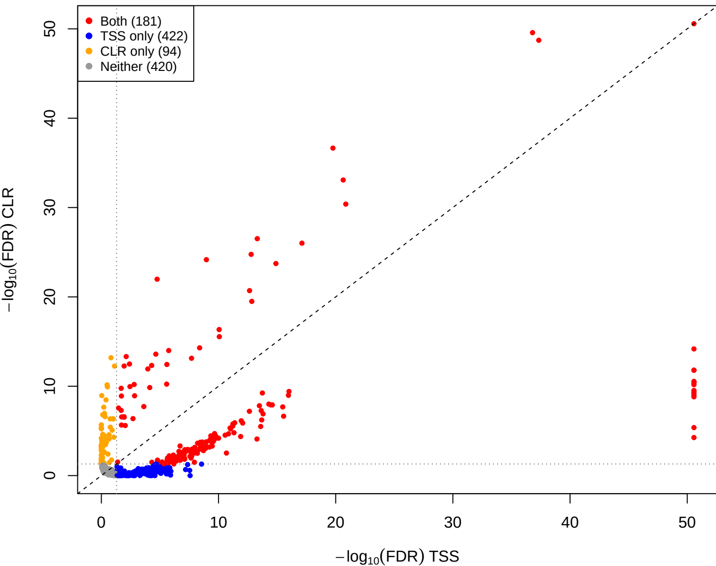
cent vs kin – CLR vs TSS(const=-1) (gamma = 0.001)
