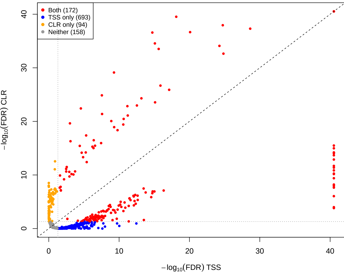
eld vs pup – CLR vs TSS(const=-1) (gamma = 0.001)
