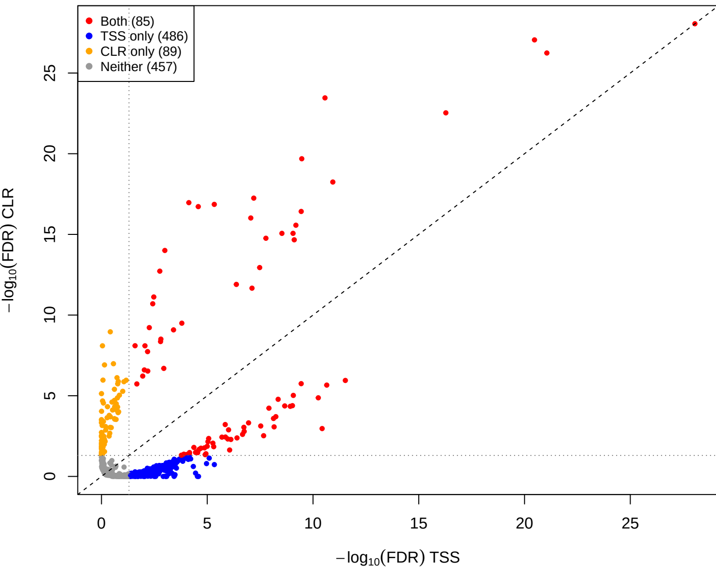
eld vs mid – CLR vs TSS(const=-1) (gamma = 0.001)
