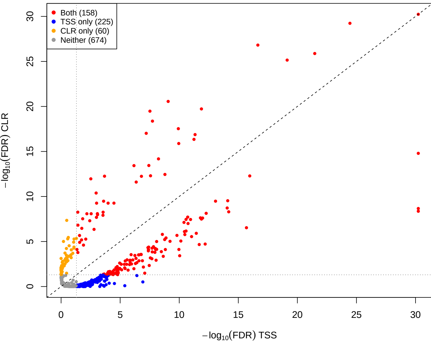
eld vs kin - CLR vs TSS(const=-1) (gamma = 0.001)
