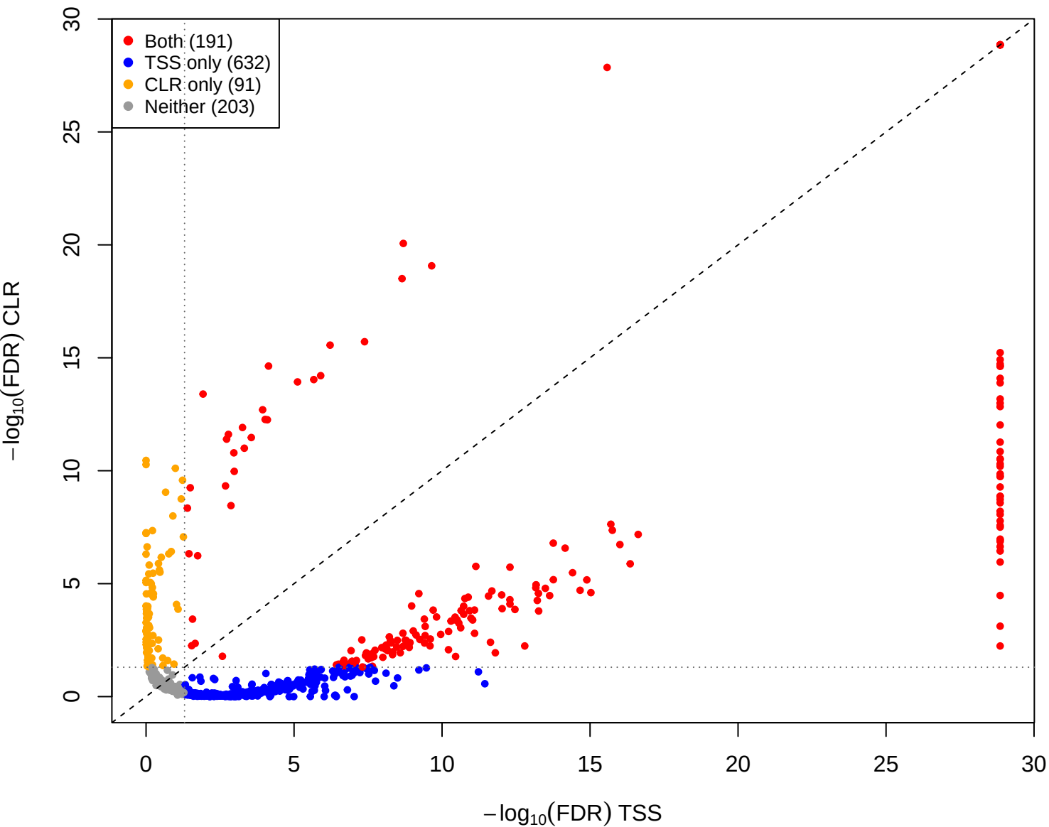
cent vs you - CLR vs TSS(const=-1) (gamma = 0.001)
