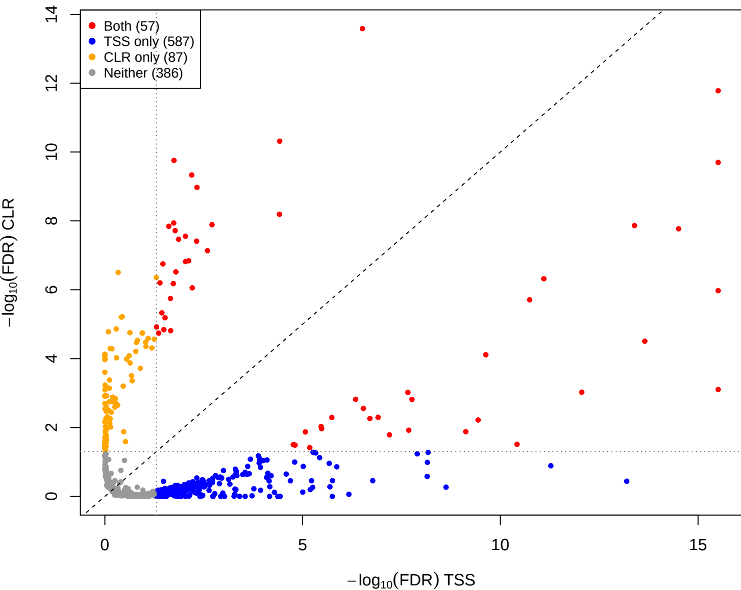
kin vs mid – CLR vs TSS(const=-1) (gamma = 0.001)
