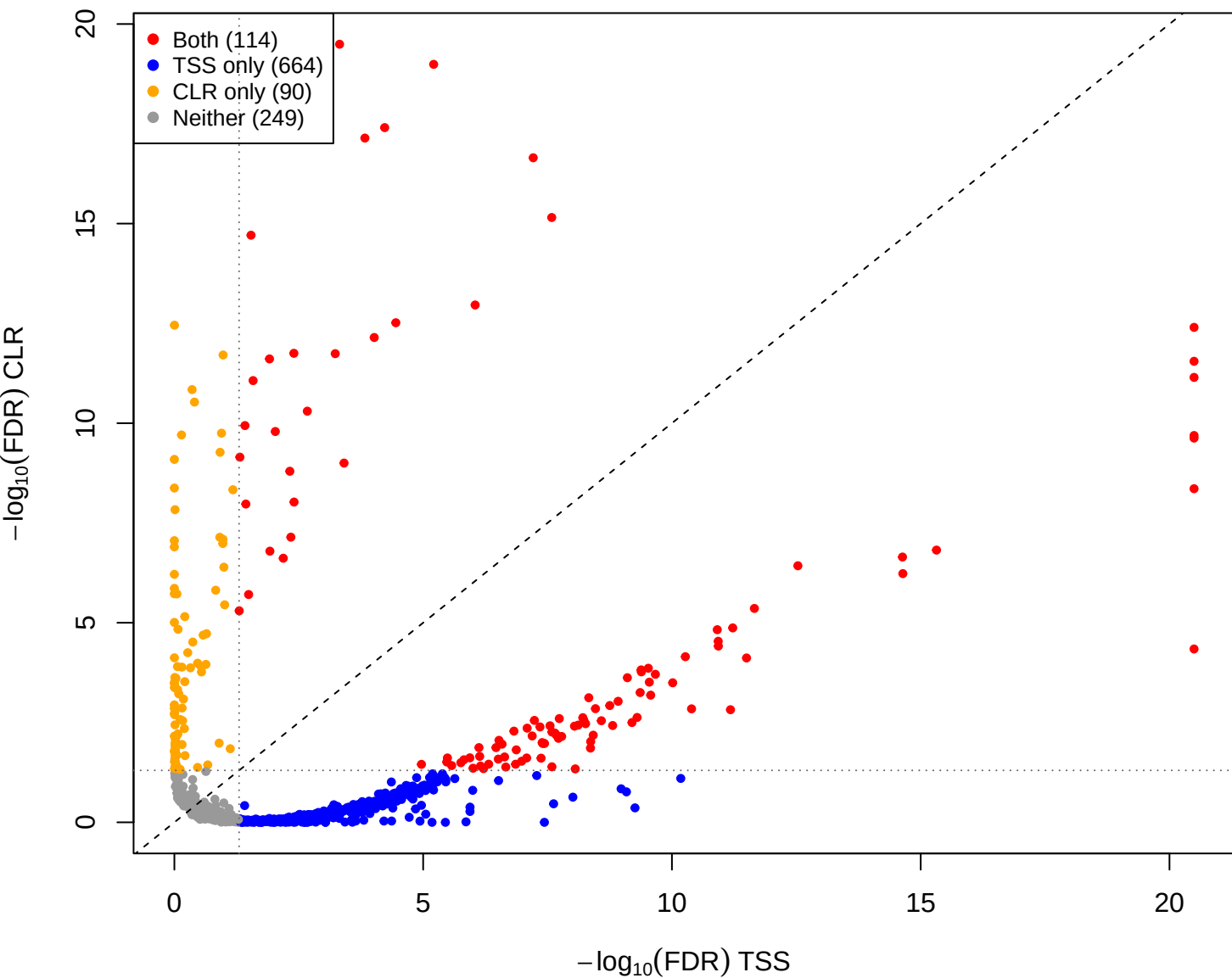
cent vs mage - CLR vs TSS(const=-1) (gamma = 0.001)
