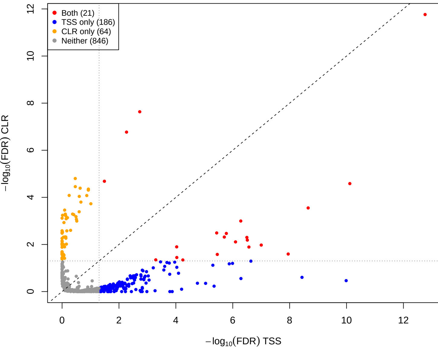
mage vs mid - CLR vs TSS(const=-1) (gamma = 0.001)
