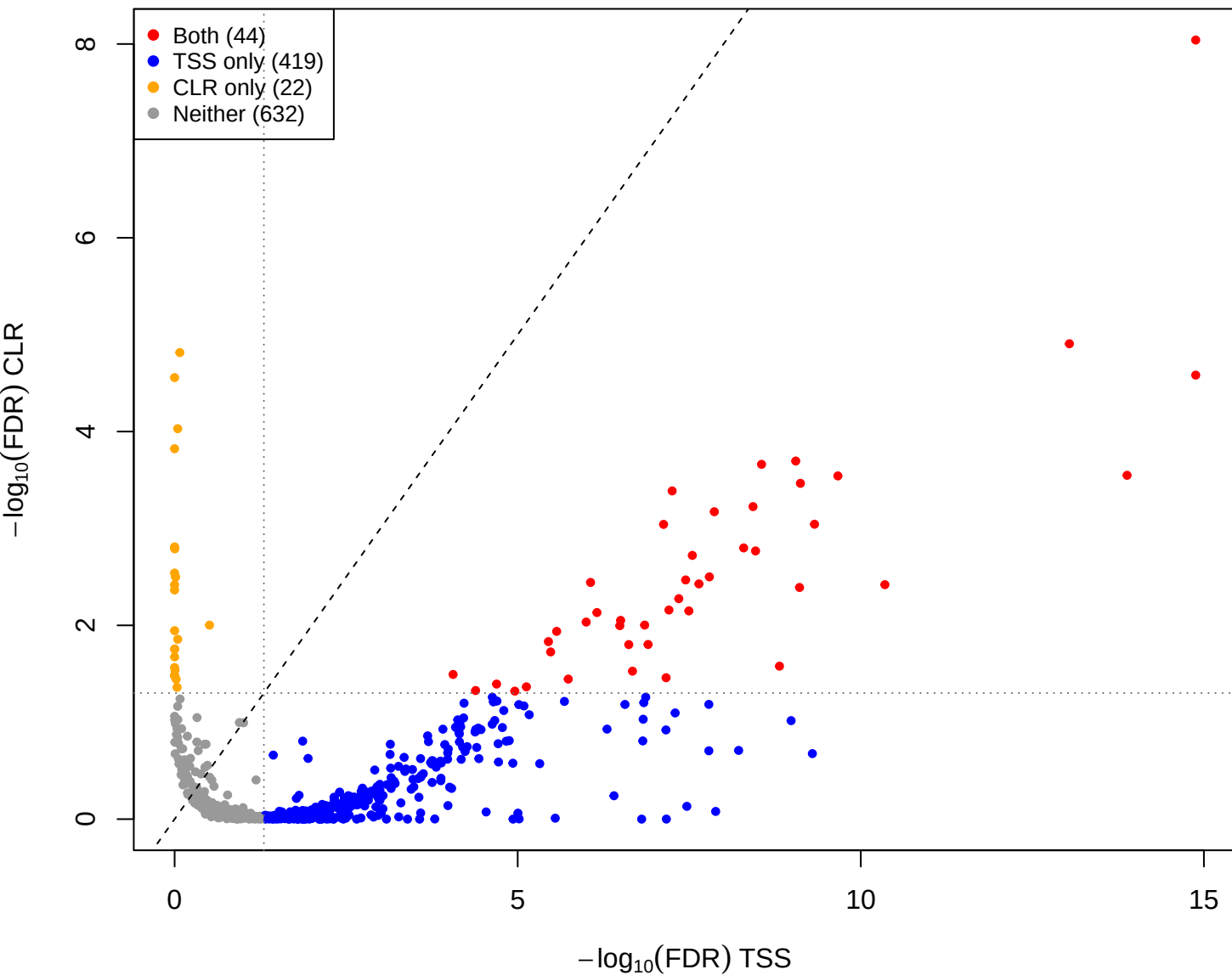
eld vs you – CLR vs TSS(const=-1) (gamma = 0.001)
