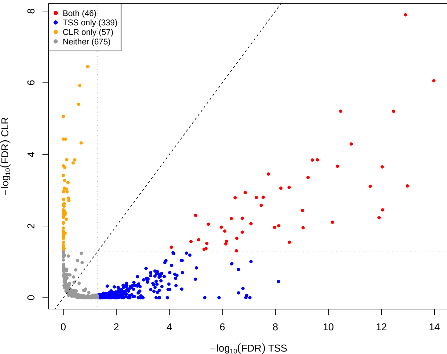
kin vs mage – CLR vs TSS(const=-1) (gamma = 0.001)
