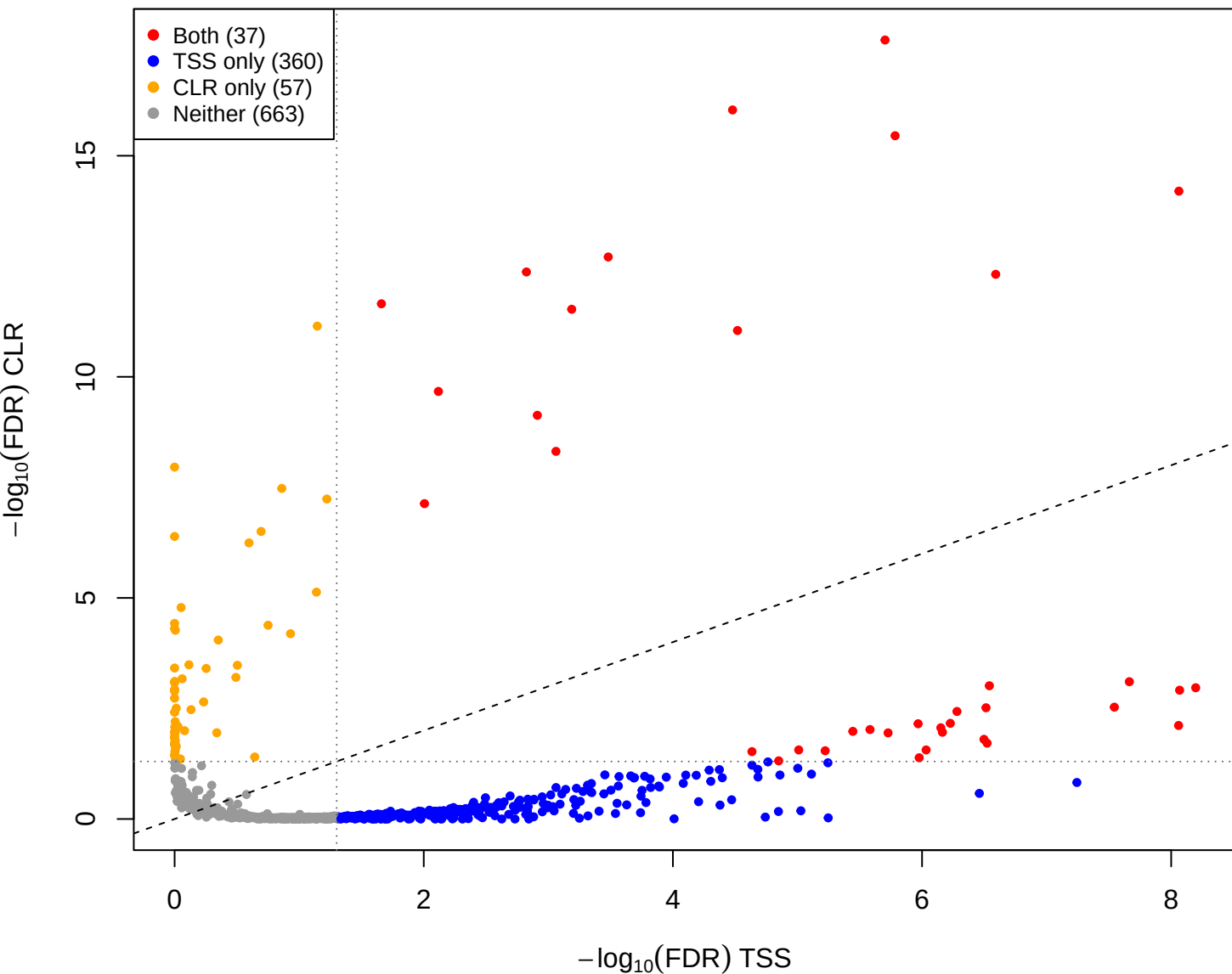
eld vs mage – CLR vs TSS(const=-1) (gamma = 0.001)
