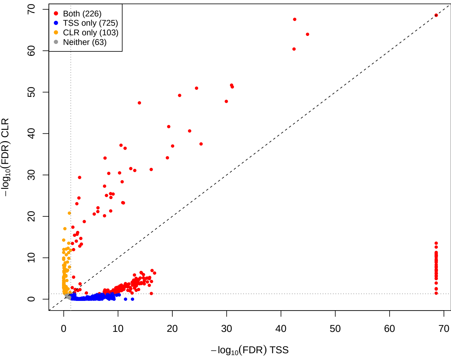
cent vs pup – CLR vs TSS(const=-1) (gamma = 0.001)
