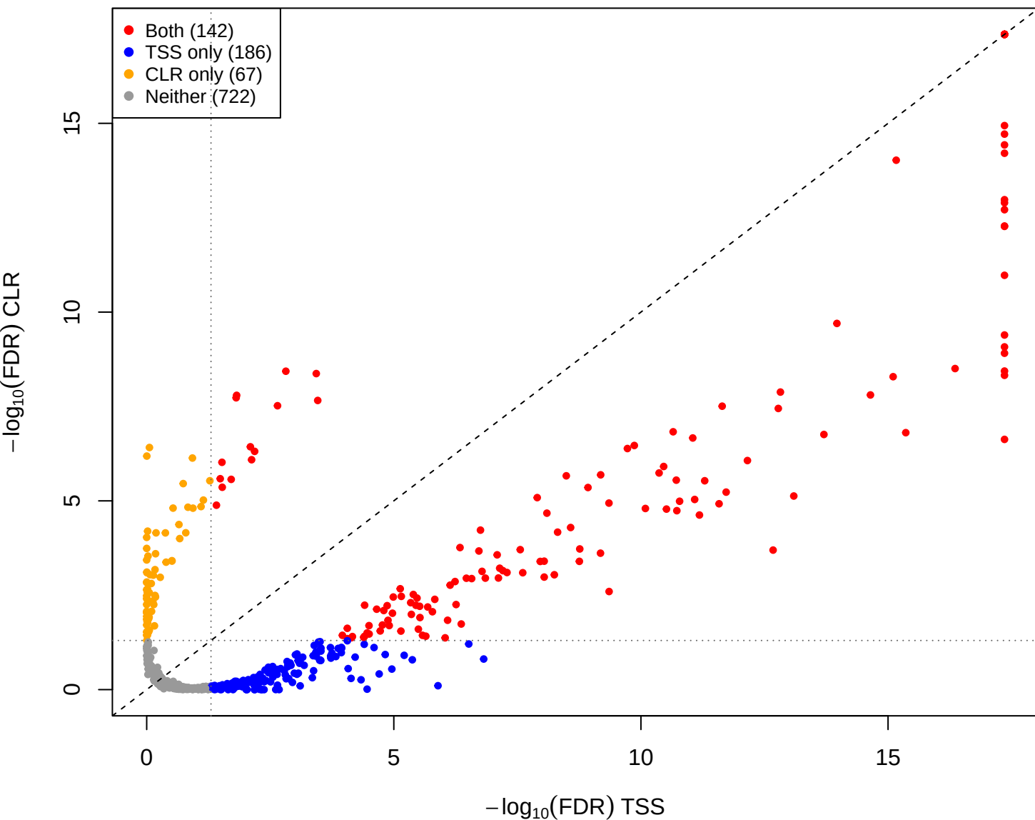
mage vs you – CLR vs TSS(const=-1) (gamma = 0.001)
