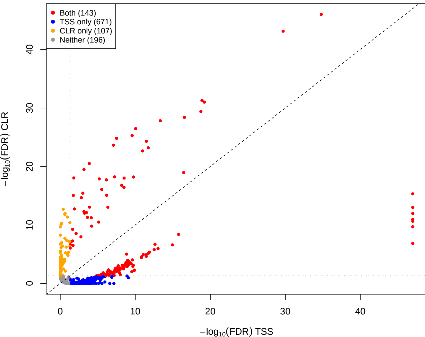
cent vs mid – CLR vs TSS(const=-1) (gamma = 0.001)
