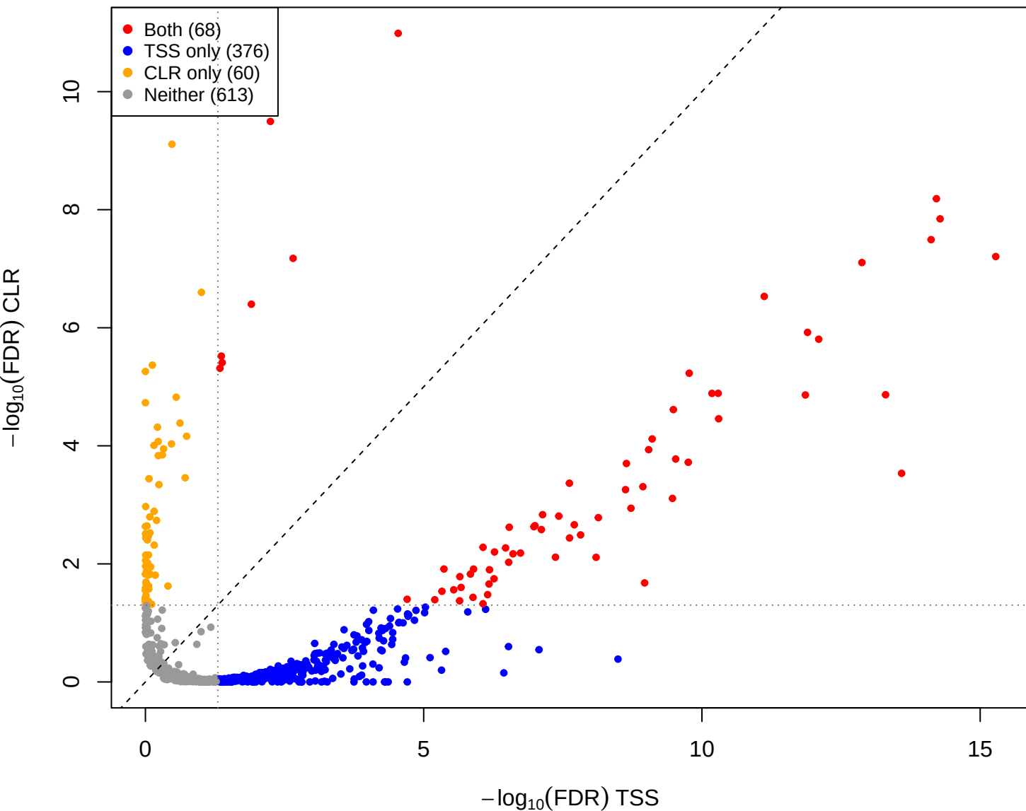
cent vs eld – CLR vs TSS(const=-1) (gamma = 0.001)
