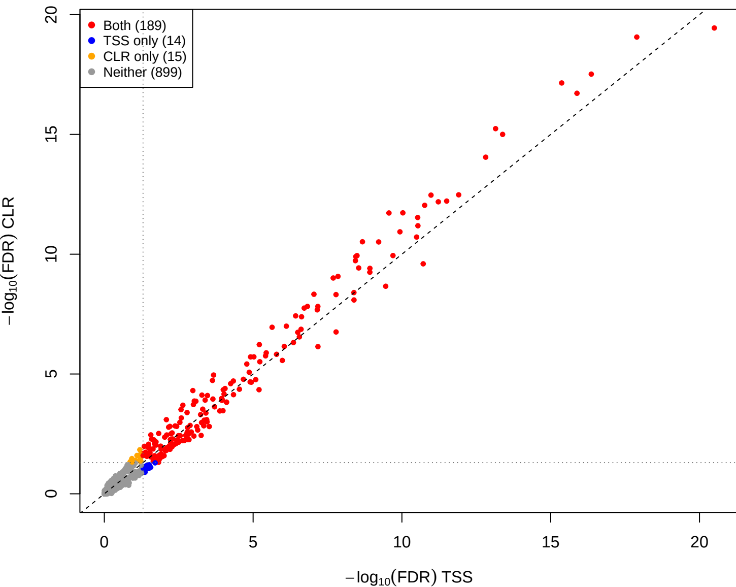
cent vs mage – CLR vs TSS(const=0.2) (gamma = 0.001)
