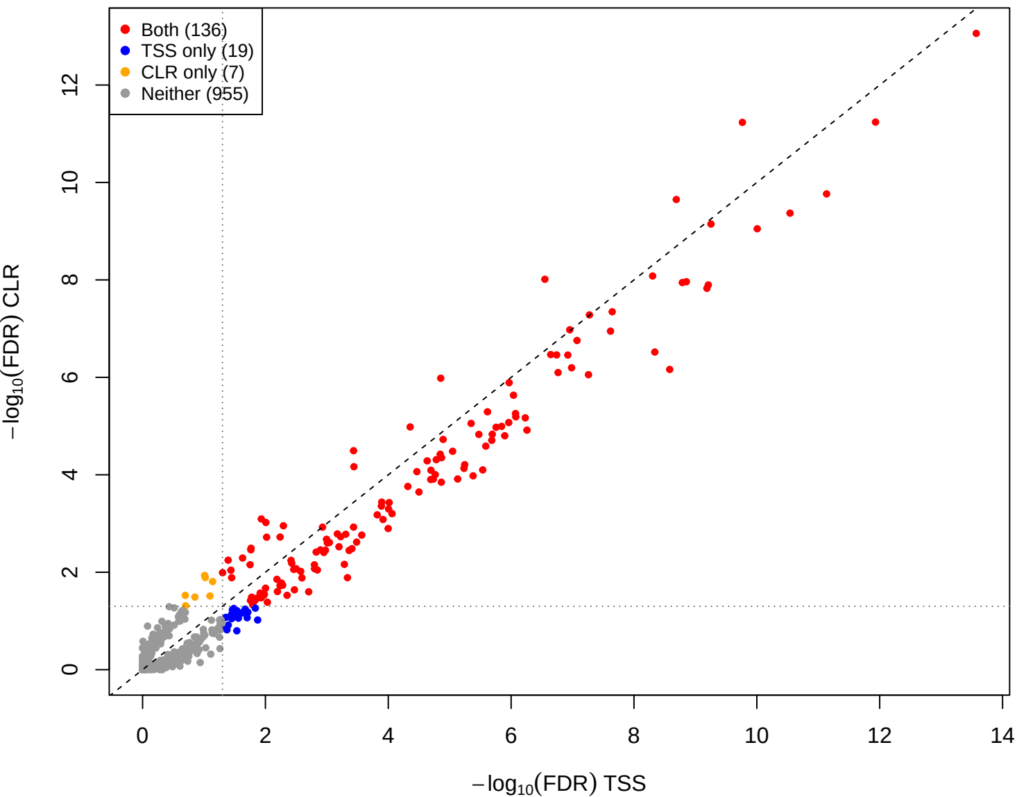
kin vs mid – CLR vs TSS(const=0.2) (gamma = 0.001)
