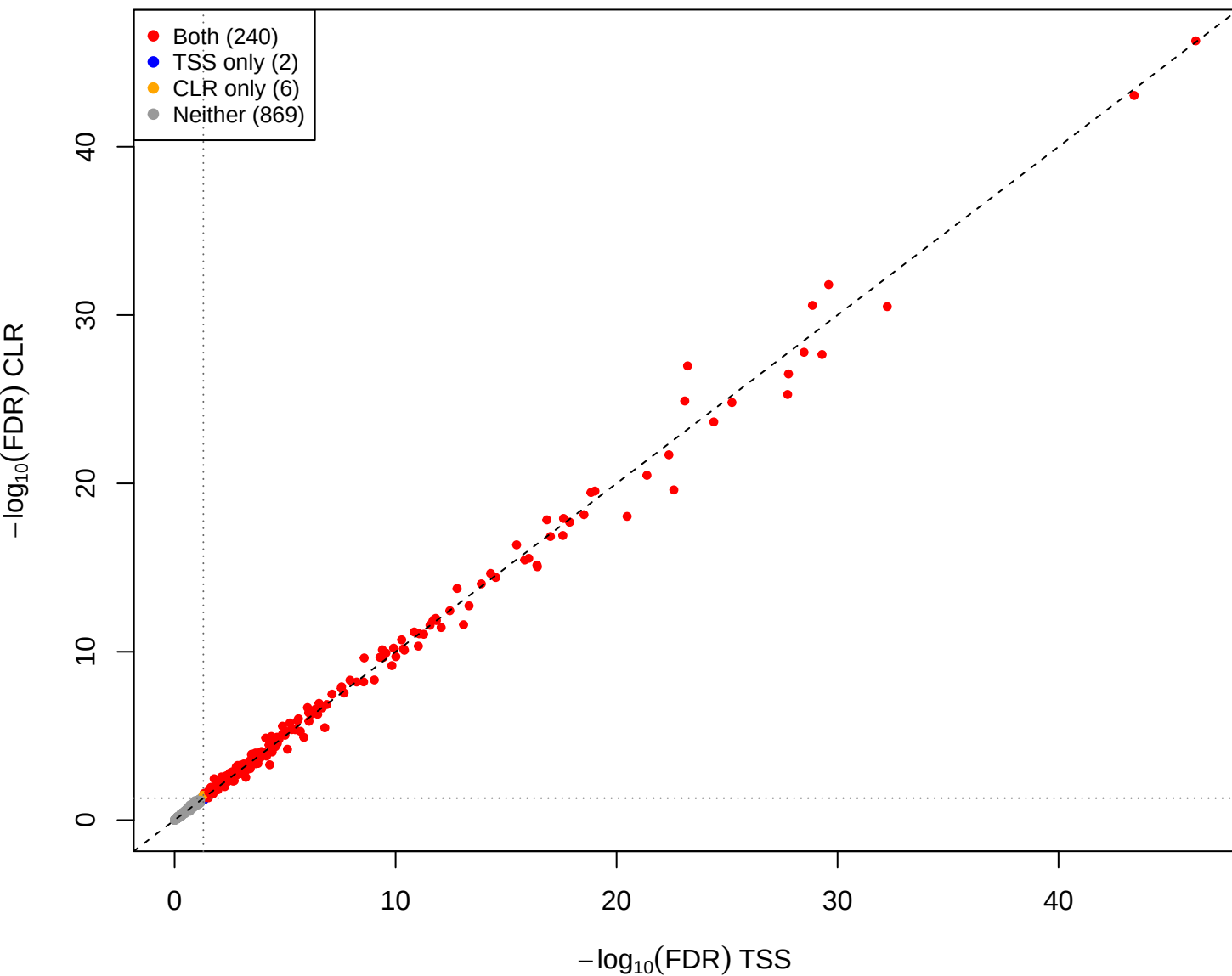
cent vs mid – CLR vs TSS(const=0.2) (gamma = 0.001)
