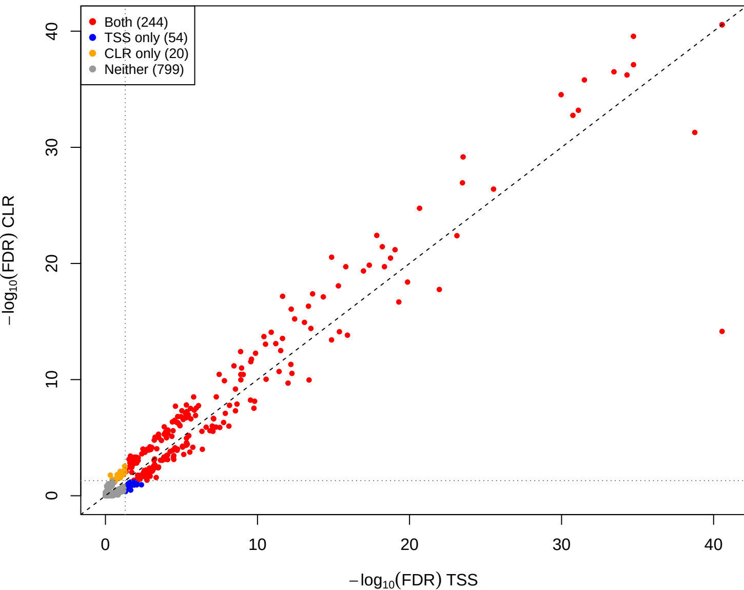
eld vs pup – CLR vs TSS(const=0.2) (gamma = 0.001)
