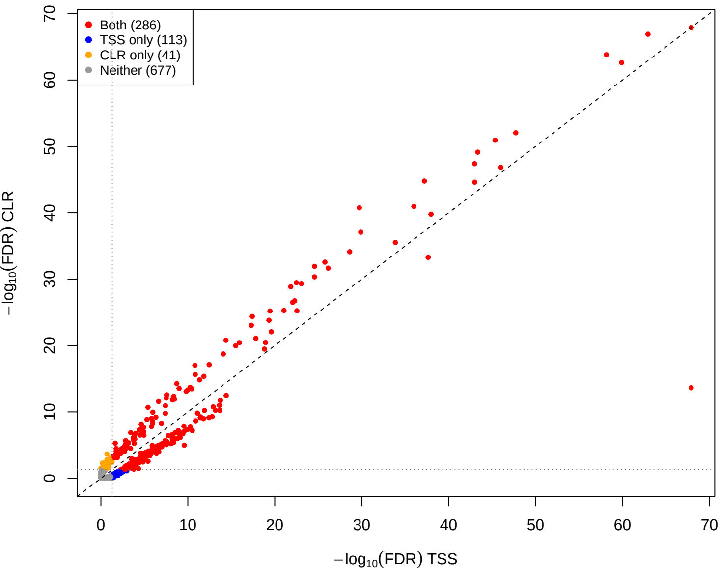
cent vs pup – CLR vs TSS(const=0.2) (gamma = 0.001)
