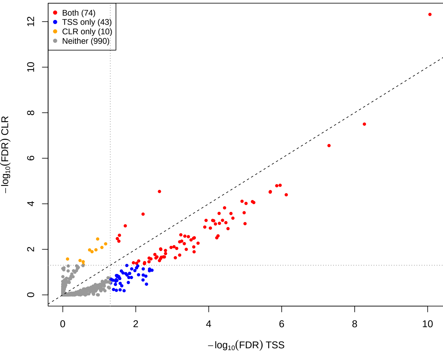
mage vs mid – CLR vs TSS(const=0.2) (gamma = 0.001)
