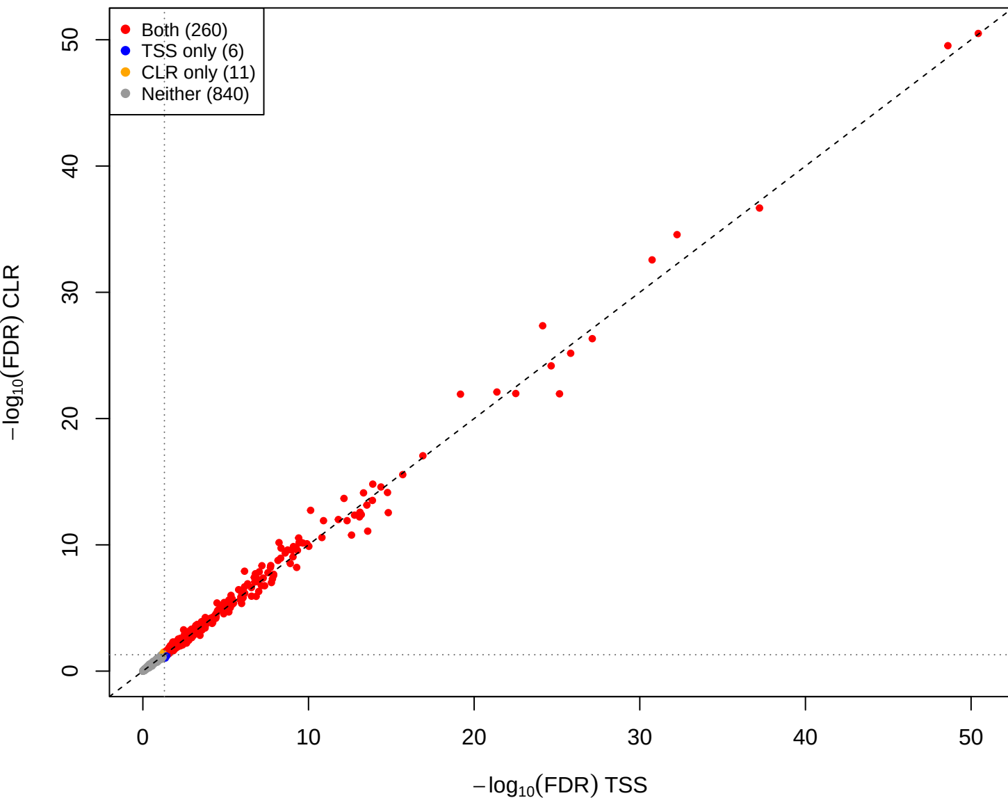
cent vs kin – CLR vs TSS(const=0.2) (gamma = 0.001)
