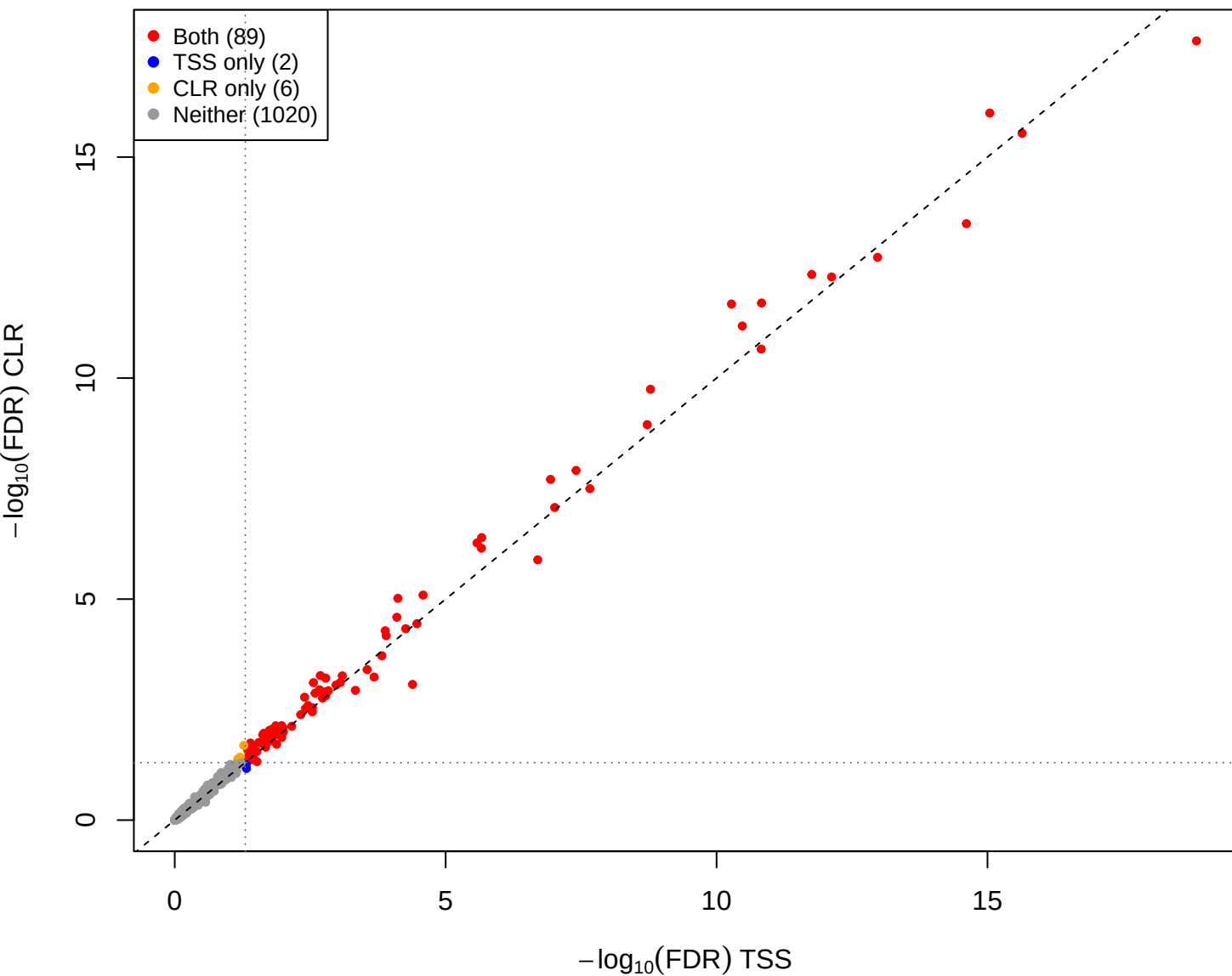
eld vs mage – CLR vs TSS(const=0.2) (gamma = 0.001)
