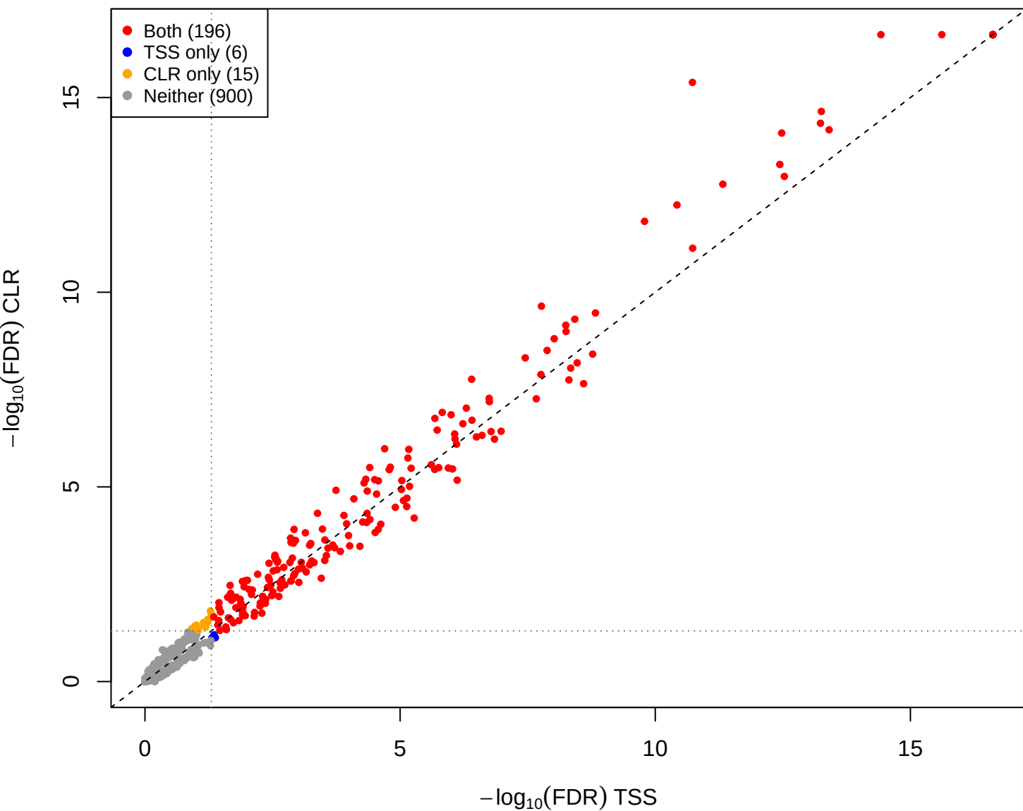
mage vs you – CLR vs TSS(const=0.2) (gamma = 0.001)
