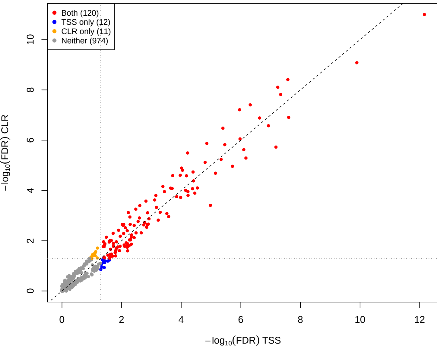
cent vs eld – CLR vs TSS(const=0.2) (gamma = 0.001)
