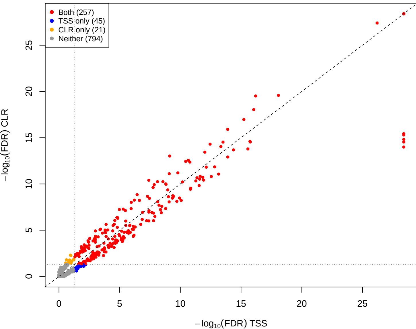
cent vs you – CLR vs TSS(const=0.2) (gamma = 0.001)
