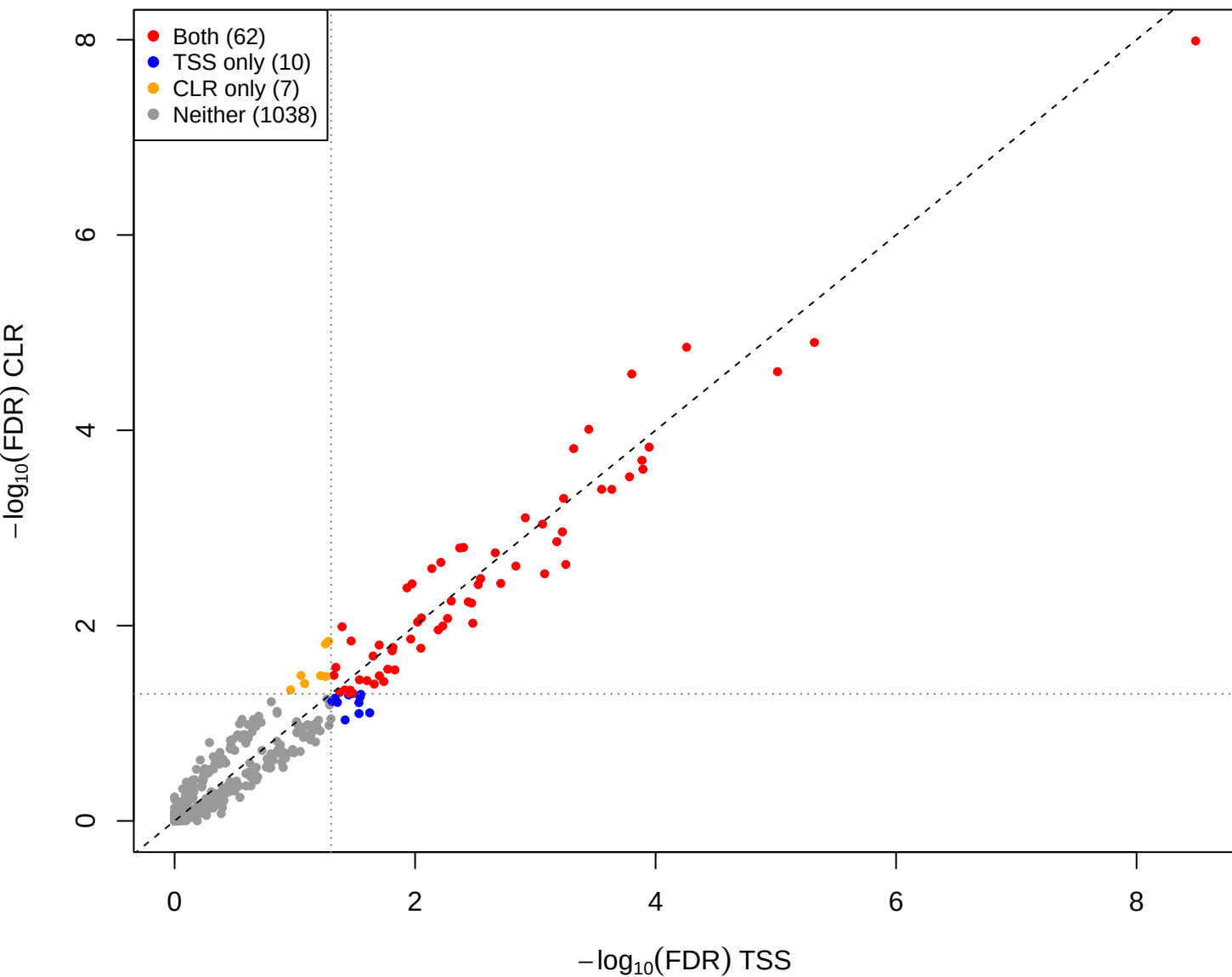
eld vs you – CLR vs TSS(const=0.2) (gamma = 0.001)
