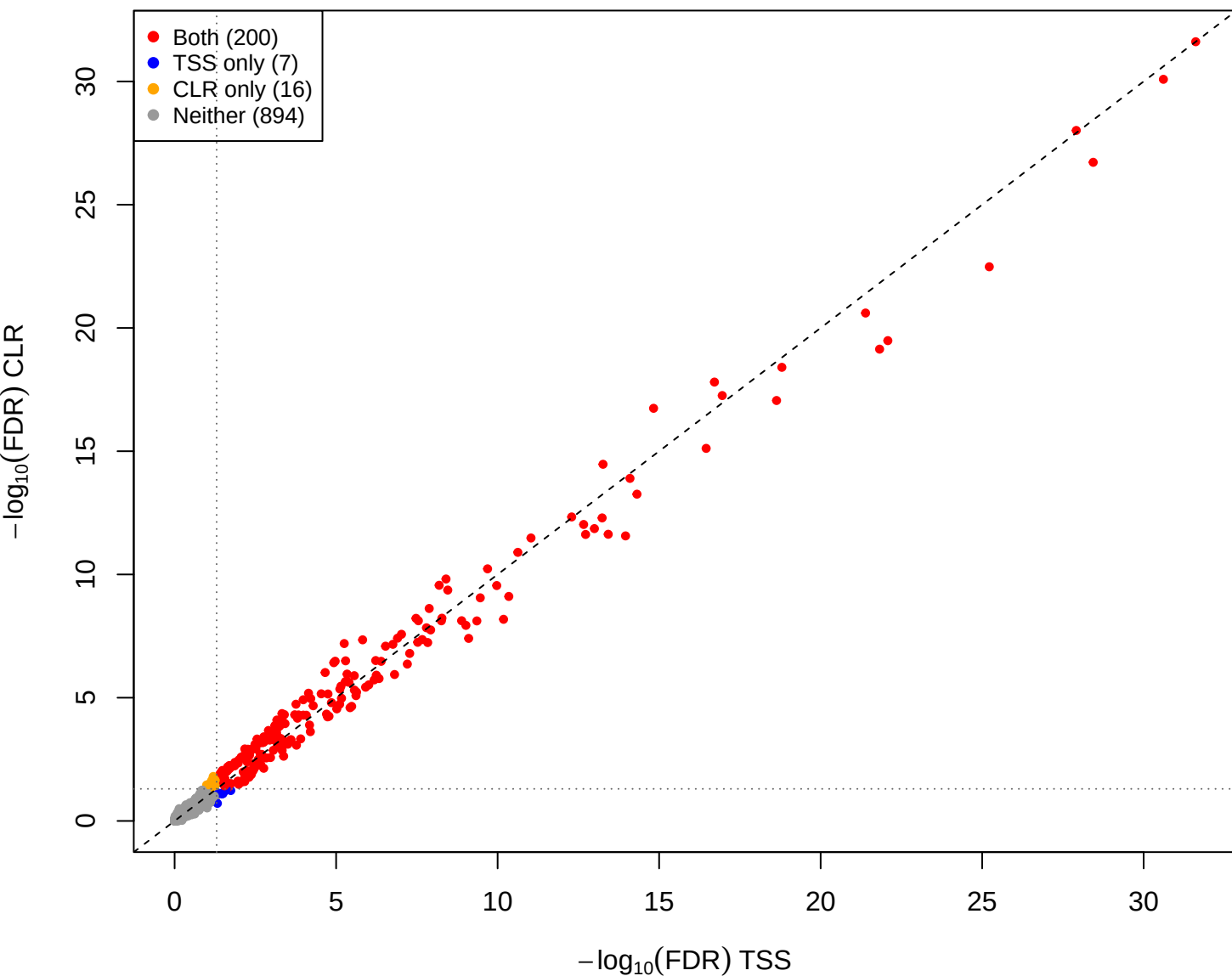
eld vs kin – CLR vs TSS(const=0.2) (gamma = 0.001)
