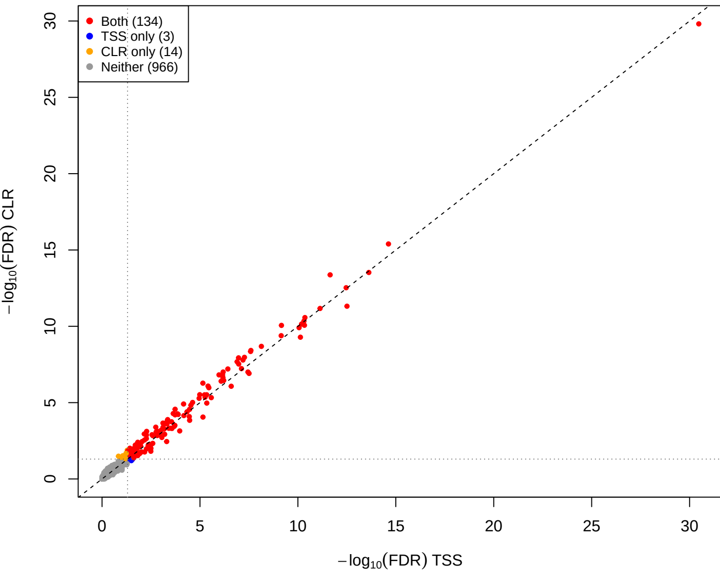
mage vs pup – CLR vs TSS(const=0.2) (gamma = 0.001)
