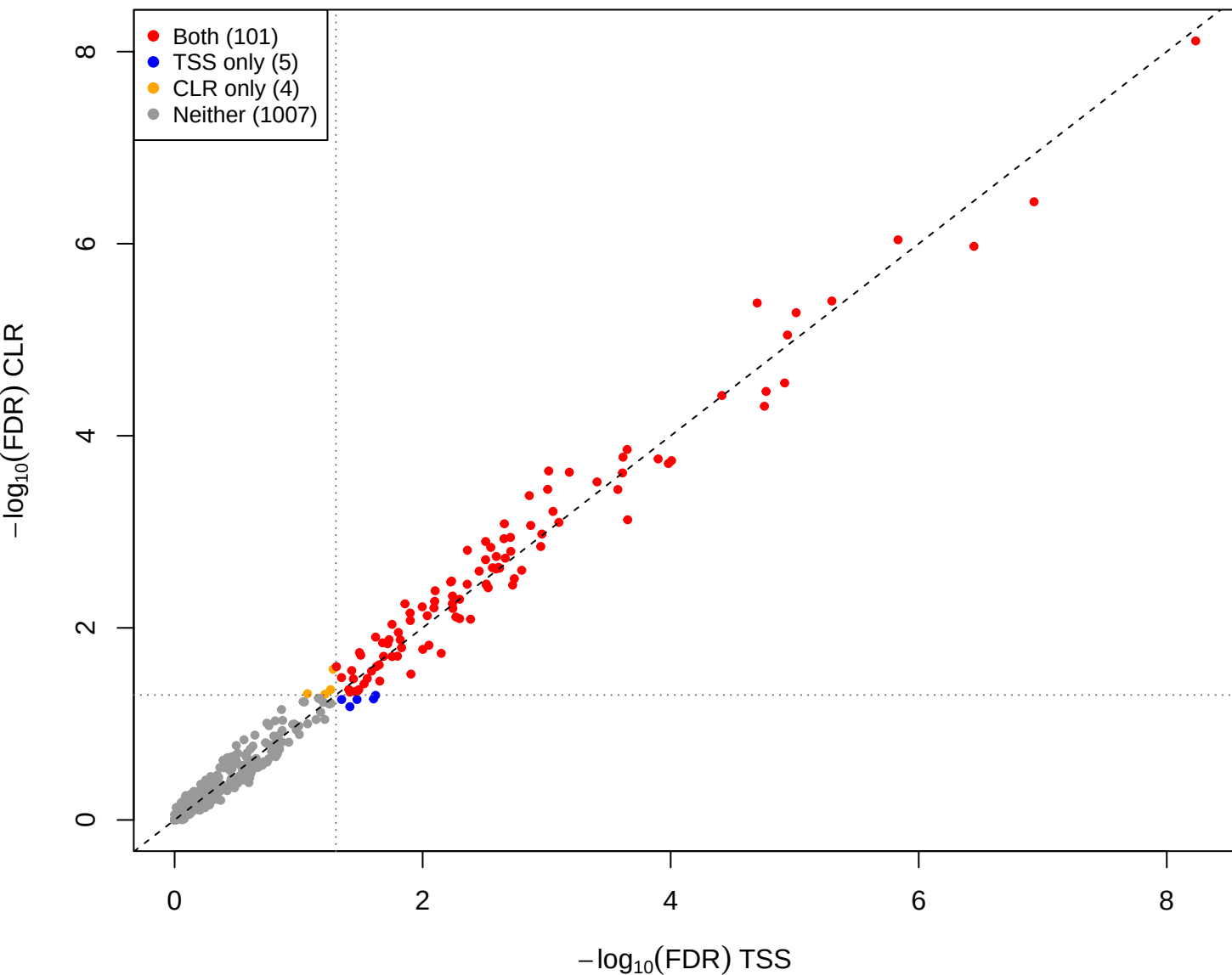
kin vs mage – CLR vs TSS(const=0.2) (gamma = 0.001)
