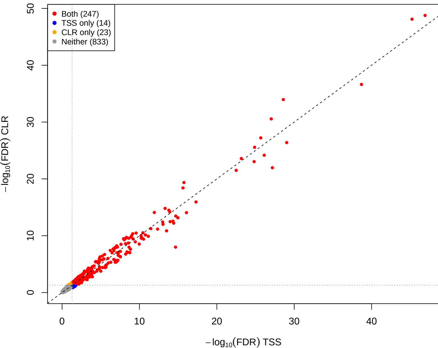
cent vs kin – CLR vs TSS(const=0.3) (gamma = 0.001)
