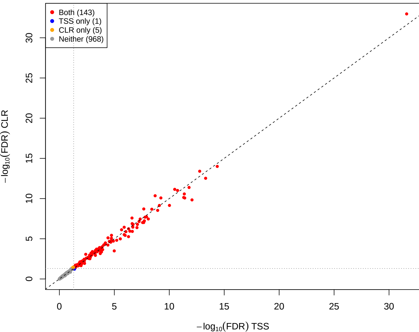
mage vs pup – CLR vs TSS(const=0.3) (gamma = 0.001)
