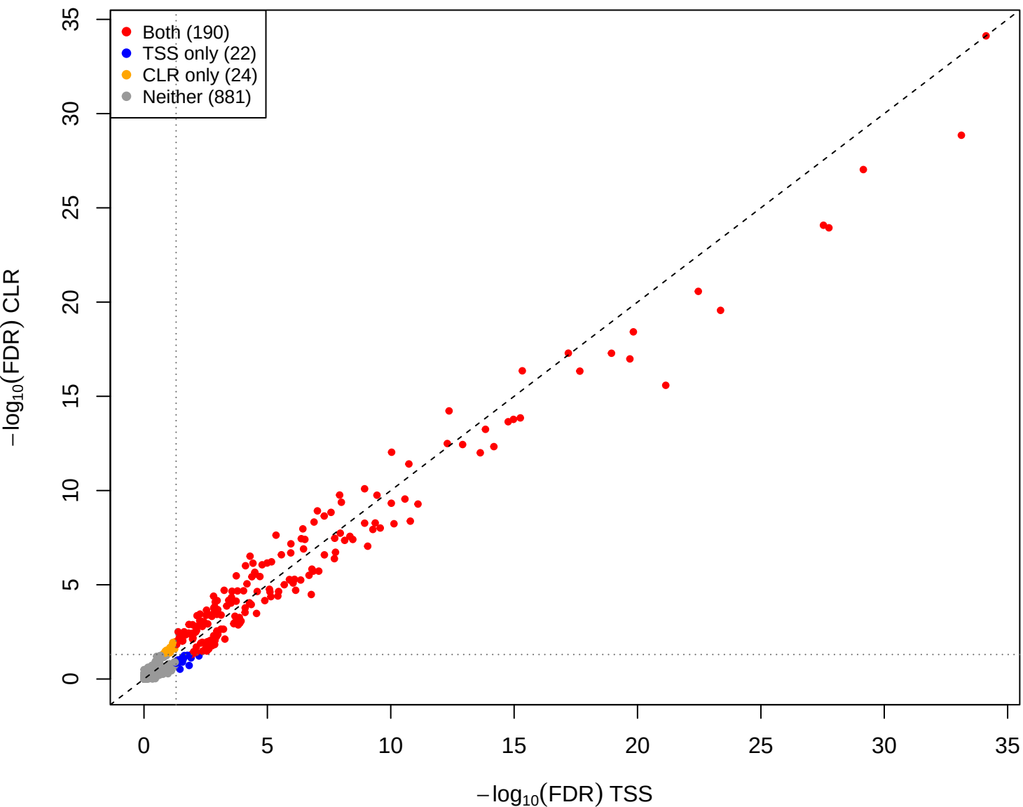
eld vs kin – CLR vs TSS(const=0.3) (gamma = 0.001)
