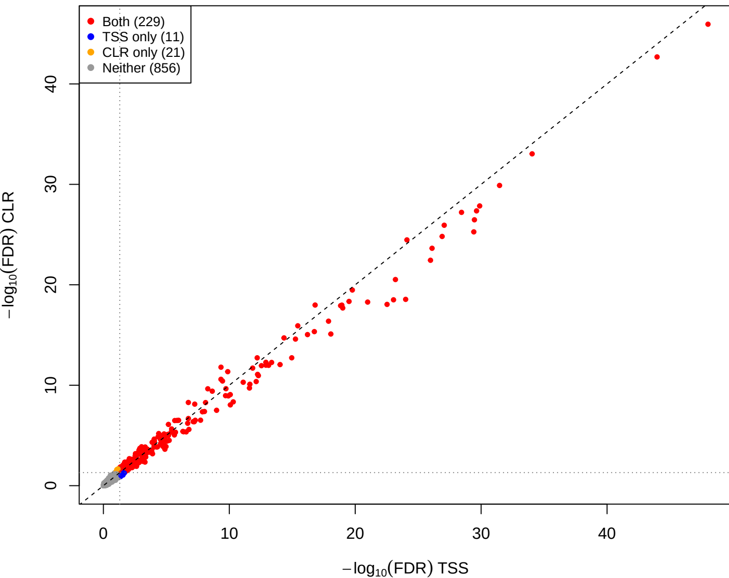
cent vs mid – CLR vs TSS(const=0.3) (gamma = 0.001)
