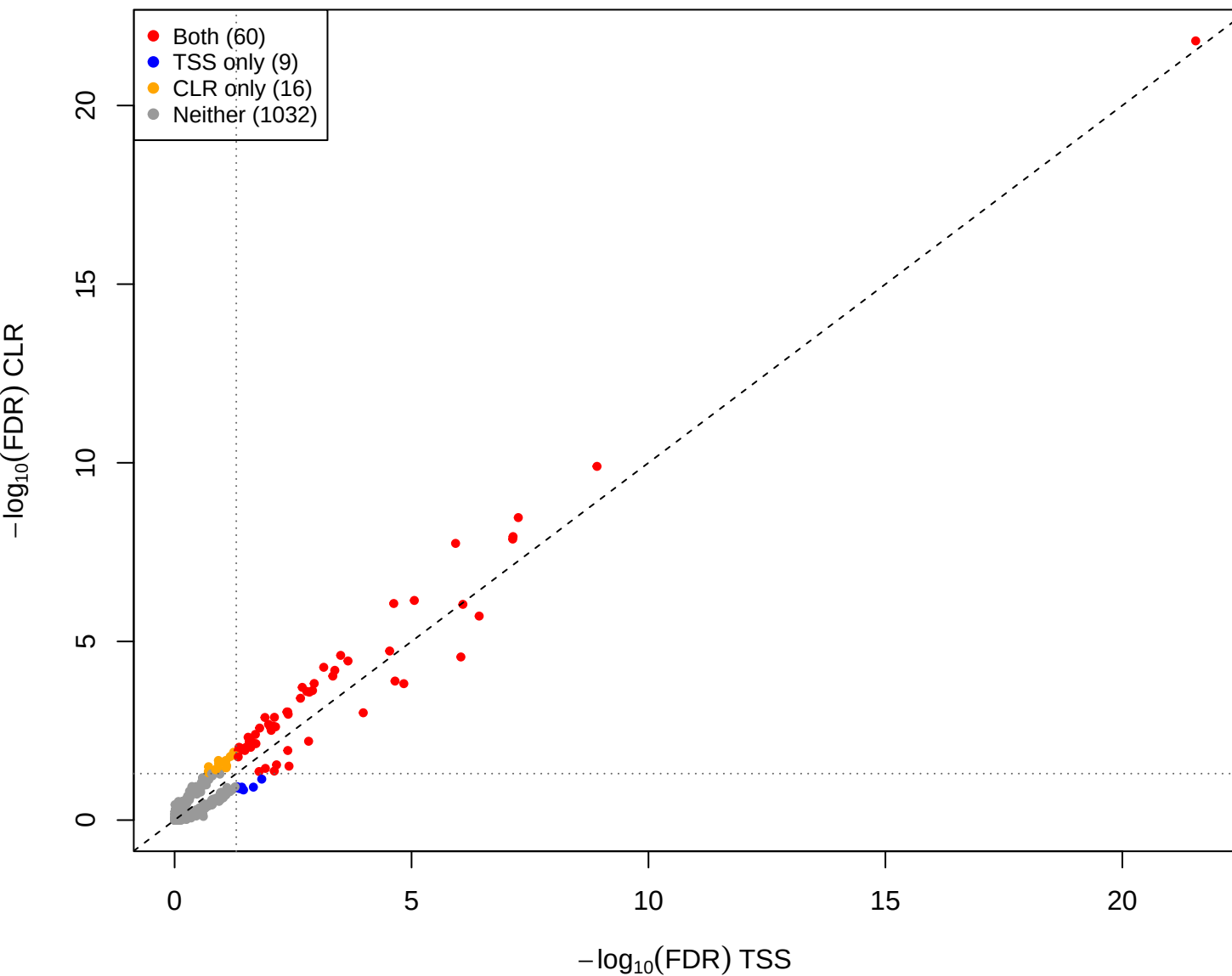
kin vs pup – CLR vs TSS(const=0.3) (gamma = 0.001)
