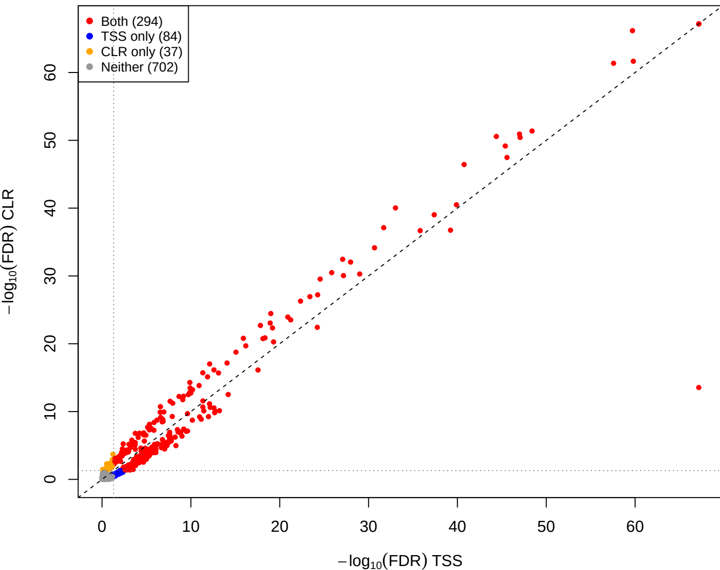
cent vs pup – CLR vs TSS(const=0.3) (gamma = 0.001)
