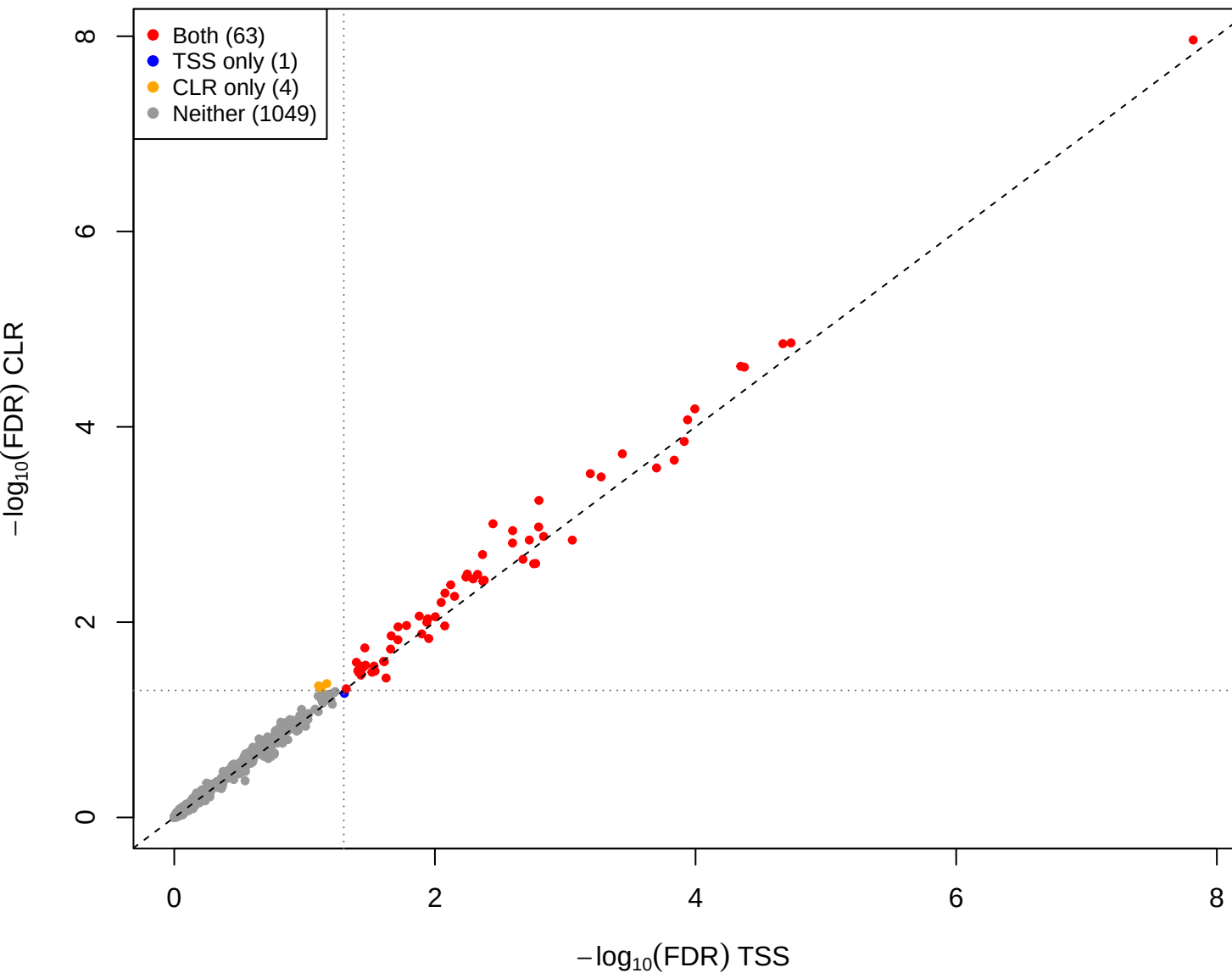
eld vs you – CLR vs TSS(const=0.3) (gamma = 0.001)
