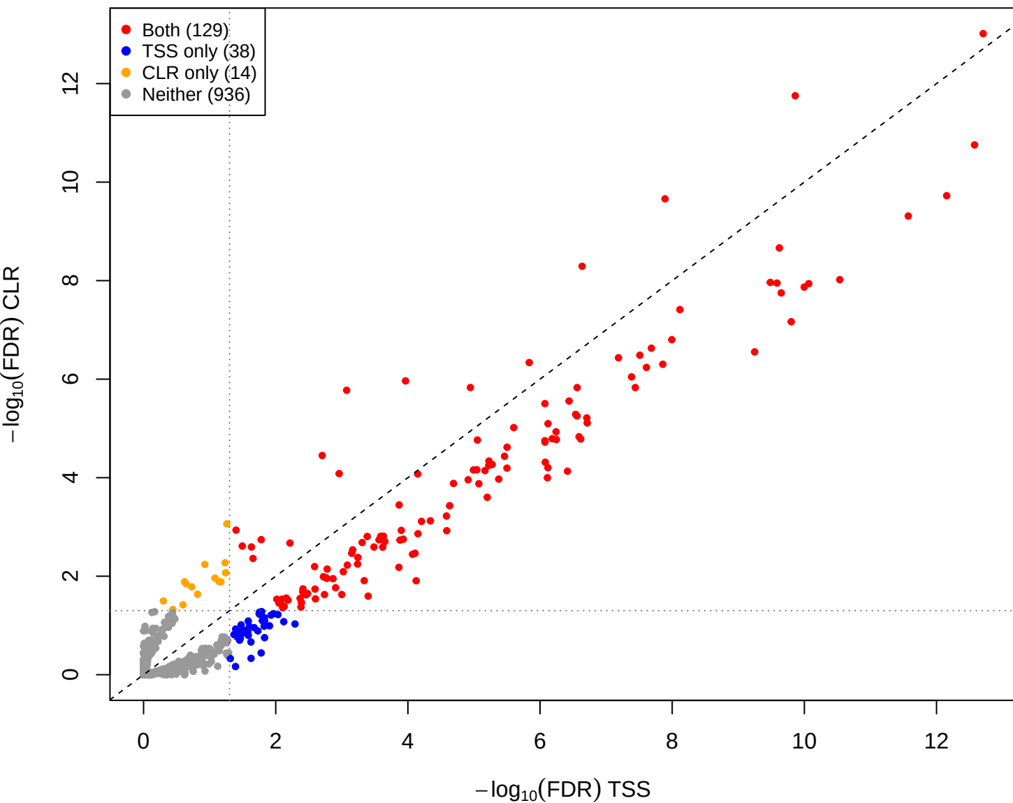
kin vs mid – CLR vs TSS(const=0.3) (gamma = 0.001)
