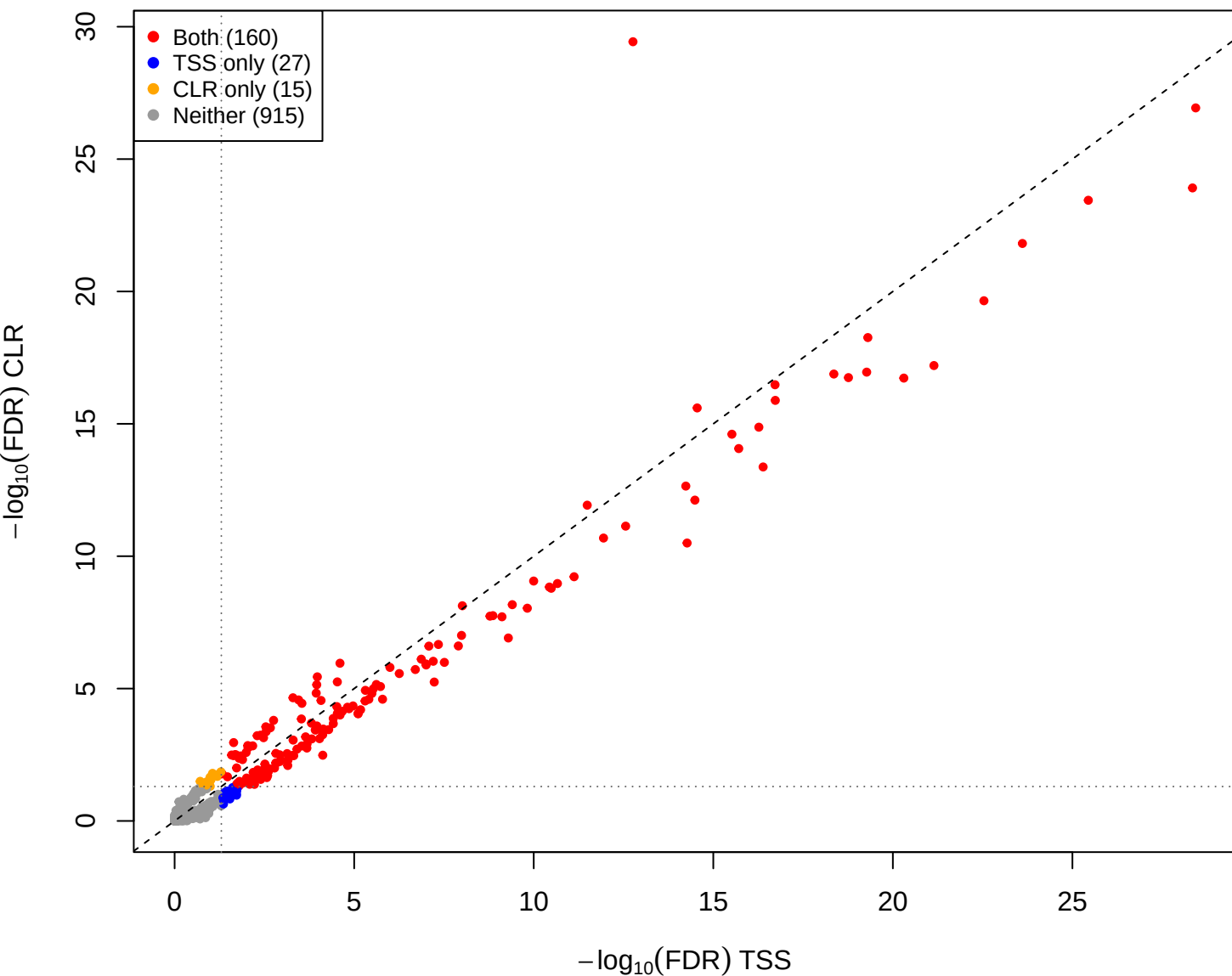
eld vs mid – CLR vs TSS(const=0.3) (gamma = 0.001)
