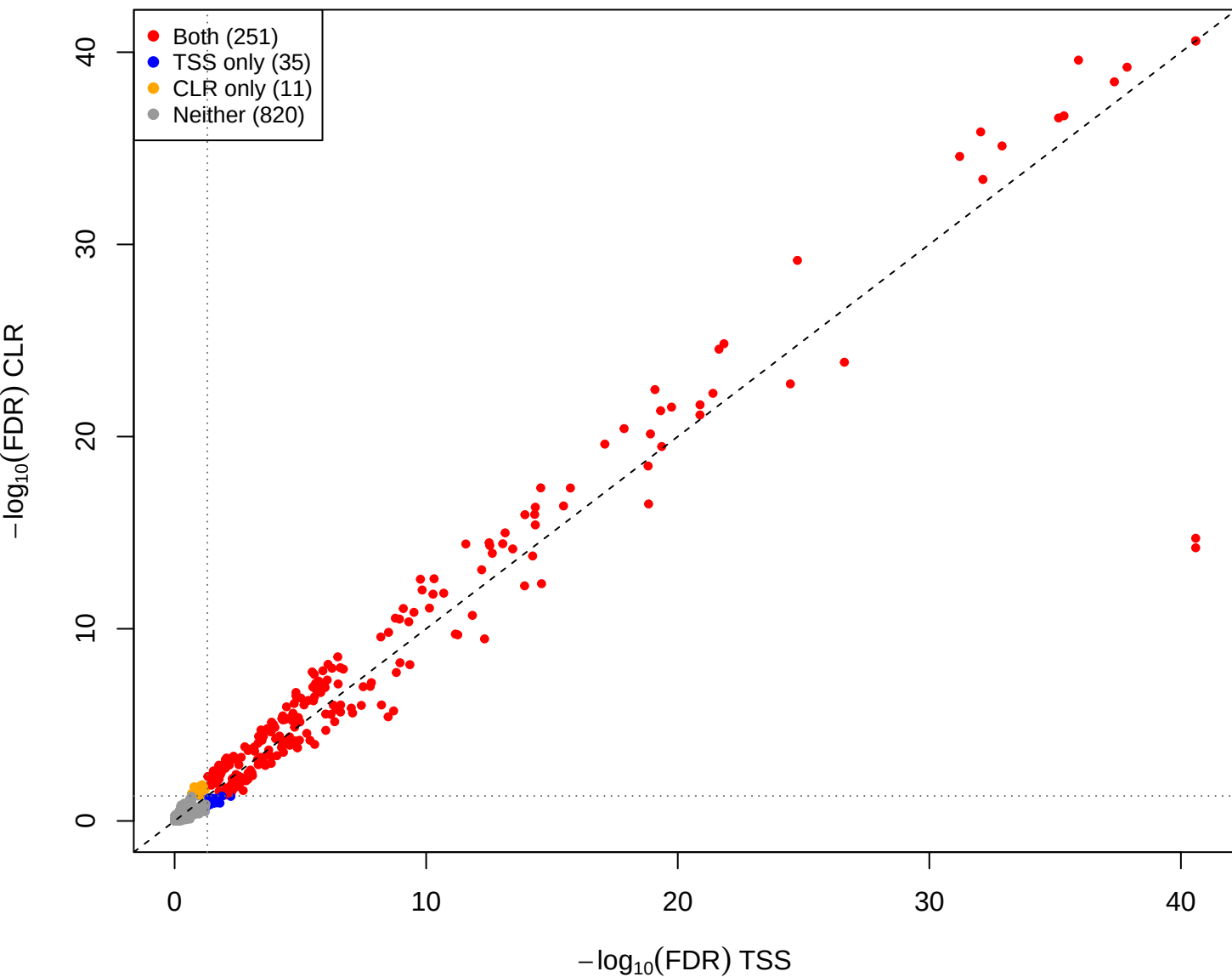
eld vs pup – CLR vs TSS(const=0.3) (gamma = 0.001)
