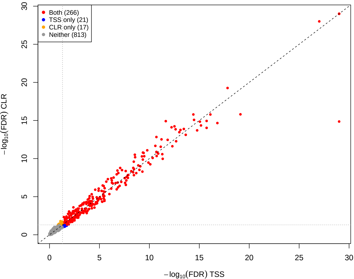
cent vs you – CLR vs TSS(const=0.3) (gamma = 0.001)
