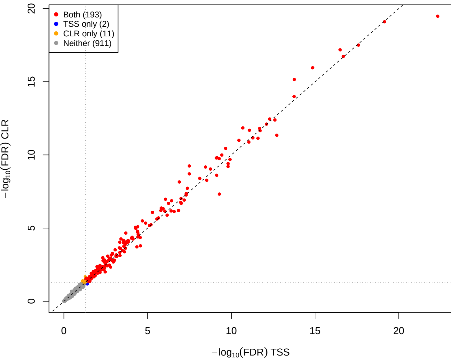
cent vs mage – CLR vs TSS(const=0.3) (gamma = 0.001)
