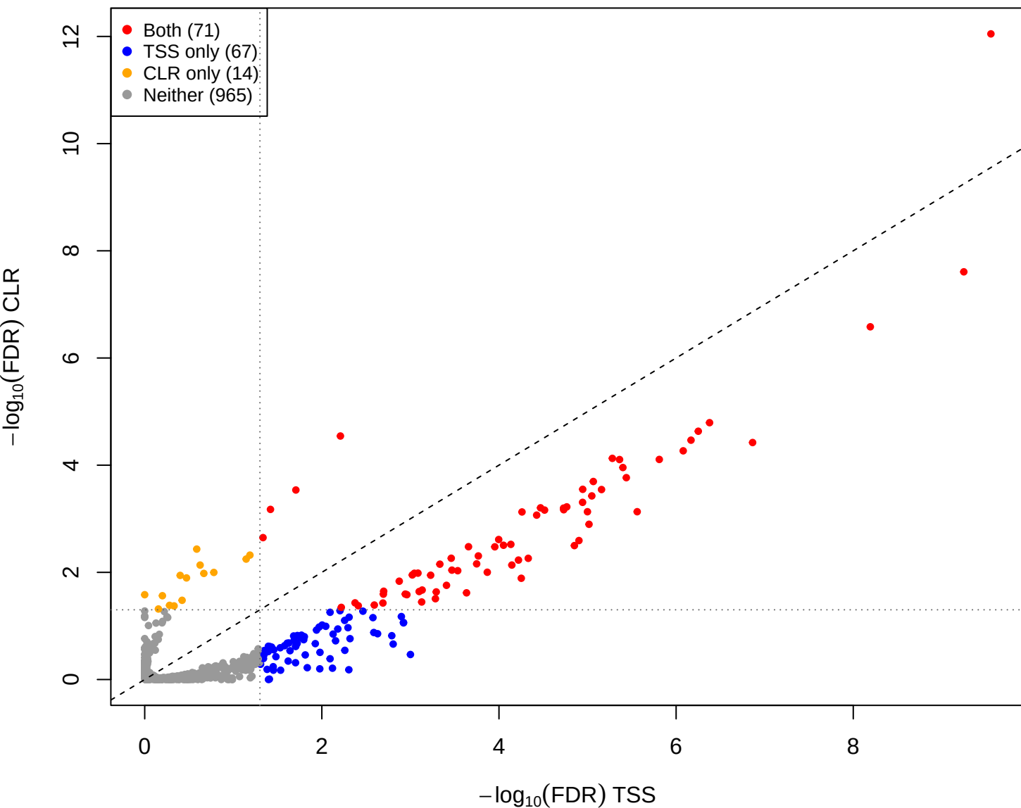
mage vs mid – CLR vs TSS(const=0.3) (gamma = 0.001)
