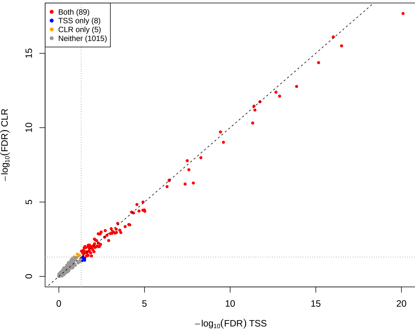
eld vs mage - CLR vs TSS(const=0.3) (gamma = 0.001)
