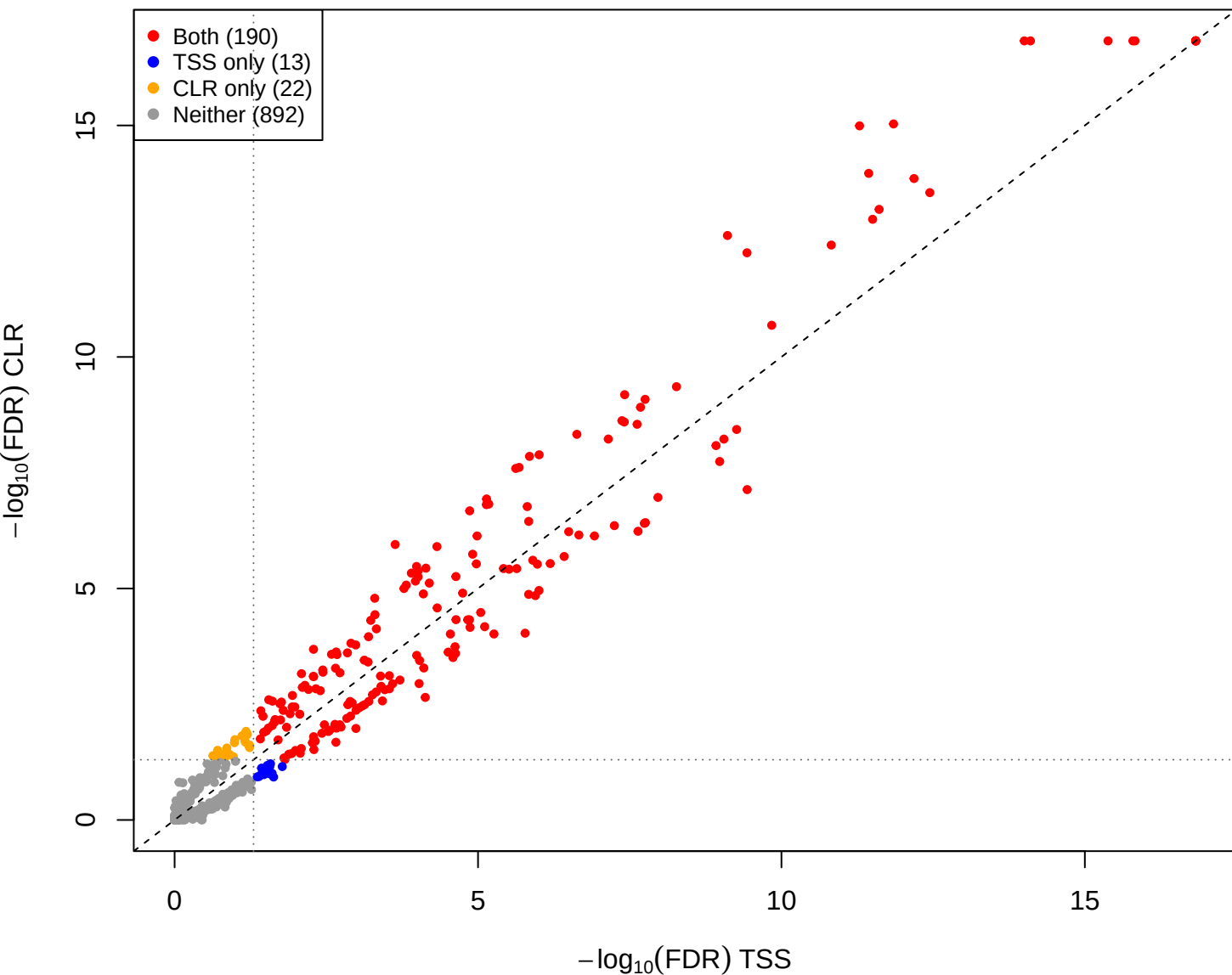
mage vs you – CLR vs TSS(const=0.3) (gamma = 0.001)
