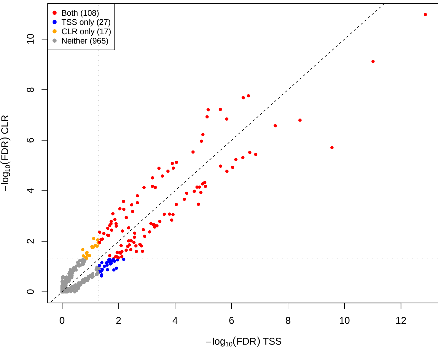
cent vs eld – CLR vs TSS(const=0.3) (gamma = 0.001)
