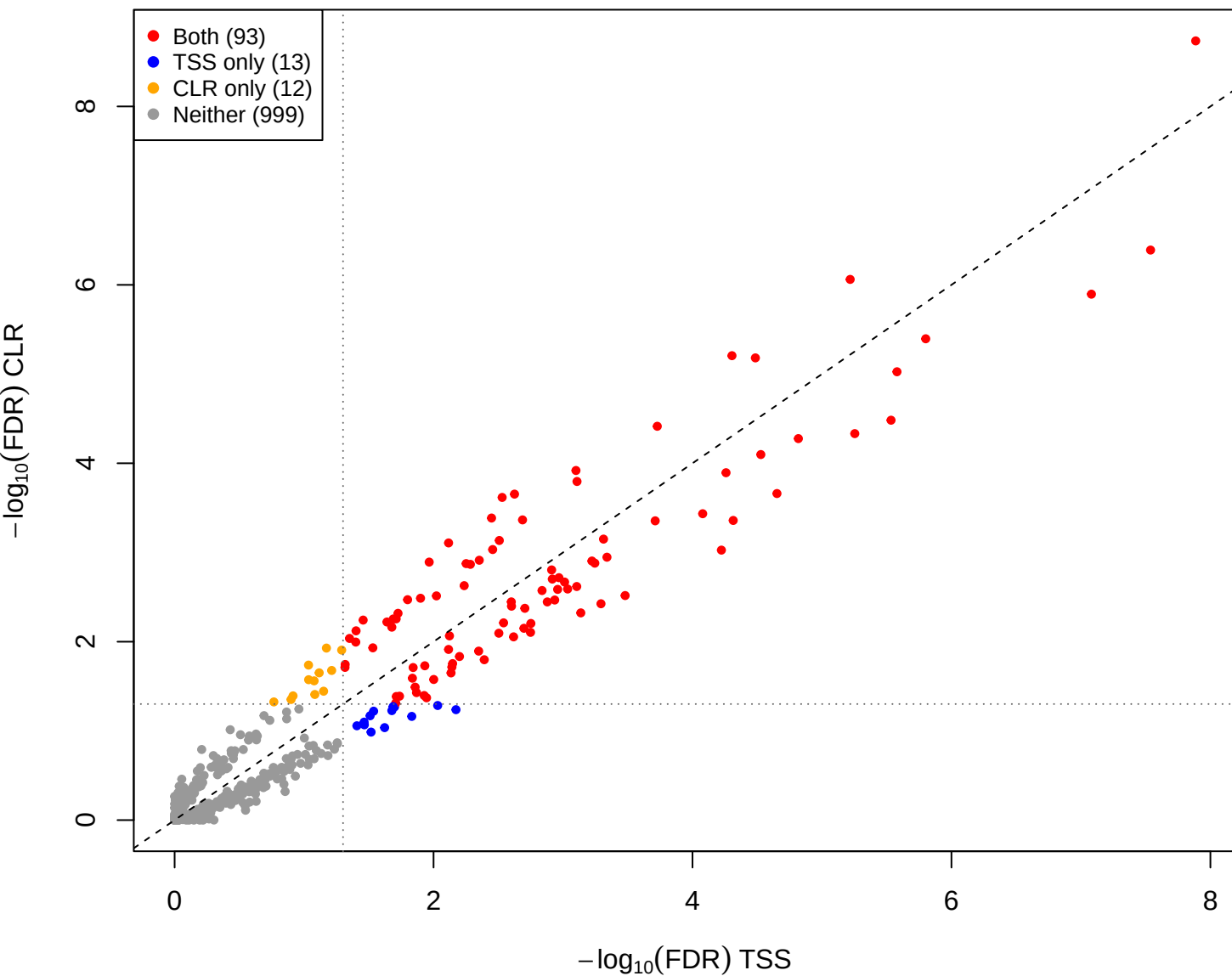
kin vs mage – CLR vs TSS(const=0.3) (gamma = 0.001)
