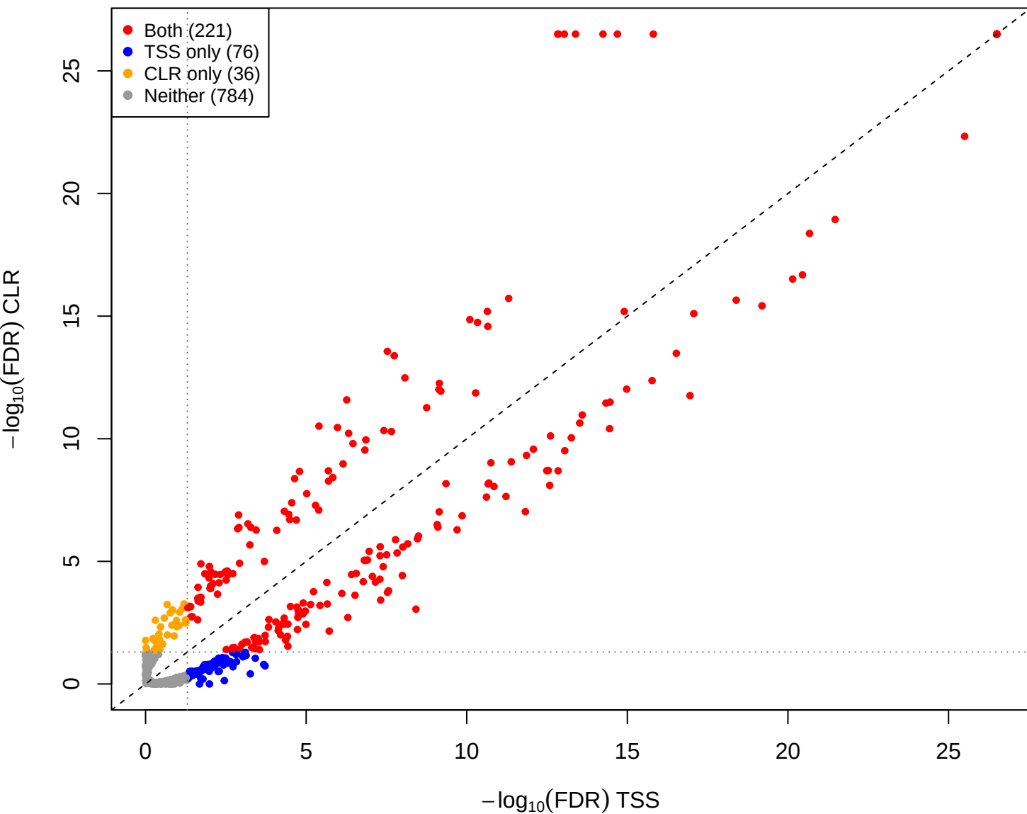
kin vs you – CLR vs TSS(const=0.8) (gamma = 0.001)
