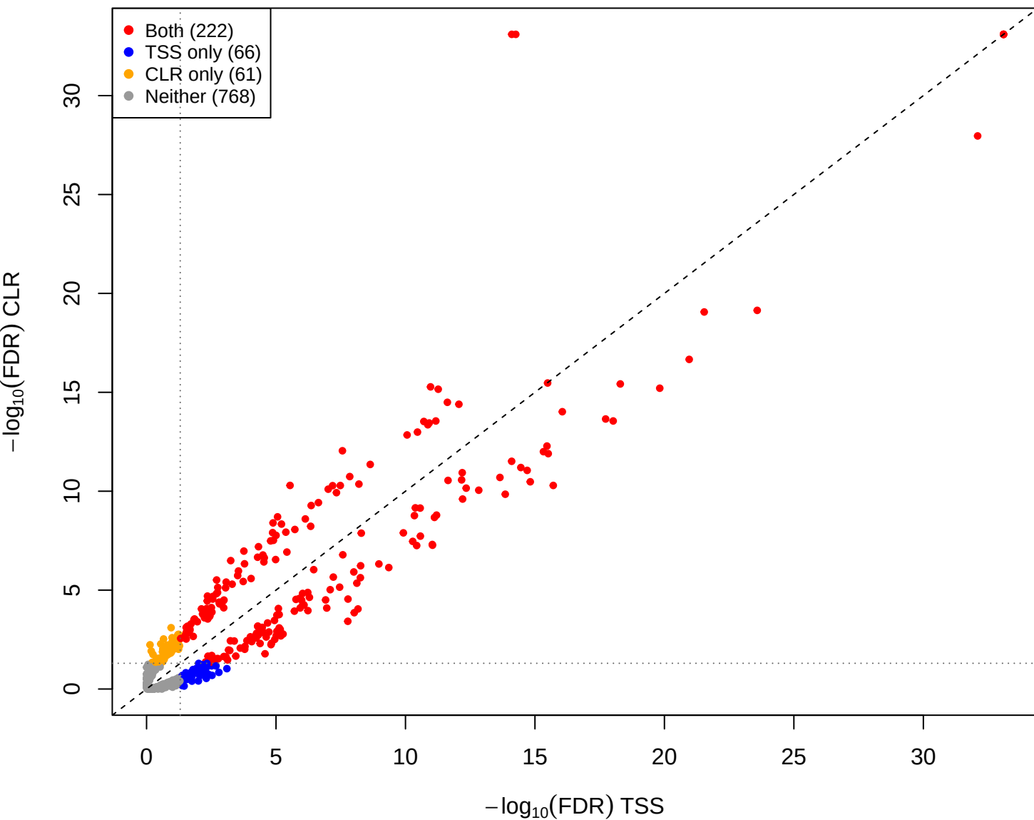
cent vs you – CLR vs TSS(const=0.8) (gamma = 0.001)
