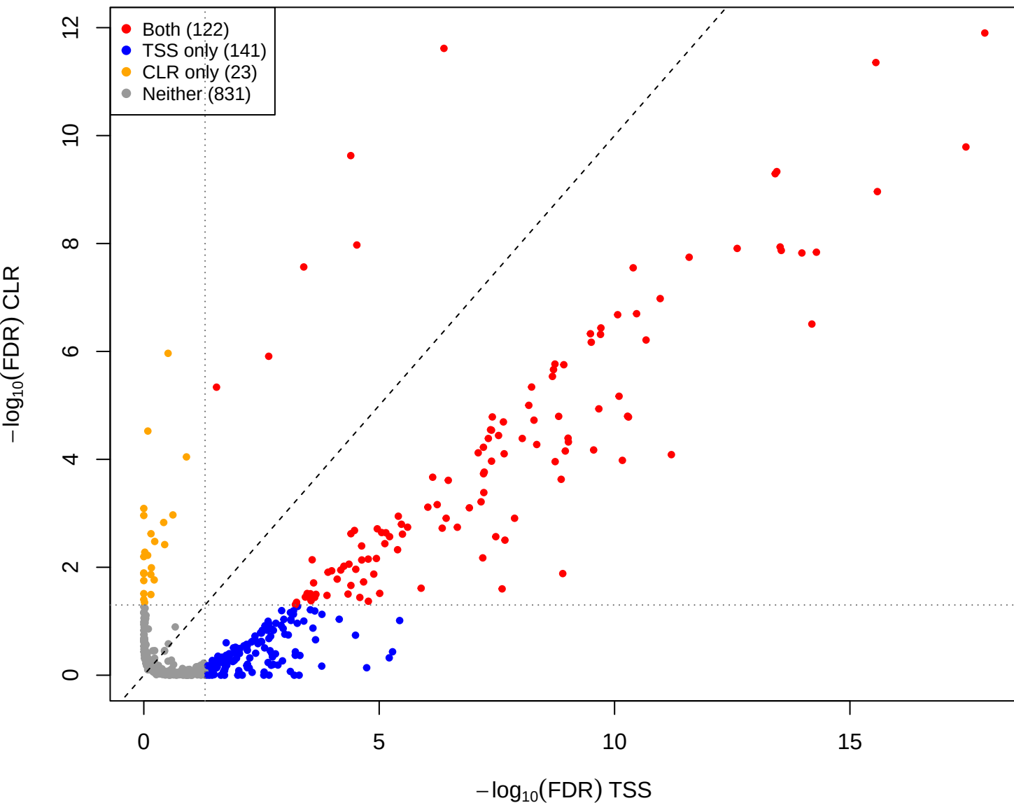
kin vs mid – CLR vs TSS(const=0.8) (gamma = 0.001)
