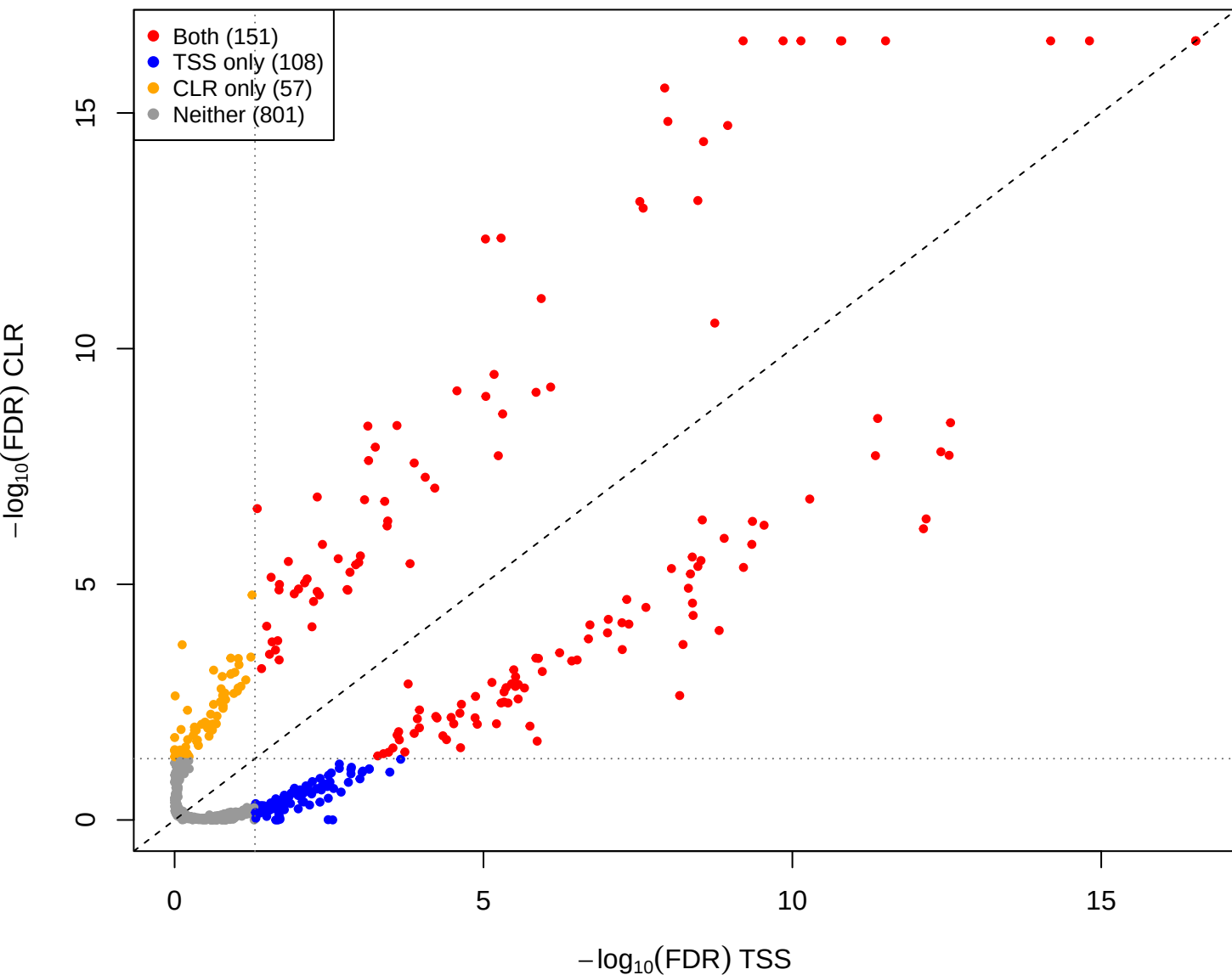
mage vs you – CLR vs TSS(const=0.8) (gamma = 0.001)
