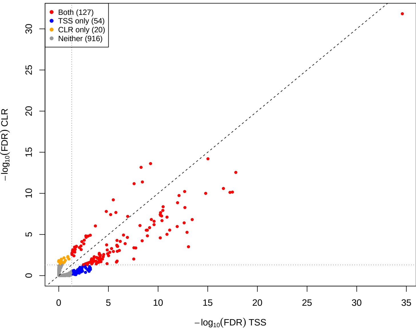
mage vs pup – CLR vs TSS(const=0.8) (gamma = 0.001)
