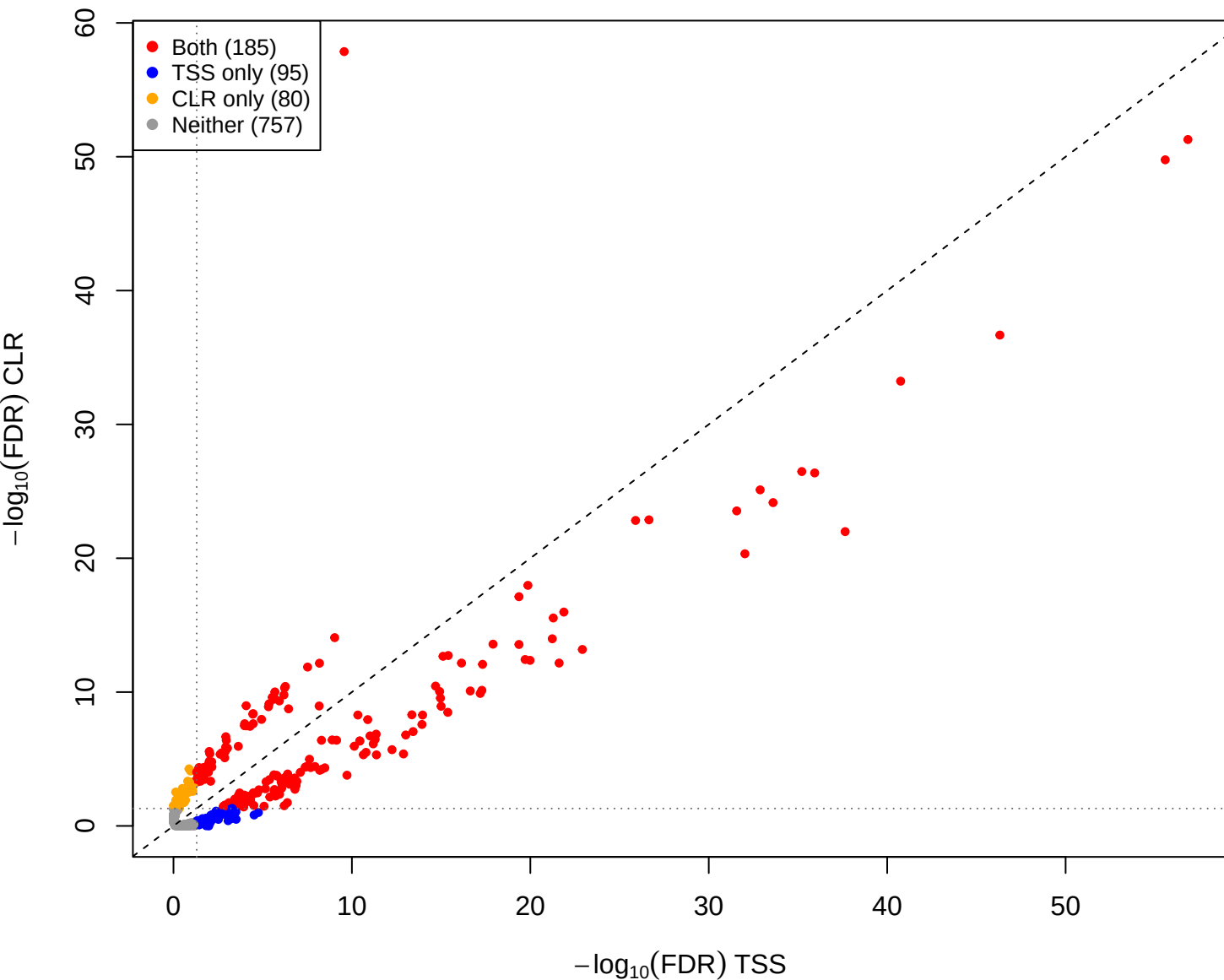
cent vs kin – CLR vs TSS(const=0.8) (gamma = 0.001)
