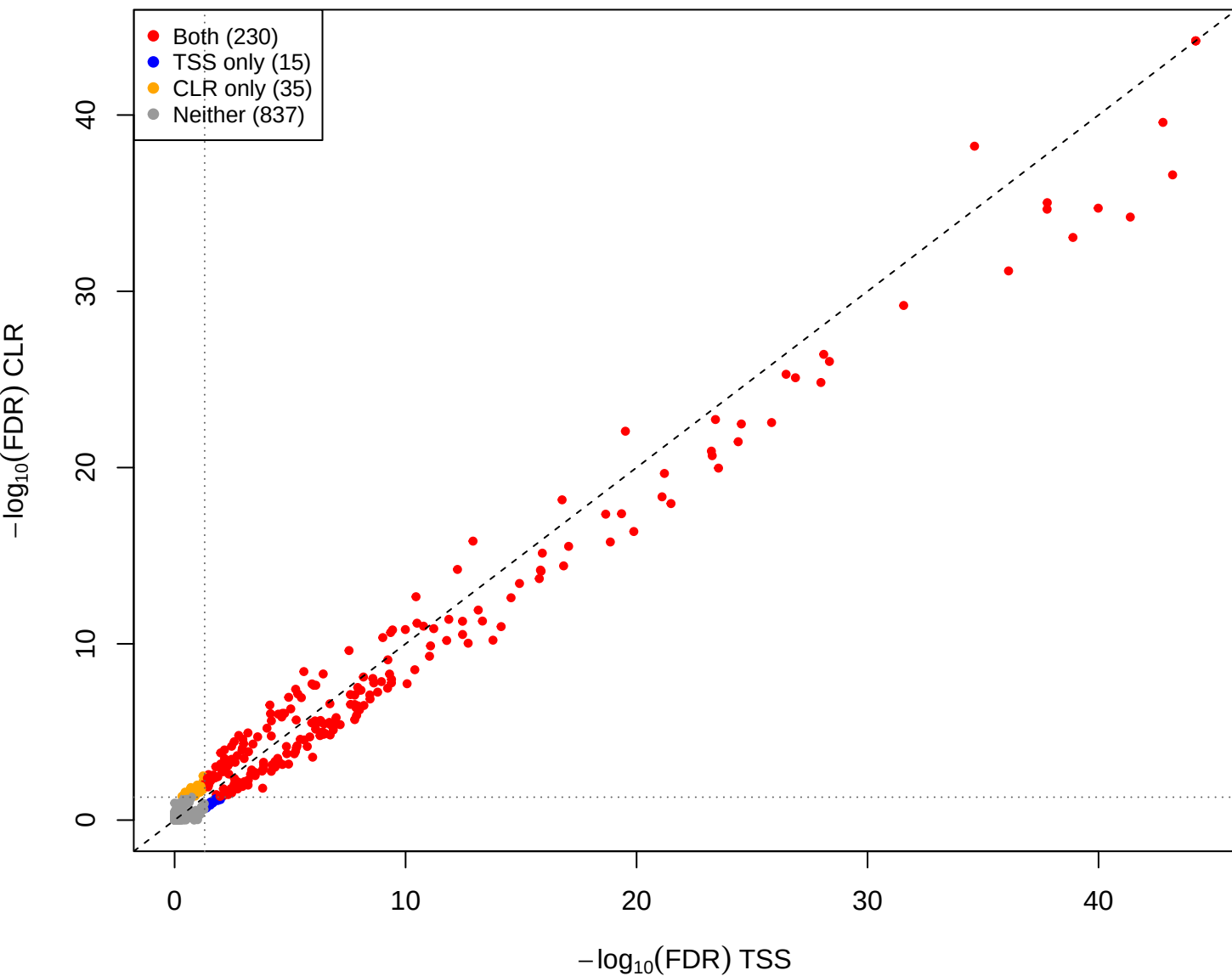
eld vs pup – CLR vs TSS(const=0.8) (gamma = 0.001)
