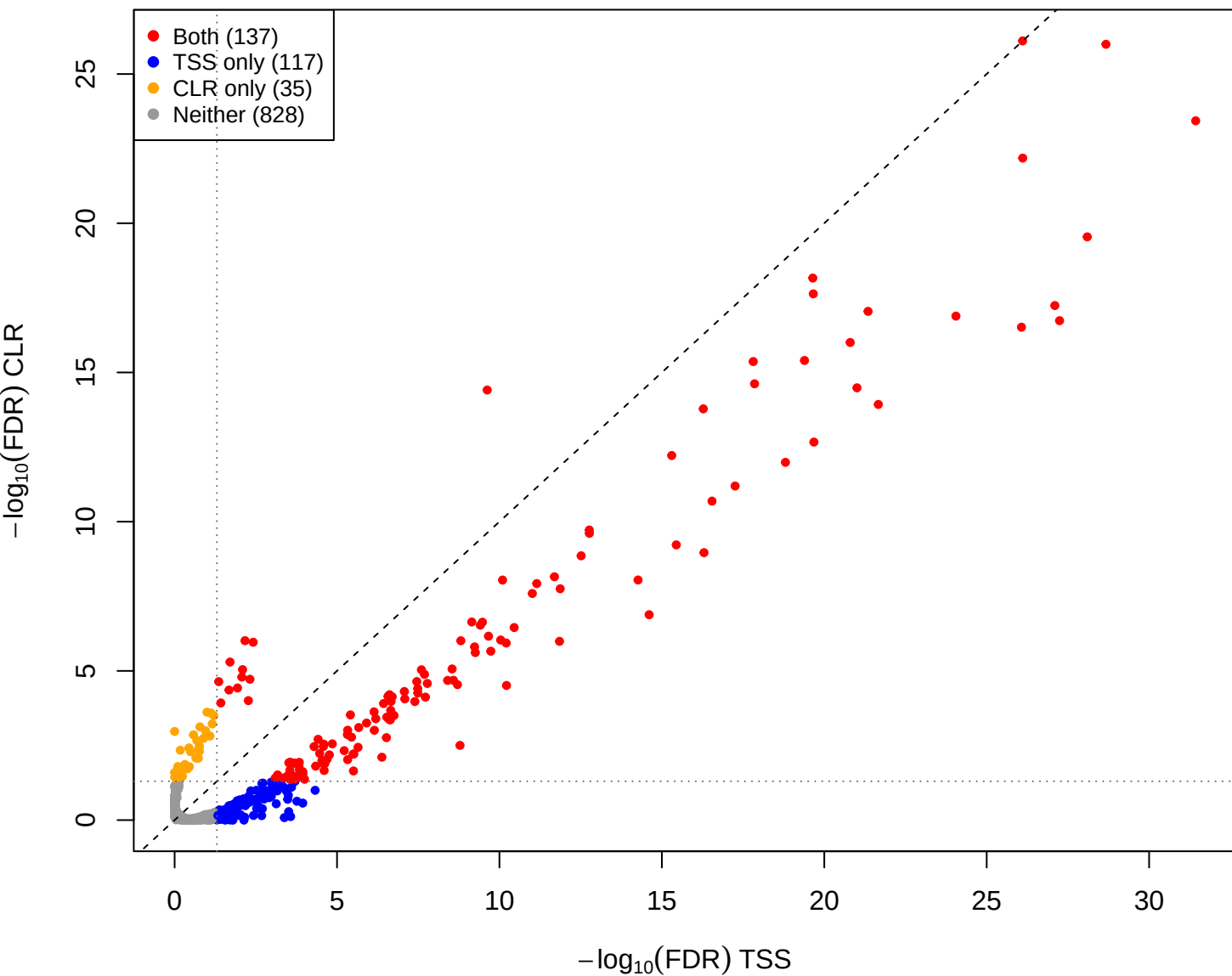
eld vs mid – CLR vs TSS(const=0.8) (gamma = 0.001)
