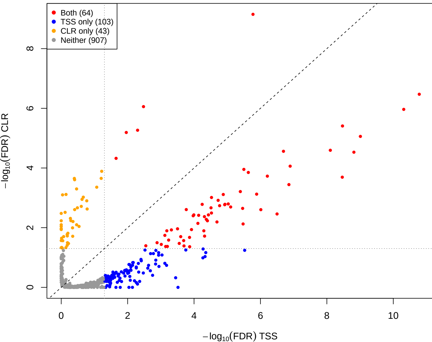
kin vs mage – CLR vs TSS(const=0.8) (gamma = 0.001)
