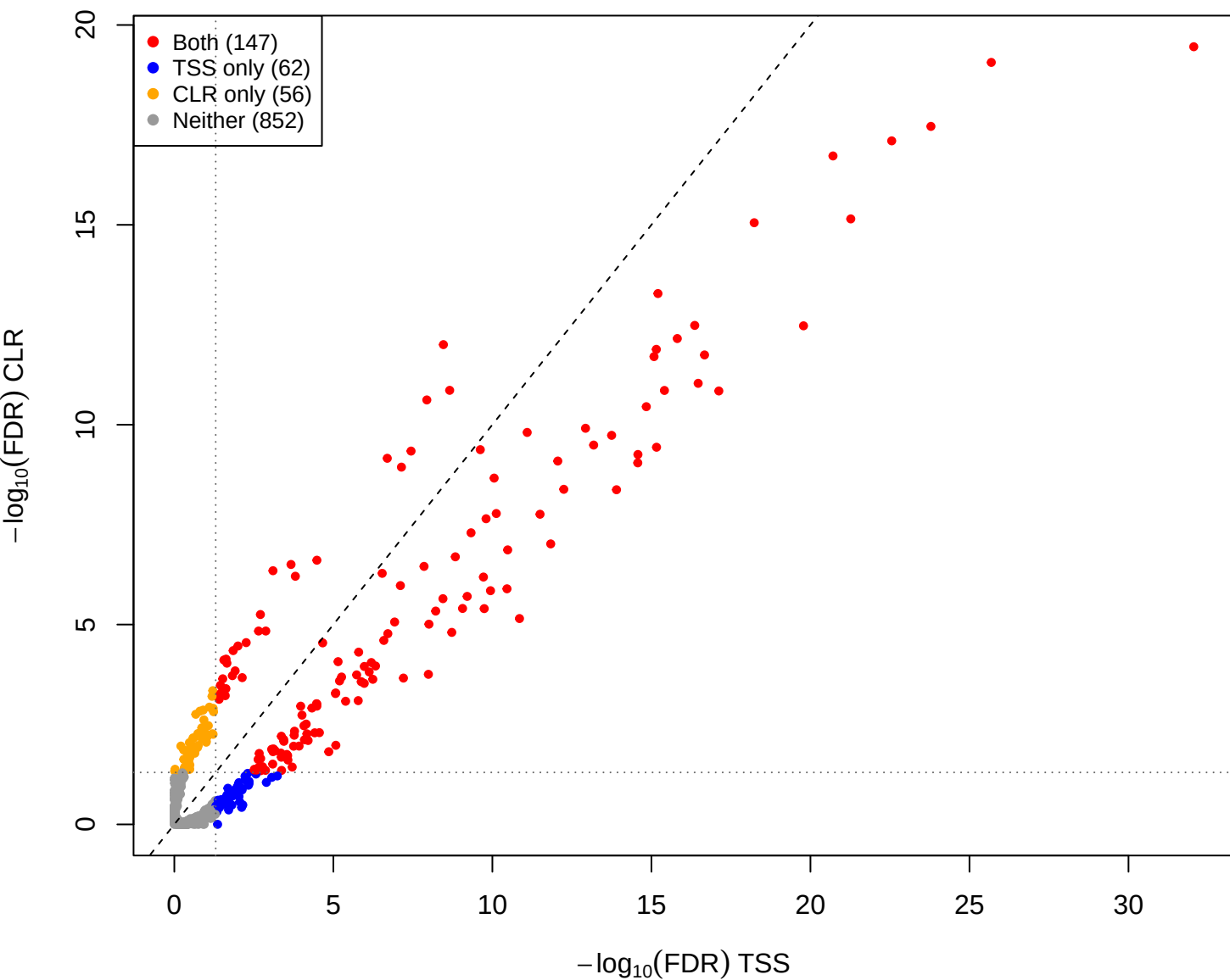
cent vs mage – CLR vs TSS(const=0.8) (gamma = 0.001)
