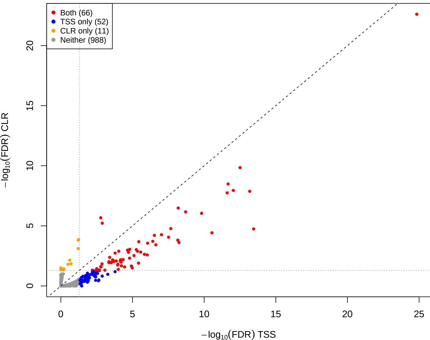
kin vs pup – CLR vs TSS(const=0.8) (gamma = 0.001)
