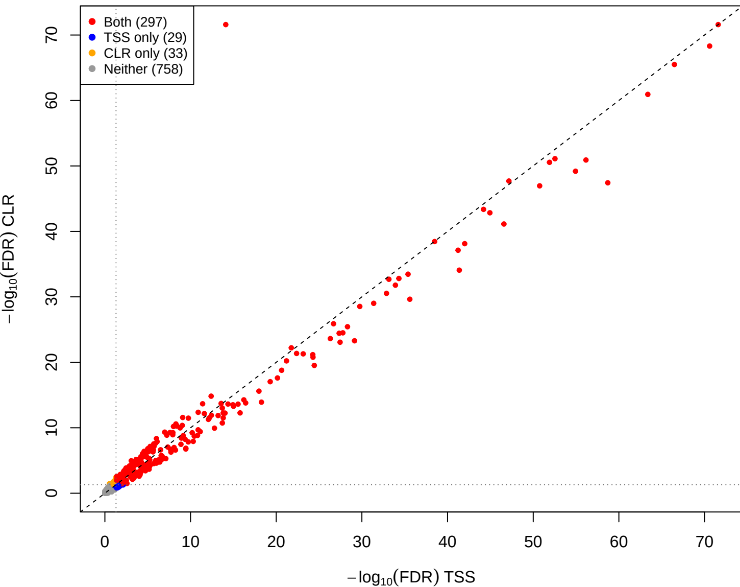
cent vs pup – CLR vs TSS(const=0.8) (gamma = 0.001)
