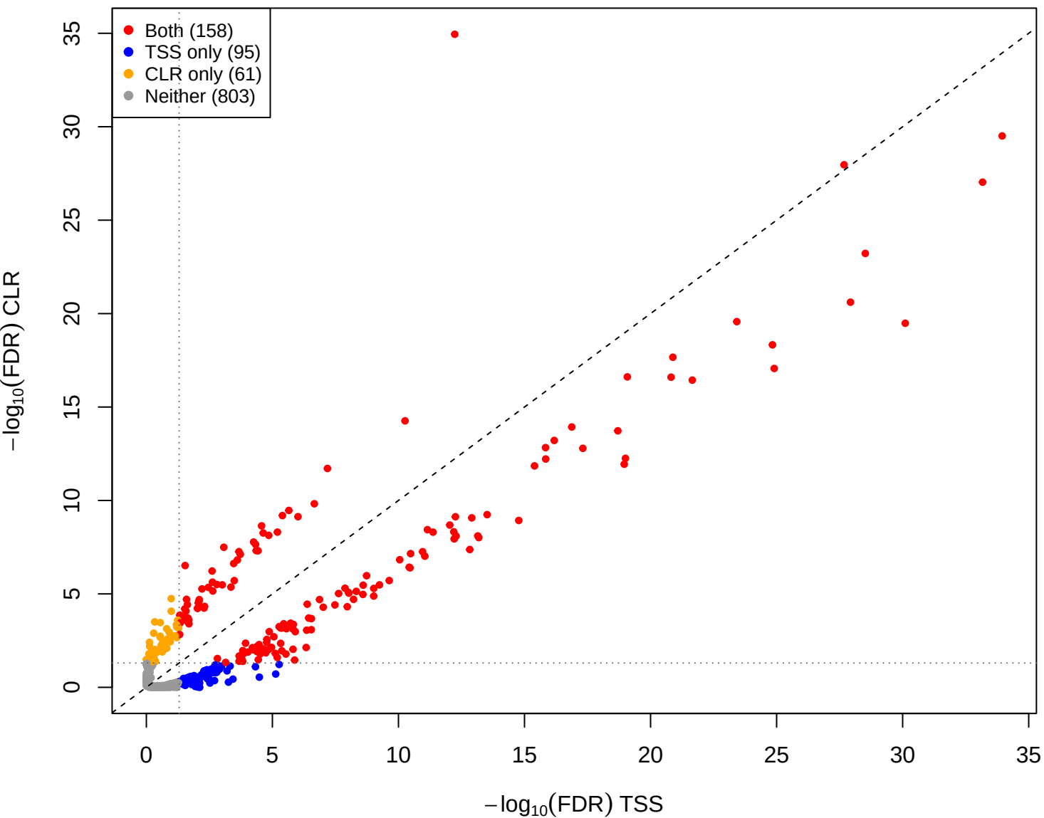
eld vs kin – CLR vs TSS(const=0.8) (gamma = 0.001)
