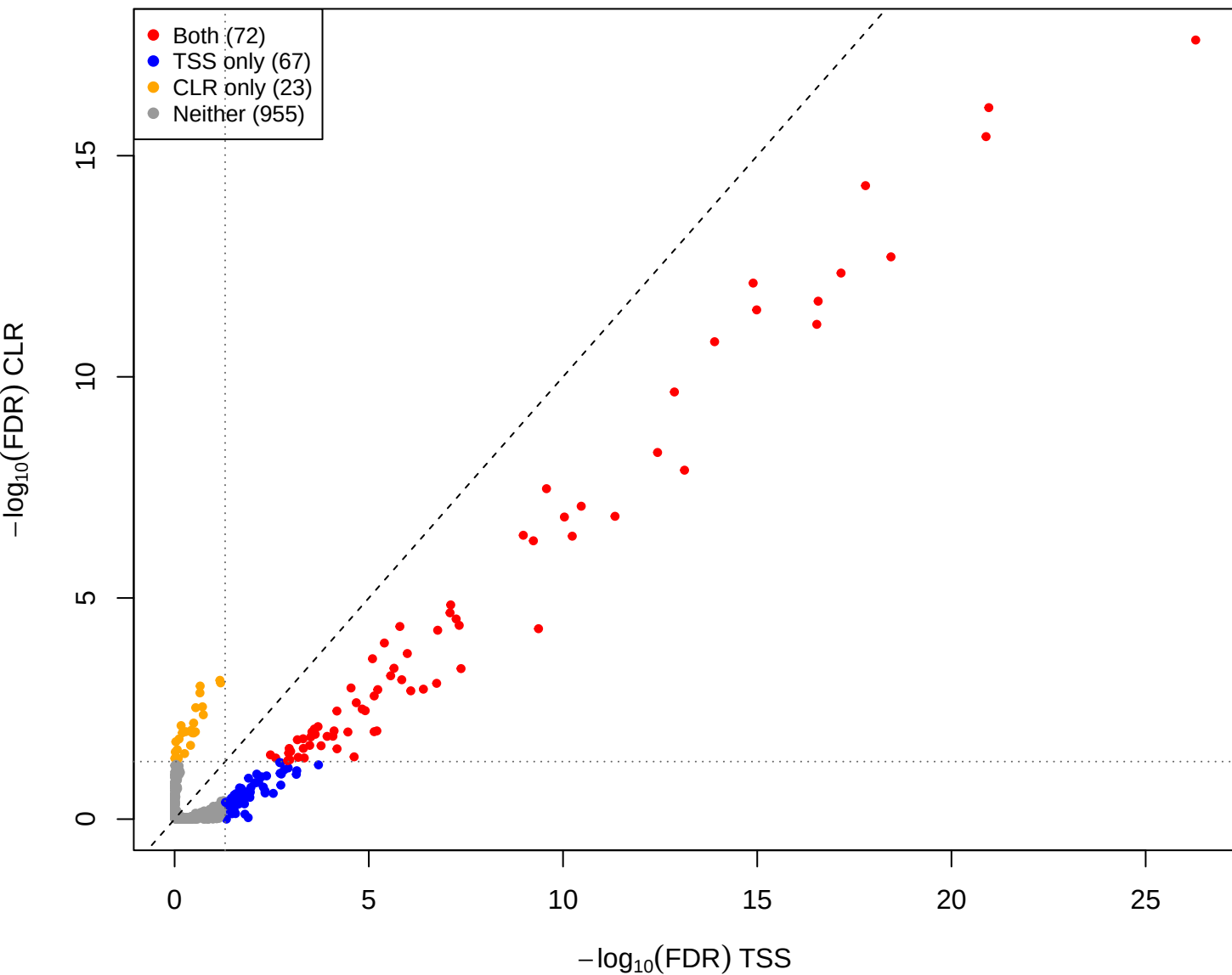
eld vs mage – CLR vs TSS(const=0.8) (gamma = 0.001)
