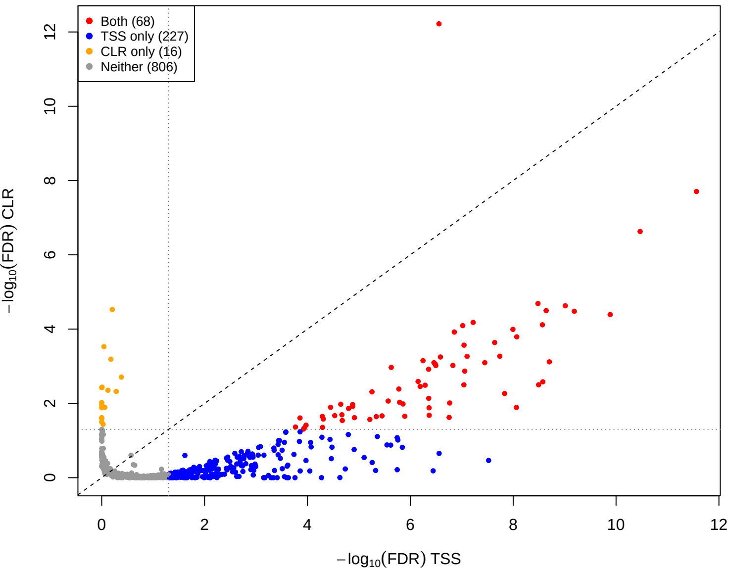
mage vs mid – CLR vs TSS(const=0.8) (gamma = 0.001)
