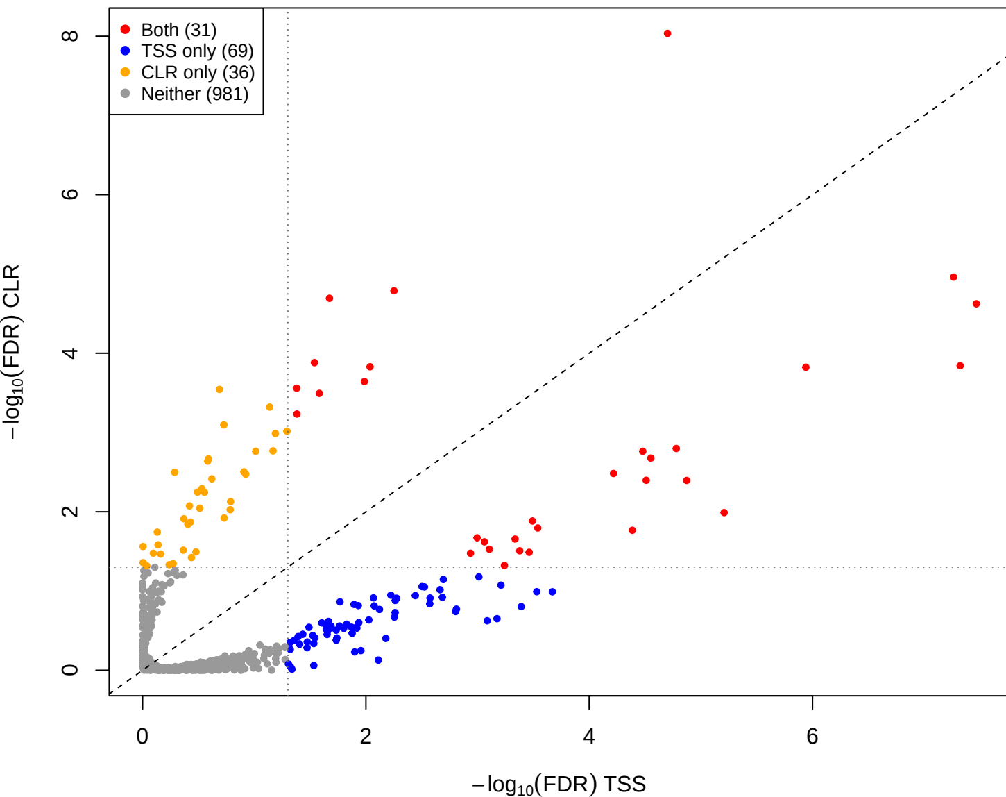
eld vs you – CLR vs TSS(const=0.8) (gamma = 0.001)
