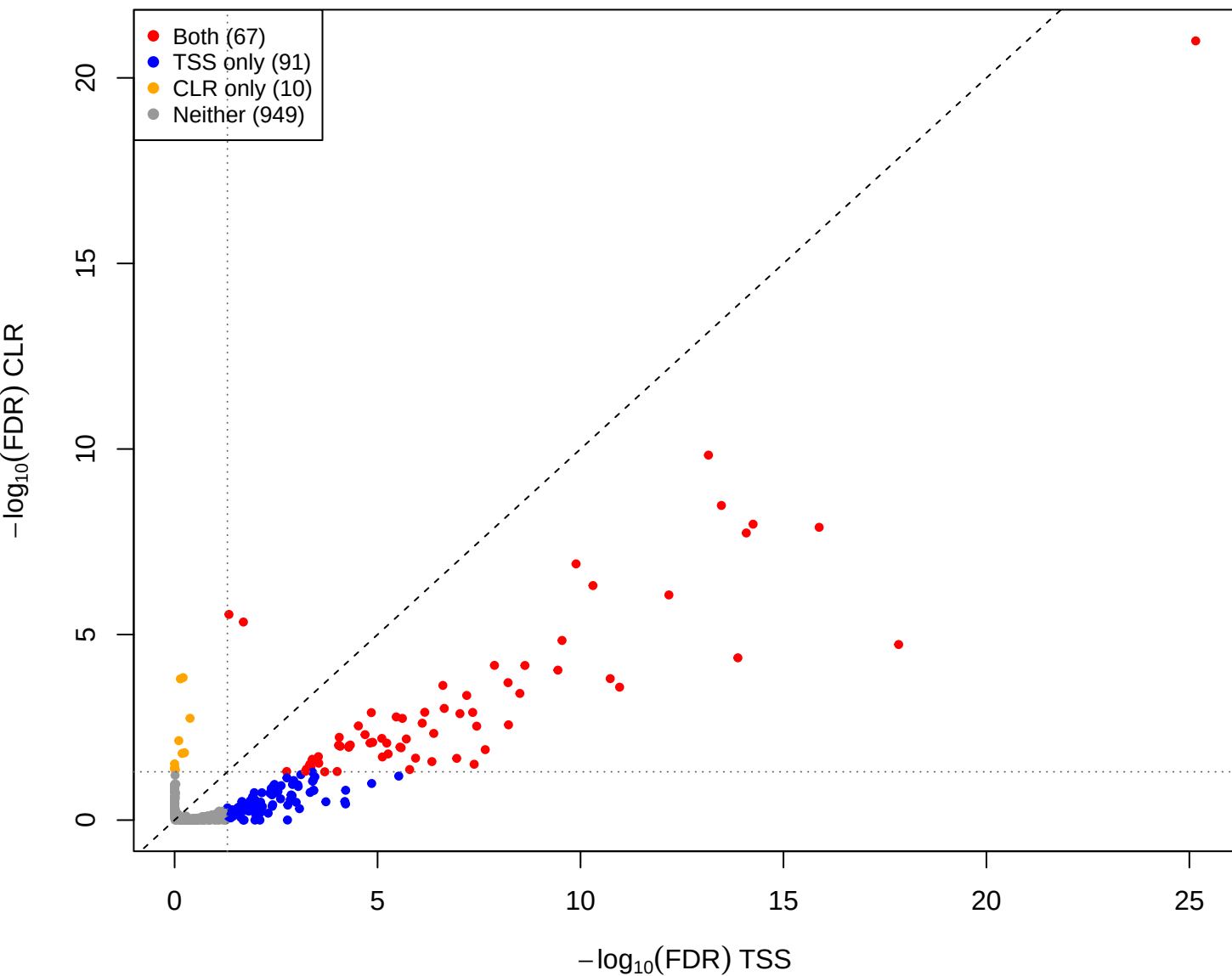
kin vs pup – CLR vs TSS(const=1) (gamma = 0.001)
