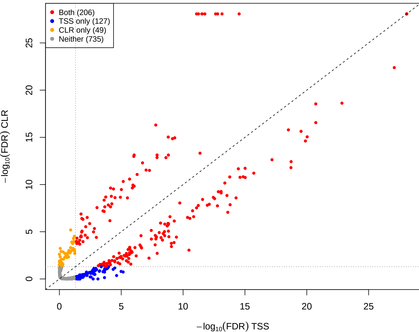
kin vs you – CLR vs TSS(const=1) (gamma = 0.001)
