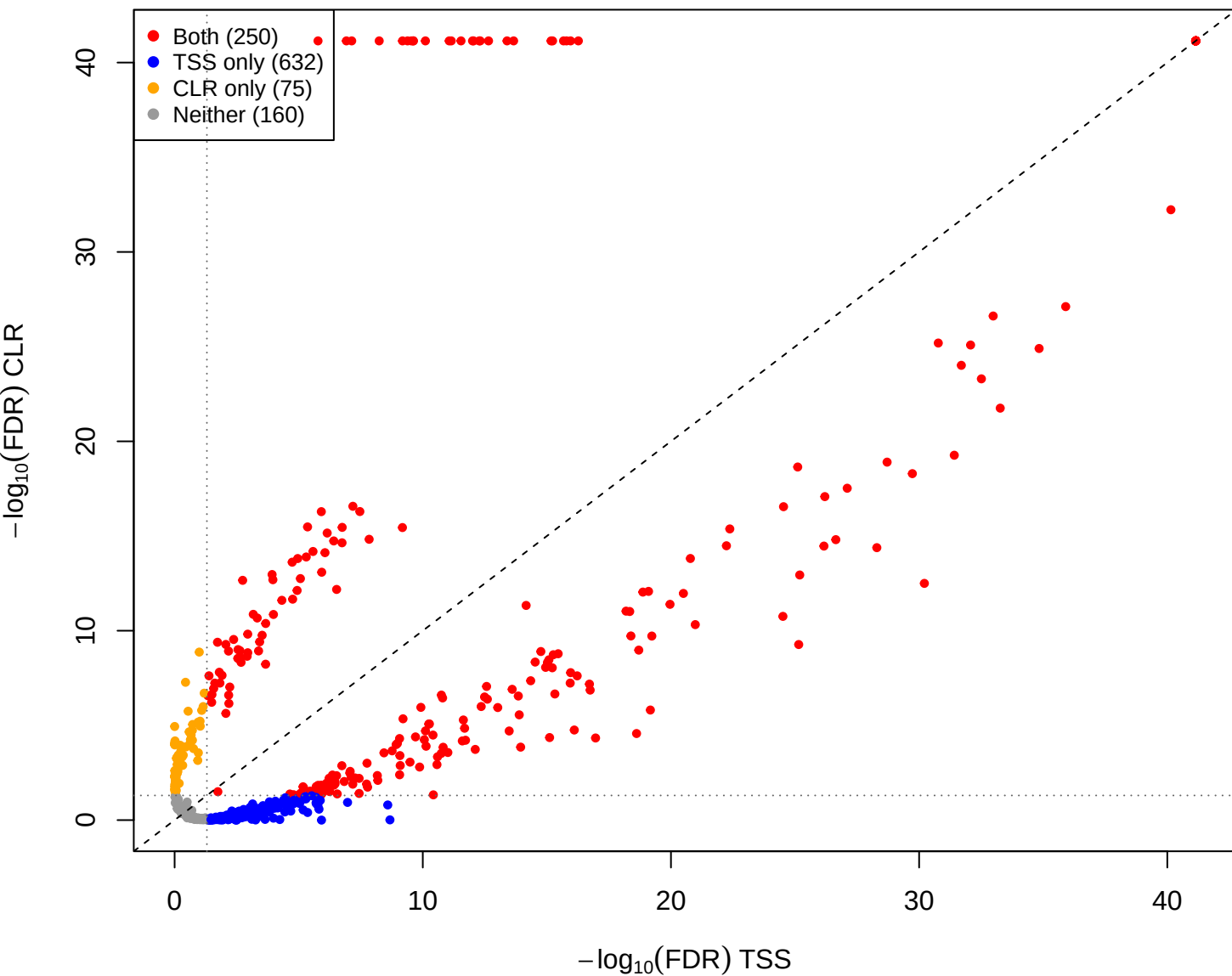
pup vs you – CLR vs TSS(const=1) (gamma = 0.001)
