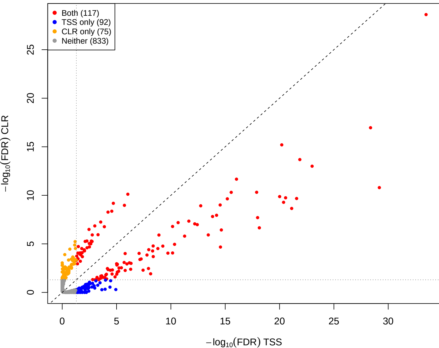
mid vs pup – CLR vs TSS(const=1) (gamma = 0.001)
