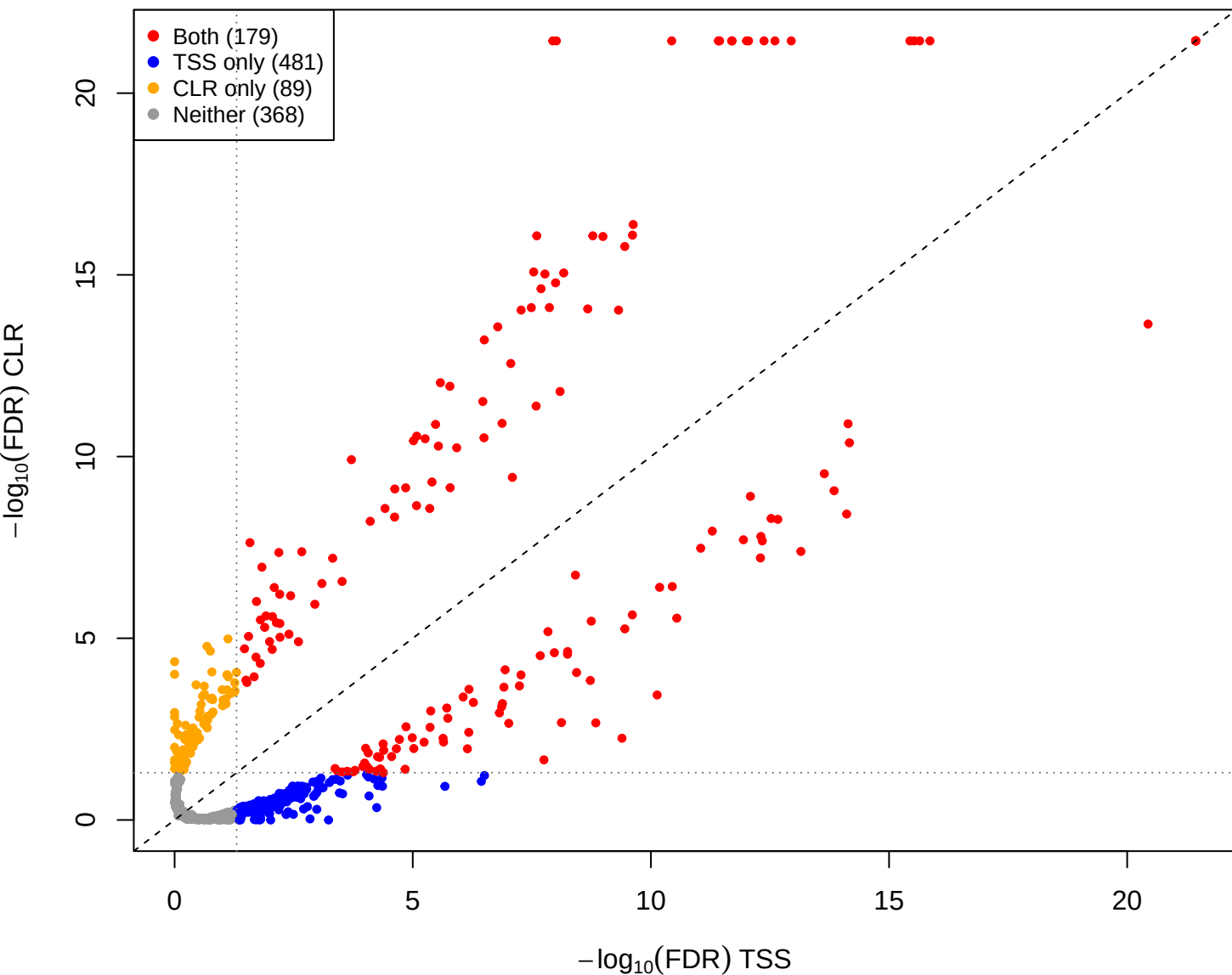
mid vs you – CLR vs TSS(const=1) (gamma = 0.001)
