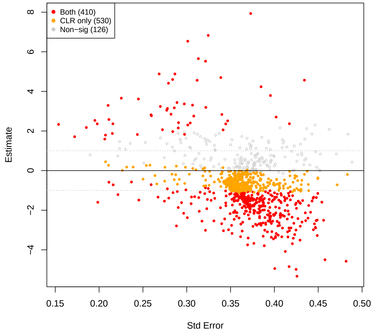
cent vs pup – TSS (CLR(const=-0.9) sig overlay)
