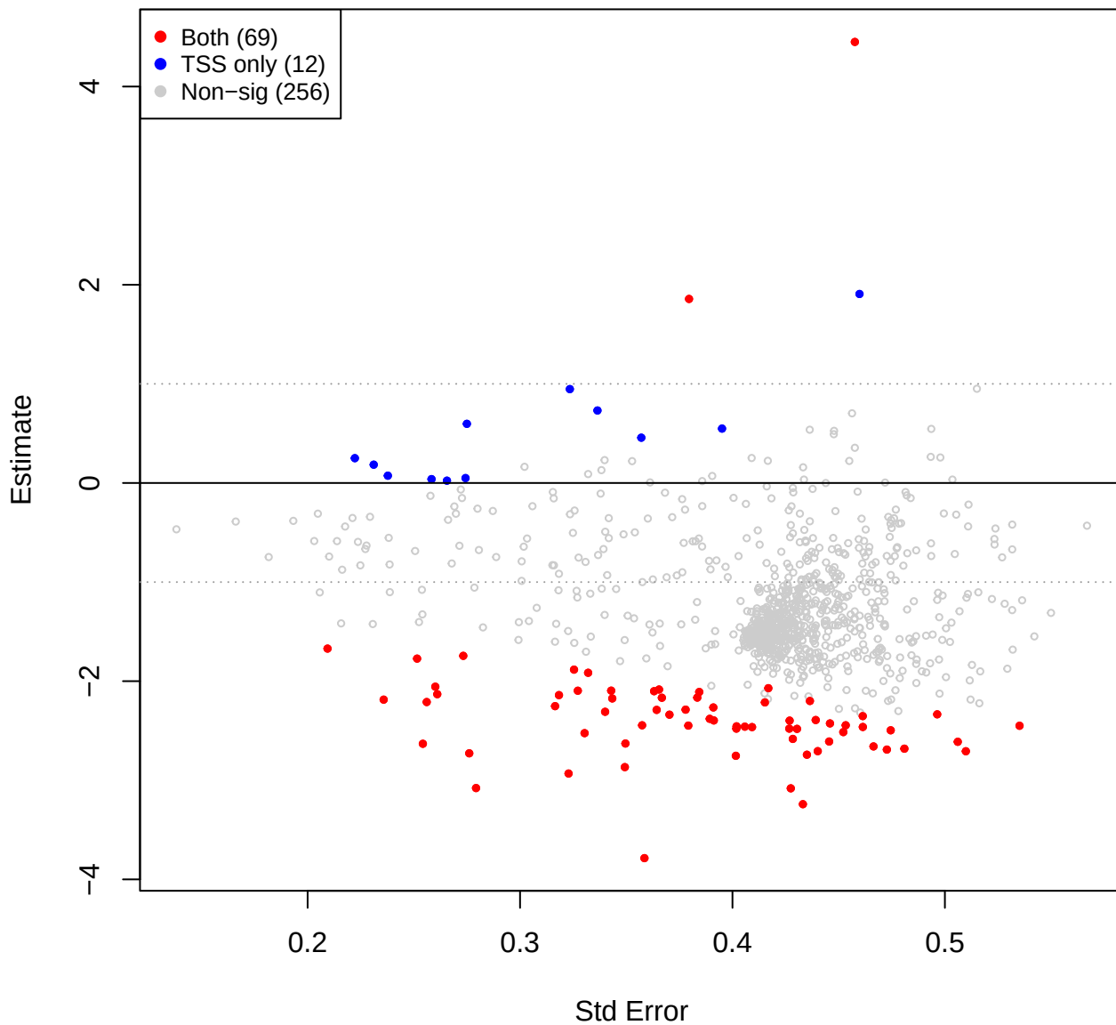
kin vs pup – CLR(const=-0.9) (TSS sig overlay)
