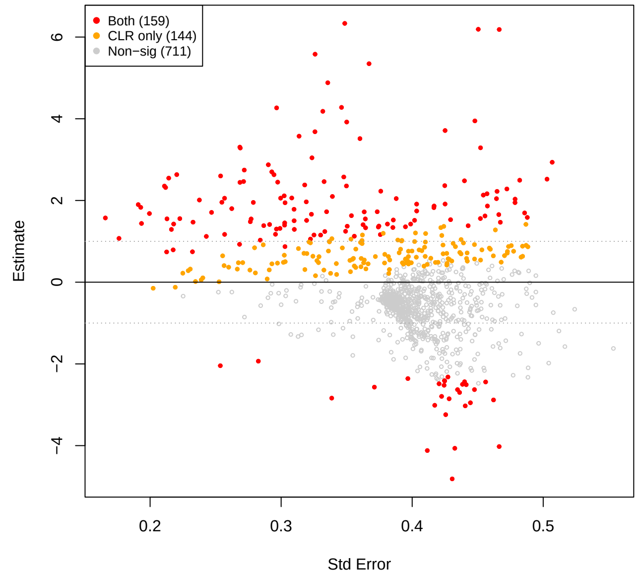
cent vs mid – TSS (CLR(const=0.8) sig overlay)
