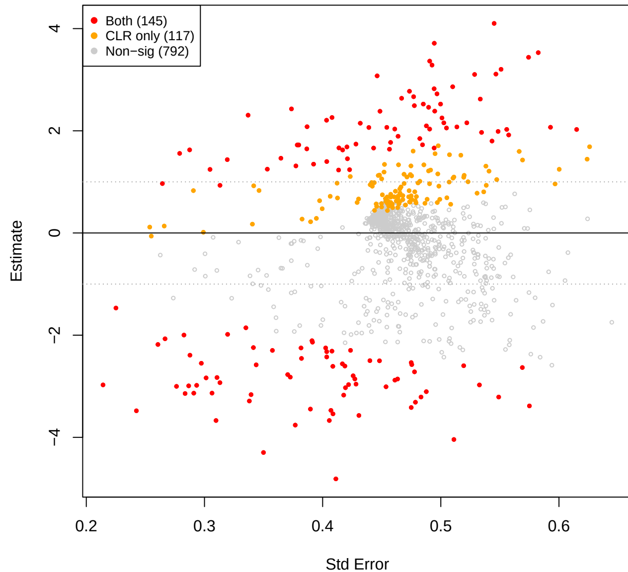
mage vs you – TSS (CLR(const=0.8) sig overlay)
