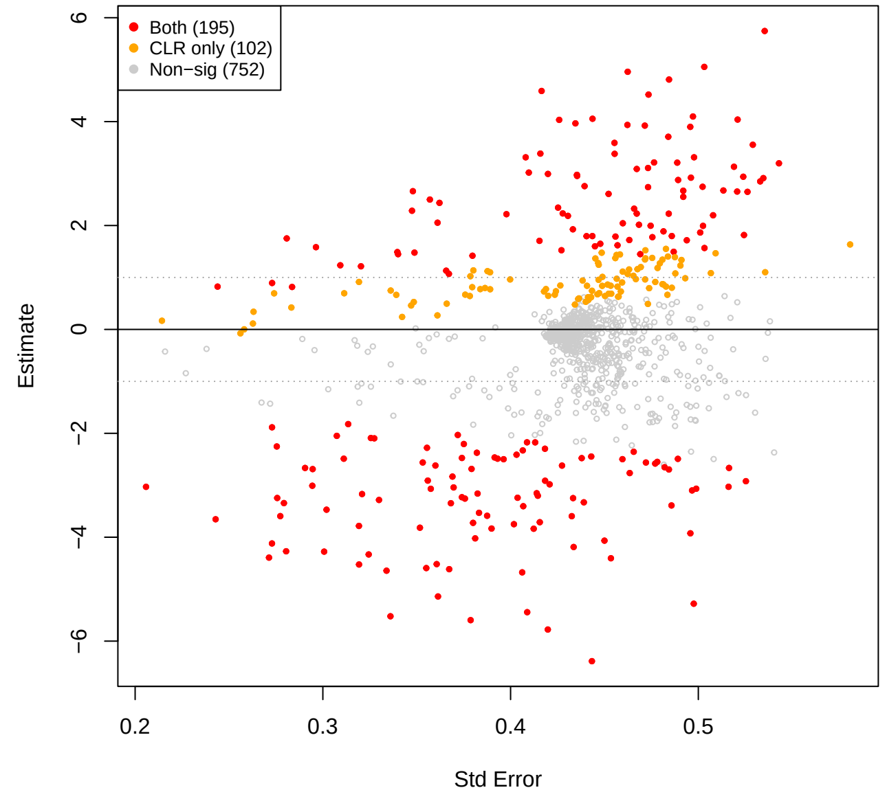
kin vs you – TSS (CLR(const=0.8) sig overlay)
