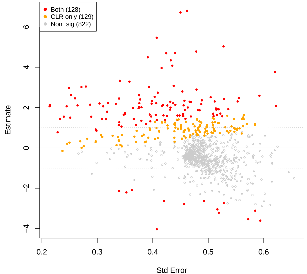
eld vs mid - TSS (CLR(const=0.8) sig overlay)
