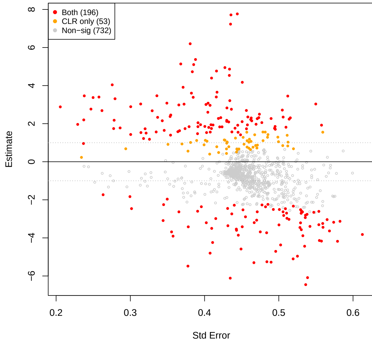
eld vs pup – TSS (CLR(const=0.8) sig overlay)
