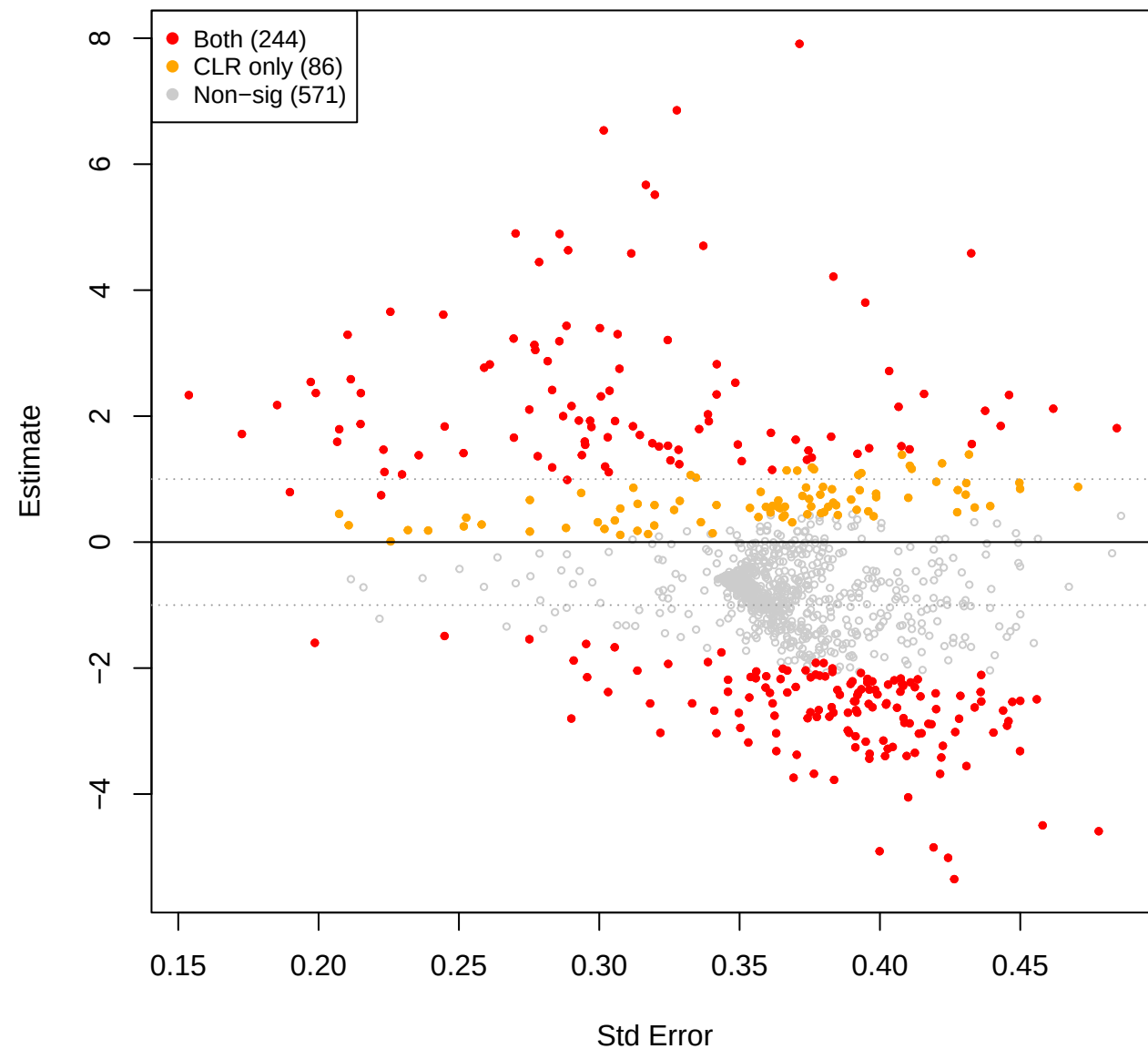
cent vs pup – TSS (CLR(const=0.8) sig overlay)
