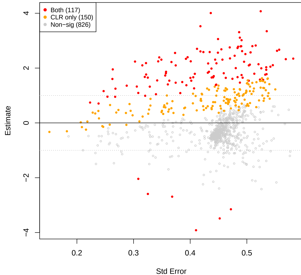
kin vs mid – TSS (CLR(const=0.8) sig overlay)
