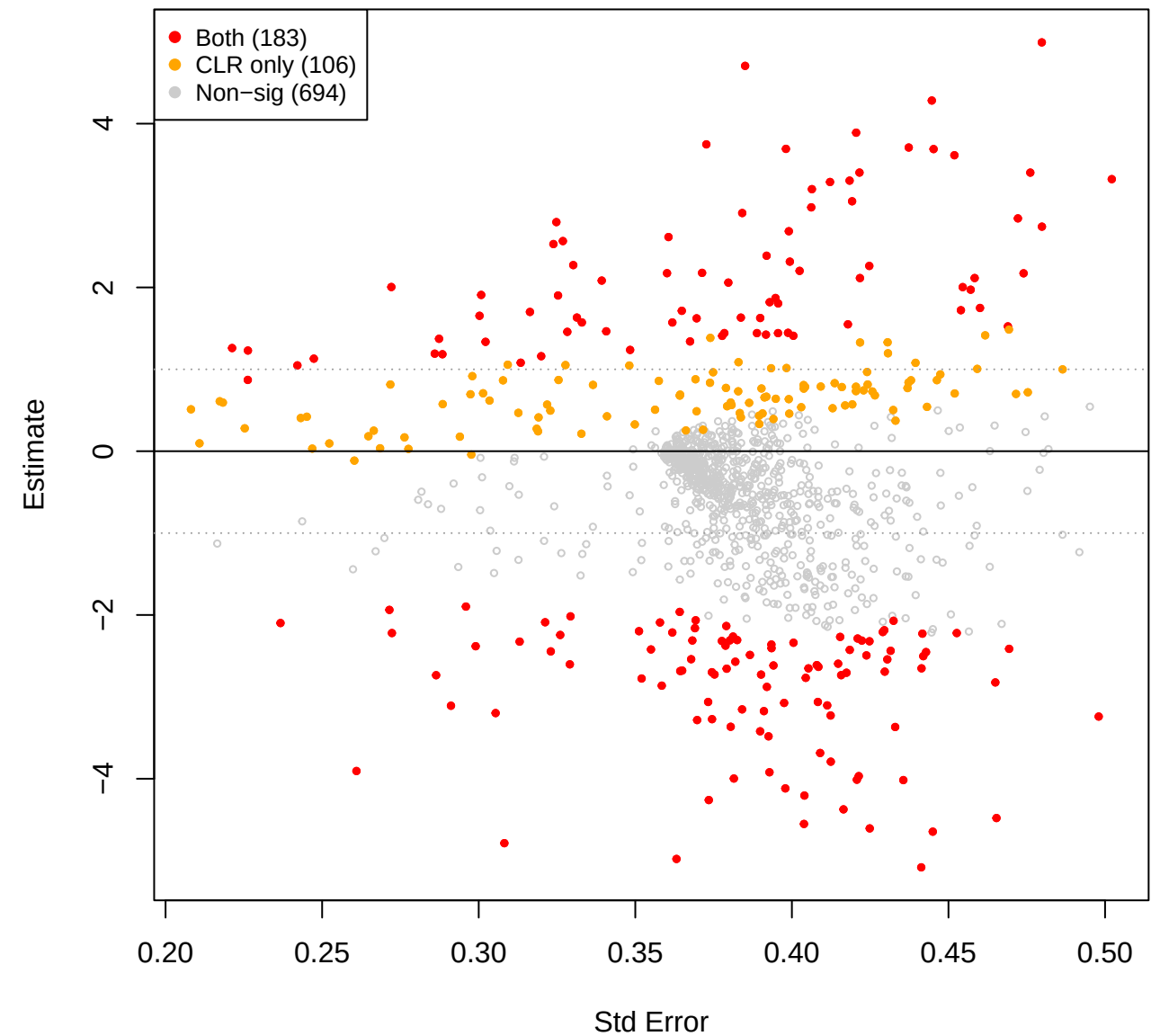
cent vs you – TSS (CLR(const=0.8) sig overlay)
