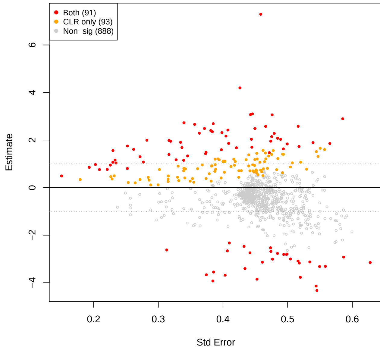
mage vs pup – TSS (CLR(const=0.8) sig overlay)
