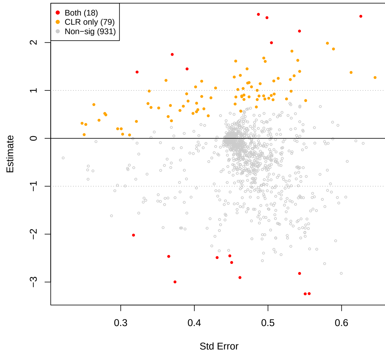
eld vs you - TSS (CLR(const=0.8) sig overlay)
