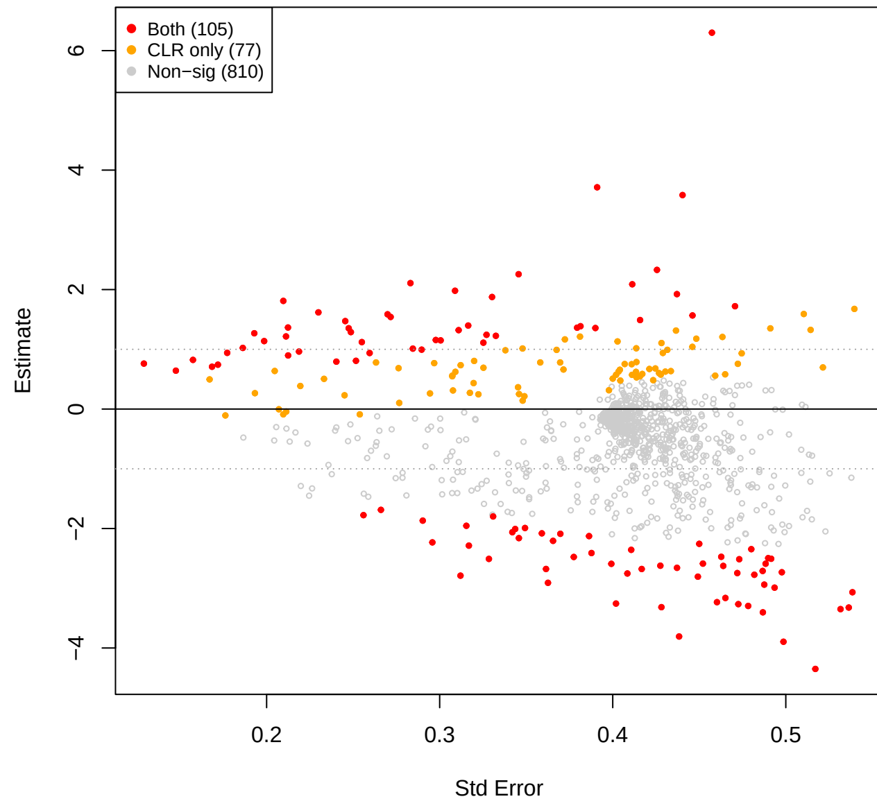
mid vs pup – TSS (CLR(const=0.8) sig overlay)
