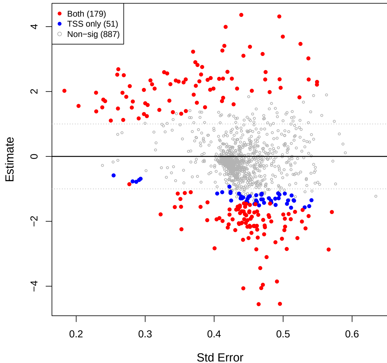
cent vs mage – CLR(const=0.2) (TSS sig overlay)
