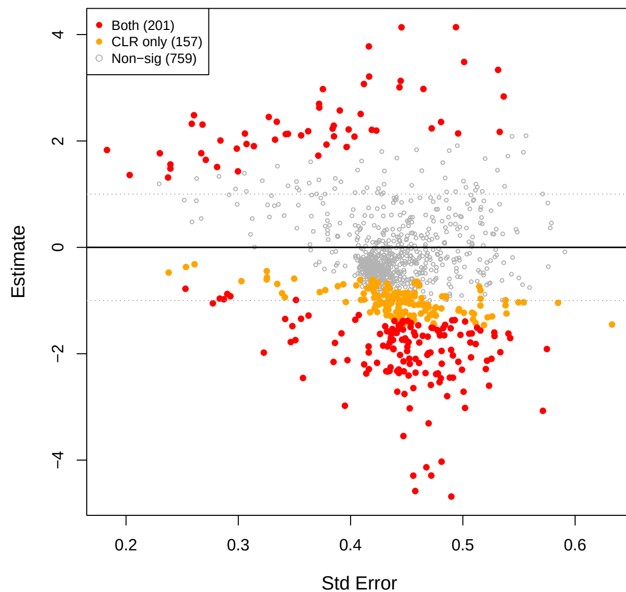
cent vs mage – TSS (CLR(const=-0.5) sig overlay)
