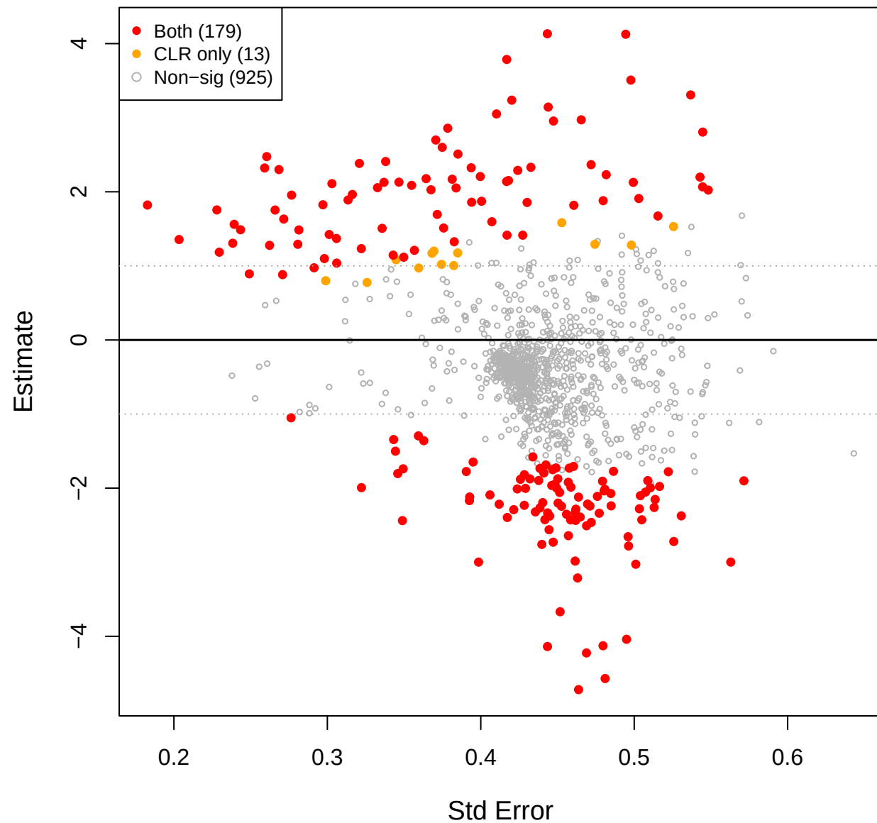
cent vs mage – TSS (CLR(const=0.2) sig overlay)
