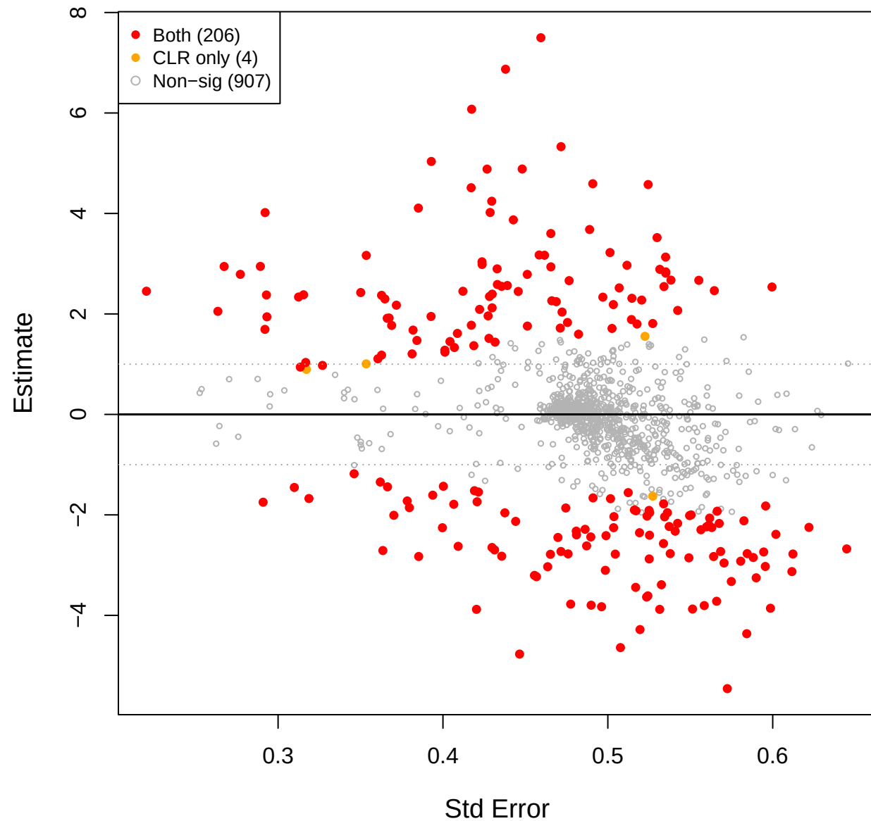
eld vs kin – TSS (CLR(const=0.1) sig overlay)
