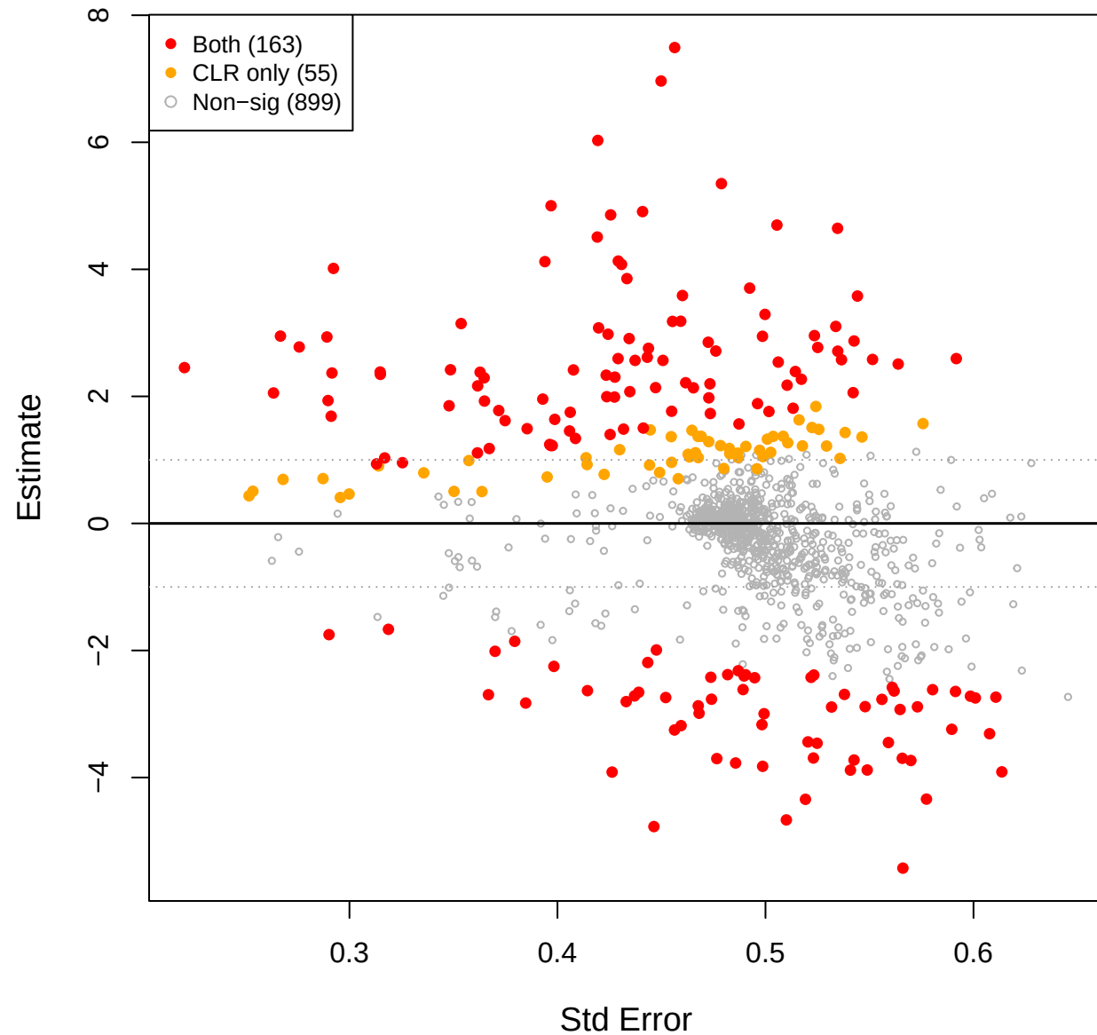
eld vs kin – TSS (CLR(const=0.5) sig overlay)
