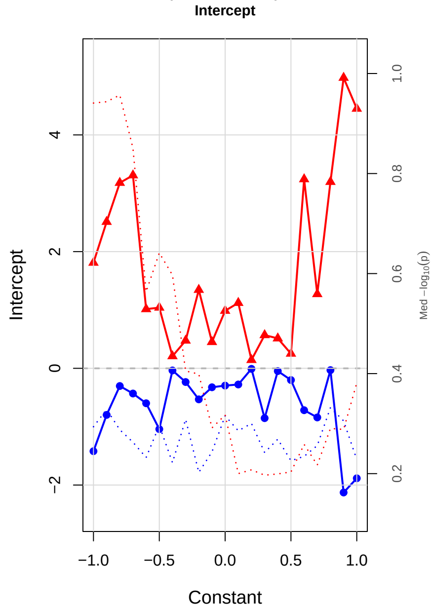
CLR_const | cent vs mage | gamma=0.5
