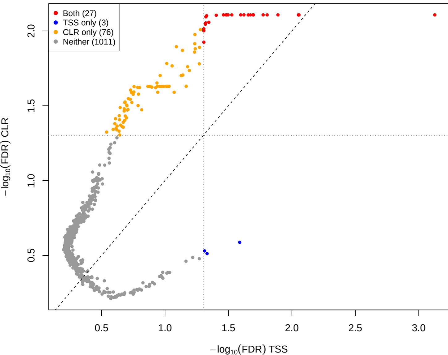
kin vs you – CLR(const=-2) vs TSS (gamma = 2)
