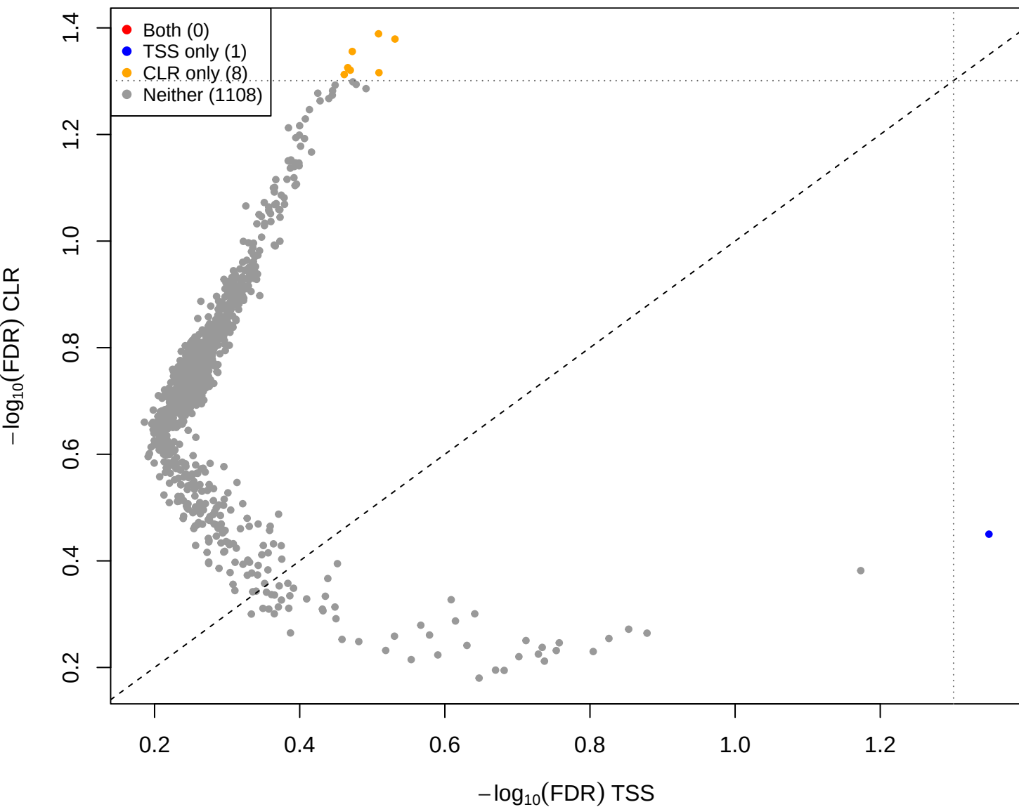
eld vs mage - CLR(const=-2) vs TSS (gamma = 2)
