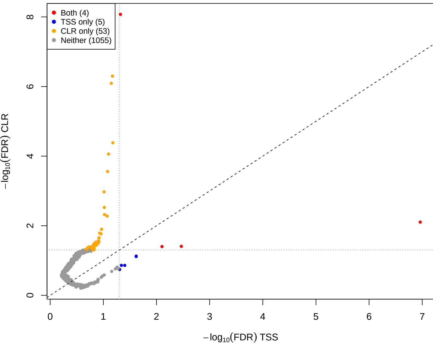
cent vs pup – CLR(const=-2) vs TSS (gamma = 2)
