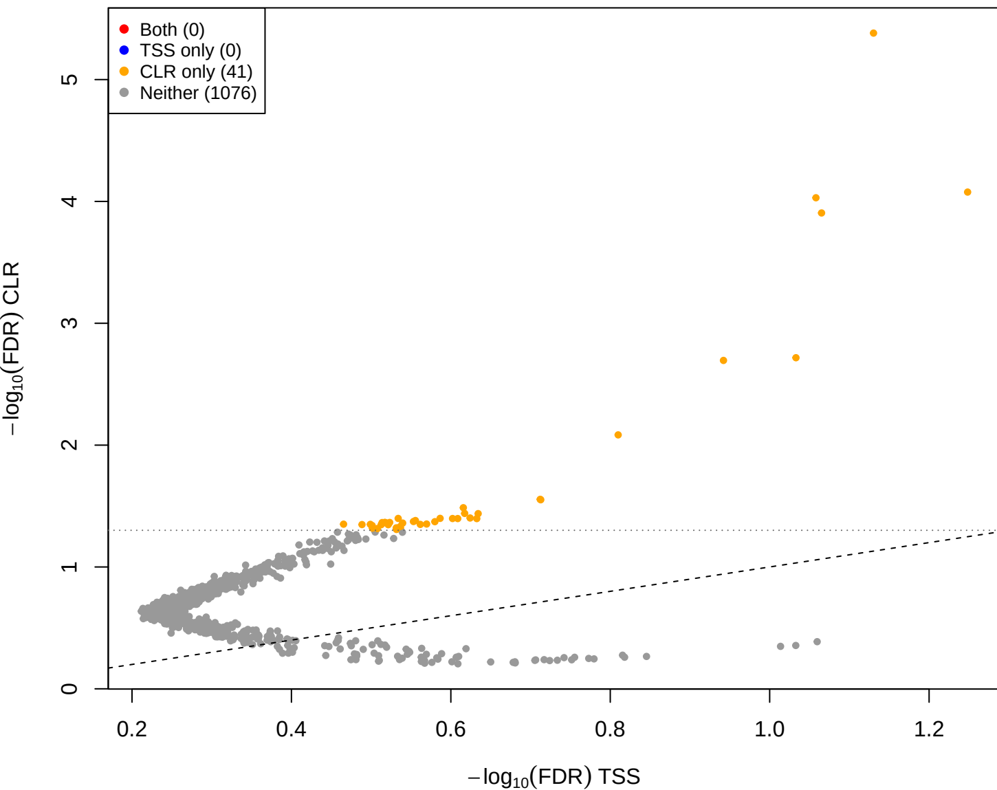
cent vs mage - CLR(const=-2) vs TSS (gamma = 2)
