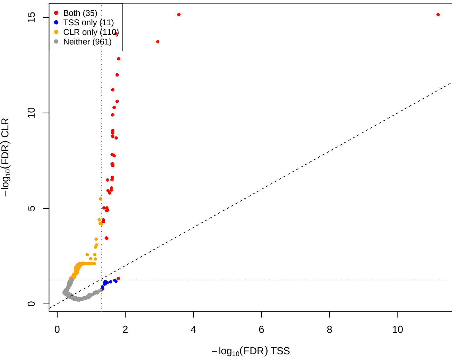
pup vs you - CLR(const=-2) vs TSS (gamma = 2)
