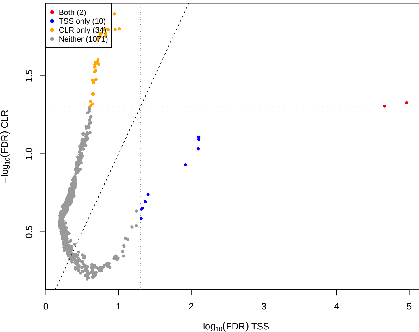
cent vs kin - CLR(const=-2) vs TSS (gamma = 2)
