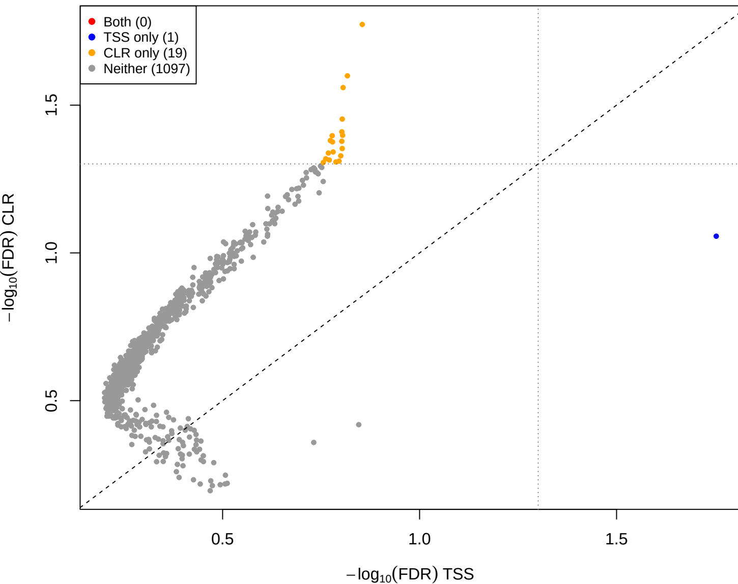
mid vs pup – CLR(const=-2) vs TSS (gamma = 2)
