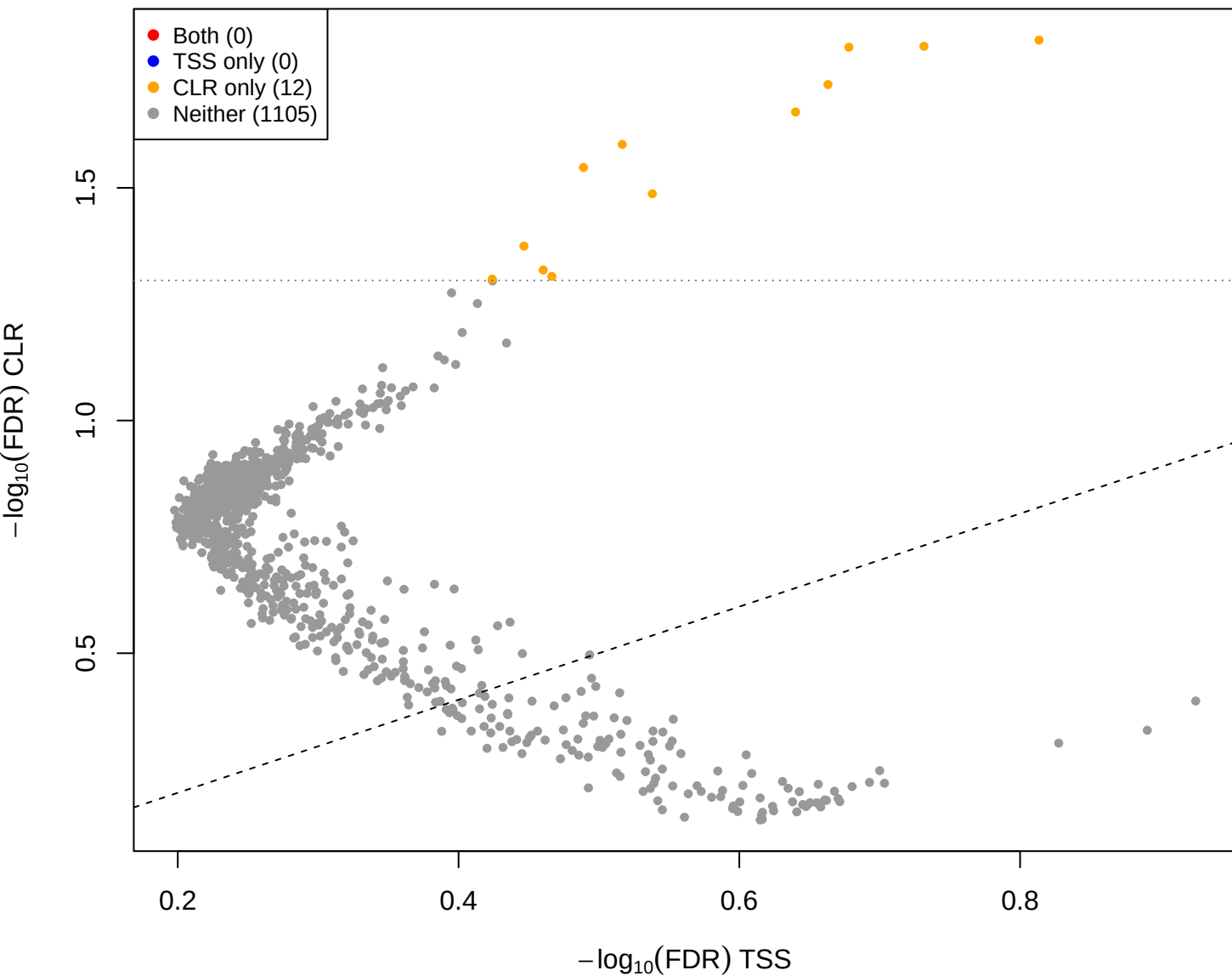
kin vs mid – CLR(const=-2) vs TSS (gamma = 2)
