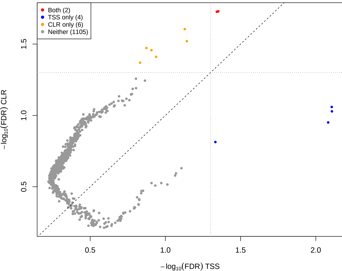
eld vs pup – CLR(const=-2) vs TSS (gamma = 3)
