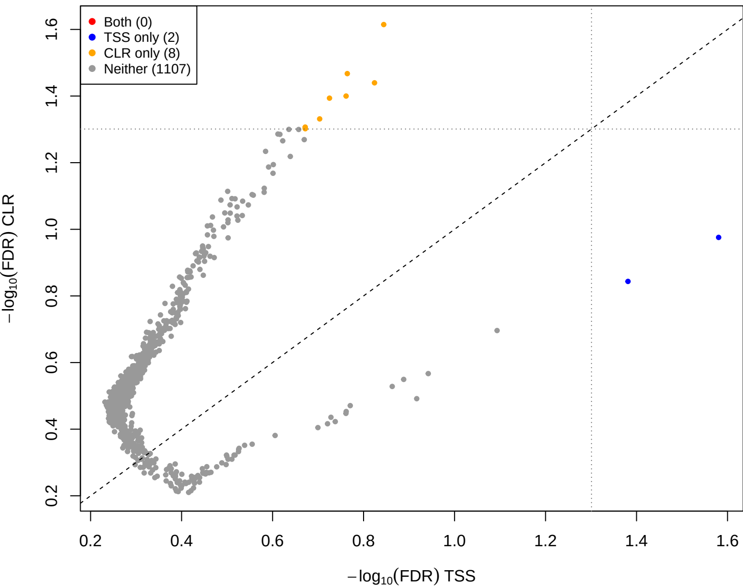
eld vs kin - CLR(const=-2) vs TSS (gamma = 3)
