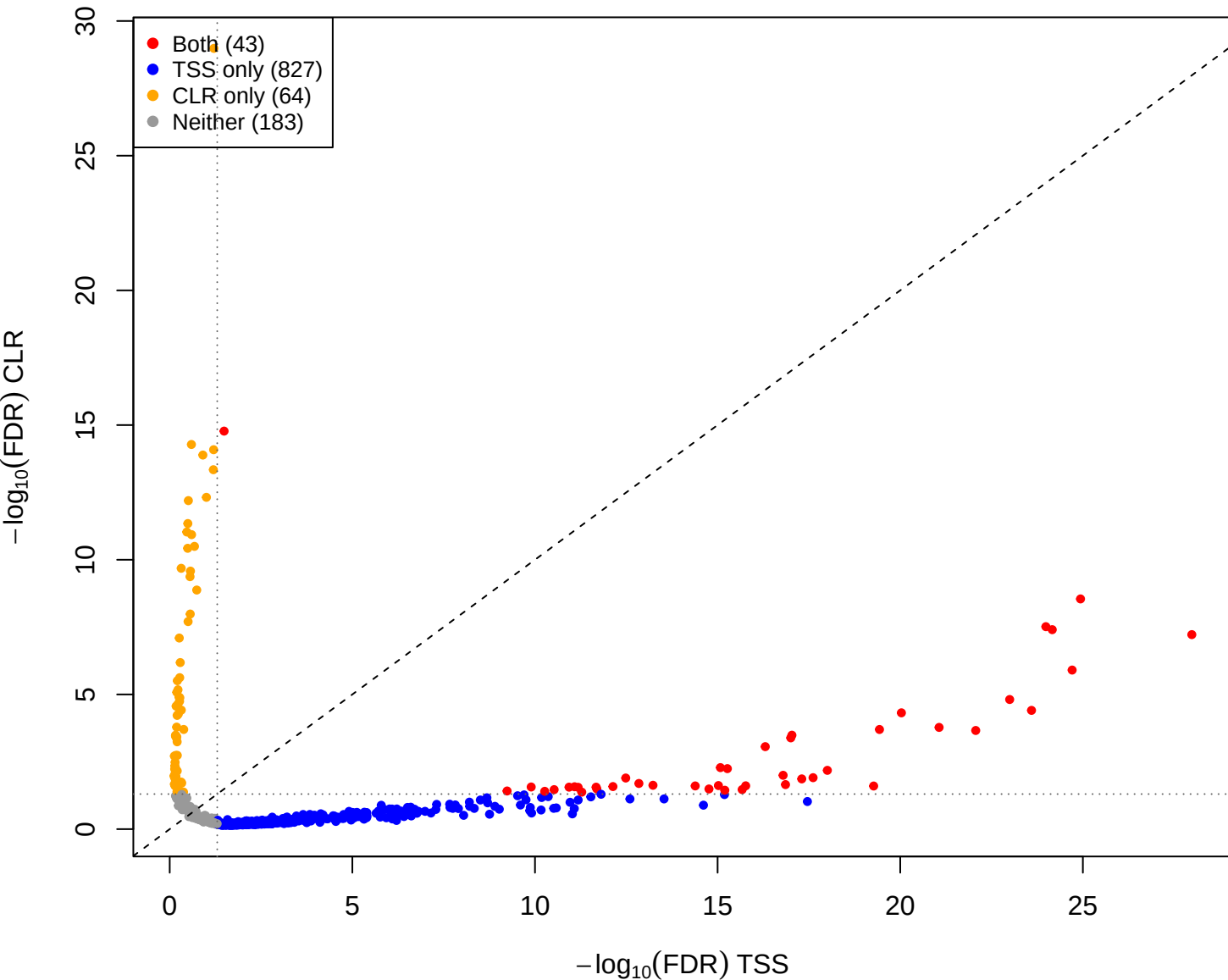
kin vs you – CLR vs TSS(const=3) (gamma = 1)
