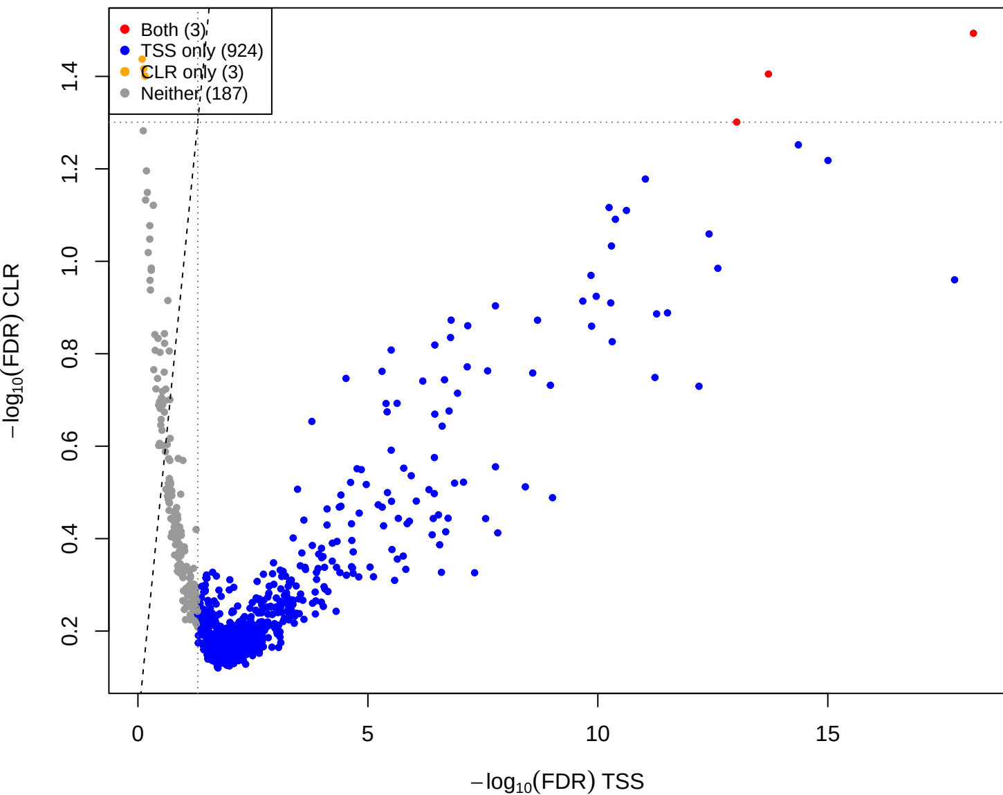
cent vs eld – CLR vs TSS(const=3) (gamma = 1)
