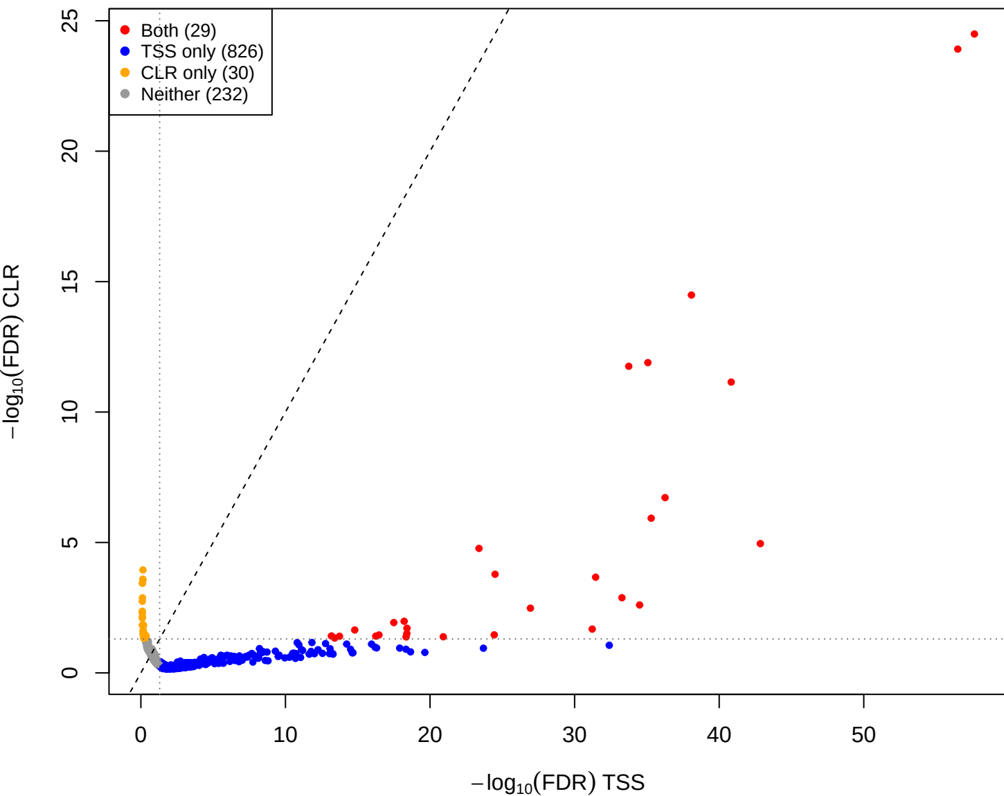
cent vs kin – CLR vs TSS(const=3) (gamma = 1)
