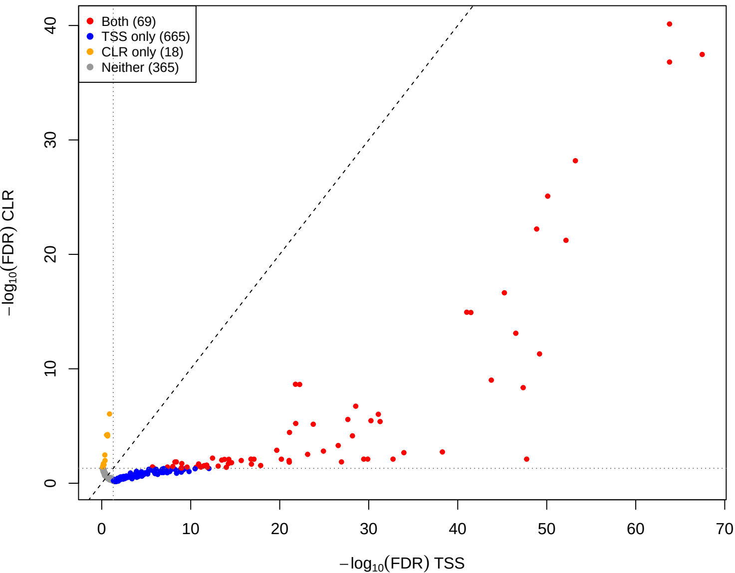
cent vs pup – CLR vs TSS(const=3) (gamma = 1)
