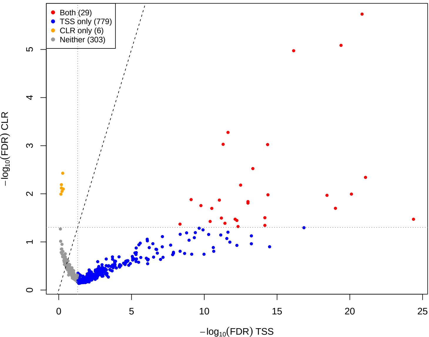
cent vs mage - CLR vs TSS(const=3) (gamma = 1)
