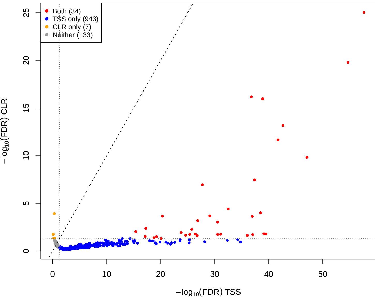
cent vs mid – CLR vs TSS(const=3) (gamma = 1)
