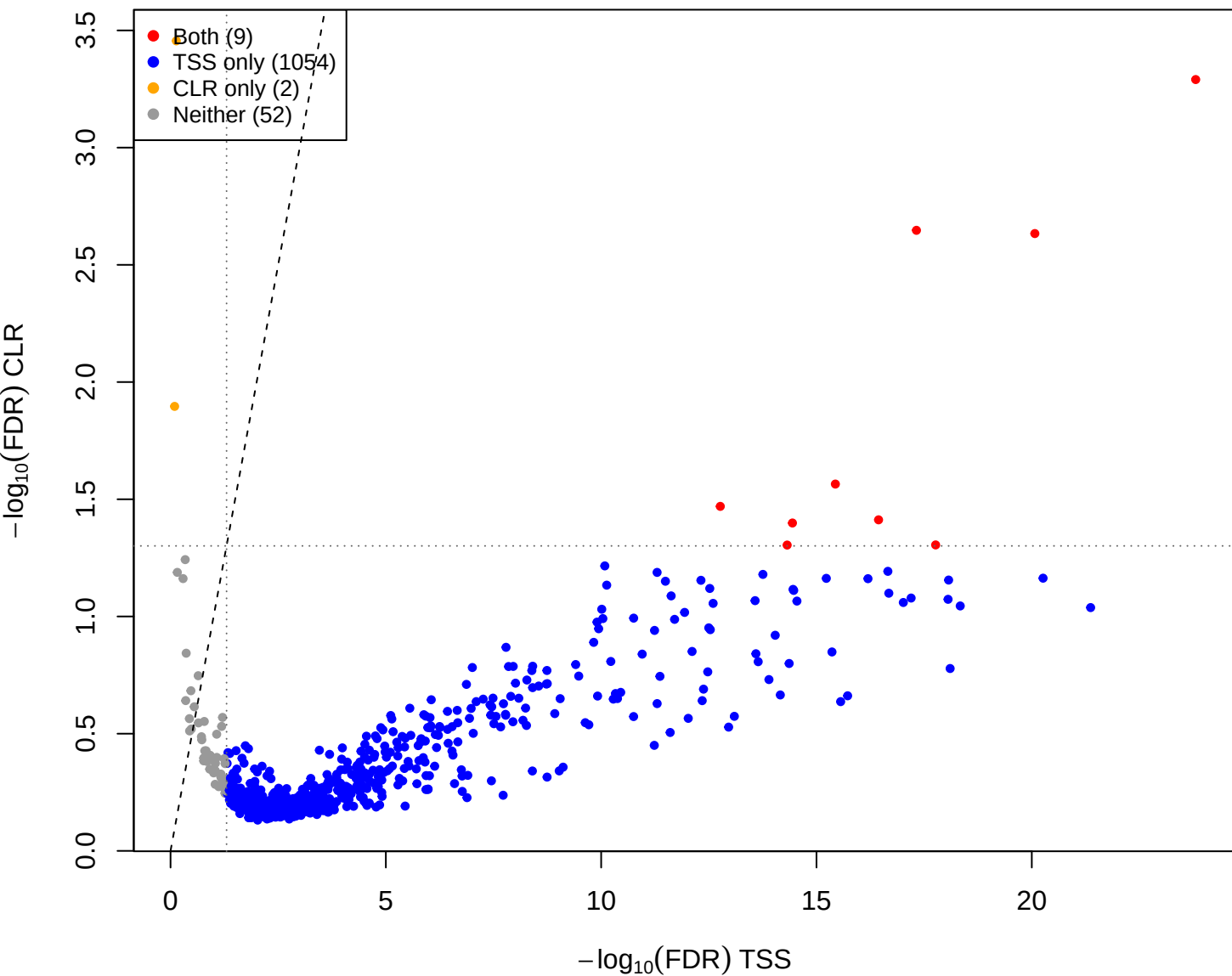
kin vs mid – CLR vs TSS(const=3) (gamma = 1)
