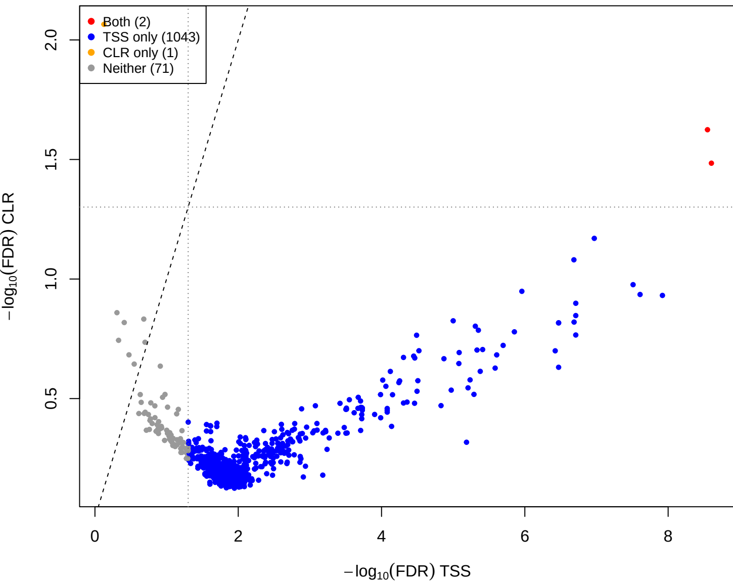
mage vs mid – CLR vs TSS(const=3) (gamma = 1)
