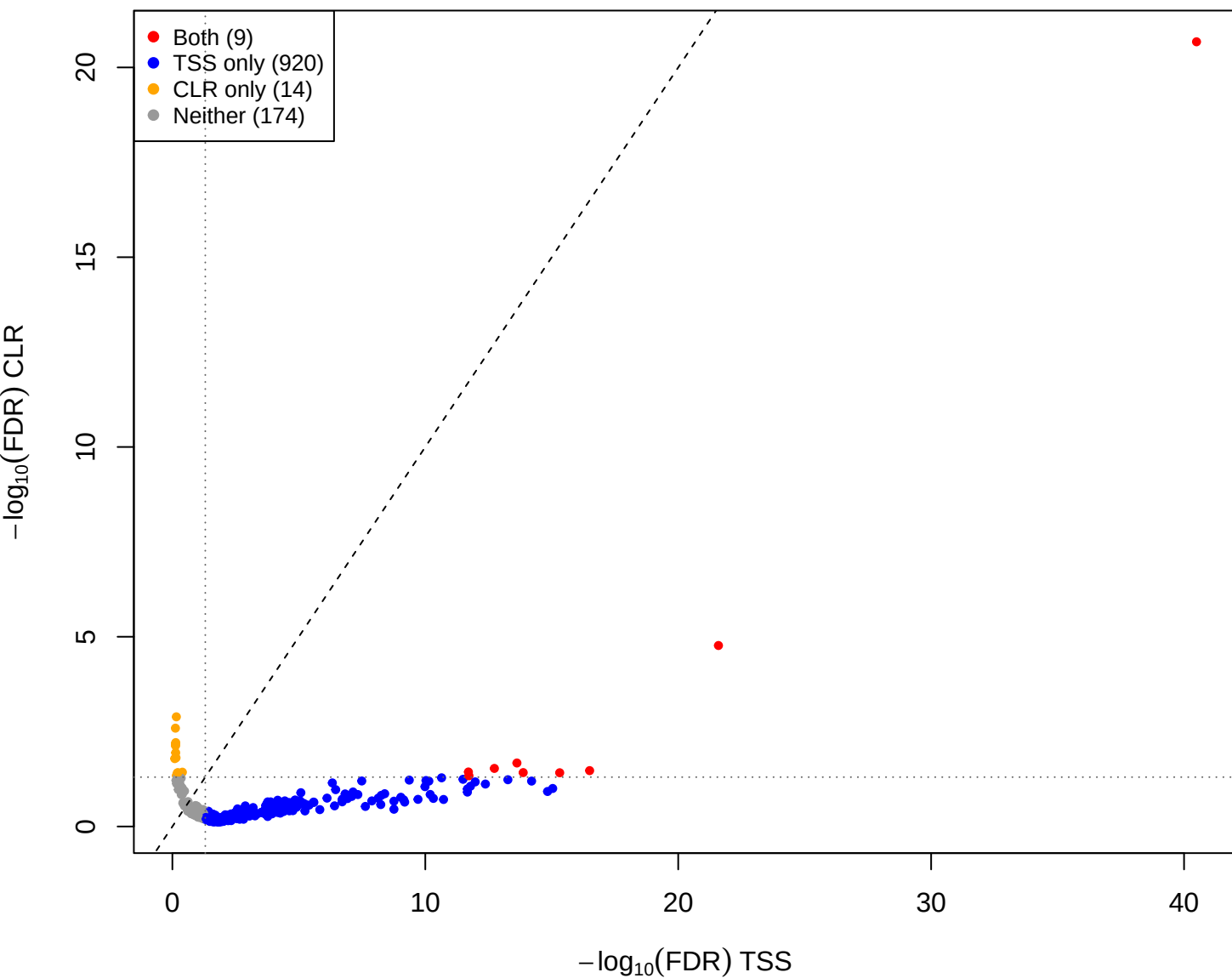
mage vs pup – CLR vs TSS(const=3) (gamma = 1)
