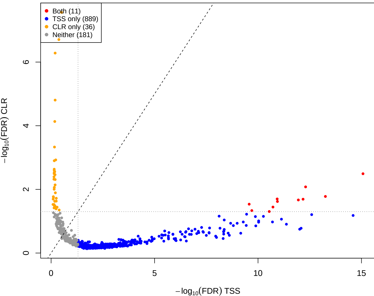
mage vs you – CLR vs TSS(const=3) (gamma = 1)
