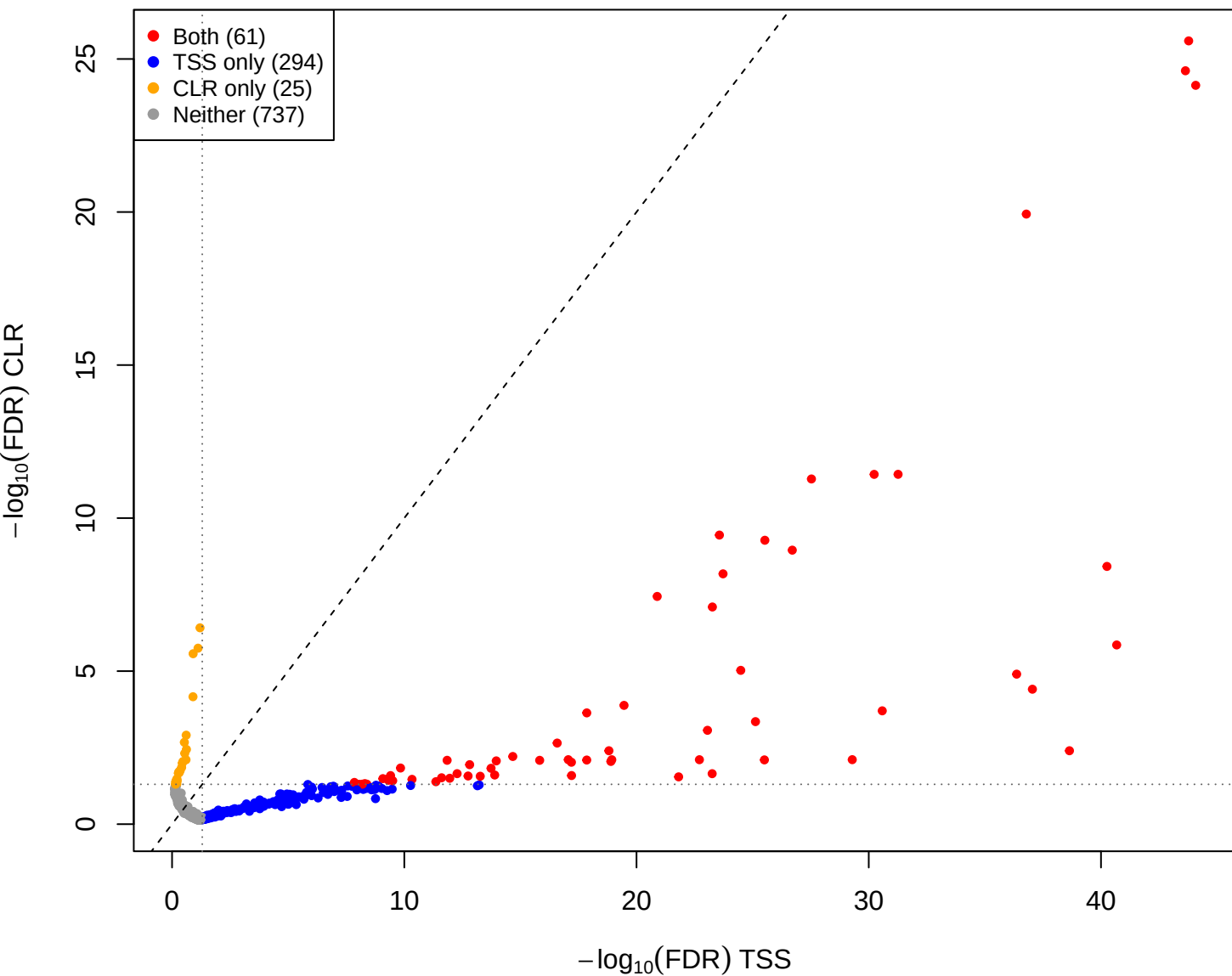
eld vs pup – CLR vs TSS(const=3) (gamma = 1)
