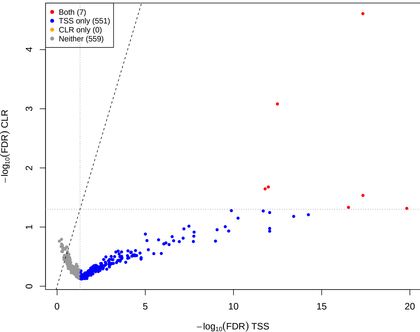
eld vs mage – CLR vs TSS(const=3) (gamma = 1)
