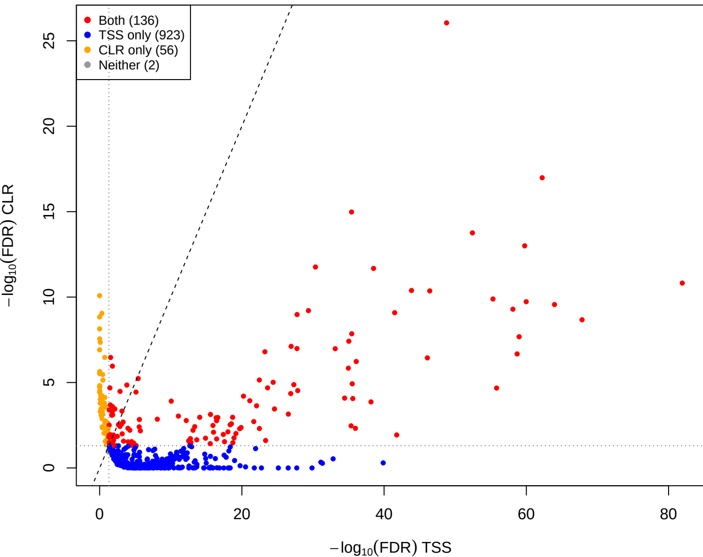
mid vs pup – CLR vs TSS(const=3) (gamma = 1e-05)
