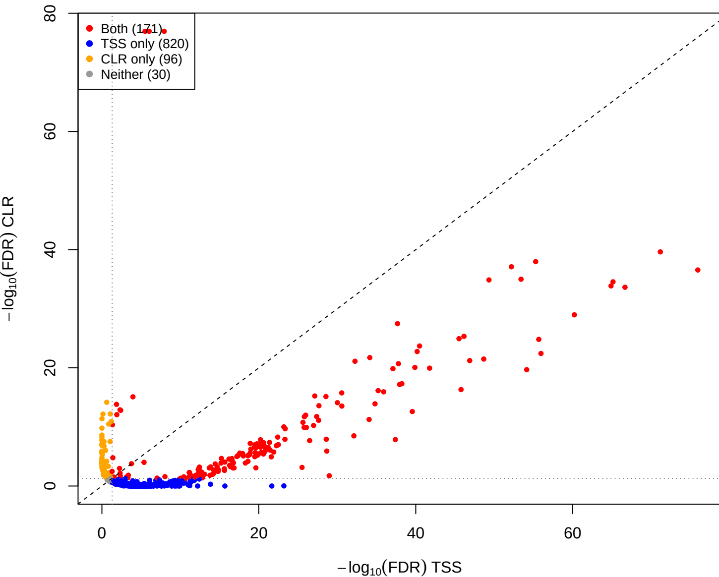
eld vs pup – CLR vs TSS(const=3) (gamma = 1e-05)
