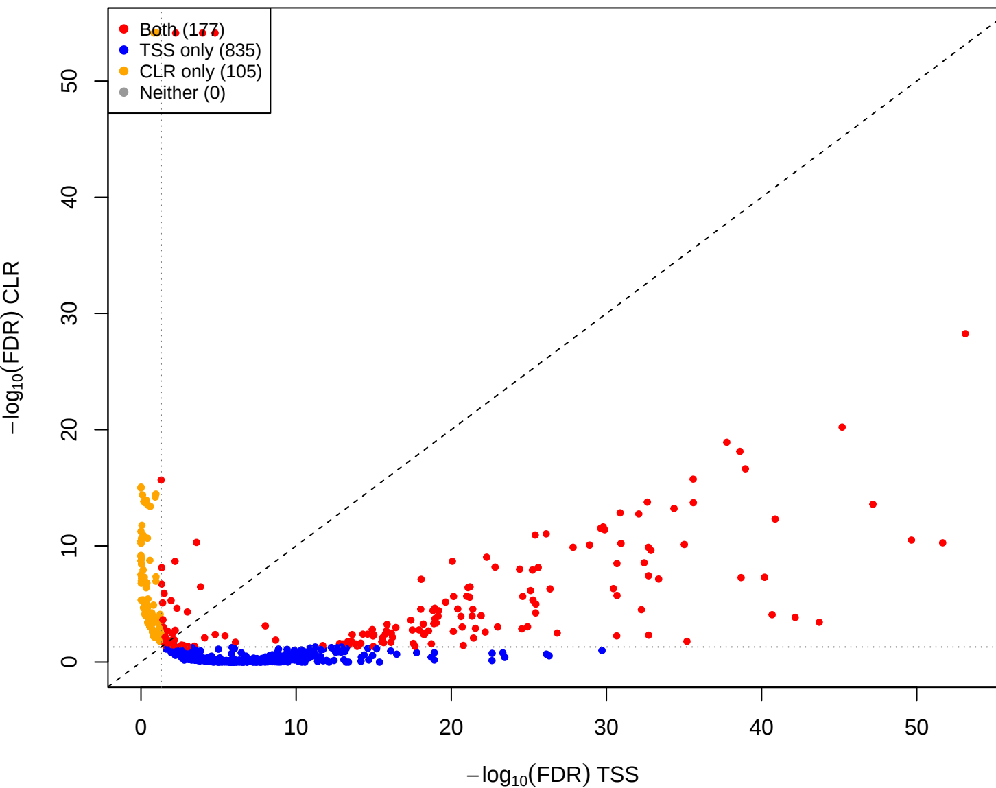
cent vs you – CLR vs TSS(const=3) (gamma = 1e-05)
