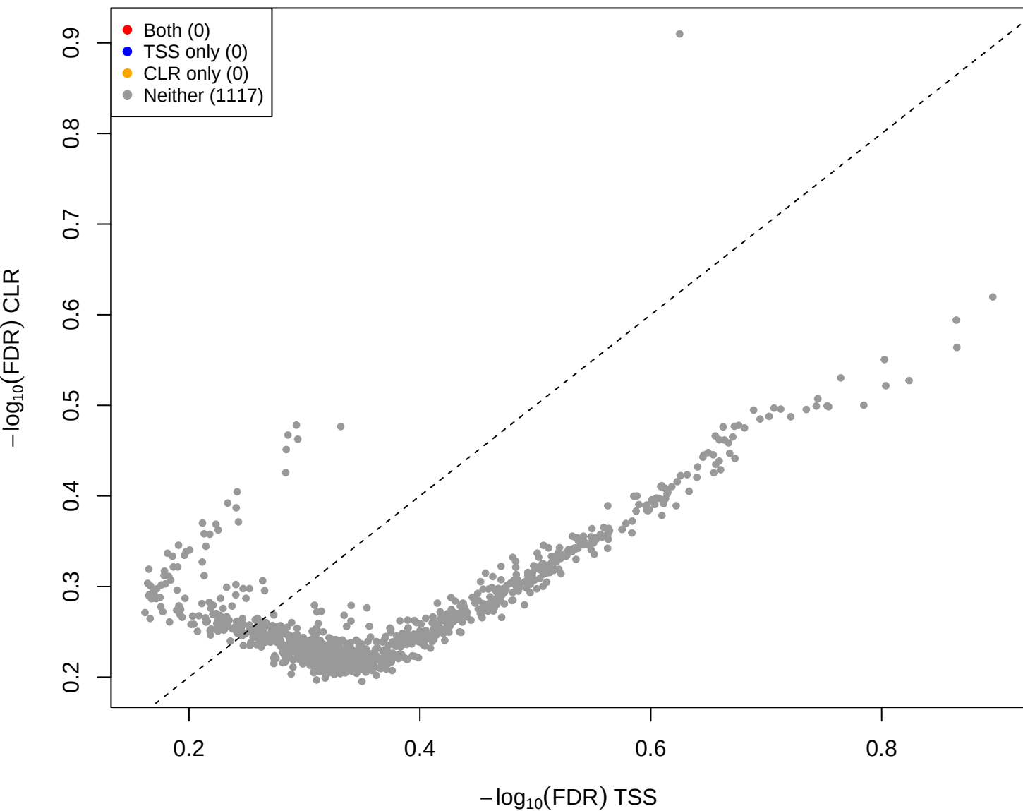
mage vs mid – CLR vs TSS(const=1) (gamma = 2)
