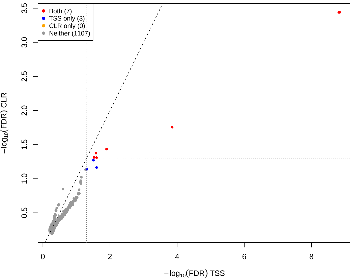
eld vs mid – CLR vs TSS(const=1) (gamma = 2)
