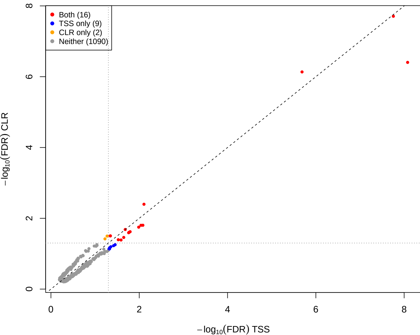
eld vs pup – CLR vs TSS(const=1) (gamma = 2)
