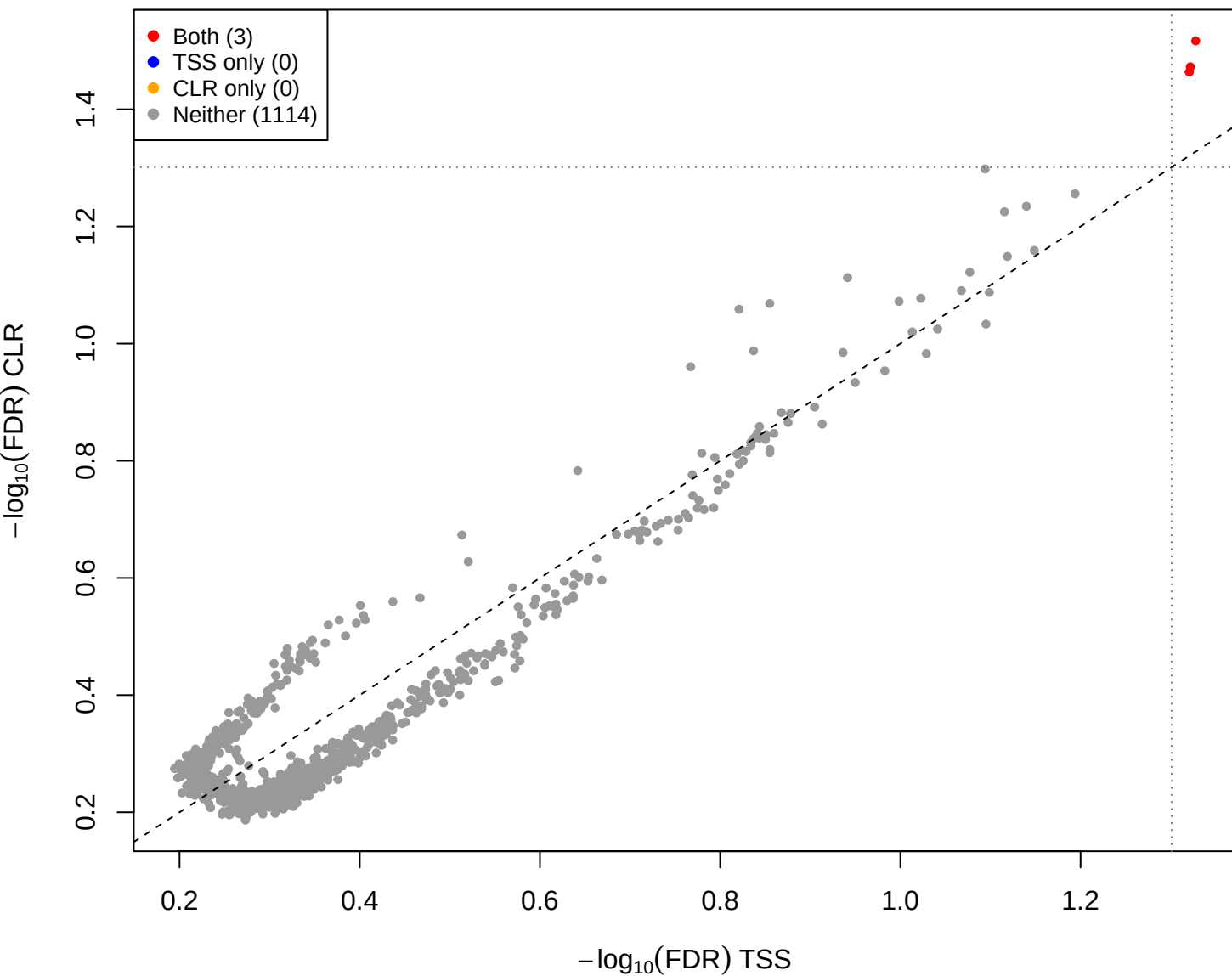
cent vs mage - CLR vs TSS(const=1) (gamma = 2)
