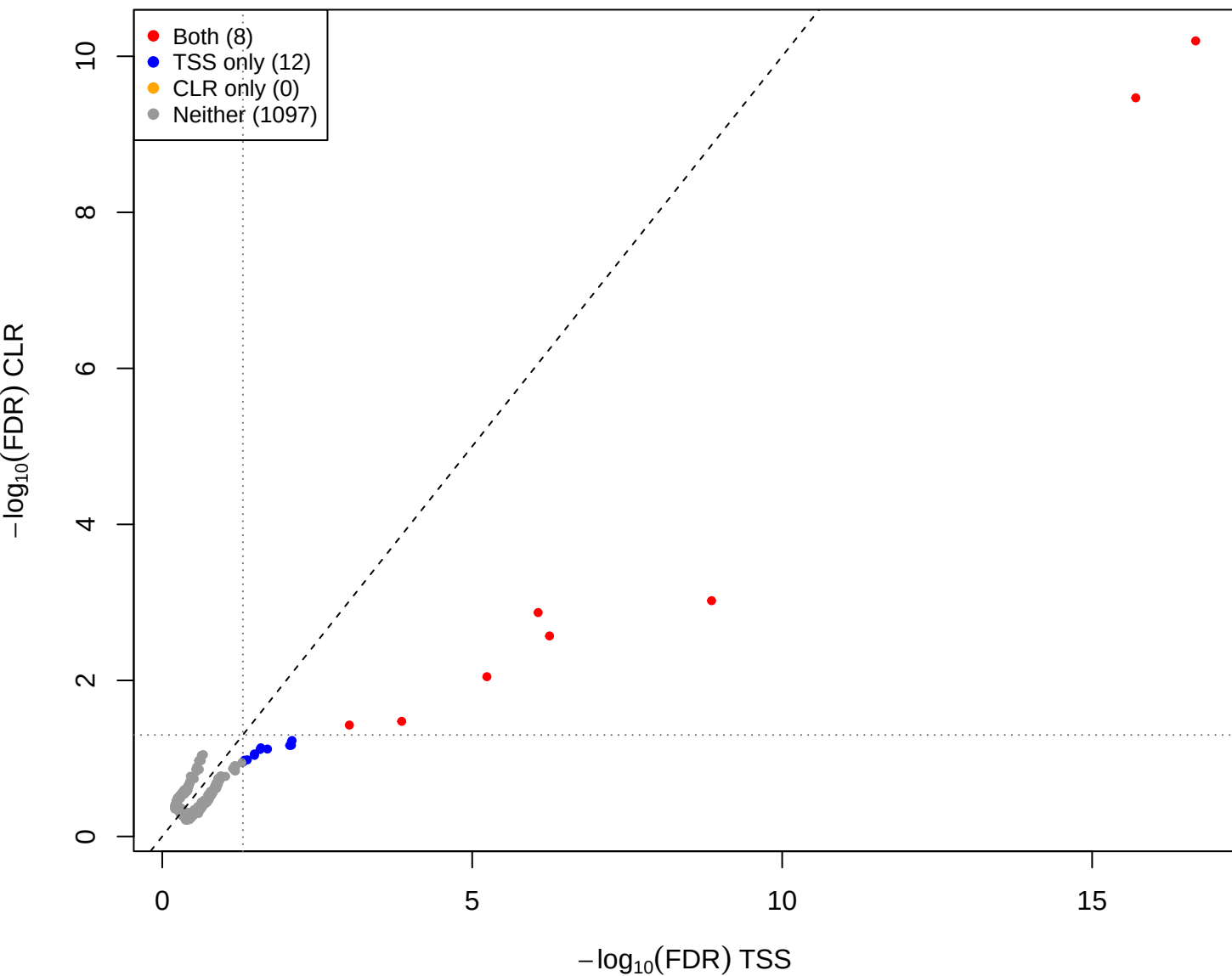
cent vs kin – CLR vs TSS(const=1) (gamma = 2)
