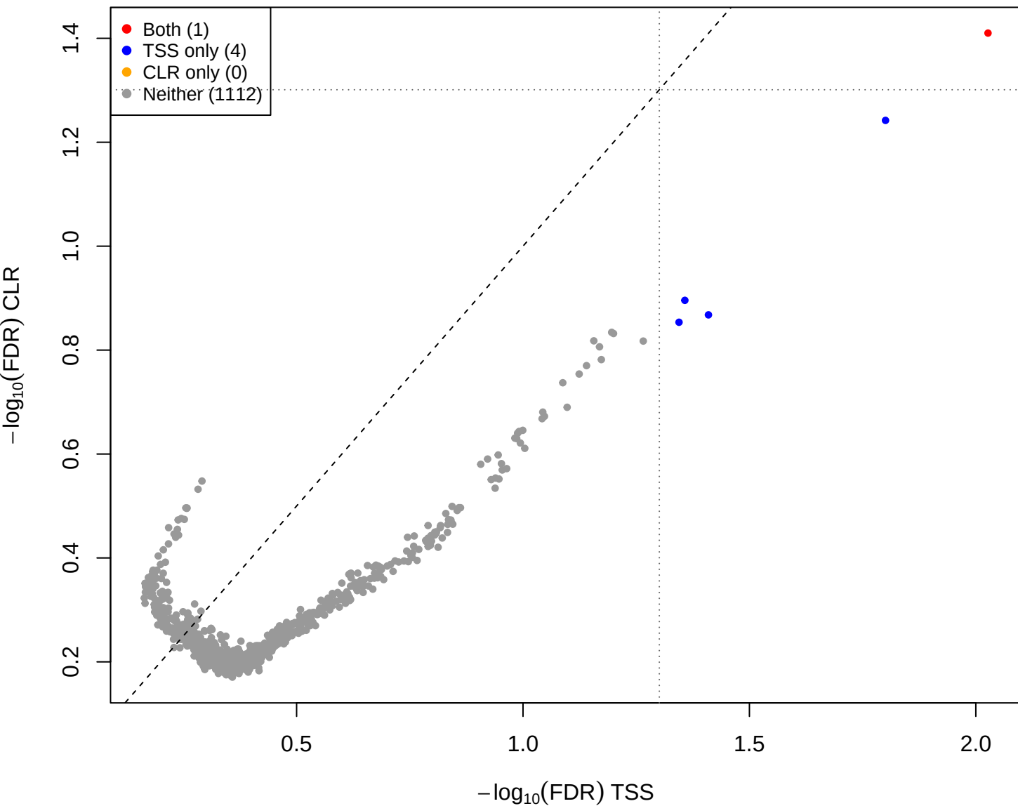
eld vs mage – CLR vs TSS(const=1) (gamma = 2)
