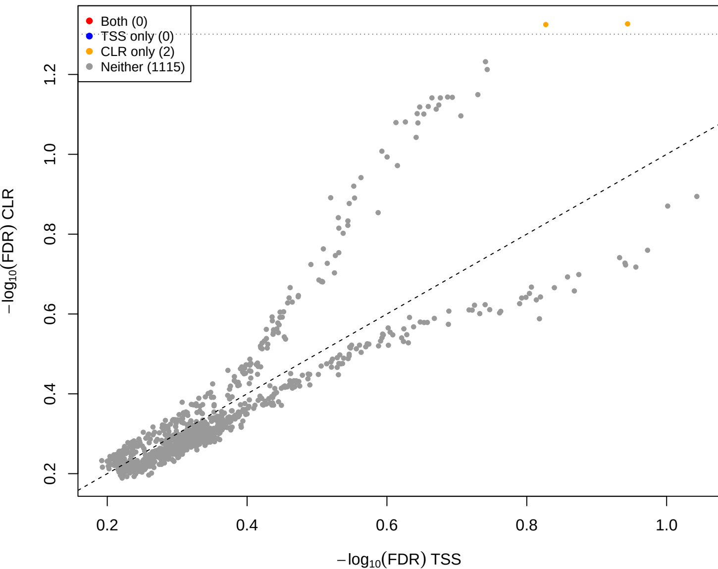
mage vs you – CLR vs TSS(const=1) (gamma = 2)
