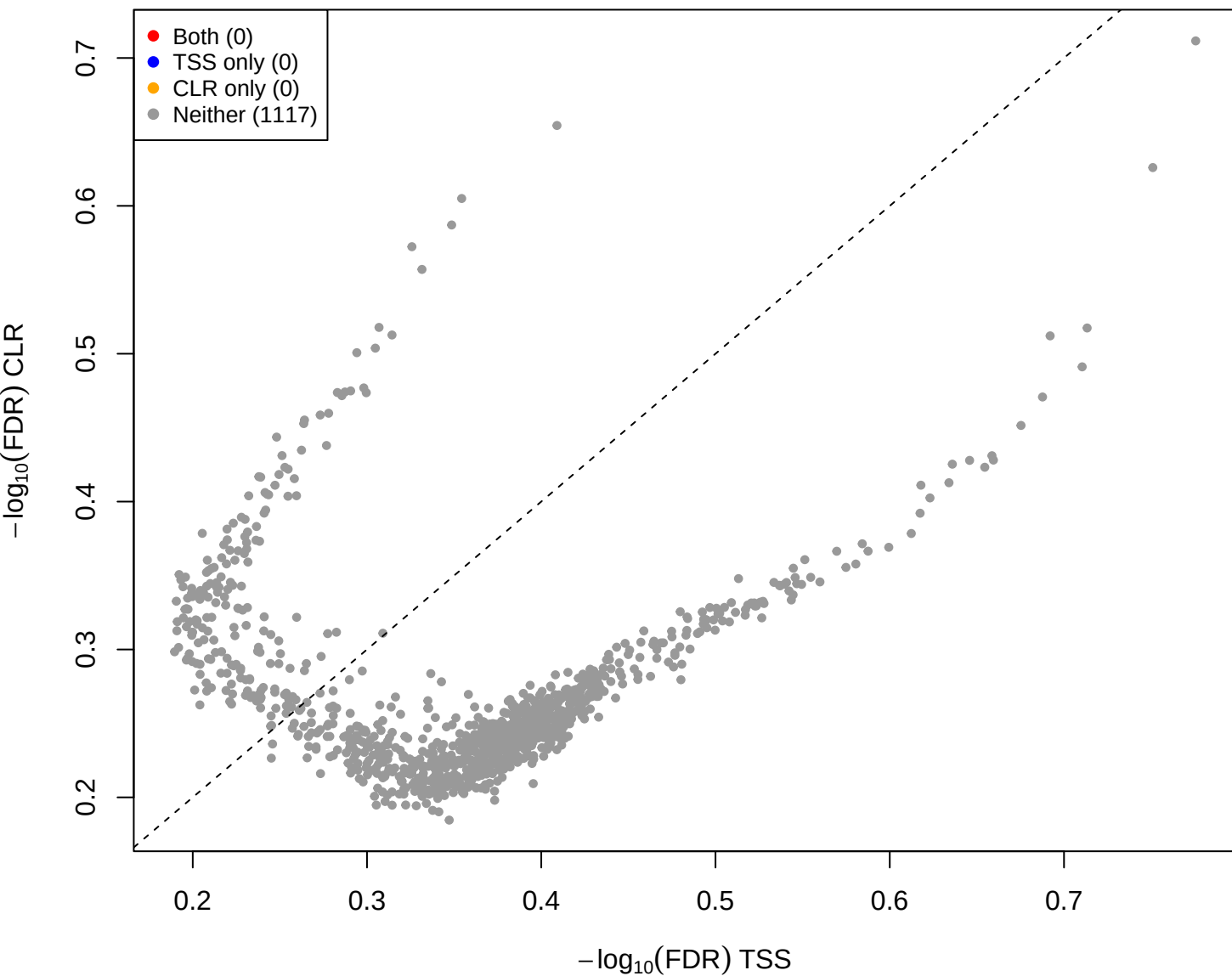
eld vs you – CLR vs TSS(const=1) (gamma = 2)
