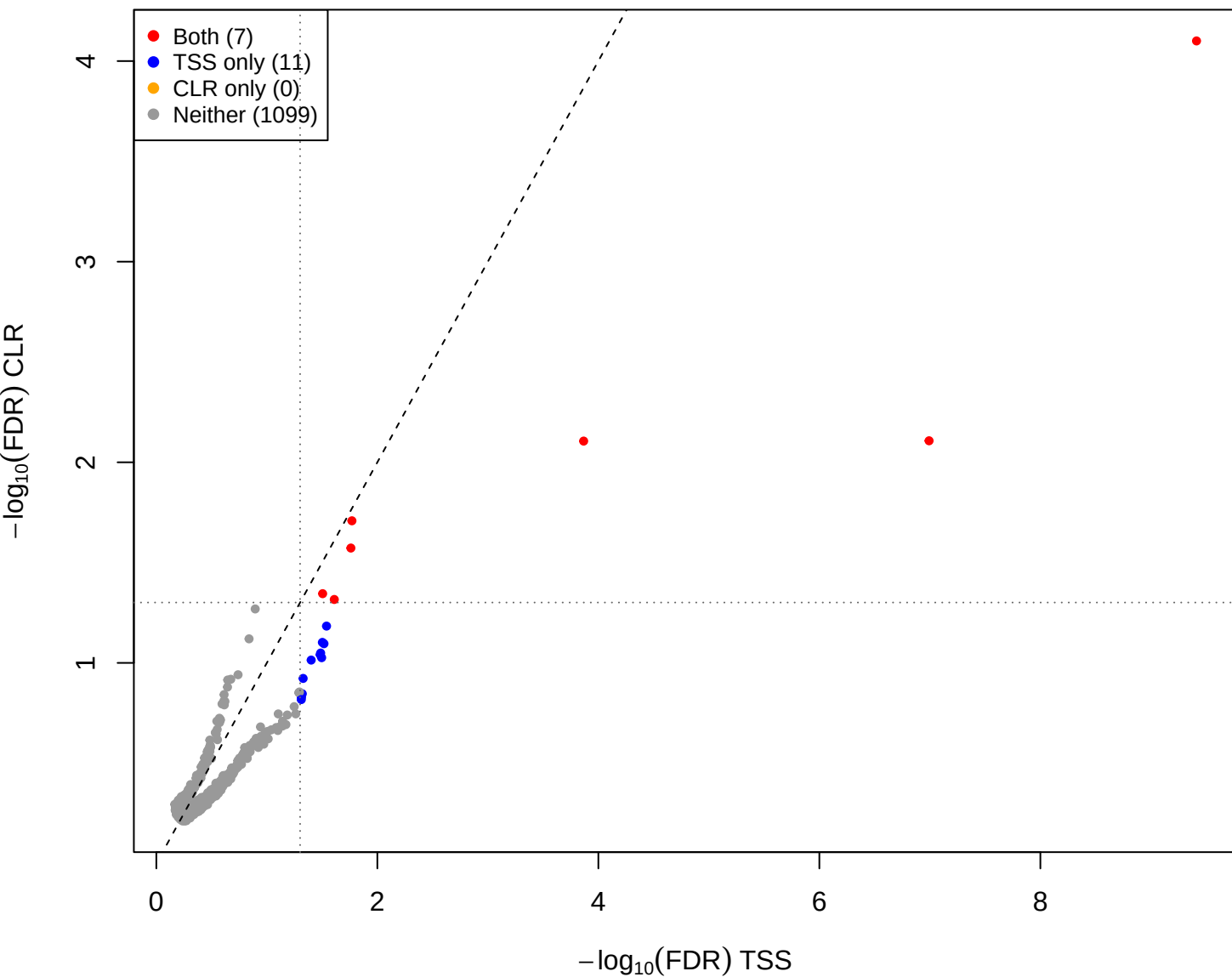
eld vs kin - CLR vs TSS(const=1) (gamma = 2)
