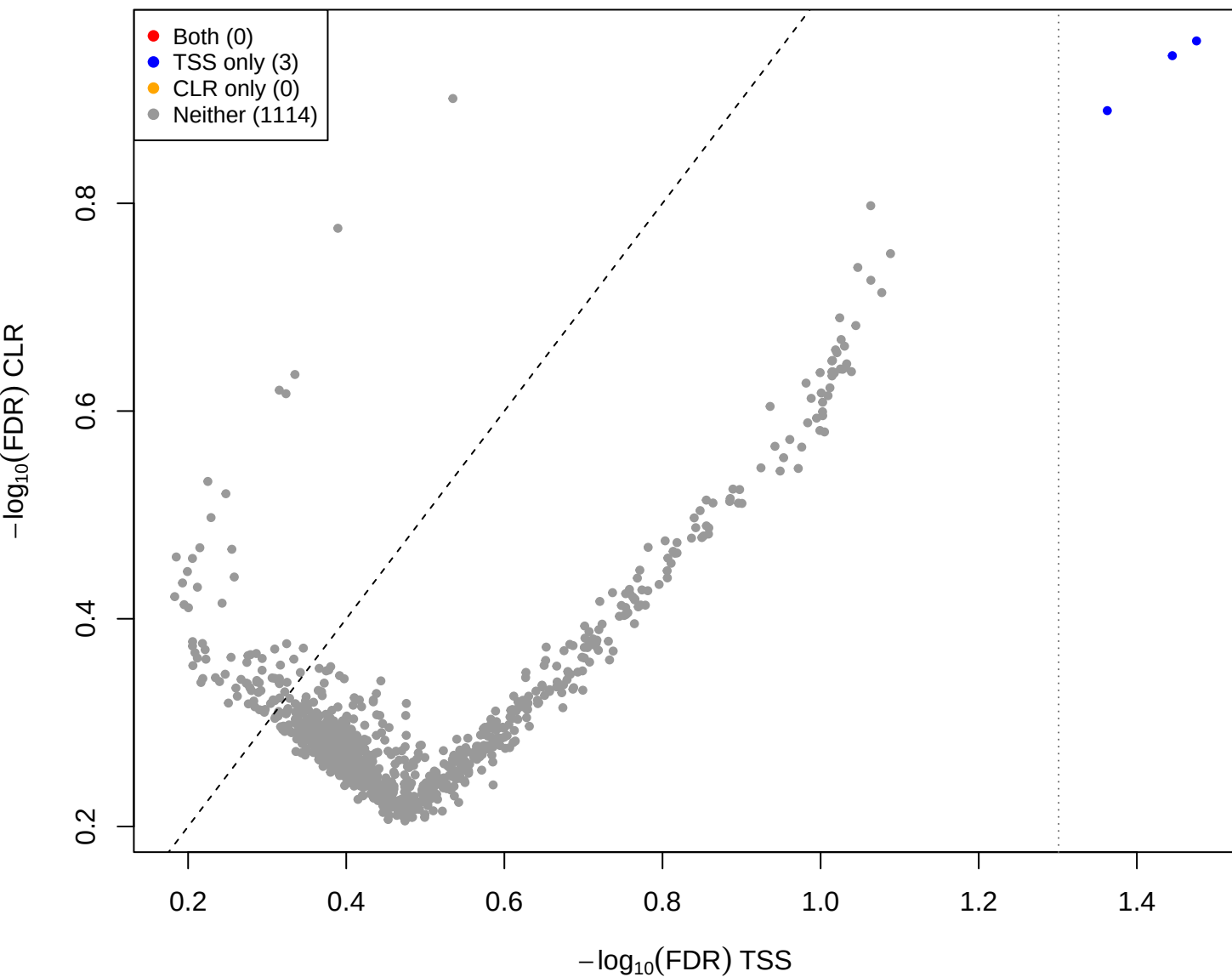
kin vs mid – CLR vs TSS(const=1) (gamma = 2)
