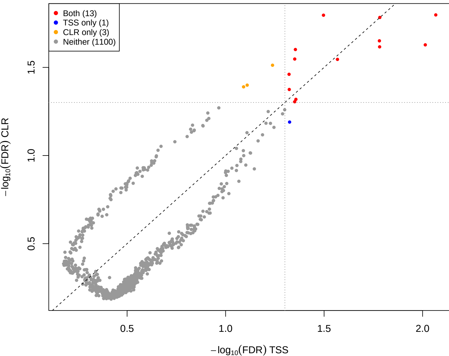
kin vs you – CLR vs TSS(const=1) (gamma = 2)
