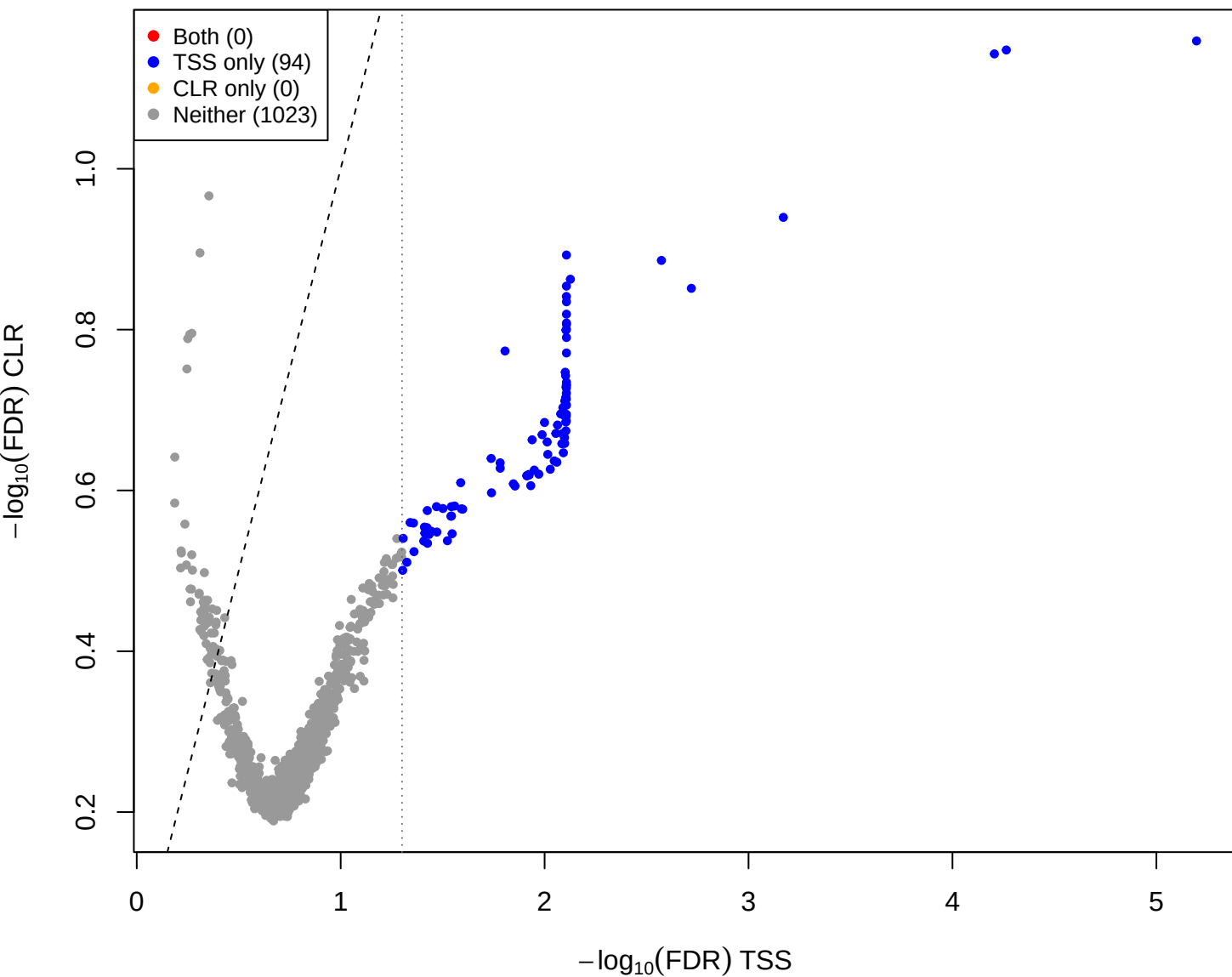
cent vs mage - CLR vs TSS(const=3) (gamma = 2)
