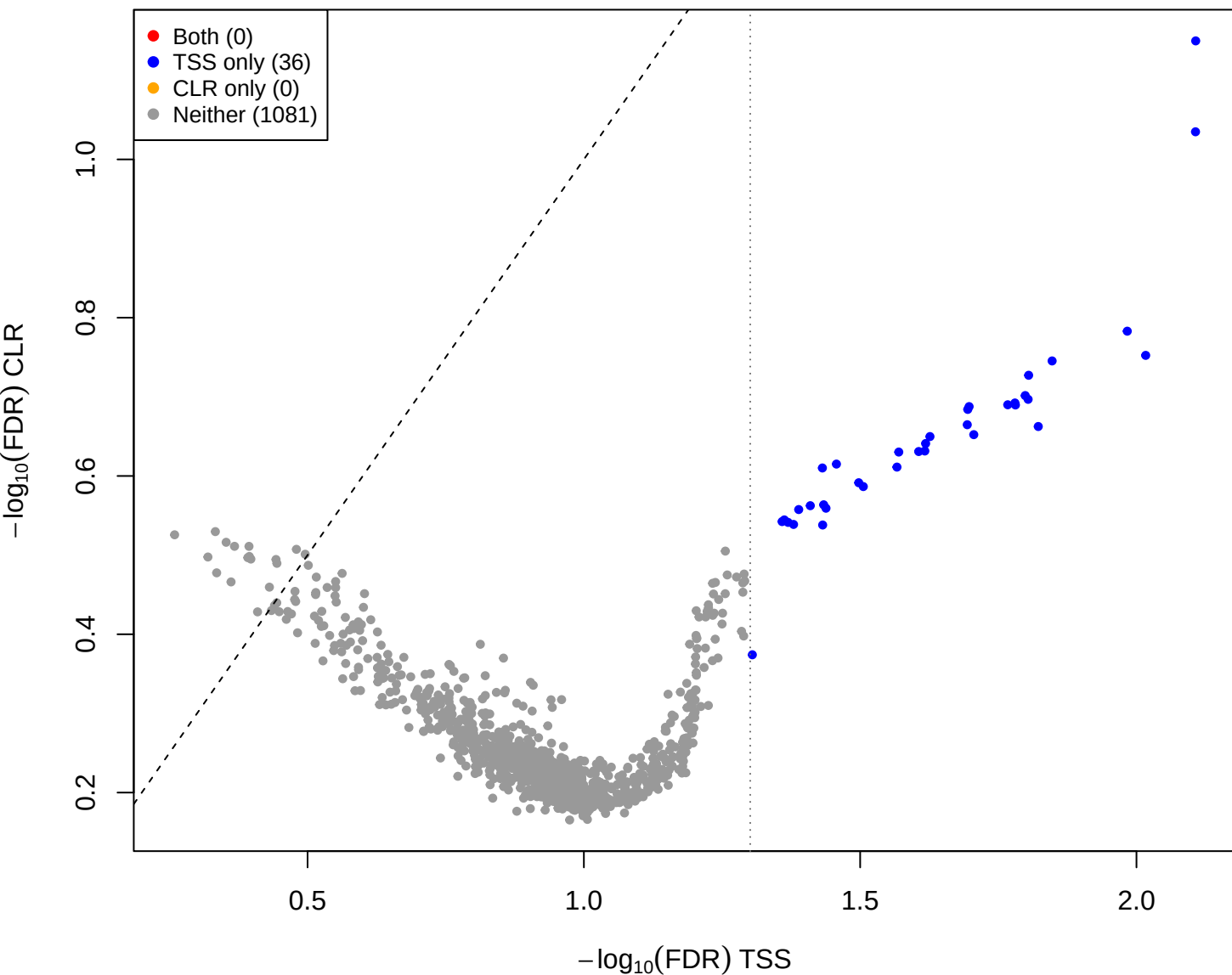
eld vs mage – CLR vs TSS(const=3) (gamma = 2)
