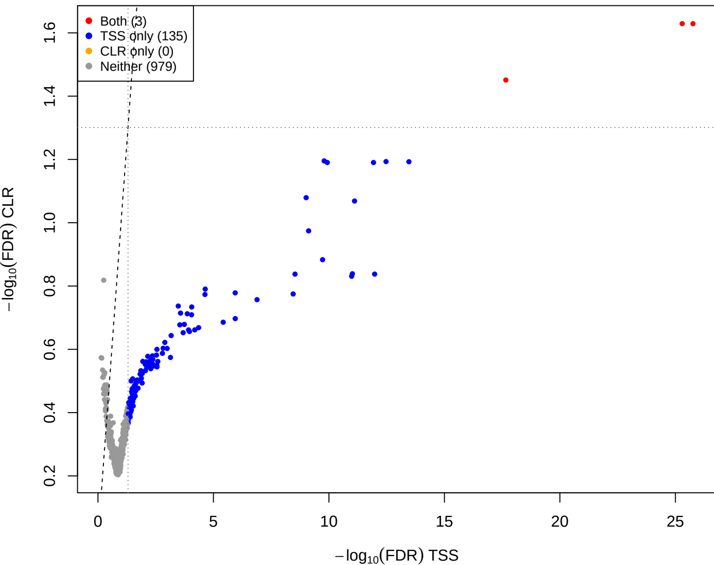
eld vs mid – CLR vs TSS(const=3) (gamma = 2)
