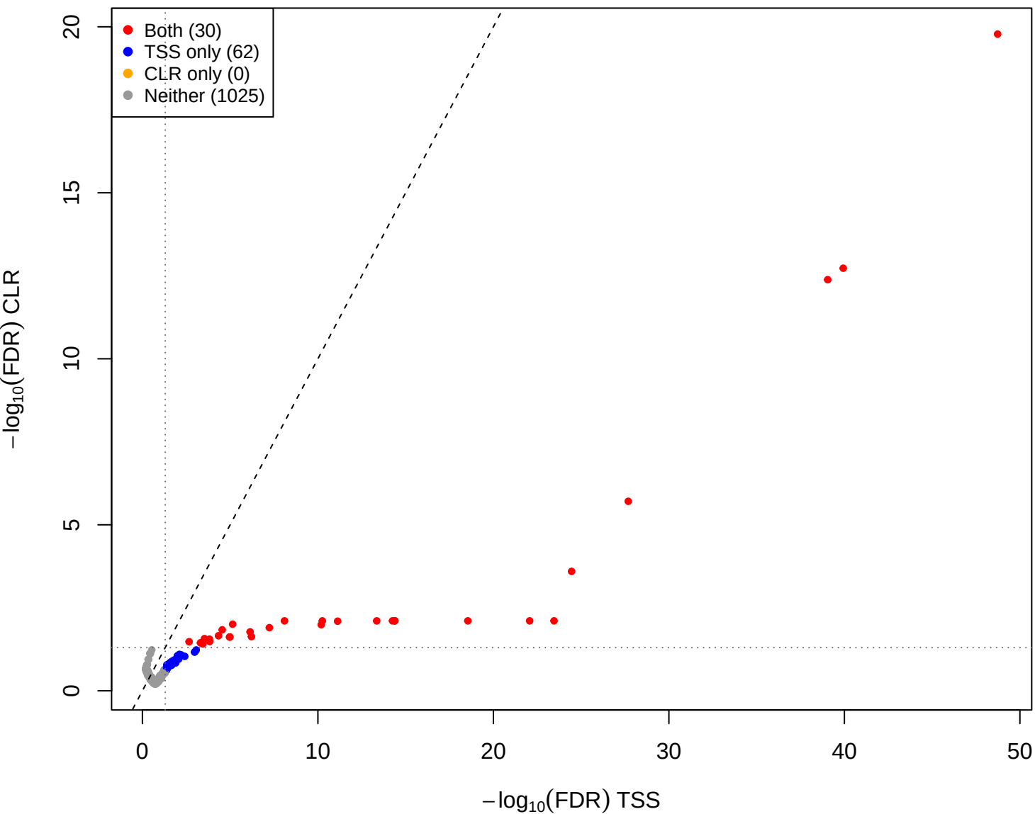
cent vs pup – CLR vs TSS(const=3) (gamma = 2)
