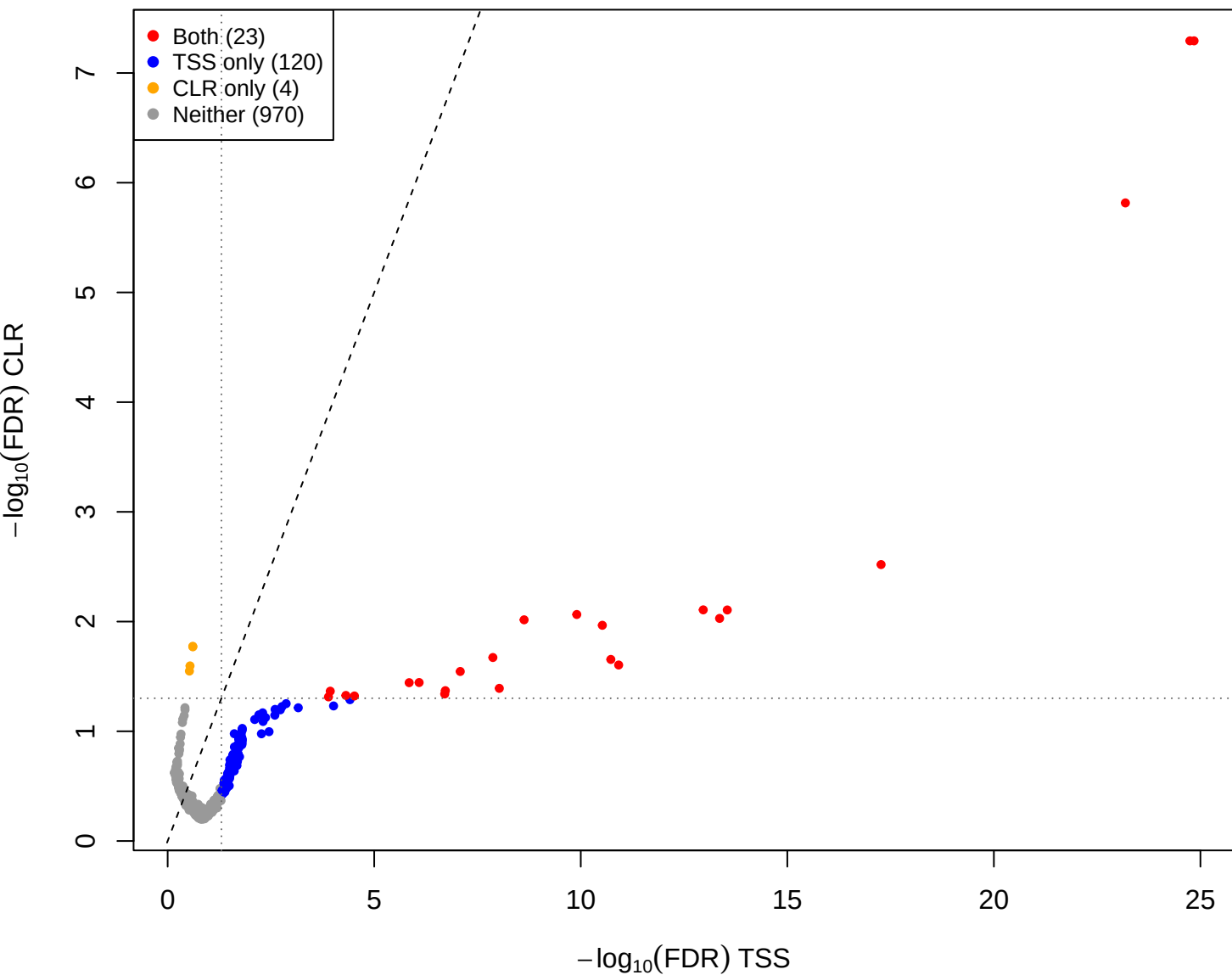
eld vs pup – CLR vs TSS(const=3) (gamma = 2)
