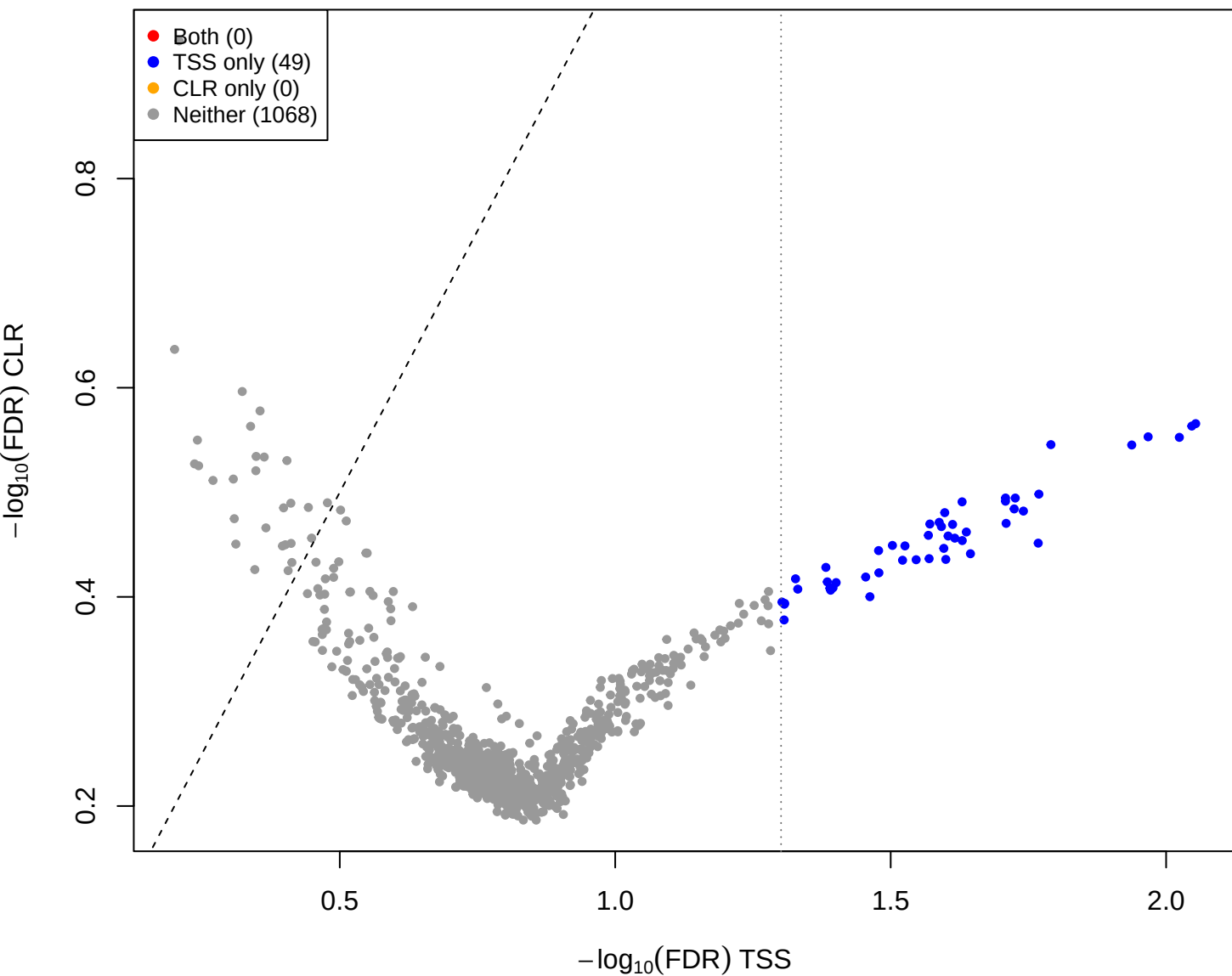
kin vs mage – CLR vs TSS(const=3) (gamma = 2)
