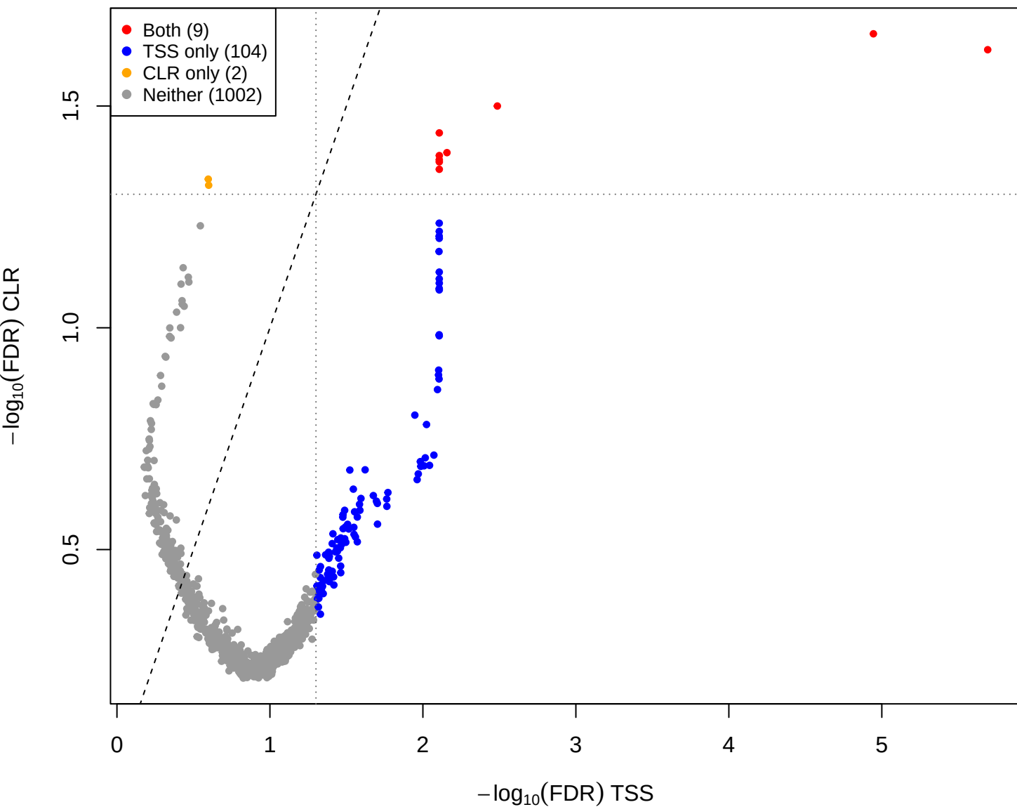
cent vs you - CLR vs TSS(const=3) (gamma = 2)
