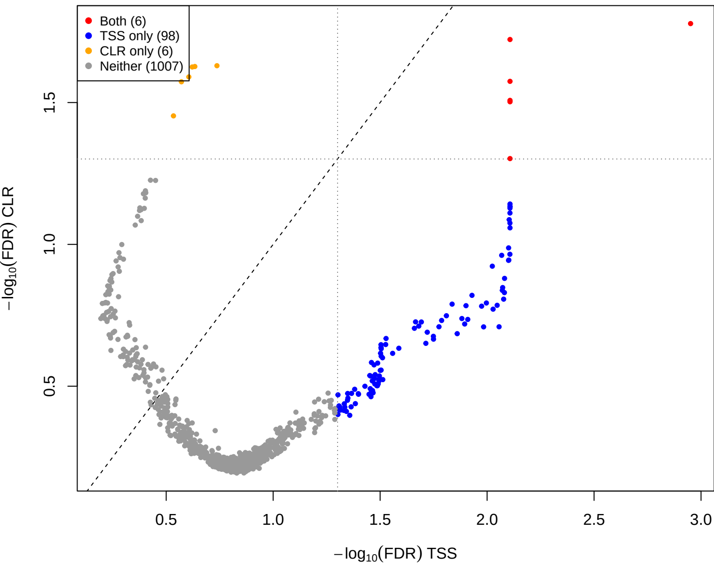
kin vs you – CLR vs TSS(const=3) (gamma = 2)
