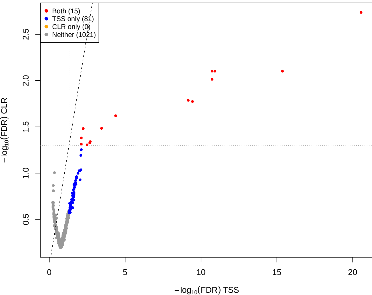
cent vs mid – CLR vs TSS(const=3) (gamma = 2)
