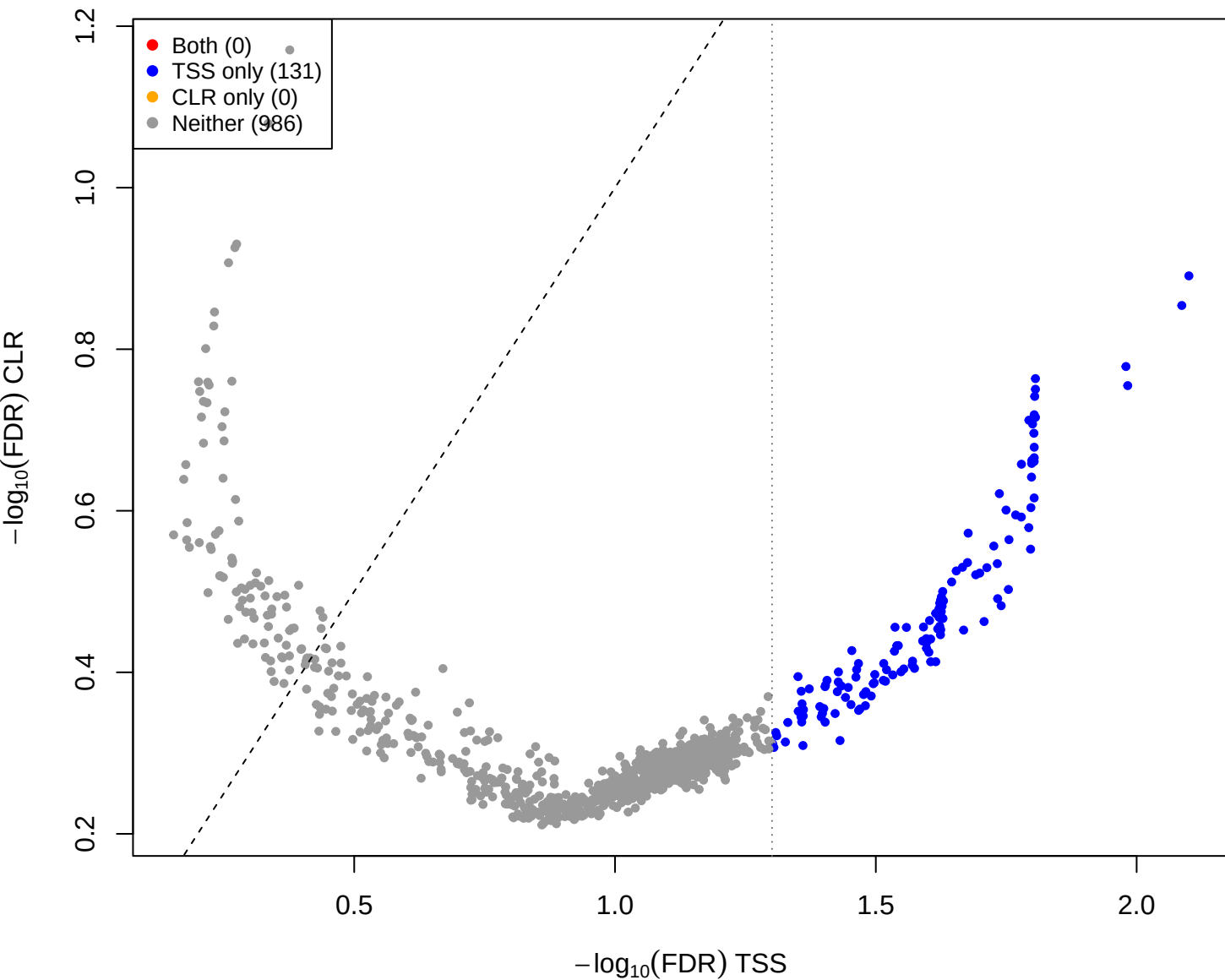
mage vs you – CLR vs TSS(const=3) (gamma = 2)
