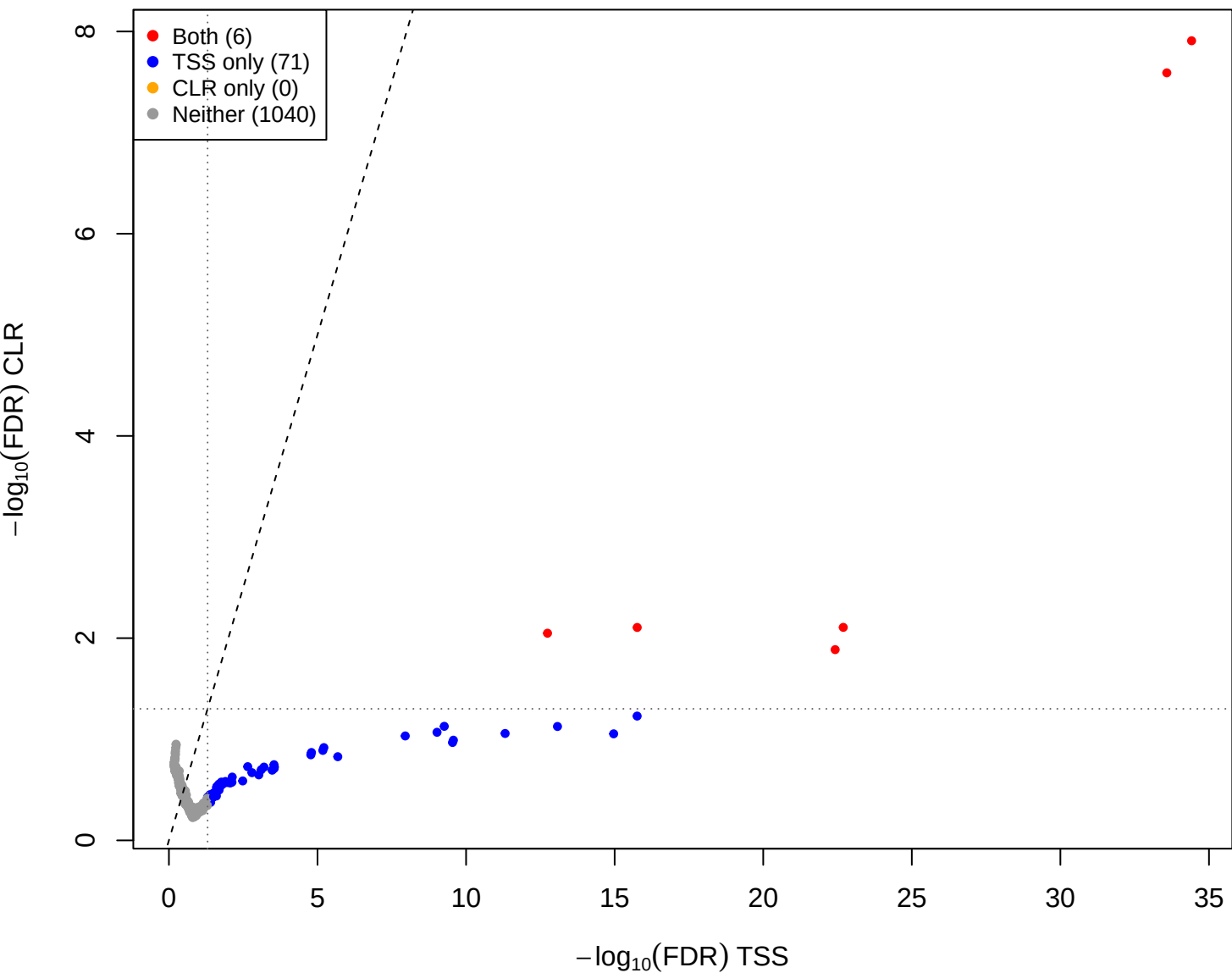
cent vs kin – CLR vs TSS(const=3) (gamma = 2)
