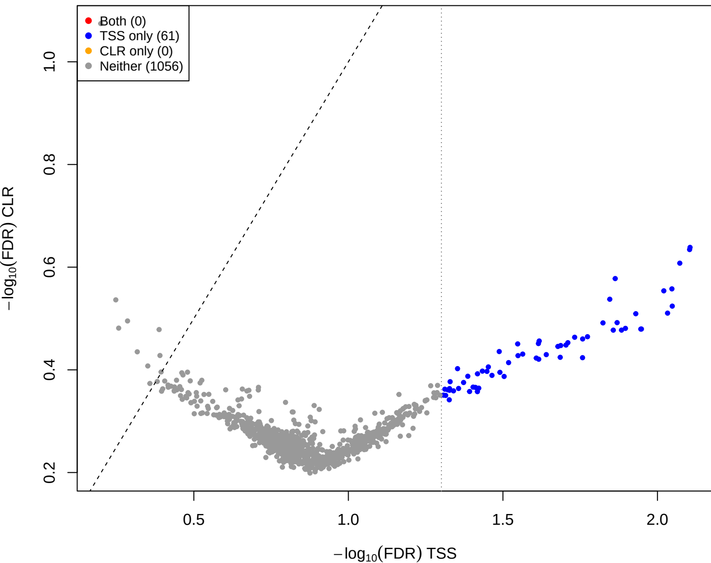
mage vs mid – CLR vs TSS(const=3) (gamma = 2)
