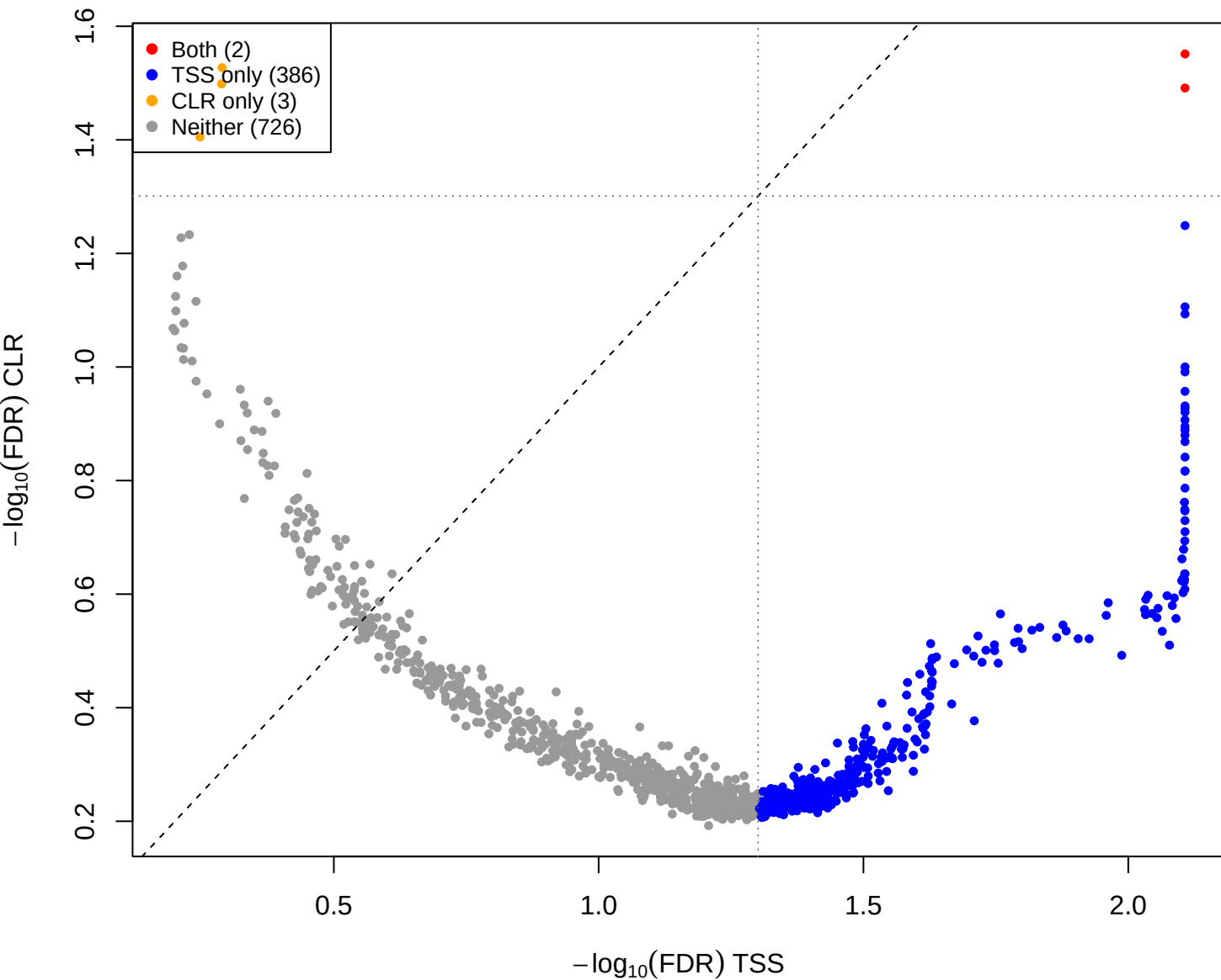
cent vs you - CLR vs TSS(const=4) (gamma = 2)
