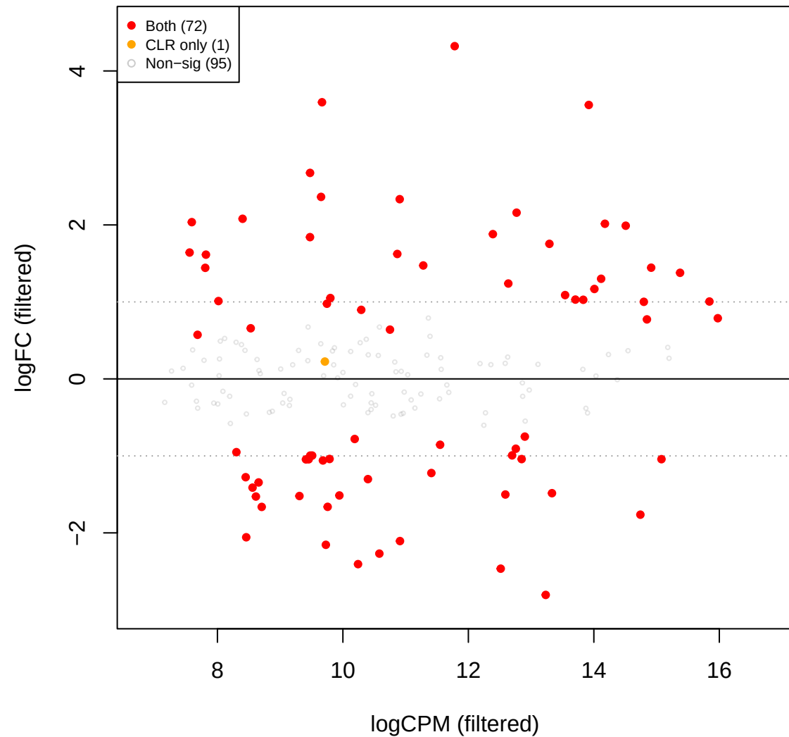
pup vs mid – edgeR TMMwsp FILTERED (207 OTUs, CLR sig overlay)
