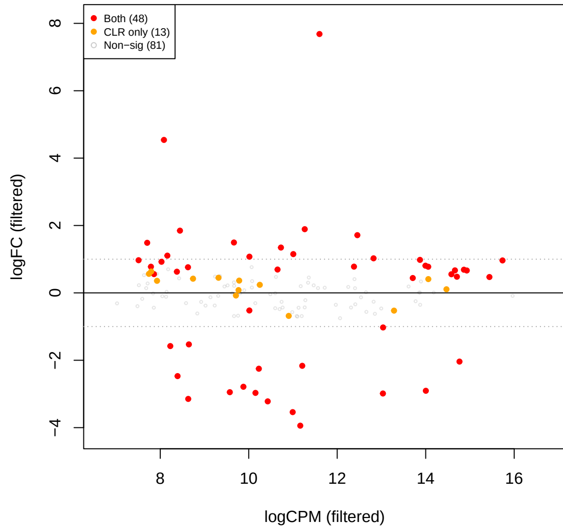
pup vs mage – edgeR TMMwsp FILTERED (218 OTUs, CLR sig ov
