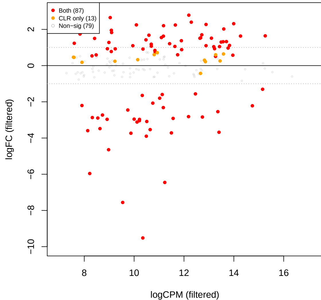
mage vs cent – edgeR TMMwsp FILTERED (251 OTUs, CLR sig ov
