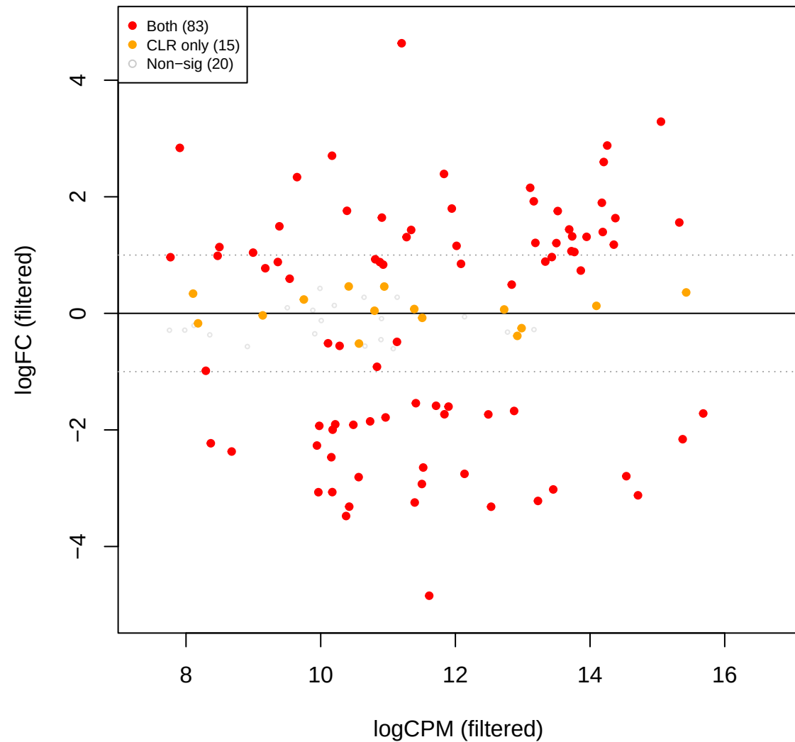
pup vs cent – edgeR TMMwsp FILTERED (173 OTUs, CLR sig ov
