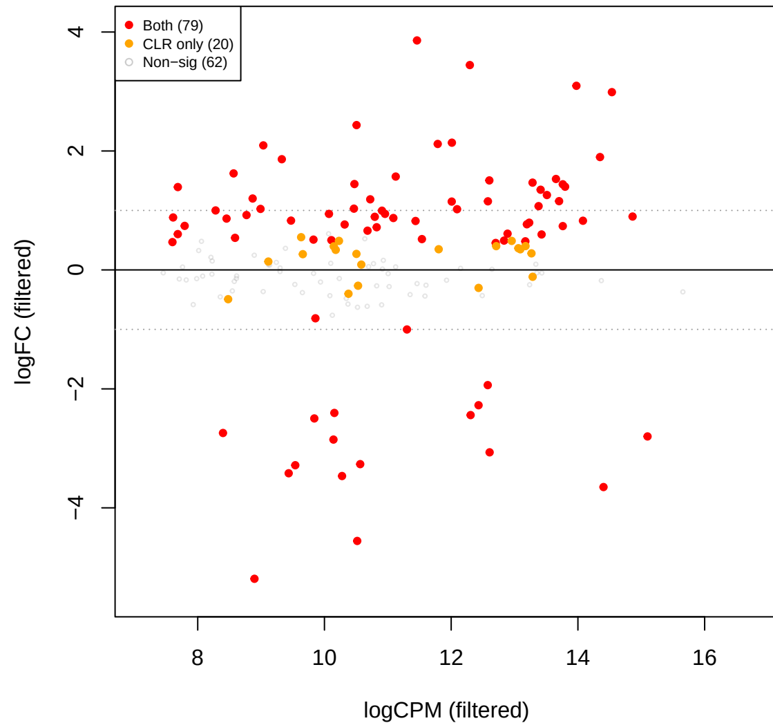
mid vs cent – edgeR TMMwsp FILTERED (238 OTUs, CLR sig overlay)
