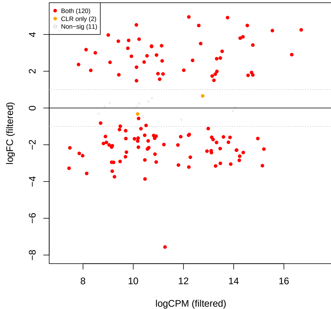
pup vs you – edgeR TMMwsp FILTERED (165 OTUs, CLR sig overlay)
