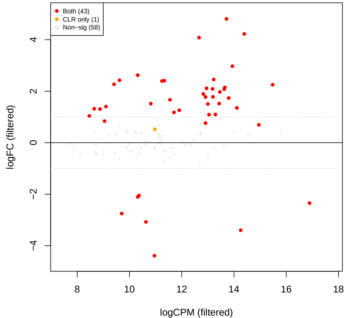
mage vs eld – edgeR TMMwsp FILTERED (173 OTUs, CLR sig ov
