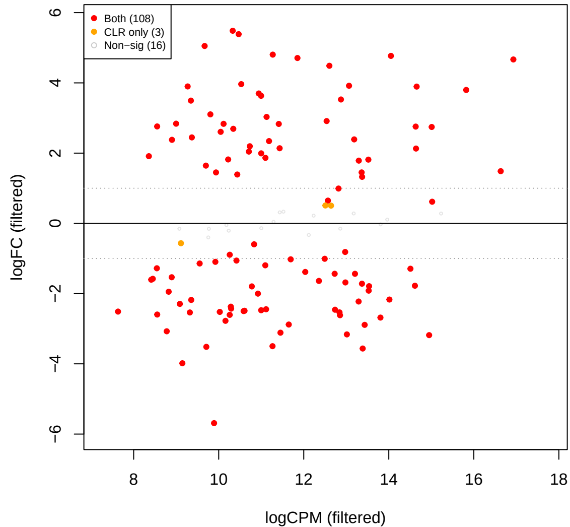
kin vs you – edgeR TMMwsp FILTERED (160 OTUs, CLR sig over
