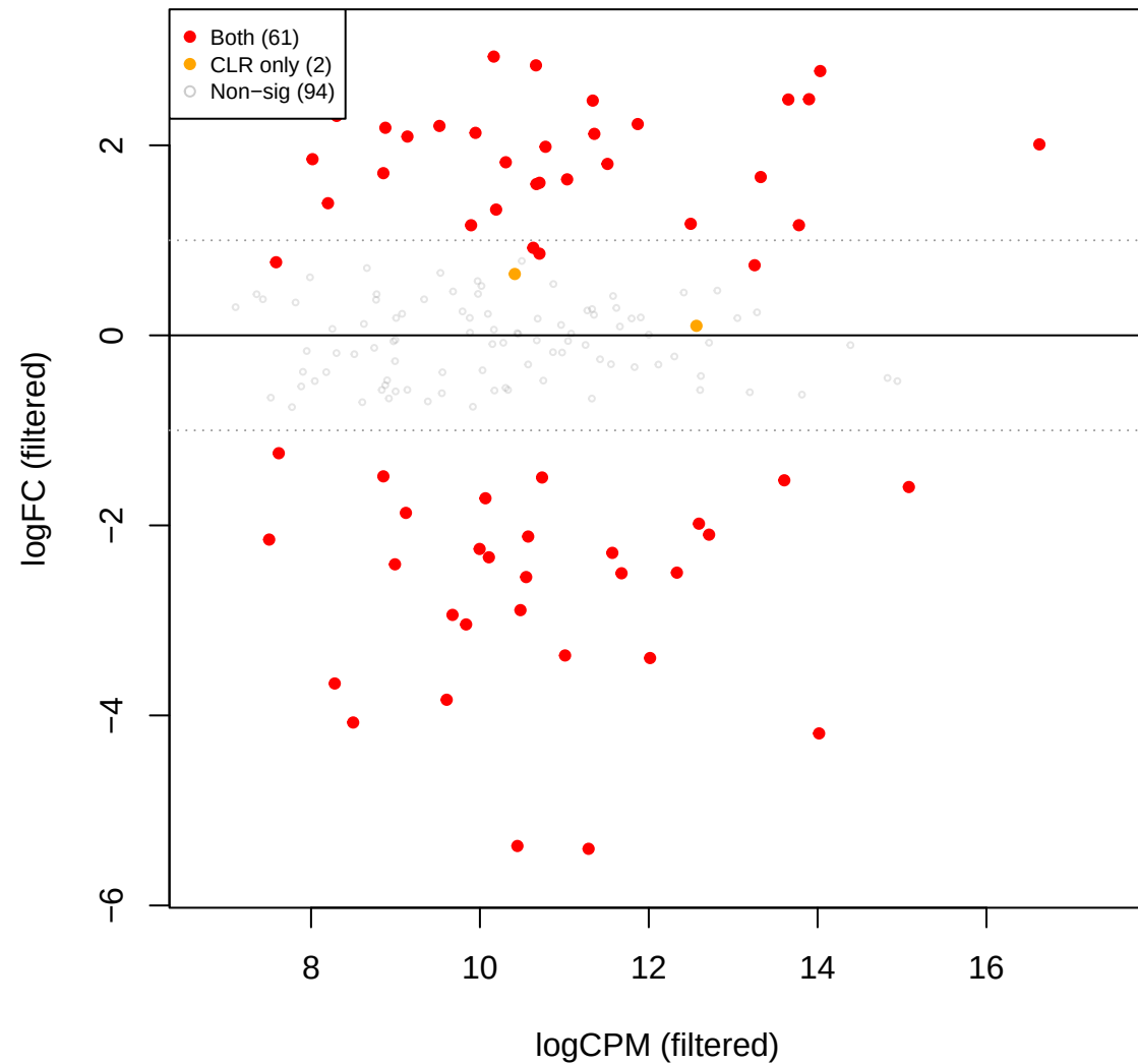
eld vs cent – edgeR TMMwsp FILTERED (252 OTUs, CLR sig over
