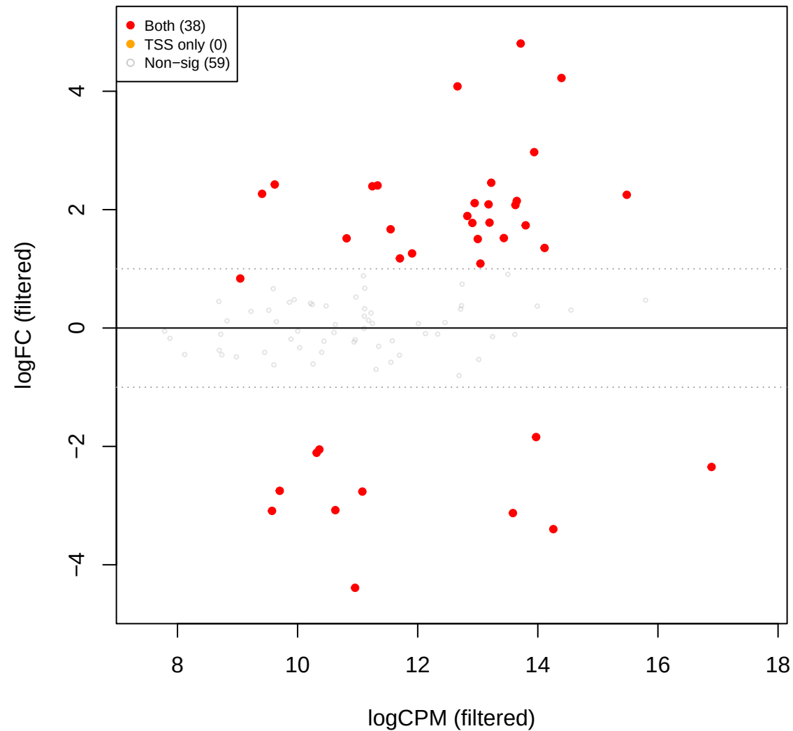
mage vs eld – edgeR TMMwsp FILTERED (173 OTUs, TSS sig ov
