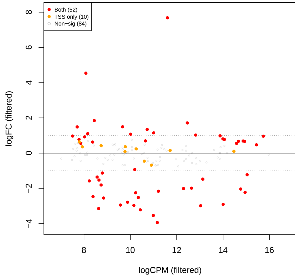
pup vs mage – edgeR TMMwsp FILTERED (218 OTUs, TSS sig ov
