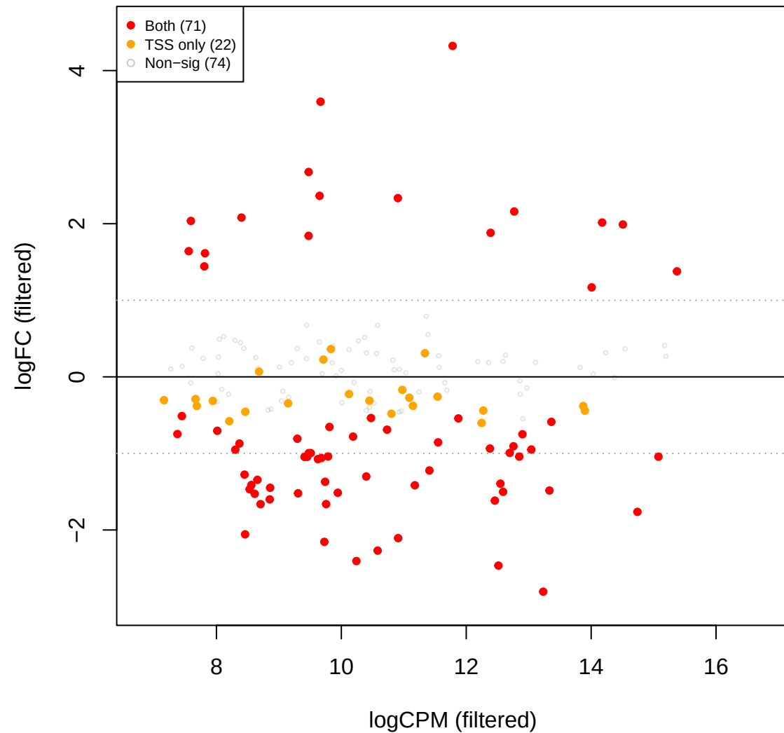
pup vs mid – edgeR TMMwsp FILTERED (207 OTUs, TSS sig over
