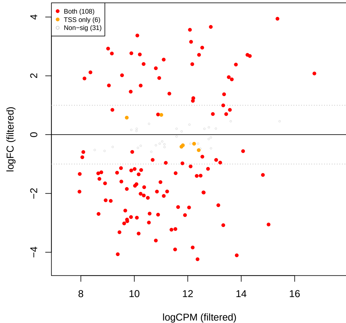
you vs cent – edgeR TMMwsp FILTERED (190 OTUs, TSS sig over
