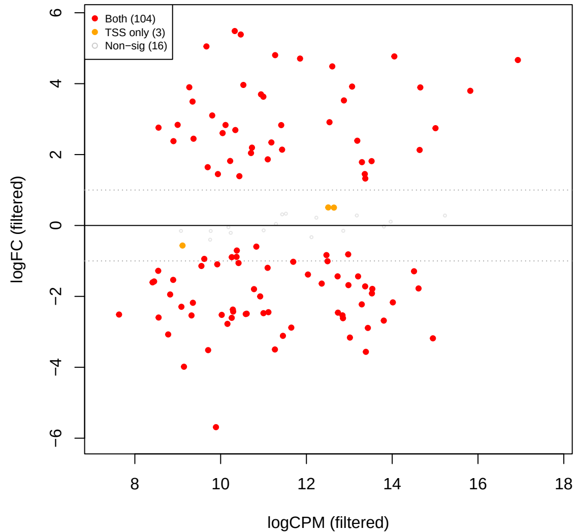
kin vs you – edgeR TMMwsp FILTERED (160 OTUs, TSS sig over
