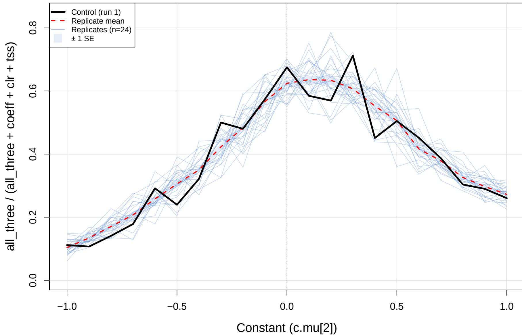
coefficient.sm vs CLR(std) vs TSS – cent_vs_mage (gamma=0.3) Robustness (1 = all agree, 0 = max disagreement)
