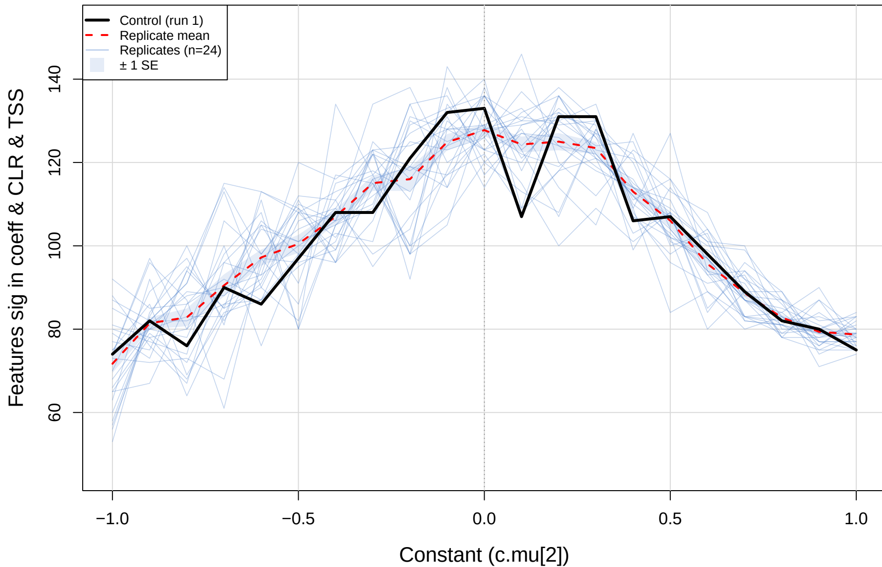
coefficient.sm vs CLR(std) vs TSS – cent_vs_mage (gamma=0.3) Three-way agreement count
