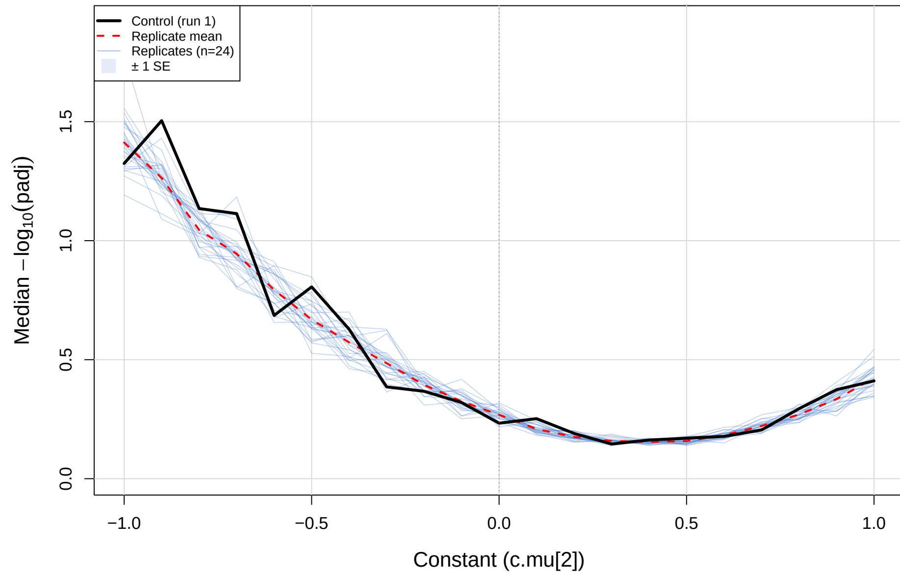
coefficient.sm vs CLR(std) vs TSS – cent_vs_mage (gamma=0.3) Median -\log_{10}(\text{padj}) coefficient model
