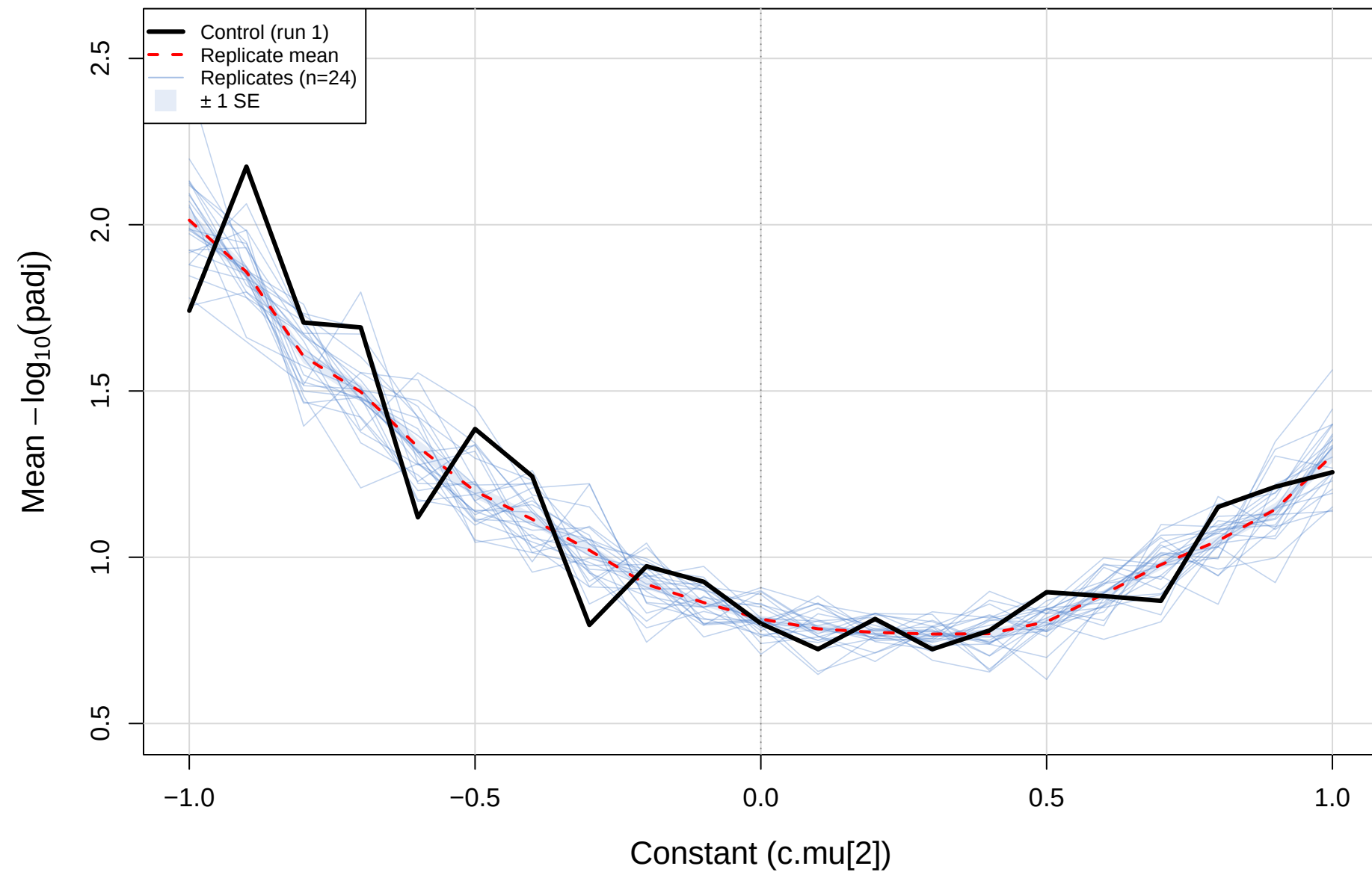
coefficient.sm vs CLR(std) vs TSS – cent_vs_mage (gamma=0.3) Mean -\log_{10}(\text{padj}) coefficient model
