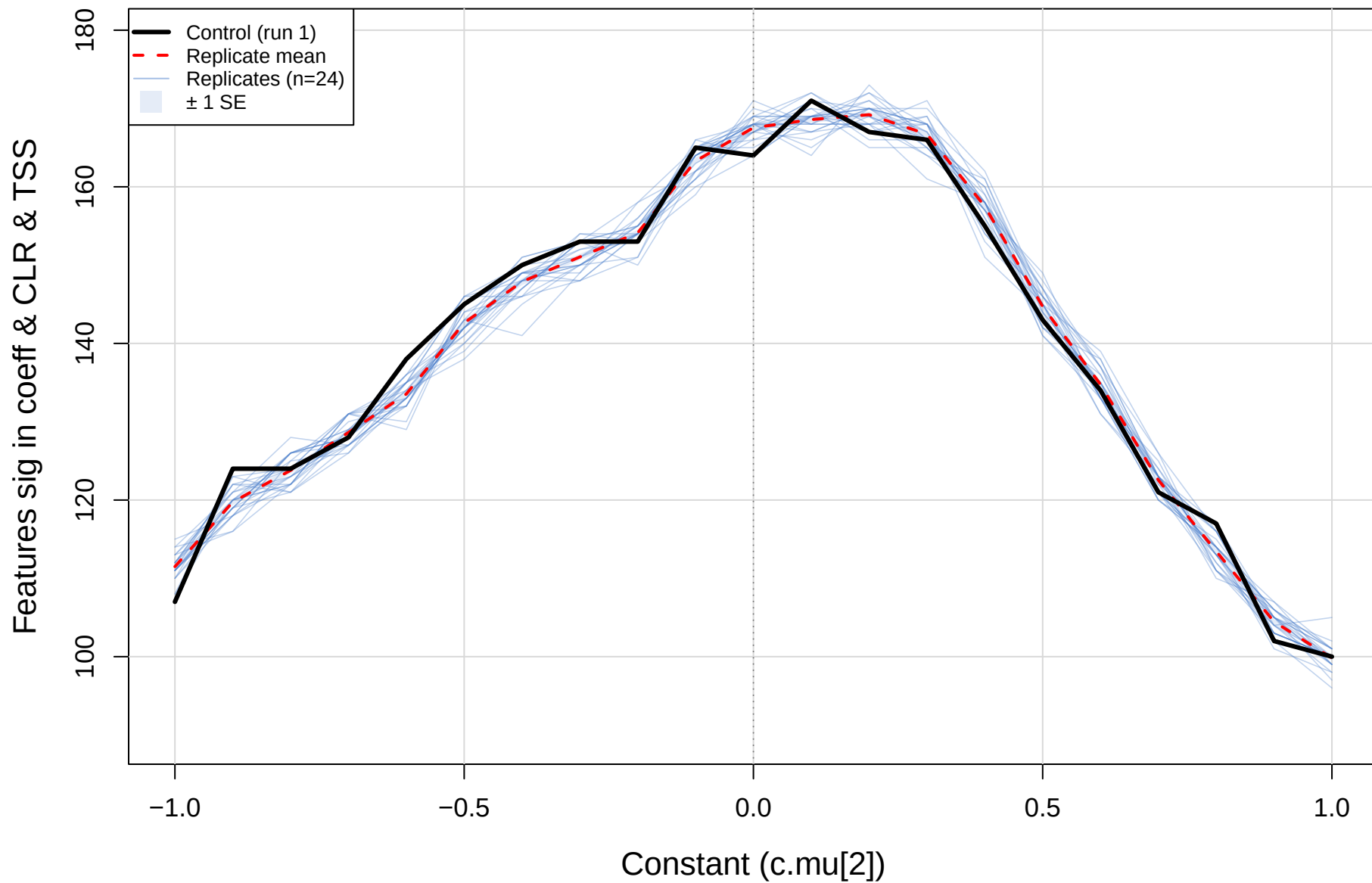
coefficient.sm vs CLR(std) vs TSS - cent_vs_mage (gamma=1e-04) Three-way agreement count
