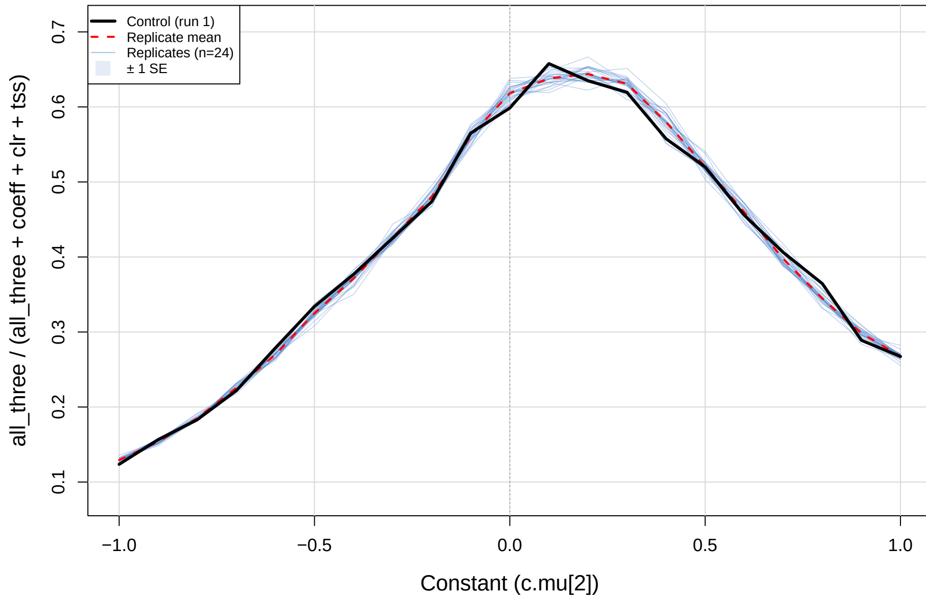
coefficient.sm vs CLR(std) vs TSS - cent_vs_mage (gamma=1e-04) Robustness (1 = all agree, 0 = max disagreement)
