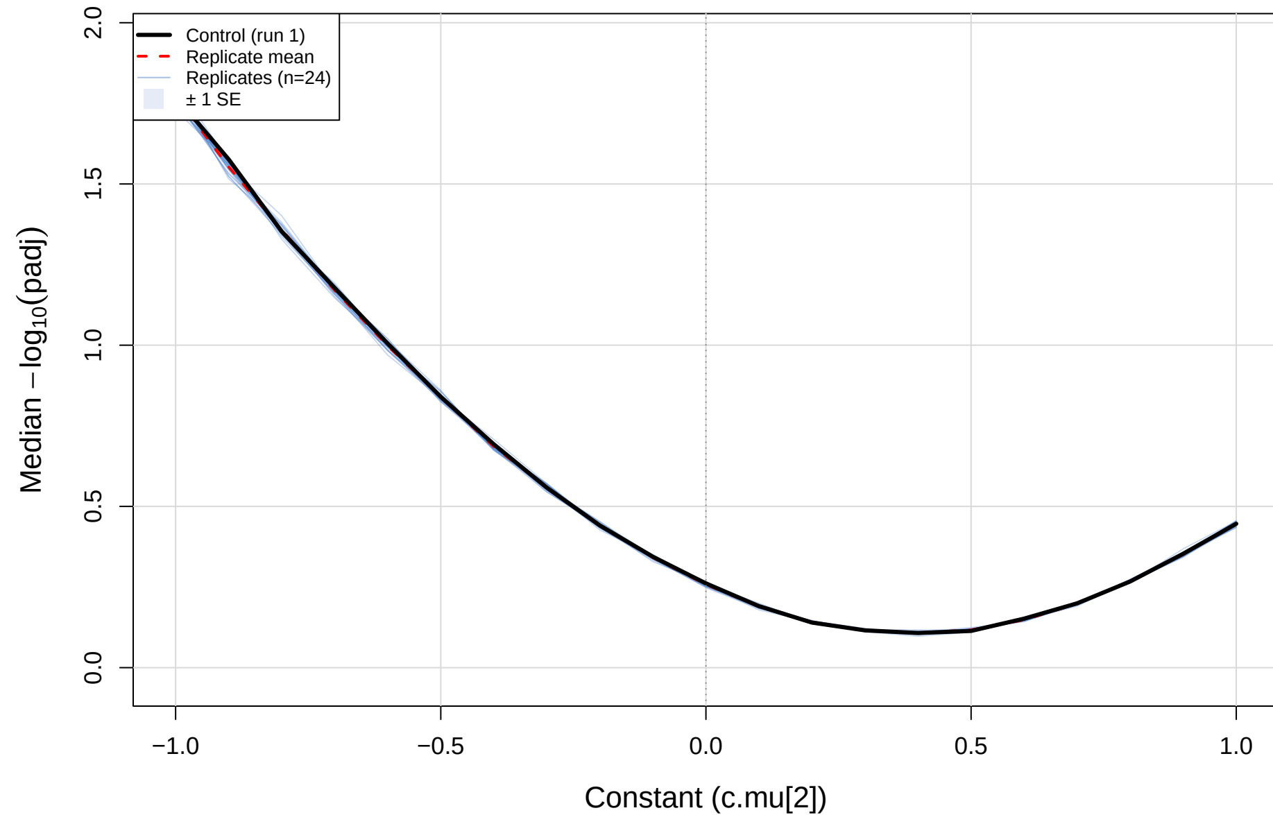
coefficient.sm vs CLR(std) vs TSS - cent_vs_mage (gamma=1e-04) Median -\log_{10}(\text{padj}) coefficient model
