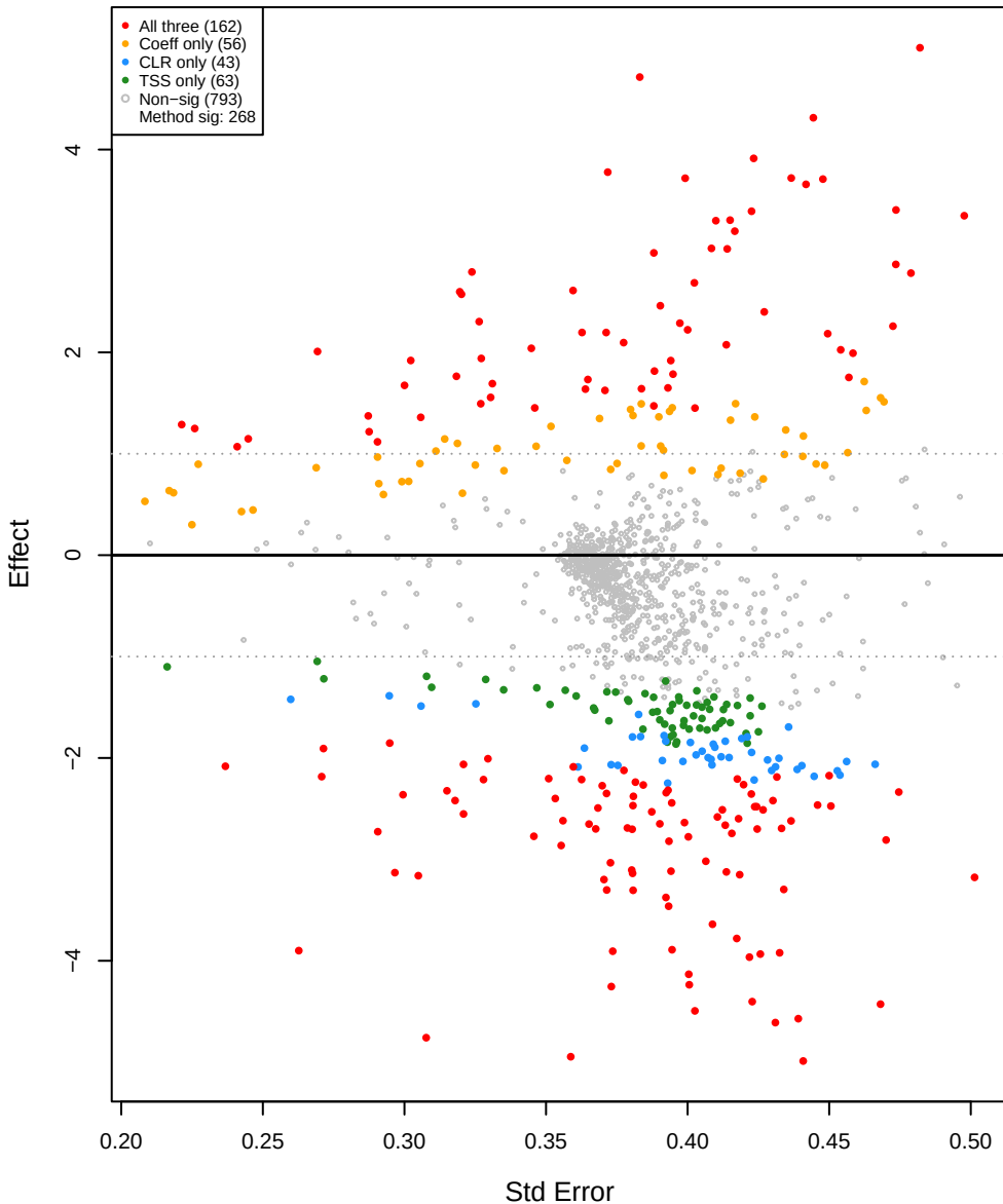
TSS(std) effect space
