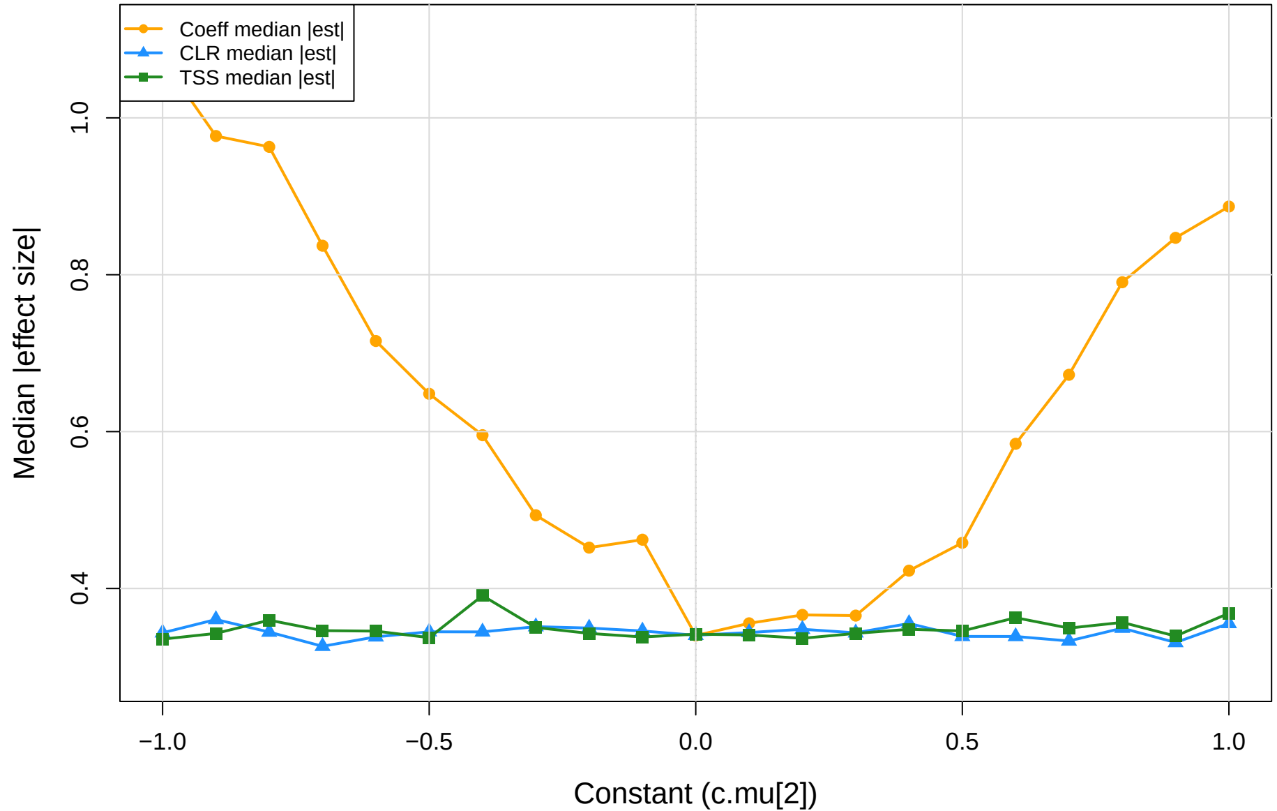
coeff.sm vs CLR vs TSS | cent vs eld | gamma=0.3 Median absolute effect size
