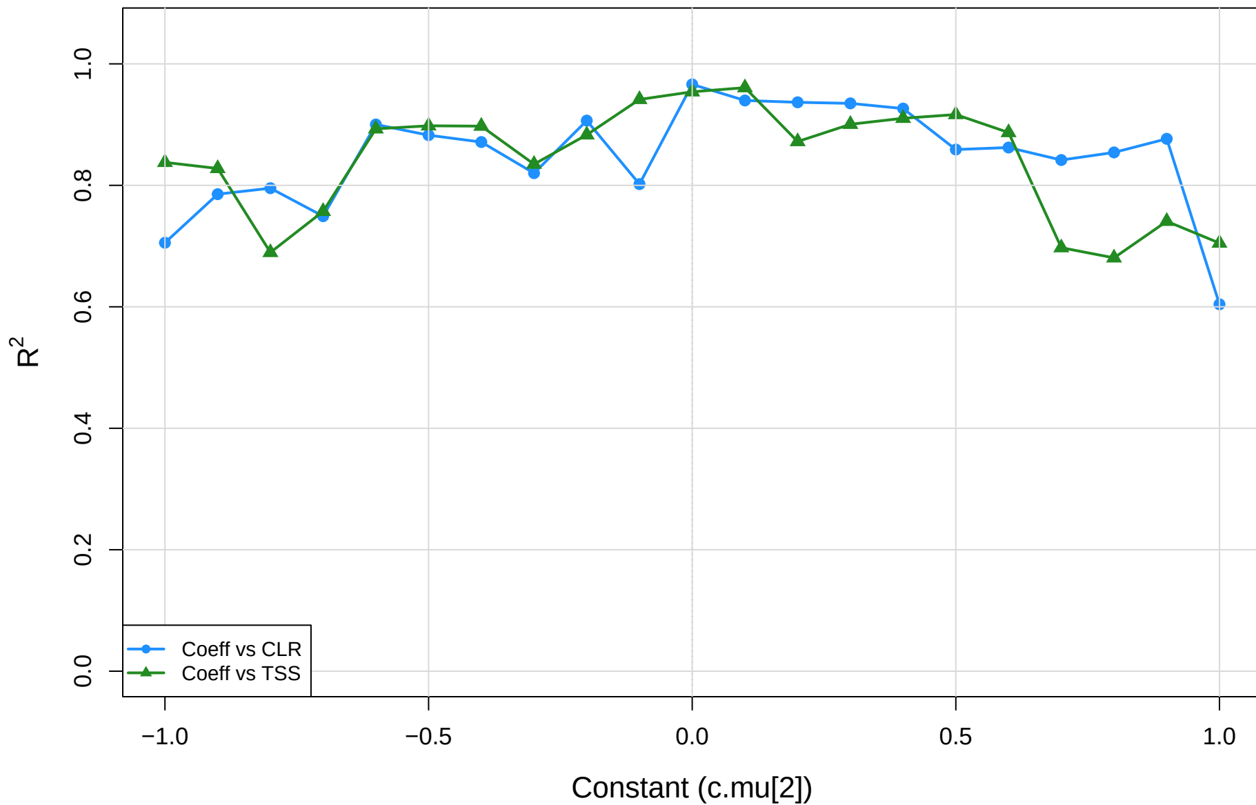
coeff.sm vs CLR vs TSS | cent vs eld | gamma=0.3 R-squared of red-dot regression
