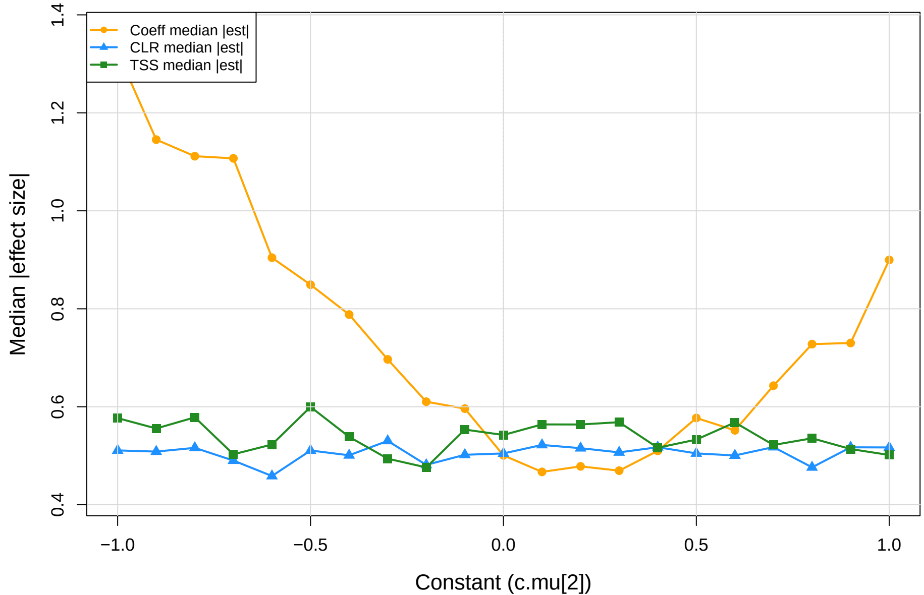
coeff.sm vs CLR vs TSS | cent vs you | gamma=0.3 Median absolute effect size
