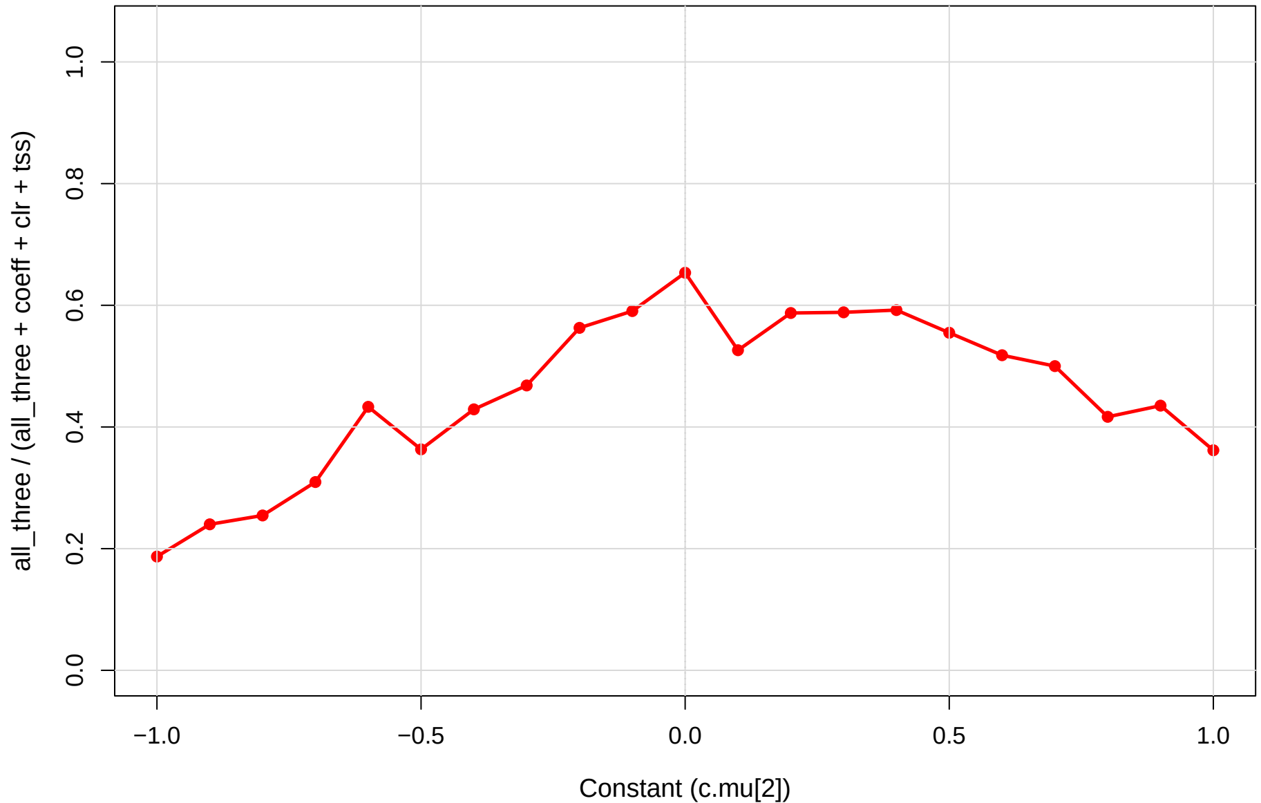
coeff.sm vs CLR vs TSS | cent vs you | gamma=0.3 Robustness (1 = all agree, 0 = max disagreement)
