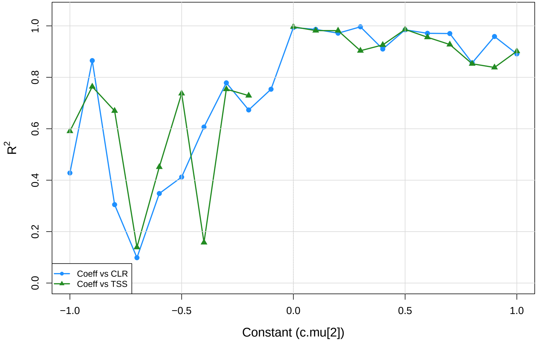
coeff.sm vs CLR vs TSS | eld vs mage | gamma=0.3 R-squared of red-dot regression
