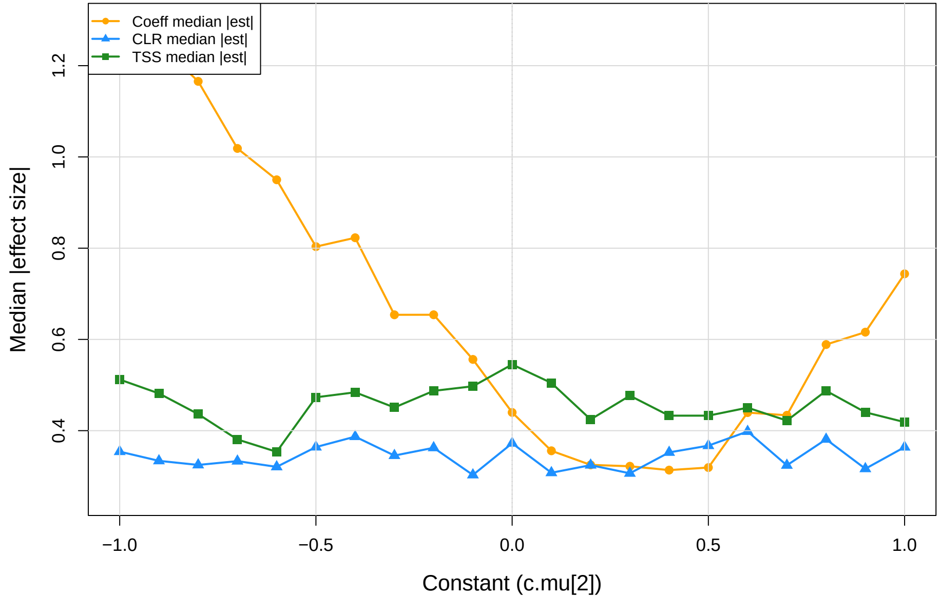
coeff.sm vs CLR vs TSS | eld vs mage | gamma=0.3 Median absolute effect size
