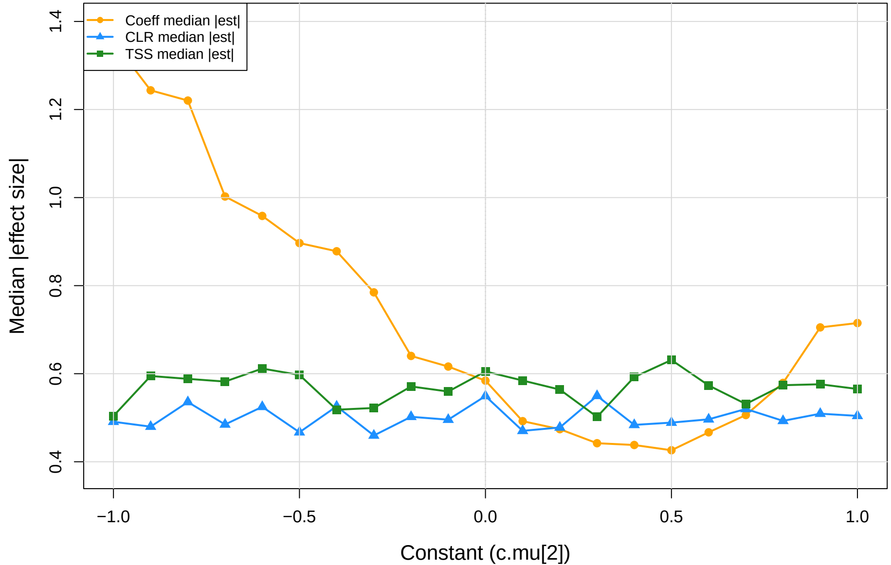
coeff.sm vs CLR vs TSS | eld vs mid | gamma=0.3 Median absolute effect size
