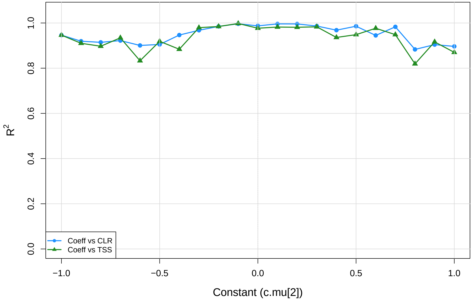
coeff.sm vs CLR vs TSS | eld vs mid | gamma=0.3 R-squared of red-dot regression
