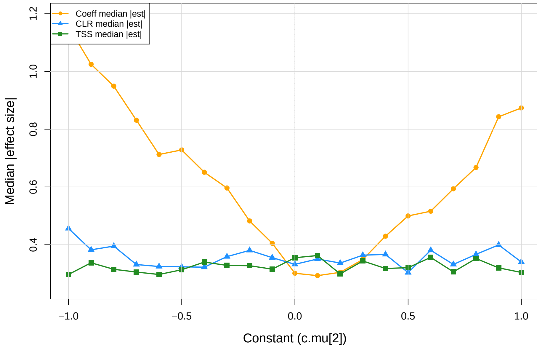
coeff.sm vs CLR vs TSS | eld vs you | gamma=0.3 Median absolute effect size
