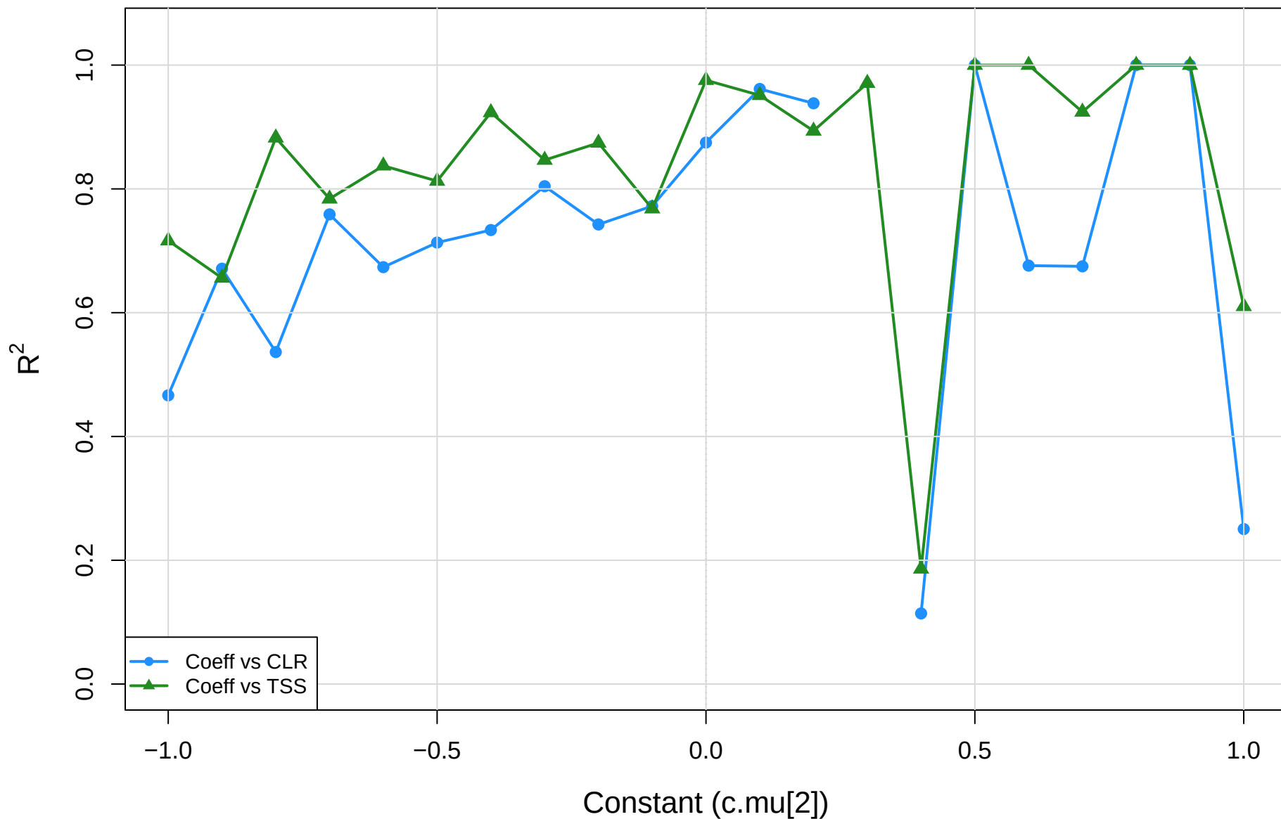
coeff.sm vs CLR vs TSS | eld vs you | gamma=0.3 R-squared of red-dot regression
