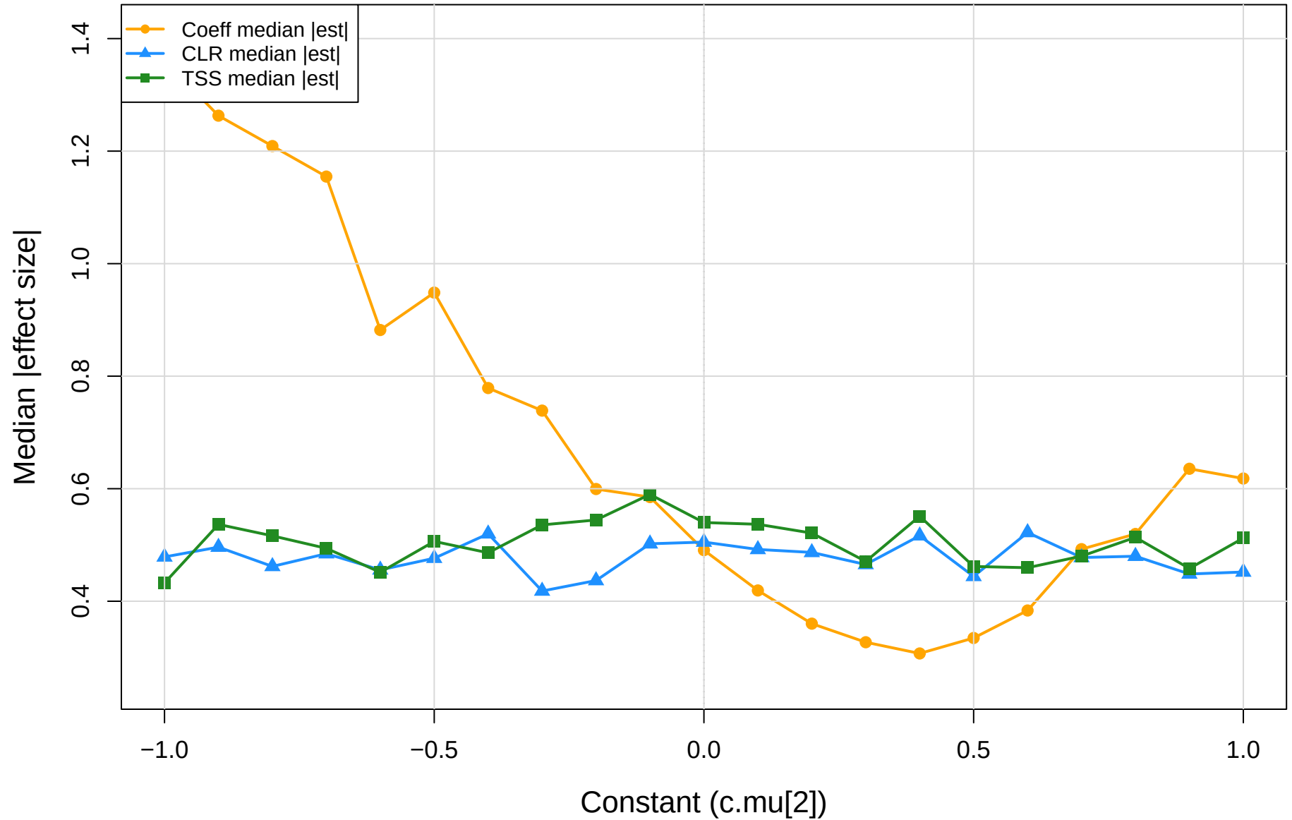
coeff.sm vs CLR vs TSS | kin vs mid | gamma=0.3 Median absolute effect size
