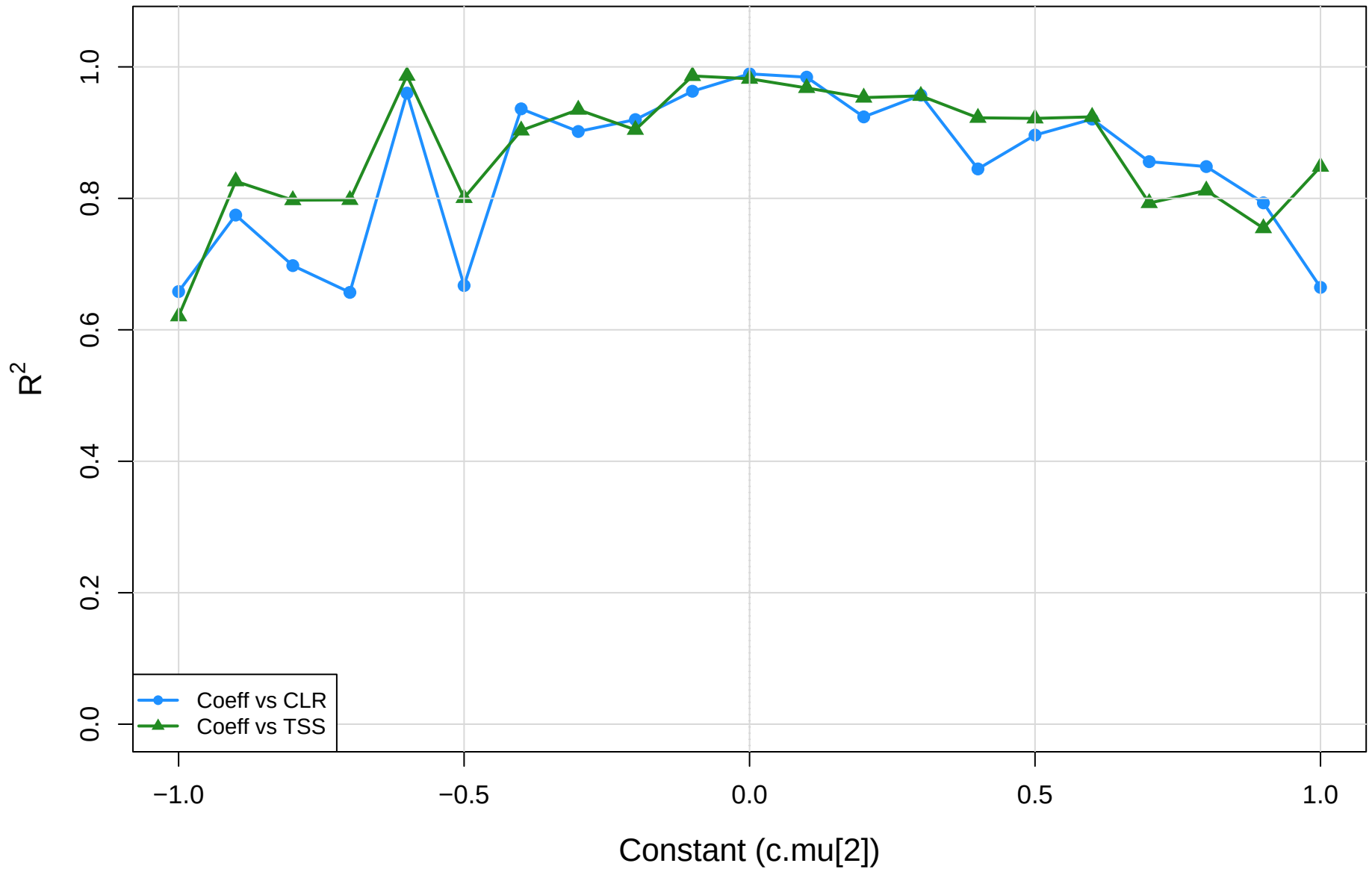
coeff.sm vs CLR vs TSS | kin vs mid | gamma=0.3 R-squared of red-dot regression
