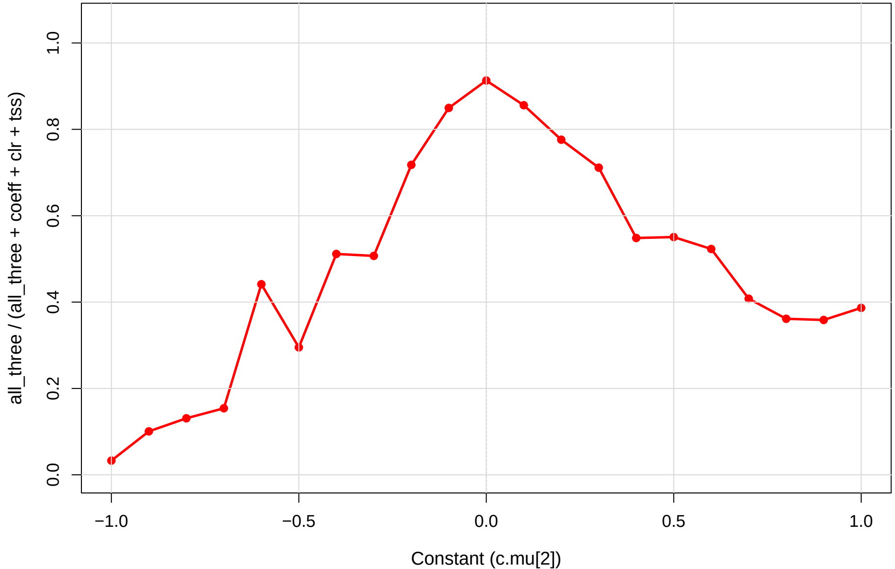
coeff.sm vs CLR vs TSS | kin vs mid | gamma=0.3 Robustness (1 = all agree, 0 = max disagreement)
