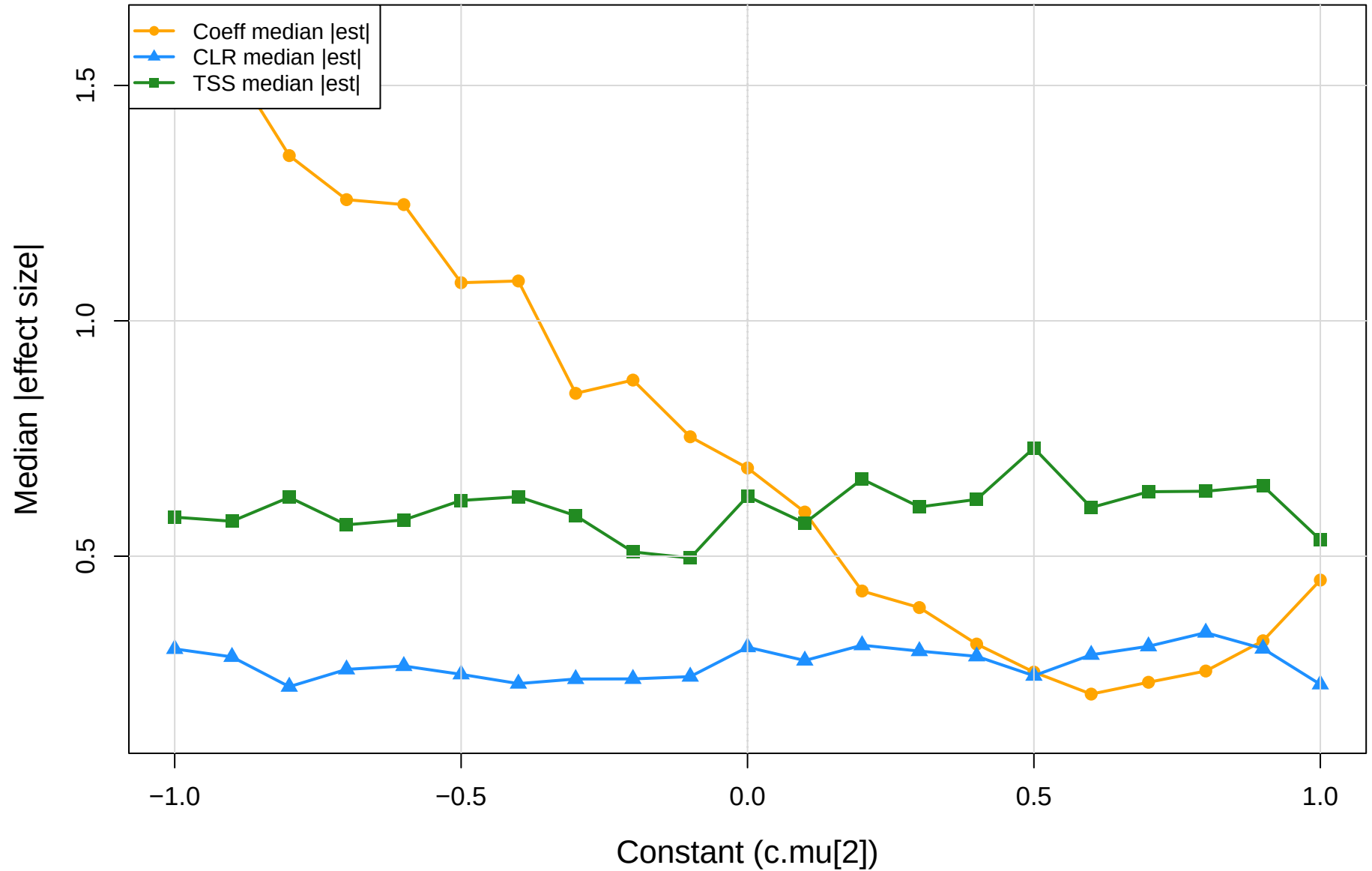
coeff.sm vs CLR vs TSS | kin vs pup | gamma=0.3 Median absolute effect size
