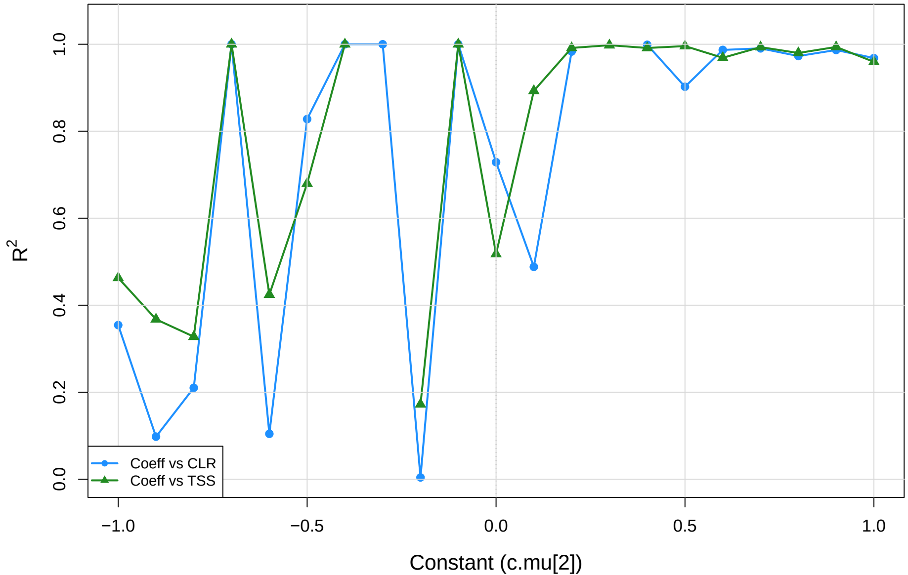
coeff.sm vs CLR vs TSS | kin vs pup | gamma=0.3 R-squared of red-dot regression
