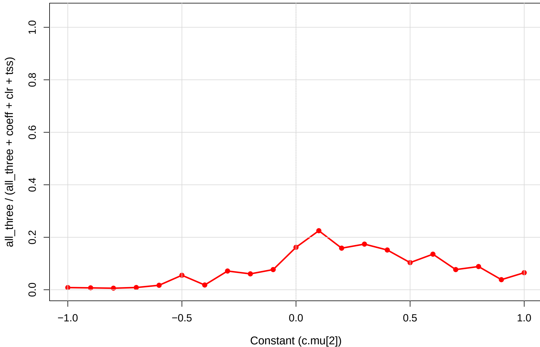
coeff.sm vs CLR vs TSS | kin vs pup | gamma=0.3 Robustness (1 = all agree, 0 = max disagreement)
