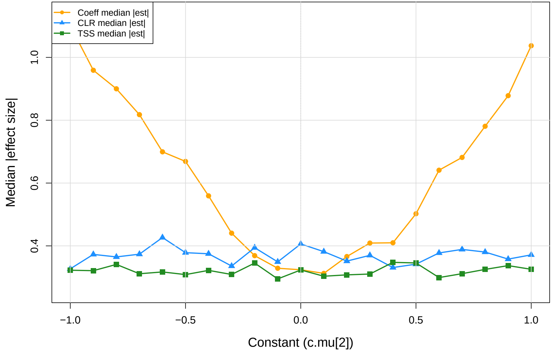
coeff.sm vs CLR vs TSS | mage vs mid | gamma=0.3 Median absolute effect size
