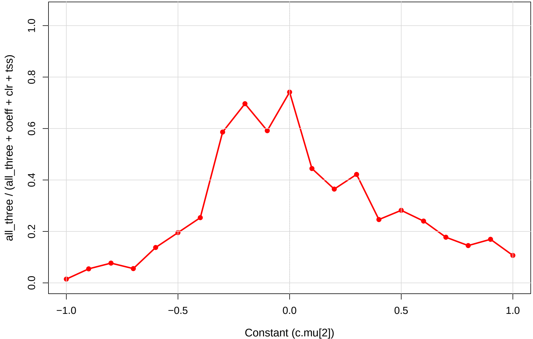
coeff.sm vs CLR vs TSS | mage vs mid | gamma=0.3 Robustness (1 = all agree, 0 = max disagreement)
