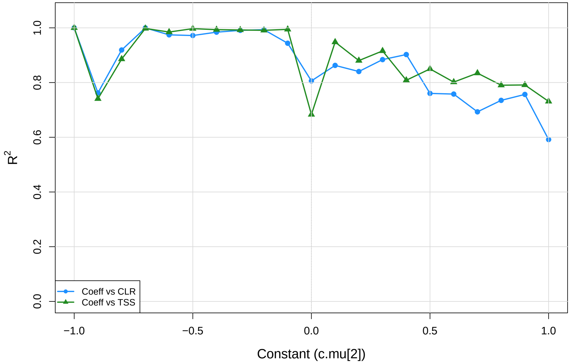
coeff.sm vs CLR vs TSS | mage vs mid | gamma=0.3 R-squared of red-dot regression
